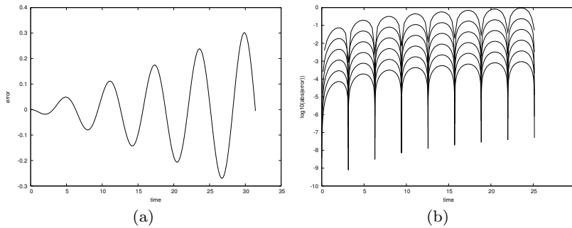
Fig. C.5 Error plots for a test problem involving an oscillating system: (a) the error as a function of time; (b) the logarithm of the absolute value of the error as a function of time, where \Delta t is reduced by one half from one curve to the next one below.
