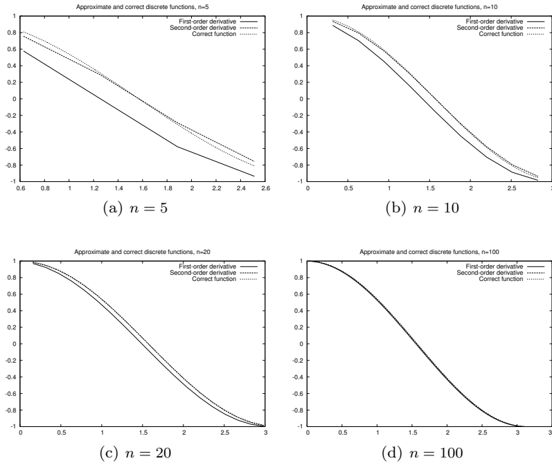
Fig. A.4 Plots of exact and approximate derivatives with various number of mesh points n .
