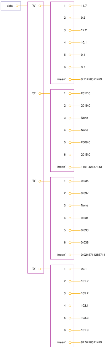
Fig. 6.1 Illustration of the nested dictionary created in the table2dict.py program.
