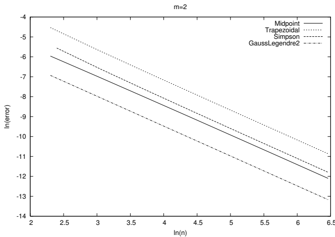
Fig. 9.5 The logarithm of the error versus the logarithm of integration points for integral \int_0^1 \sqrt[3]{x} dx computed by the Trapezoidal method and Simpson's rule (upper two lines), and Midpoint and Gauss-Legendre methods (lower two lines).
