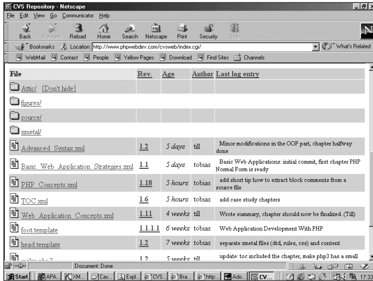
Figure 5.4 The CVSSweb interface.
