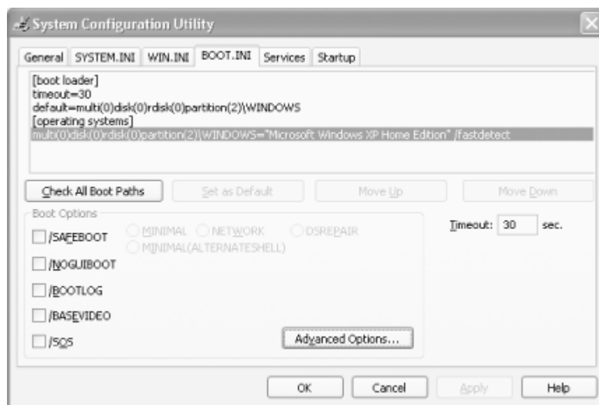
Figure 1-1. The System Configuration Utility
