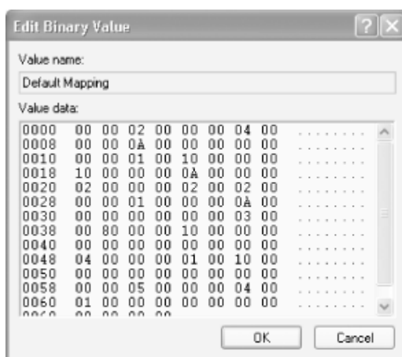
Figure 7-3. Binary values
