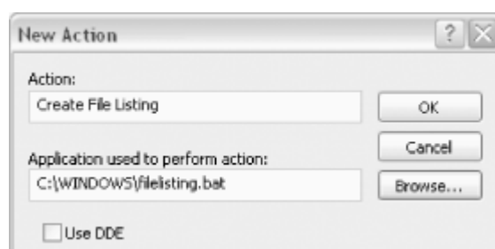
Figure 3-3. Creating a new action for the context menus
