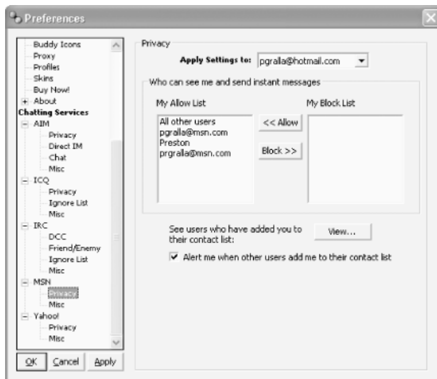
Figure 8-22. Customizing privacy options in Trillian
