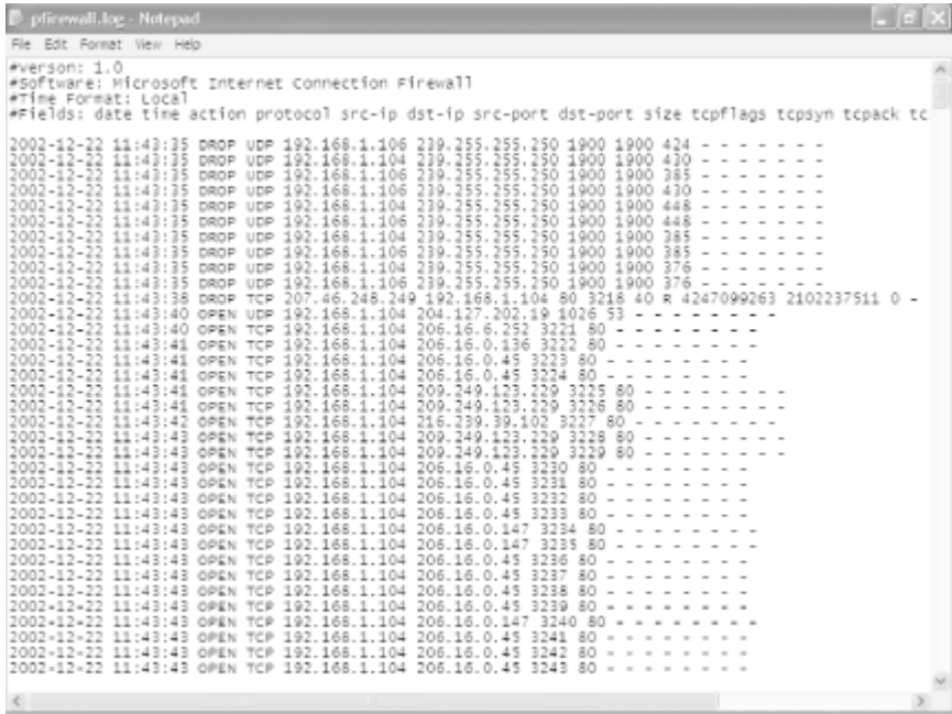
Figure 5-10. A log generated by the ICF
