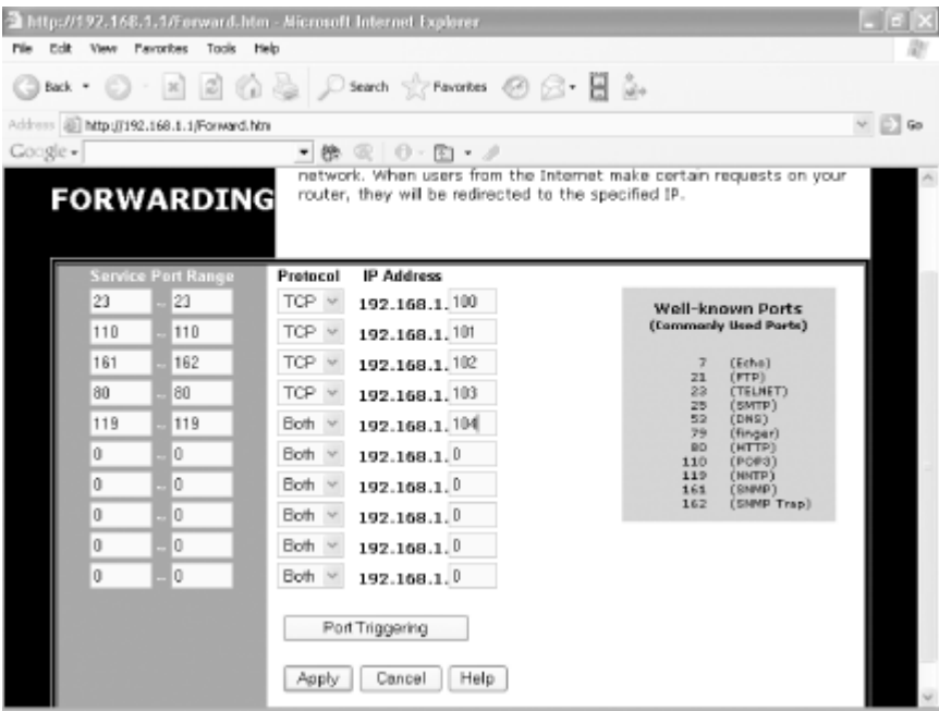
Figure 5-17. Forwarding incoming requests to the proper server or device
