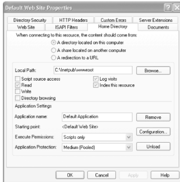
Figure 4-12. The Default Web Site Home Directory tab
