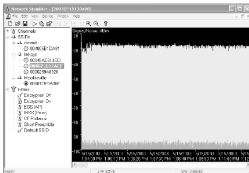
Figure 5-2. Detecting nearby wireless networks with Network Stumbler
