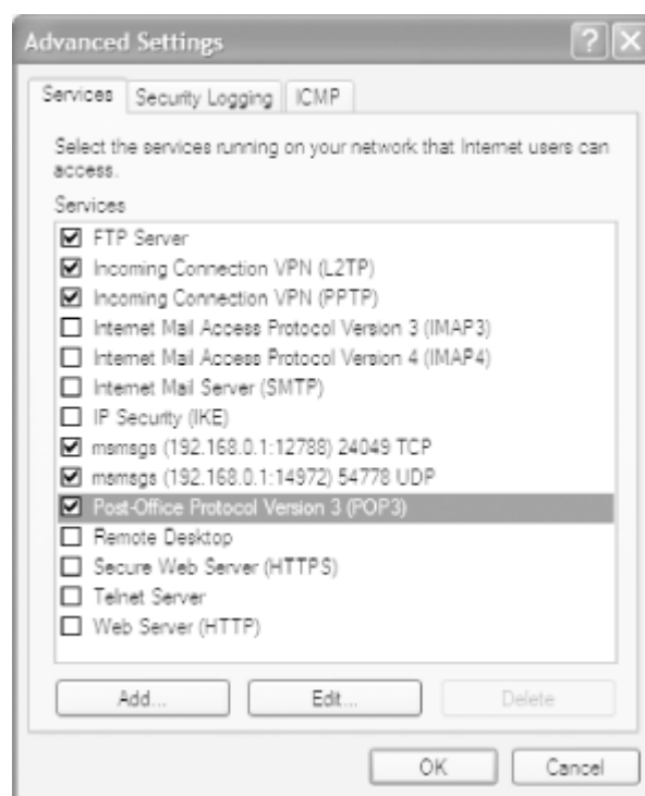
Figure 5-19. Enabling specific incoming services and traffic to bypass XP's ICF
