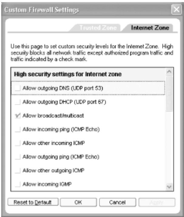
Figure 5-23. Allowing specific incoming traffic to bypass ZoneAlarm
