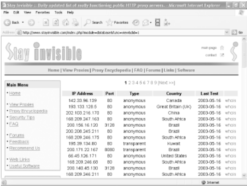
Figure 5-11. Stay Invisible's list of free public proxy servers around the world
