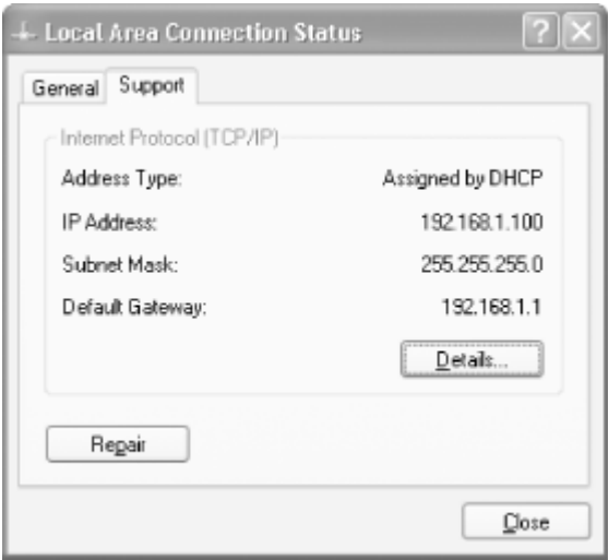
Figure 5-28. Confirming that you've gotten a new IP address
