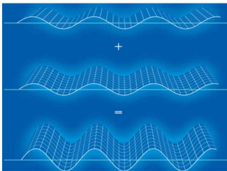
Interference Like people, when waves meet they can tend to either enhance or diminish each other.
