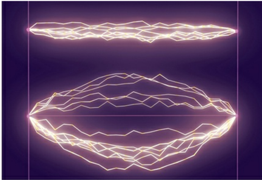
The Paths from A to B The “classical” path between two points is a straight line. The phases of paths that are near to the classical path tend to enhance each other, while the phases of paths farther from it tend to cancel out.
