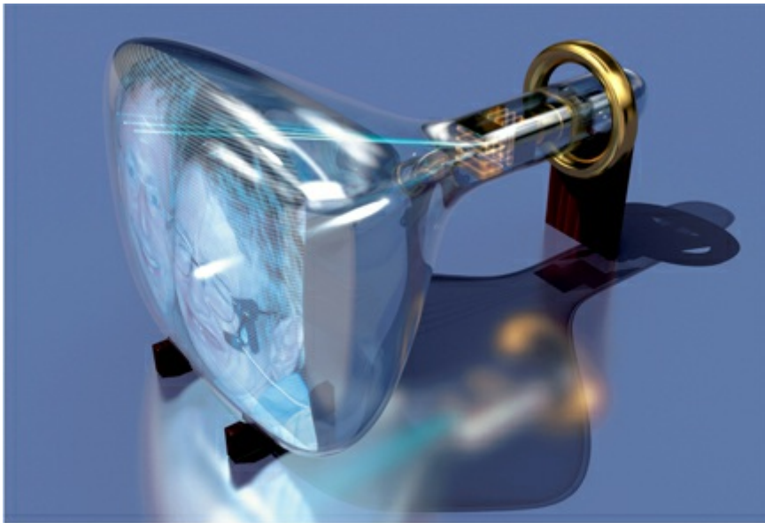
Cathode Rays We can't see individual electrons, but we can see effects they produce.
