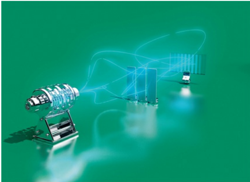
Particle Paths Feynman's formulation of quantum theory provides a picture of why particles such as buckyballs and electrons form interference patterns when they are shot through slits in a screen.
