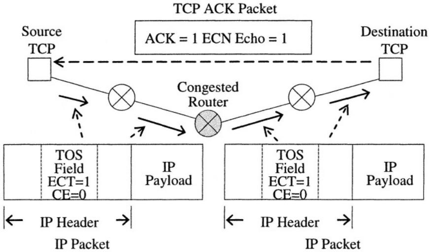
Figure 4-33. ECN operation.
