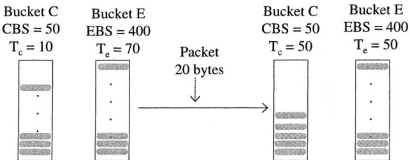
Figure 4-20. Example 5: srTCM.
