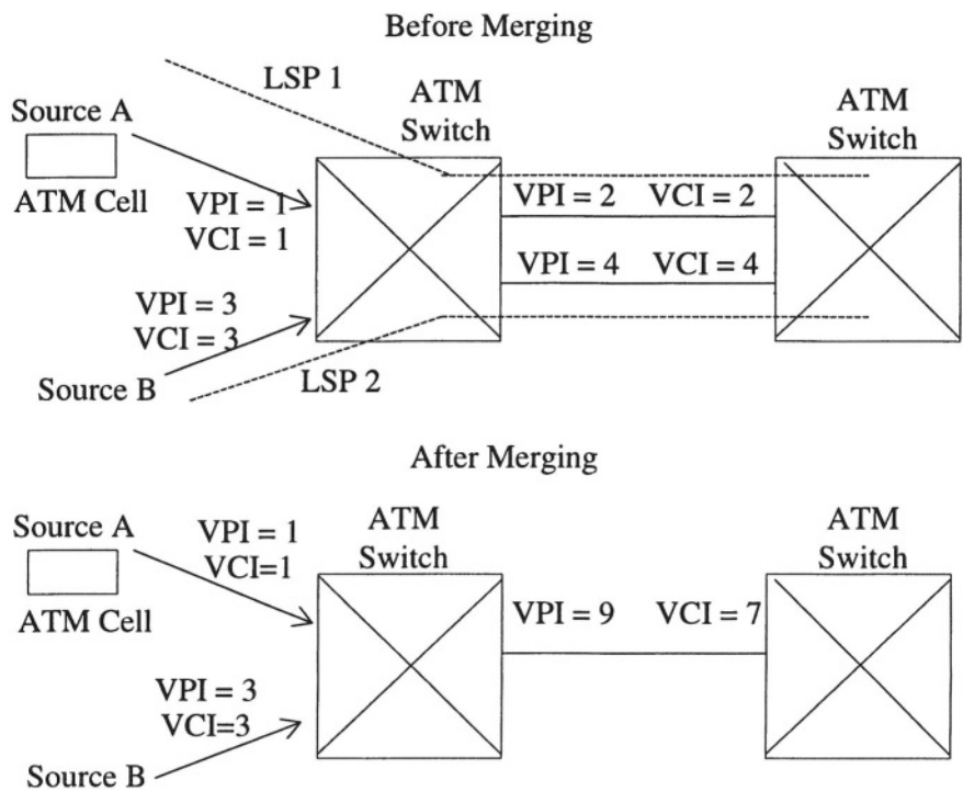
Figure 7-18. VC merging.
