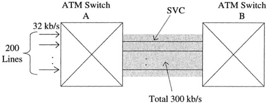
Figure 6-22. VBR CAC example.
