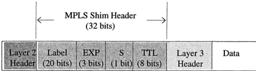
Figure 7-3. MPLS Shim header.
