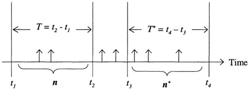
Figure 2-18. Poisson arrival.
