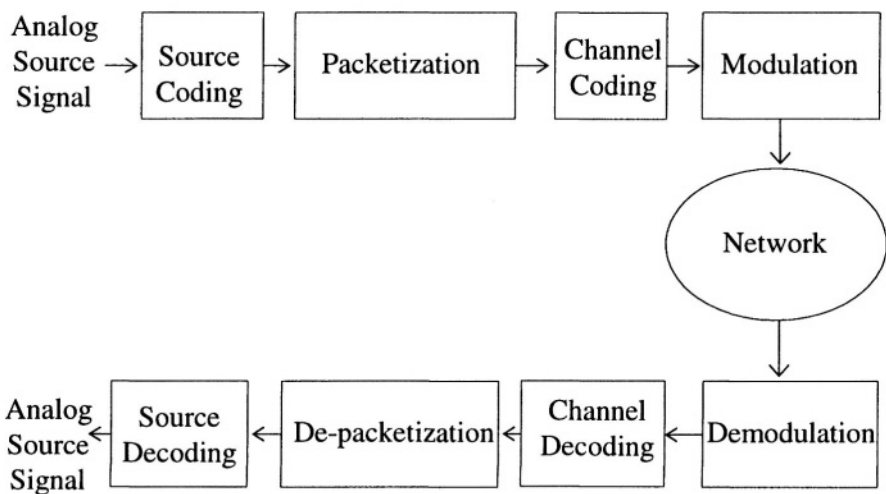
Figure 3-2. Digital communications.
