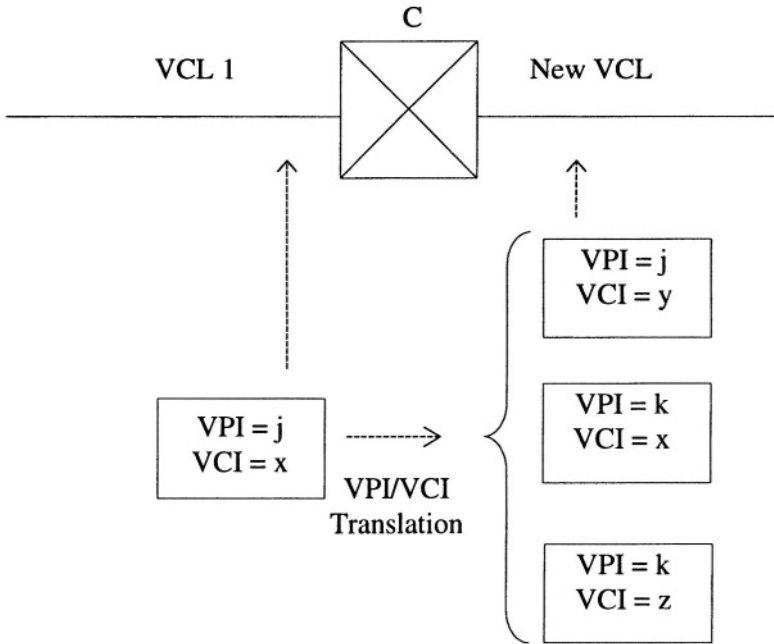
Figure 6-6. VPI/VCI Translation.
