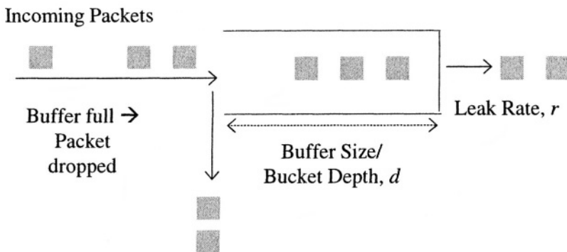
Figure 4-25. Tail drop queue management.
