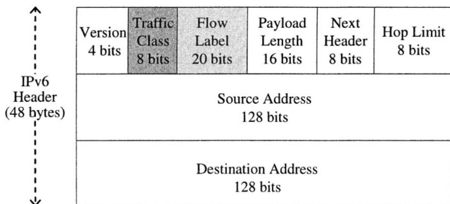
Figure 5-18. IPv6 header.
