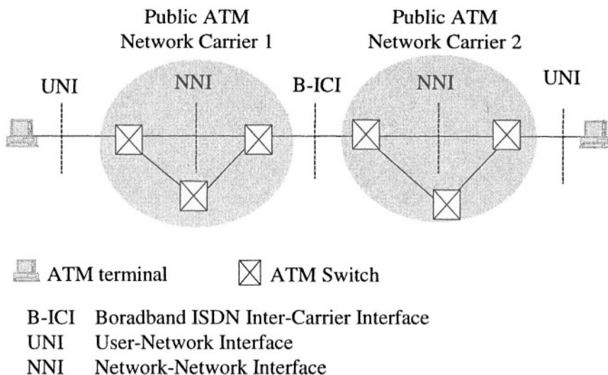
Figure 6-1. ATM interfaces.
