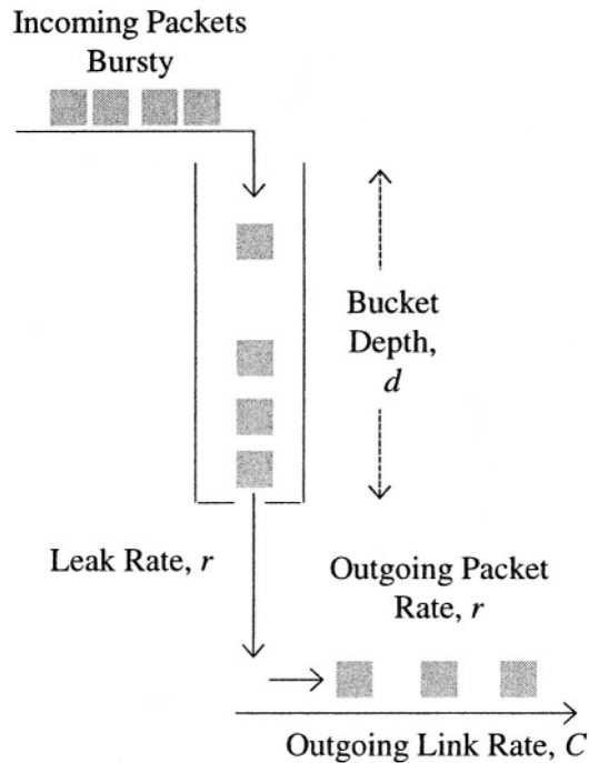
Figure 4-49. The pure traffic shaper.
