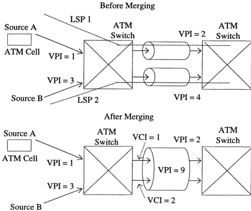
Figure 7-17. VP merging.
