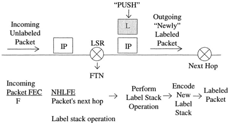
Figure 7-14. Label pushing.
