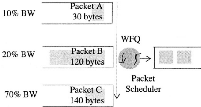
Figure 4-48. Example 11: WFQ
