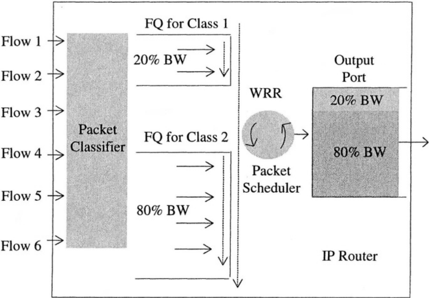
Figure 4-52. Exercise 4.
