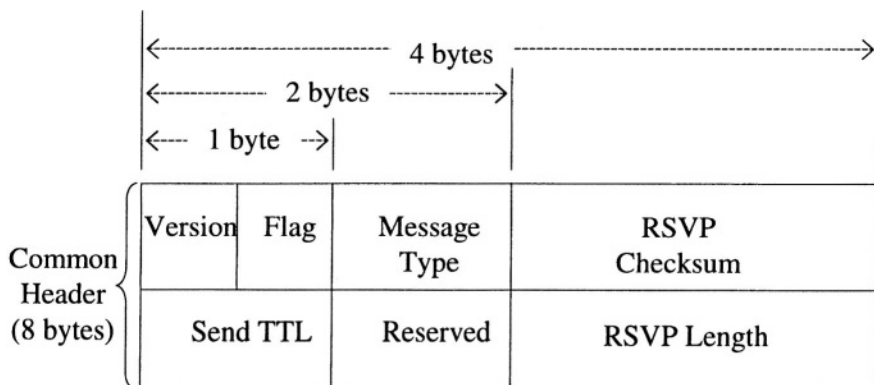
Figure 5-5. RSVP common header format.
