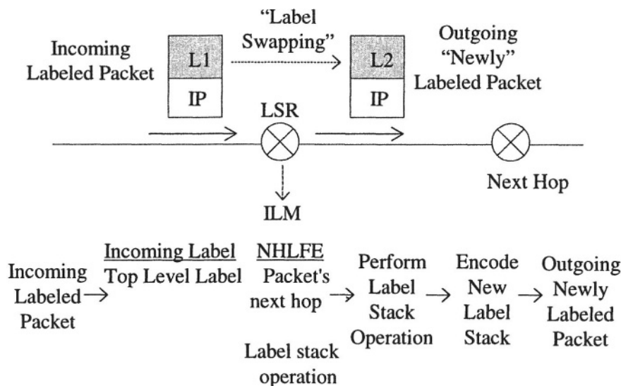
Figure 7-13. Label swapping.
