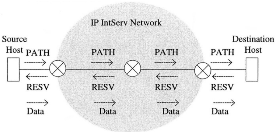
Figure 5-1. RSVP operation.
