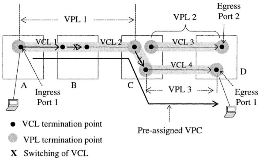
Figure 6-12. SVCC.
