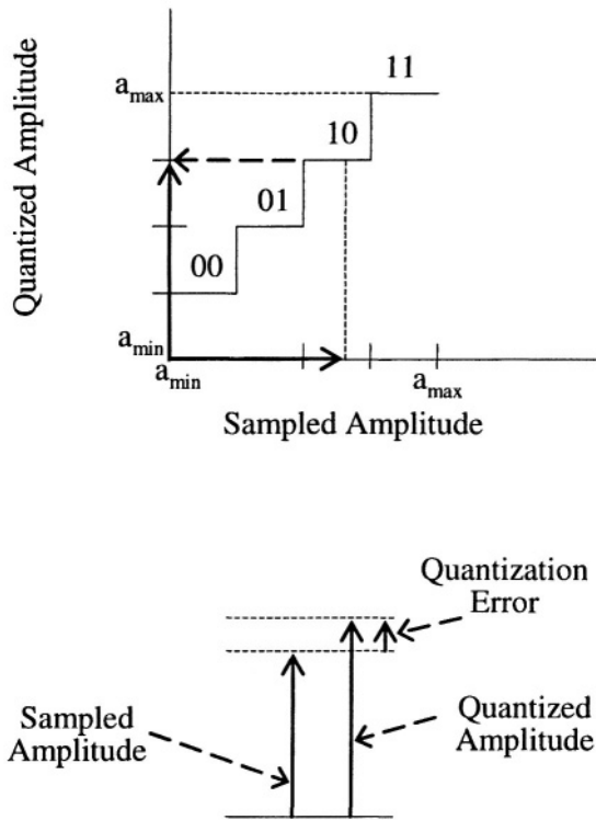
Figure 3-14. Quantization error.
