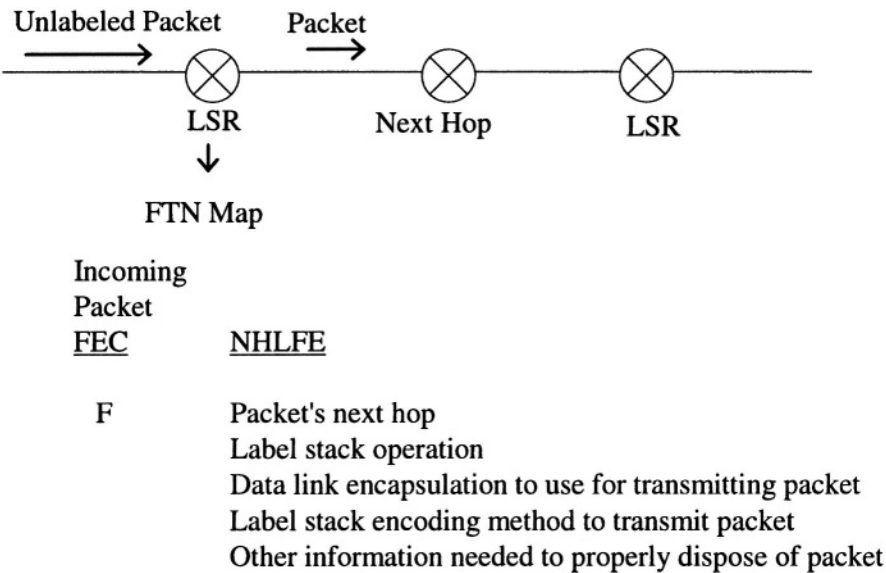
Figure 7-12. The FTN map.
