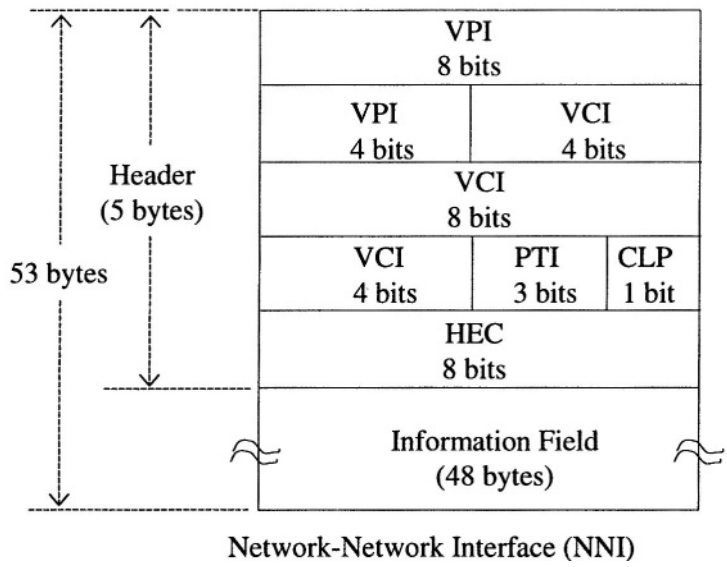
Figure 6-3. ATM cell formats.
