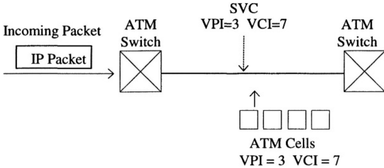
Figure 7-5. MPLS LSP using the ATM SVC.
