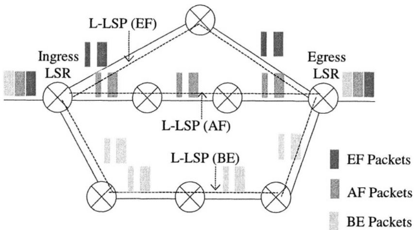
Figure 7-21. L-LSP.
