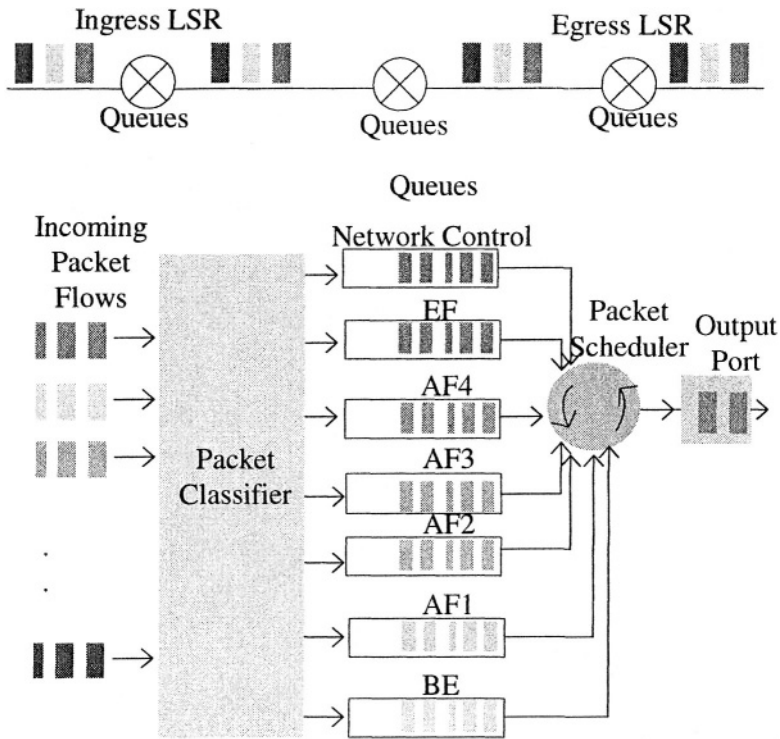
Figure 7-20. E-LSP.
