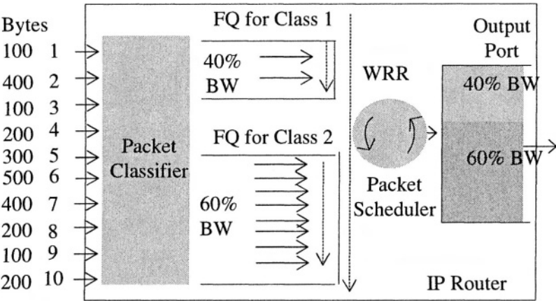
Figure 4-44. Example 10: WRR.
