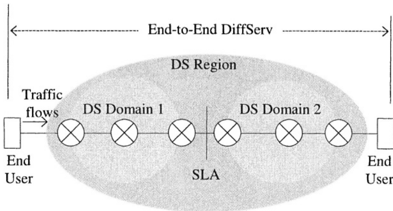
Figure 5-15. DS region.
