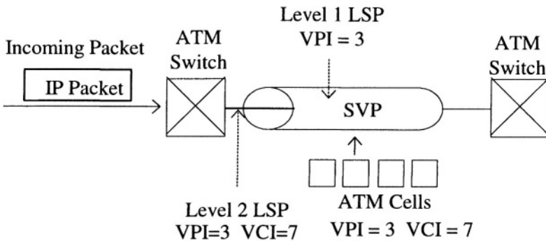
Figure 7-6. MPLS LSP by ATM SVP
