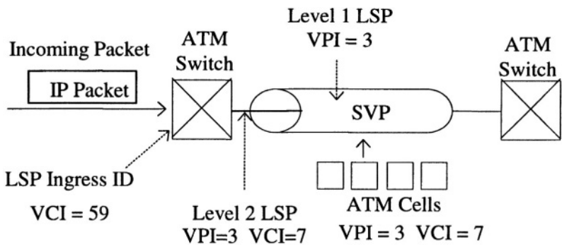
Figure 7-7. MPLS LSP by ATM SVP multipoint coding
