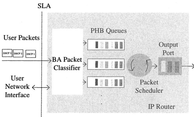
Figure 5-11. DiffServ steps.
