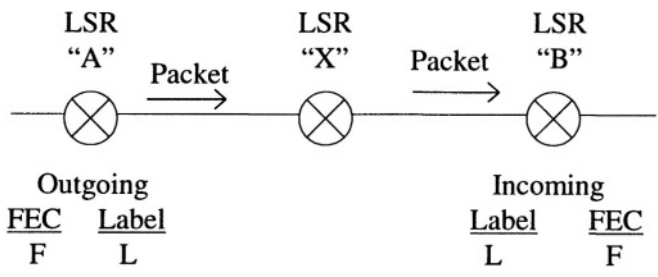
Figure 7-8. Label binding.
