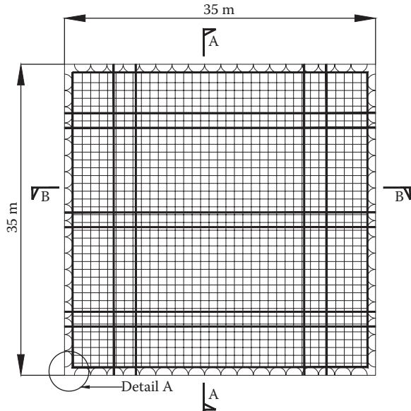
Example 7.1.2: Drawing 3: Steel rod system
