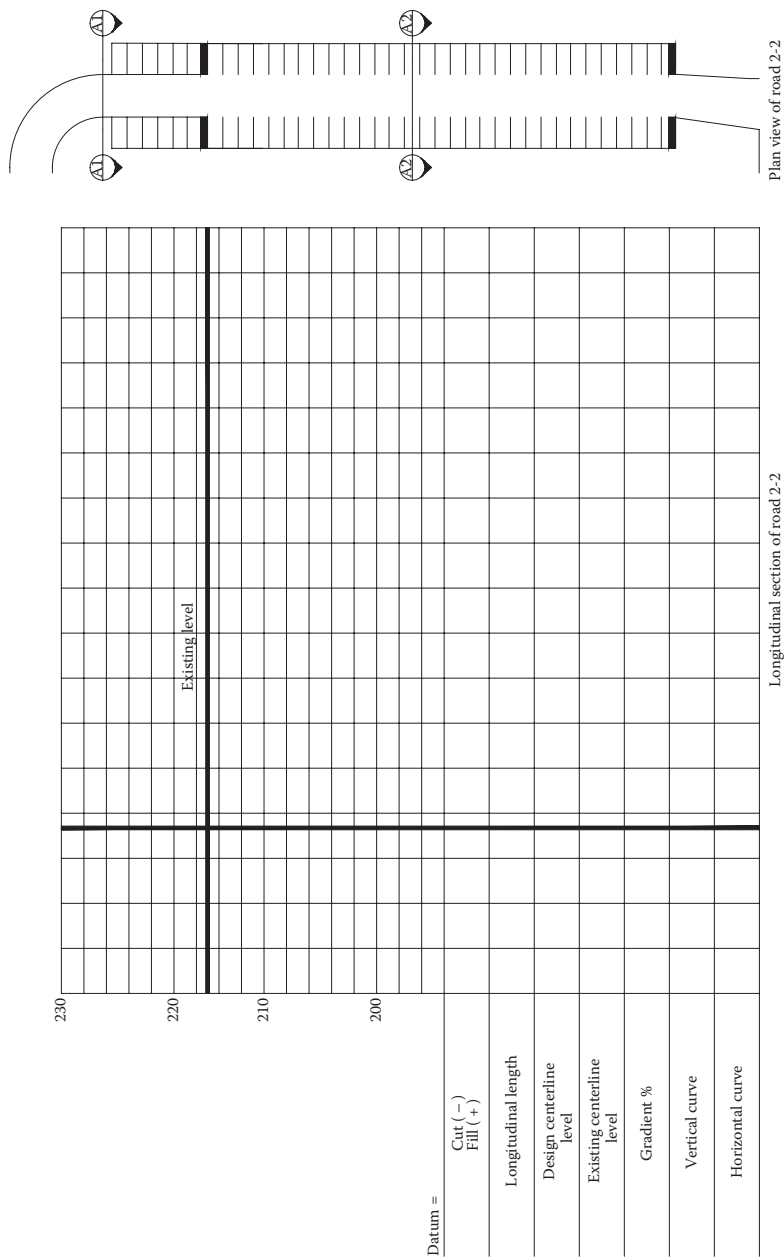
Example 7.1.1c: Road 2-2 plan and longitudinal section (not to scale)
