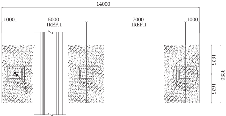
Figure 4.2 Generic illustrative comparable footing plan.
