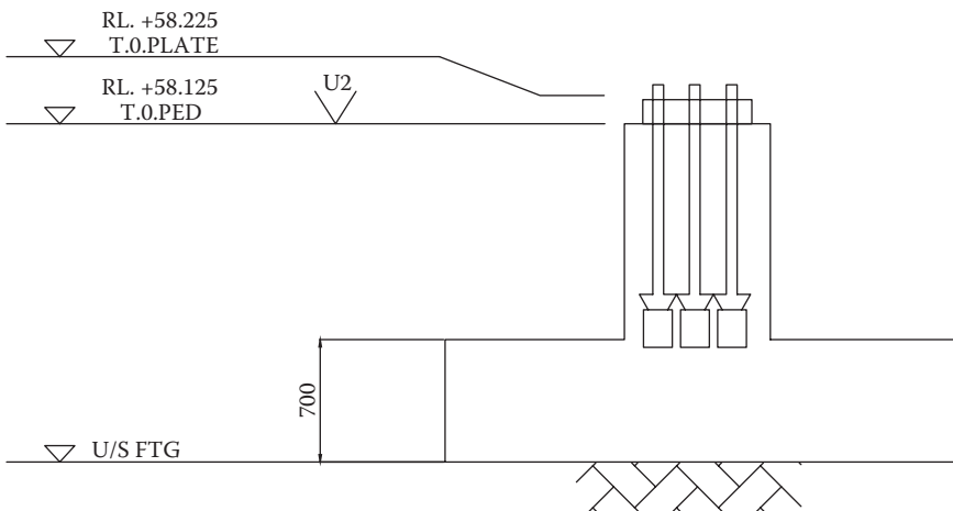
Figure 4.3 Generic illustrative section view of comparable footing (mixed method precasting).
