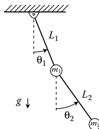
FIGURE 1.8 Planar double-compound pendulum with concentrated masses.
