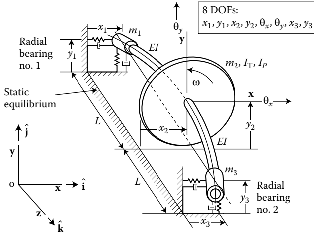
FIGURE 2.4 Simple nontrivial 8-DOF model for LRV.
