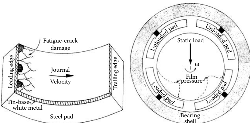
FIGURE 2.20 Four-pad tilting-pad bearing with unloaded pads.
