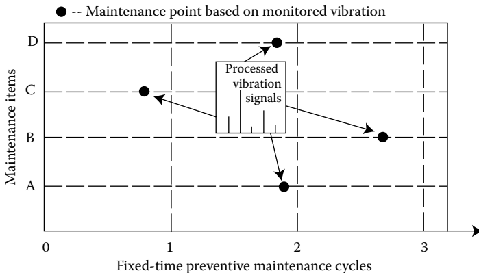
FIGURE 7.2 Predictive maintenance contrasted to preventive maintenance.
