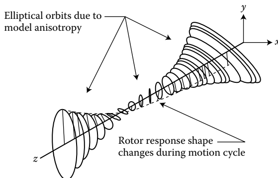
FIGURE 4.9 Response orbits of an anisotropic model with damping.
