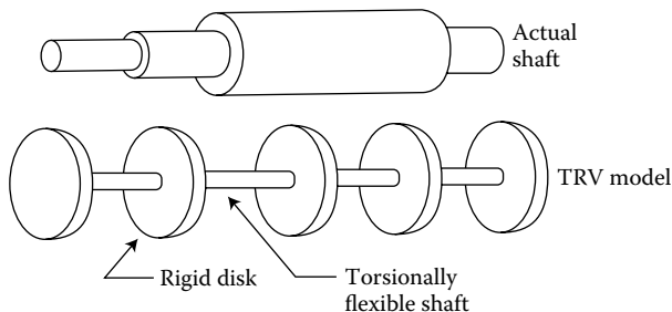
FIGURE 3.1 Multielement TRV model for a single-shaft rotor.
