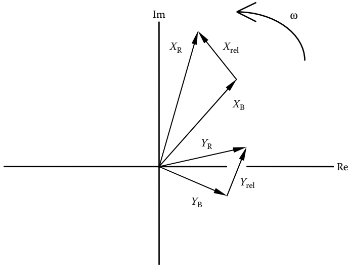
FIGURE 4.4 Rotor and bearing displacements (R, rotor; B, bearing).
