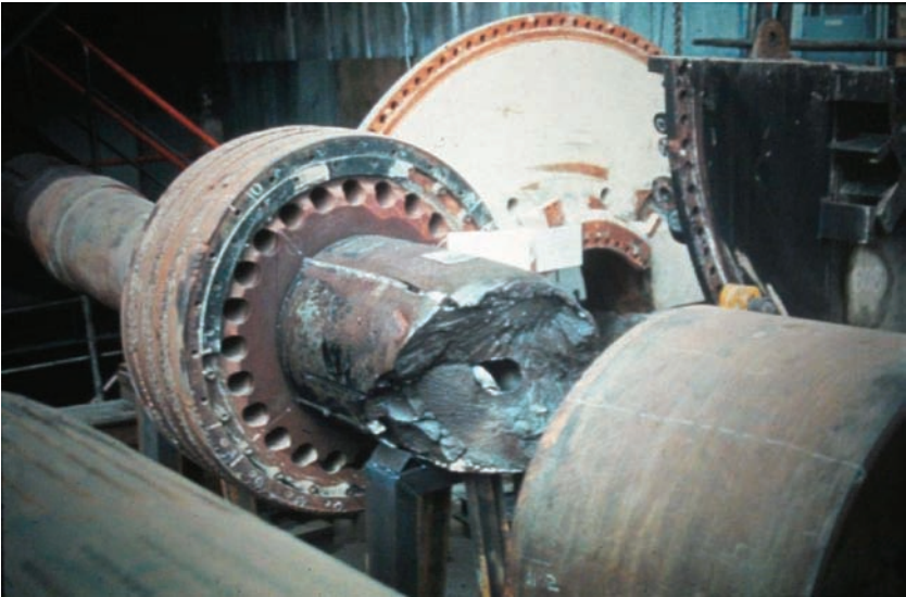
FIGURE 2.15 Photos from the two 1970s catastrophic failures of large 600 MW steam turbine-generator sets. Using nonlinear rotor dynamic response computations, failures could be potentially traced to the large unbalance from loss of one or more large LP turbine blades at running speed, coupled with behavior of fixed-arc journal bearings during large unbalance. (a) LP steam turbine outer casing. (b) Brushless exciter shaft. (c) Generator shaft. (d) LP steam turbine last stage.
