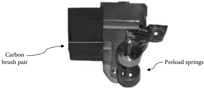
FIGURE 12.10 (See color insert following page 262.) Carbon brush pair in holder with preload springs.
