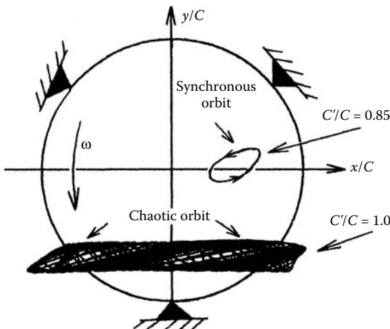
FIGURE 9.18 Chaotic rotor vibration originating in a pivoted-pad bearing.
