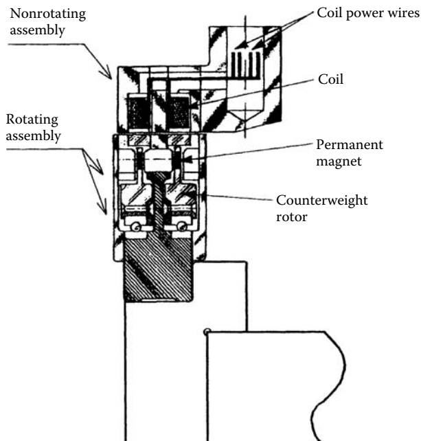
FIGURE 12.20 Lord Corporation automatic rotor mass balancer.
