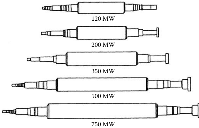
FIGURE 12.15 Maximum two-pole generator rotor sizes from the 1940s to the late 1960s.
