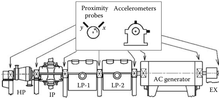
FIGURE 7.10 Vibration monitoring channels for an electric power turbine.
