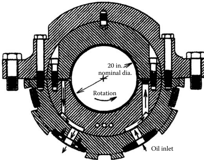
FIGURE 12.14 LP turbine bearing of a 750 MW 3600 rpm unit.
