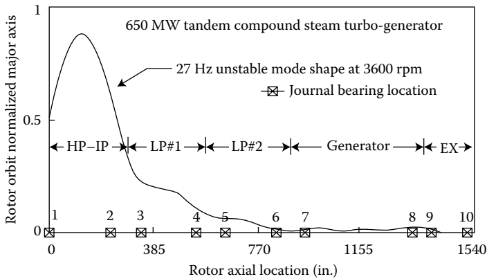
FIGURE 11.4 Steam whirl unstable mode of complete drive line.
