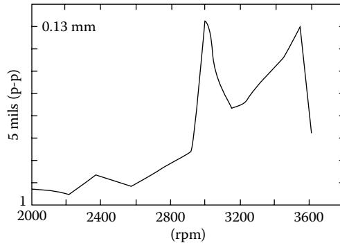
FIGURE 10.21 Measured 60 Hz vibration.
