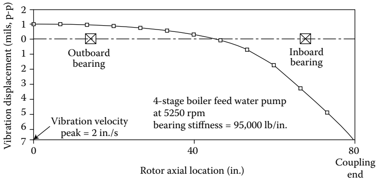
FIGURE 10.8 Critical speed rotor response shape with typical unbalances.
