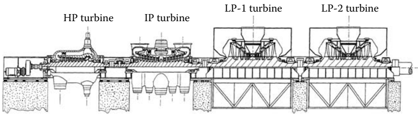
FIGURE 3.9 Turbine section of an 800 MW 3600 rpm turbo-generator (generator not shown).
