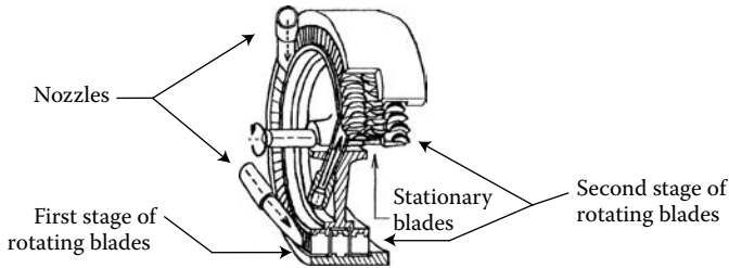
FIGURE 6.7 Laboratory impulse steam turbine stage with three nozzles.
