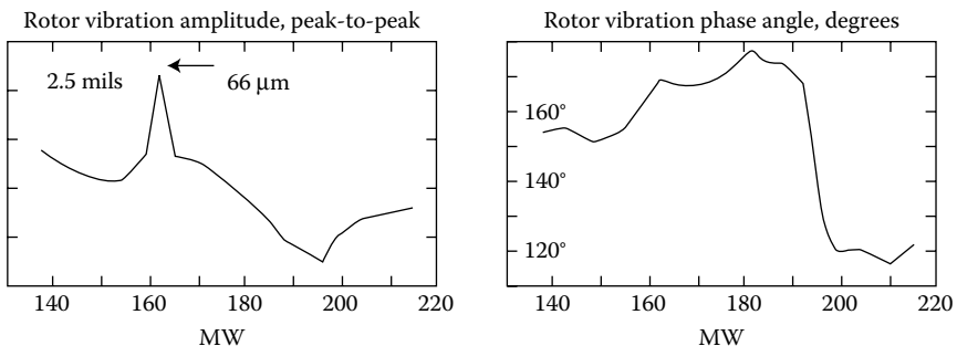
FIGURE 10.2 Measured shaft vibration versus power at HP-IP bearing no. 2.
