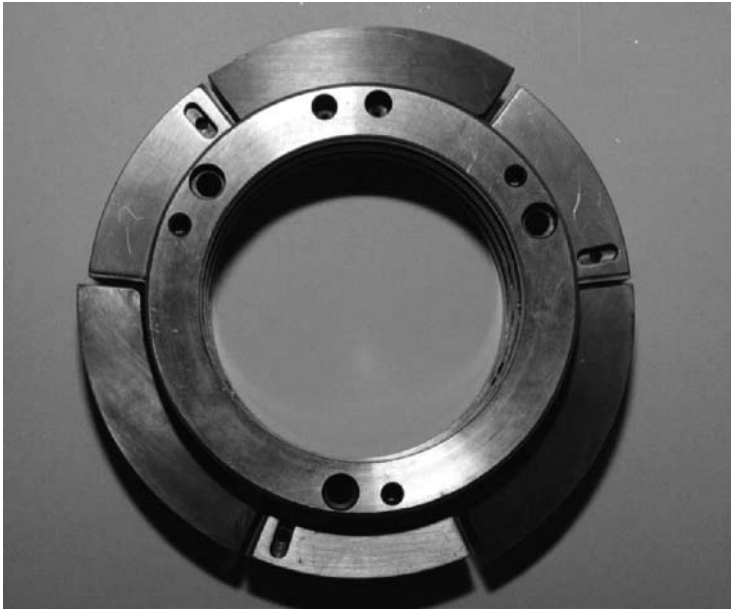
FIGURE 5.8 (See color insert following page 262.) Photo of three-pad inside-out PPJB with three copper pads to facilitate heat removal; three steel thrust sectors.
