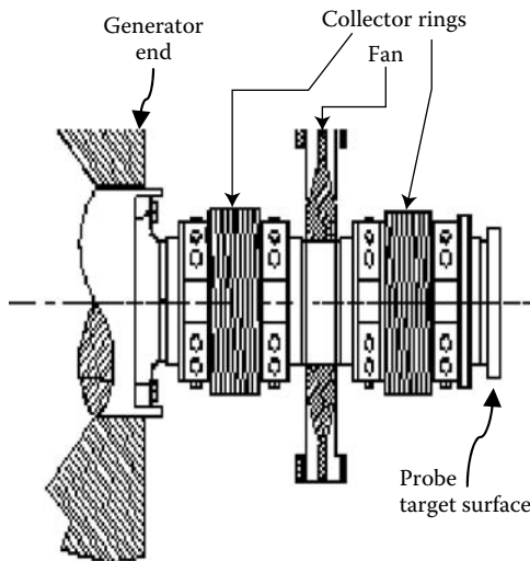
FIGURE 10.20 Collector shaft.
