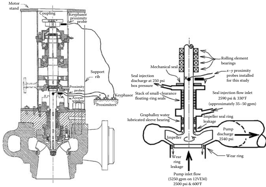
FIGURE 10.17 Boiler circulation pump: (a) cross section and (b) seal injection.
