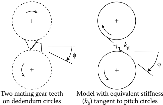
FIGURE 3.7 TRV-flexible gear-set model ( \phi \equiv gear pressure angle).
