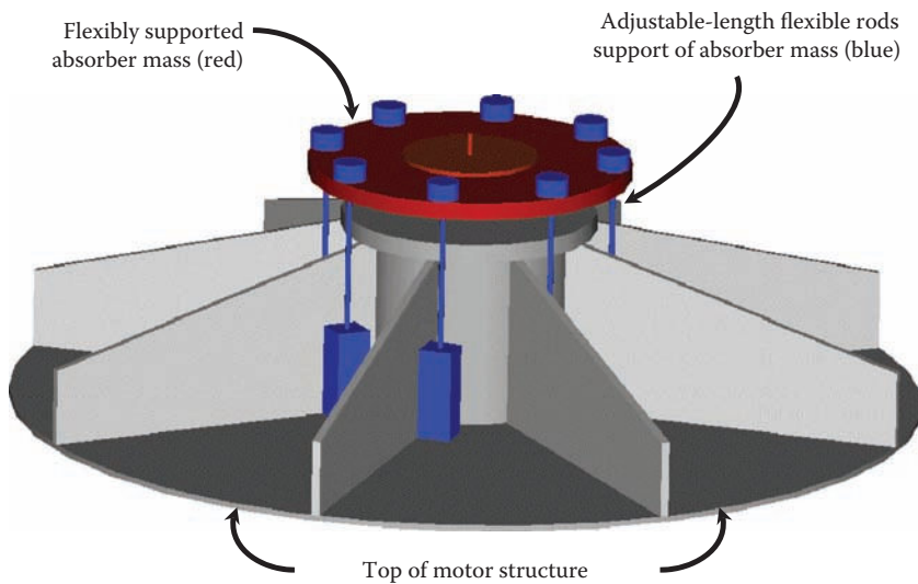
FIGURE 10.19 Vibration absorber (blue and red) atop pump motor.
