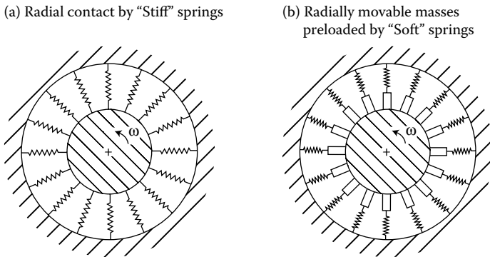
FIGURE 12.5 Rub force modulation models: (a) stiffness modulated and (b) inertia modulated. (Adams, M. L. and Pollard, M. A., Rotor Vibration Vector Turning Due to Rotor Rubs , Proceedings of the EPRI Symposium on Trouble Shooting Power Plant Rotating Machinery Vibrations, LaJolla, CA, May 19–21, 1993.)
