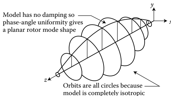
FIGURE 4.7 Isotropic model with no damping and very near resonance gives circular orbits that are all in phase.
