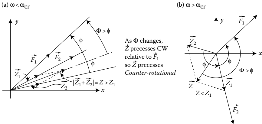
FIGURE 12.4 Stiffness modulated simple 2-DOF isotropic model.
