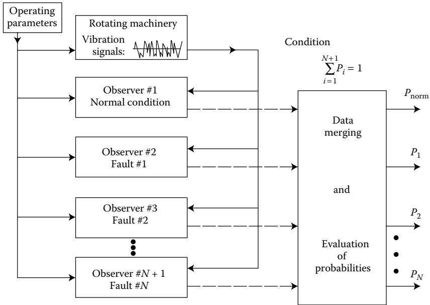
FIGURE 7.4 Real-time probabilities for defined faults and severity levels from statistical correlation of monitored and model-predicted vibration signals.
