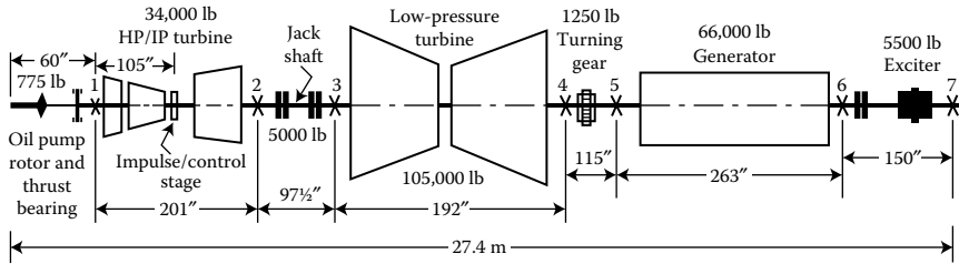
FIGURE 10.3 Rotor vibration model for 240 MW 3600 rpm turbine generator.
