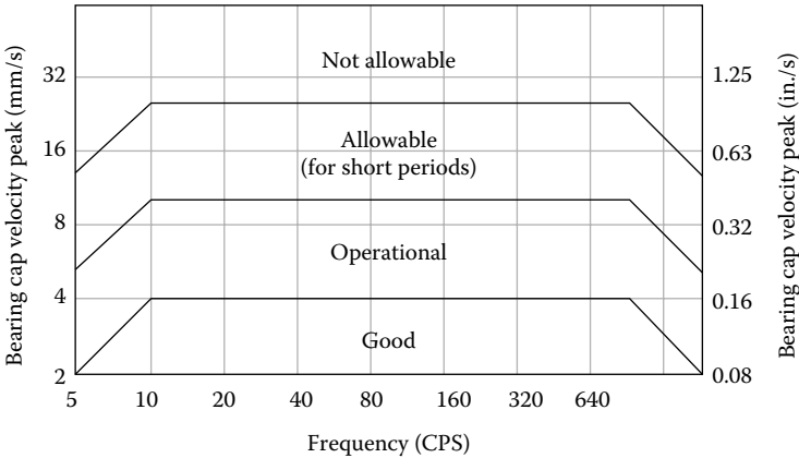
FIGURE 8.2 Bearing cap vibration velocity peak guideline.
