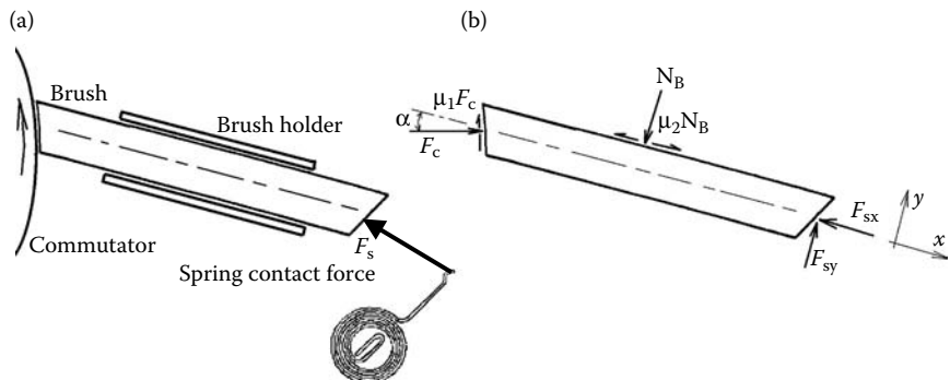
FIGURE 12.11 (a) Brush, holder, and spring. (b) Force free-body diagram of brush.
