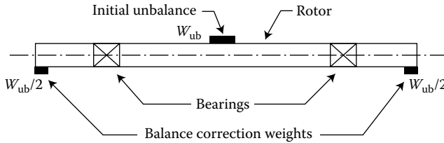
FIGURE 12.17 Simple uniform diameter flexible rotor.
