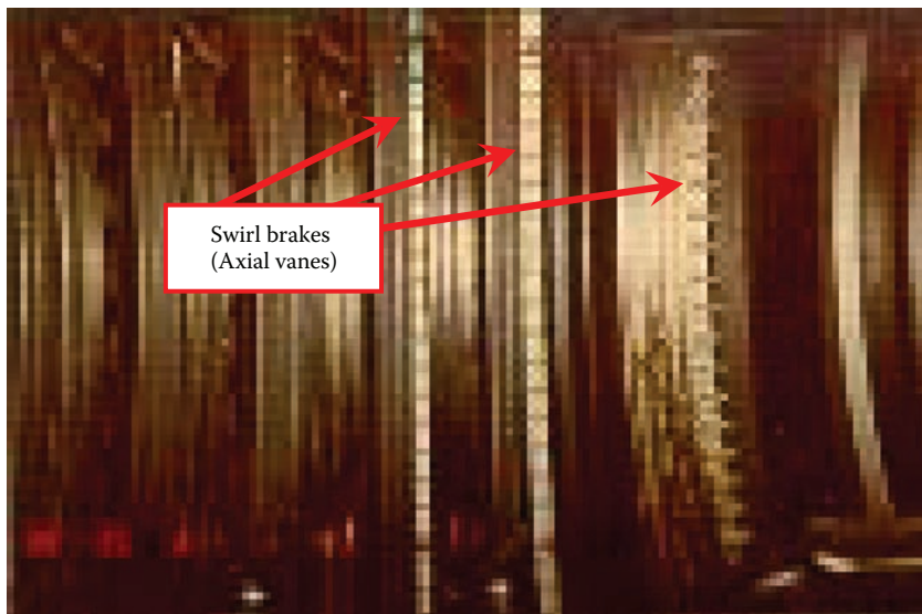
FIGURE 11.3 HP turbine swirl brakes on a 1300 MW steam turbine.
