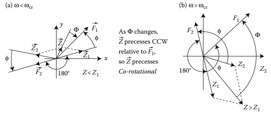
FIGURE 12.6 Inertia-modulated simple 2-DOF isotropic model.
