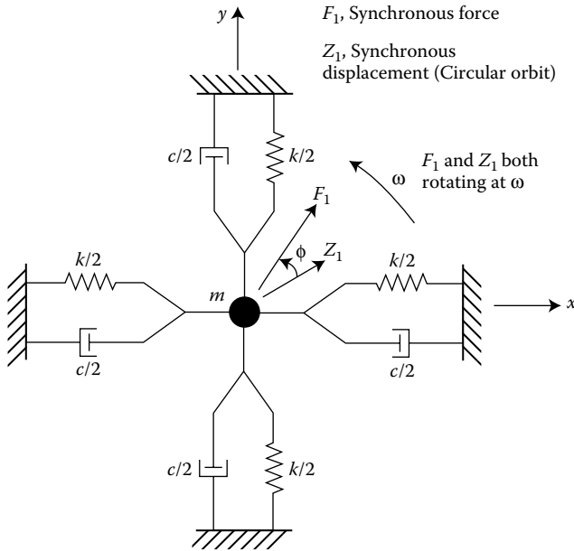
FIGURE 12.3 Simple 2-DOF model for rub-induced “vector turning” vibration.
