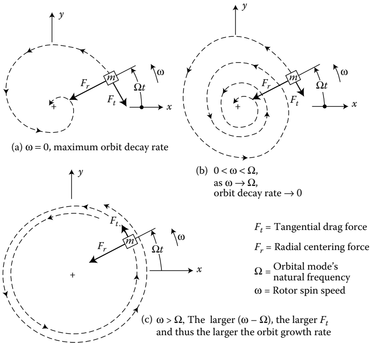
FIGURE 9.21 Transient orbits if rotor-based damping is the only damping present.
