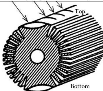
FIGURE 12.16 Rotor construction for two-pole generators.
