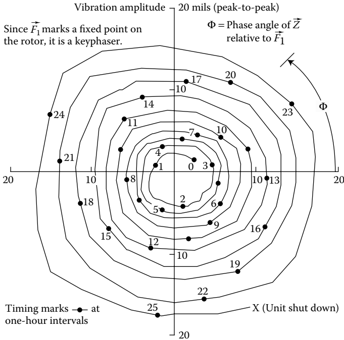
FIGURE 12.2 Polar plot of exciter journal vibration ( Z ) over 1 day.
