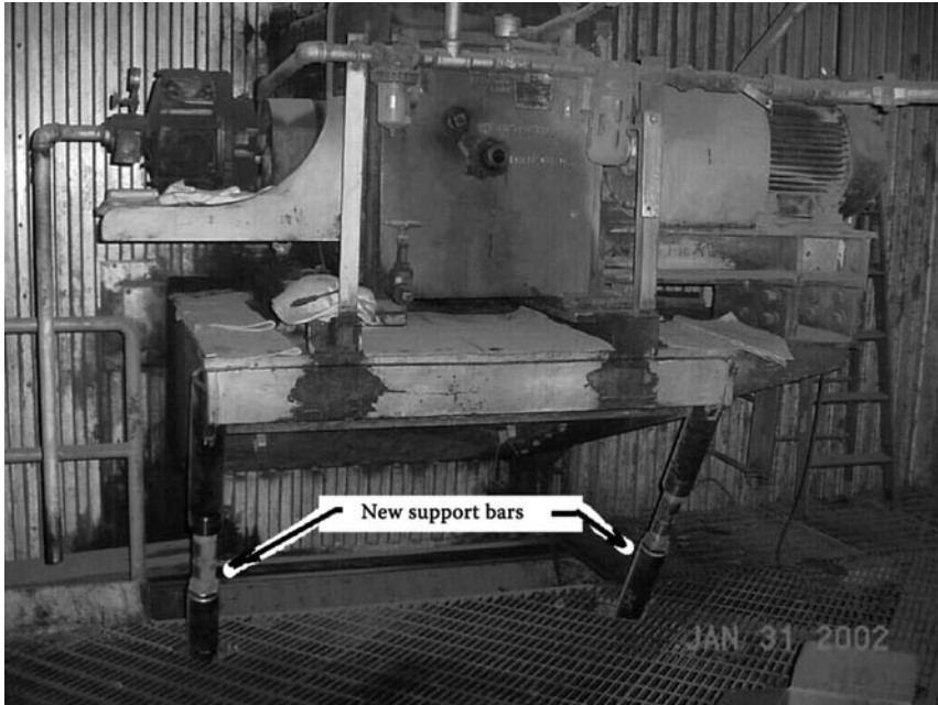
FIGURE 12.7 (See color insert following page 262.) Air preheater drive/platform with overhang support bars.
