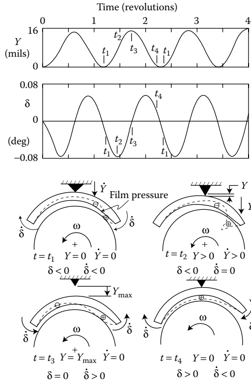
FIGURE 2.21 Simulation results of unloaded pad self-excited vibration.
