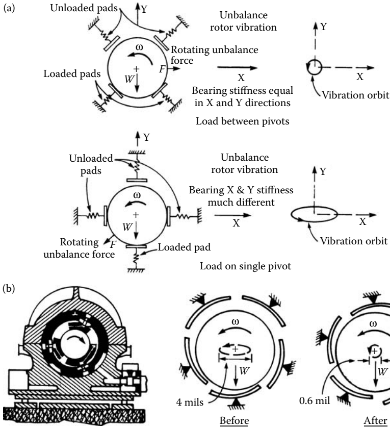
FIGURE 5.5 Load-direction vibration factors of tilting-pad journal bearings.
