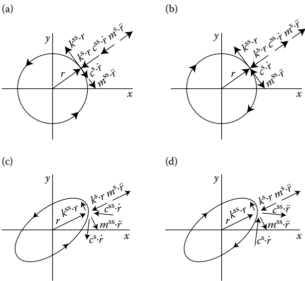
FIGURE 2.13 Force components delineated by the symmetric/skew-symmetric decomposition of the k_{ij} , c_{ij} , and m_{ij} coefficient matrices for the isotropic model: (a) circular orbit, forward whirl, (b) circular orbit, backward whirl, (c) elliptical orbit, forward whirl, and (d) elliptical orbit, backward whirl.
