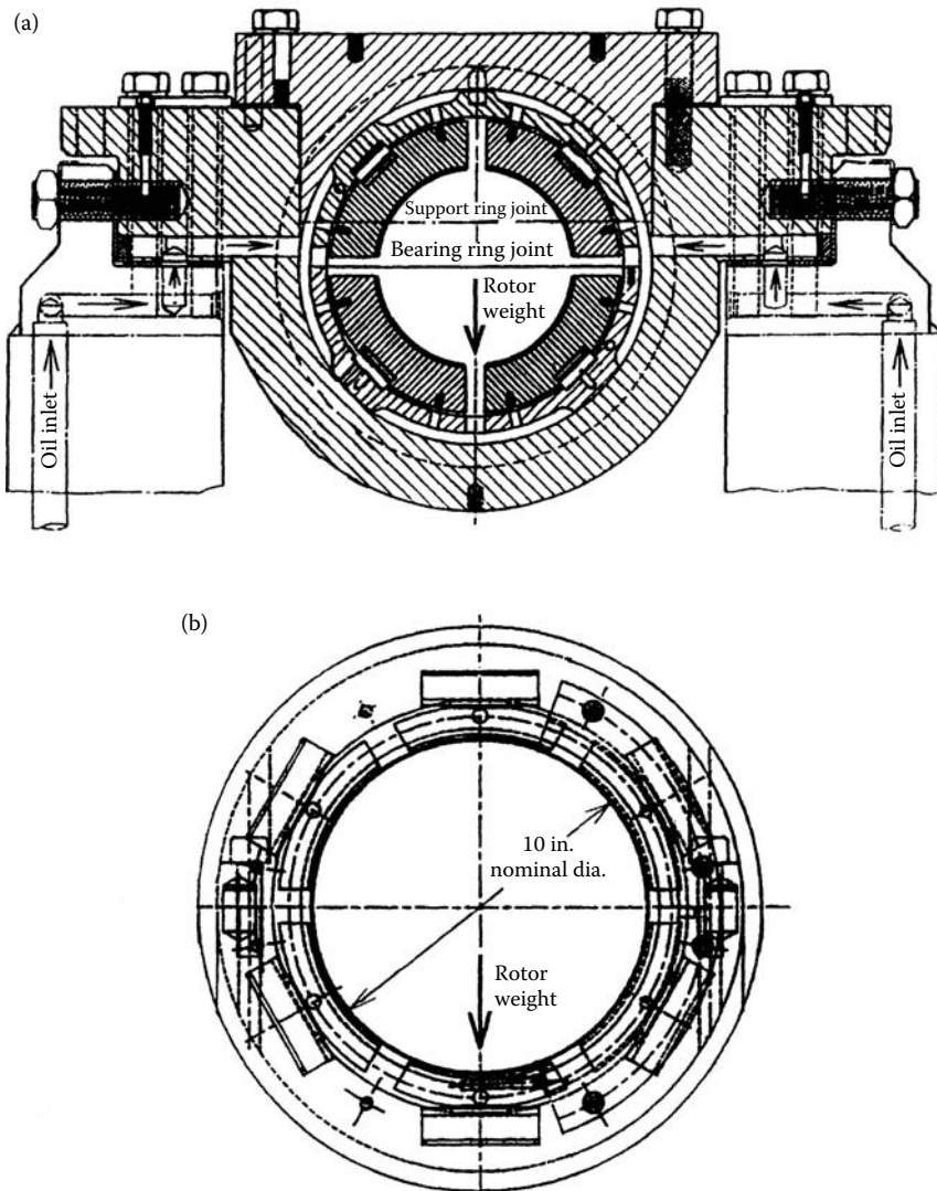
FIGURE 12.13 HP turbine tilting-pad journal bearings for a 350 MW unit.
