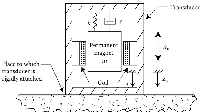
FIGURE 7.6 Elementary schematic for a velocity transducer.
