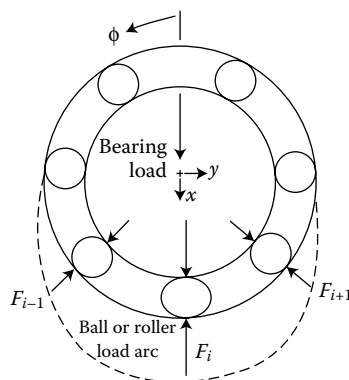
FIGURE 5.19 Typical distribution of contact loads in an RCB.
