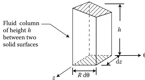
FIGURE 5.16 BFM CV fluid element.
