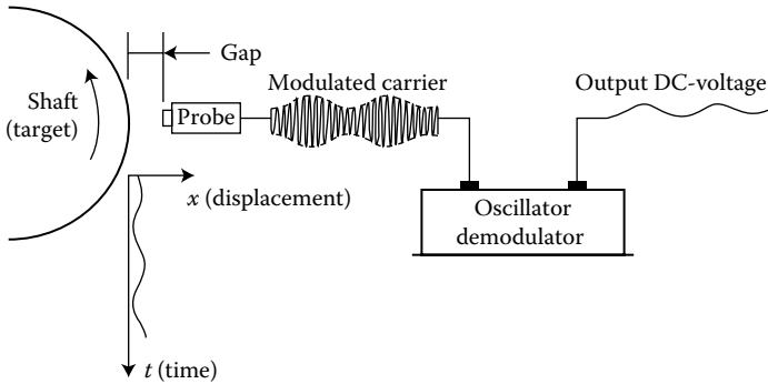
FIGURE 7.7 Inductance (eddy-current) position sensing system.
