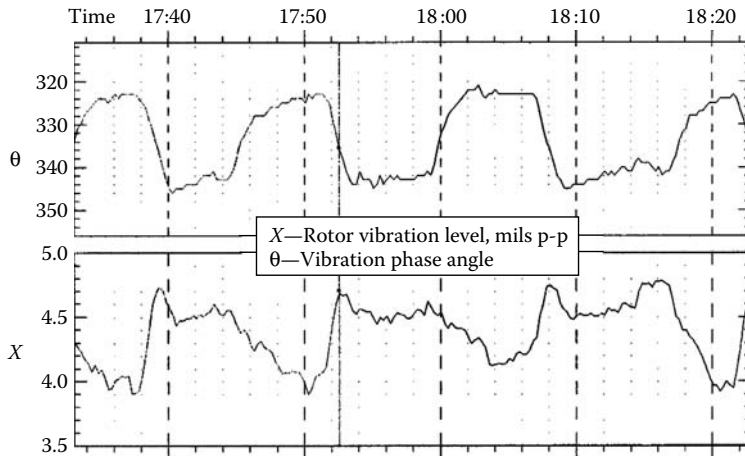
FIGURE 10.15 Fifty-minute vibration record from feed water B-Pump Unit-2.
