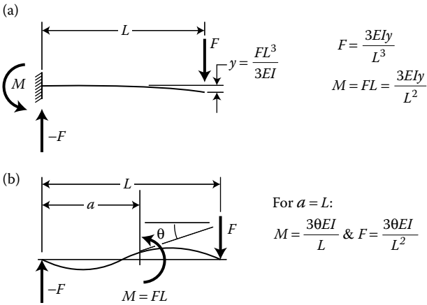
FIGURE 2.6 Beam deflection formulas.
