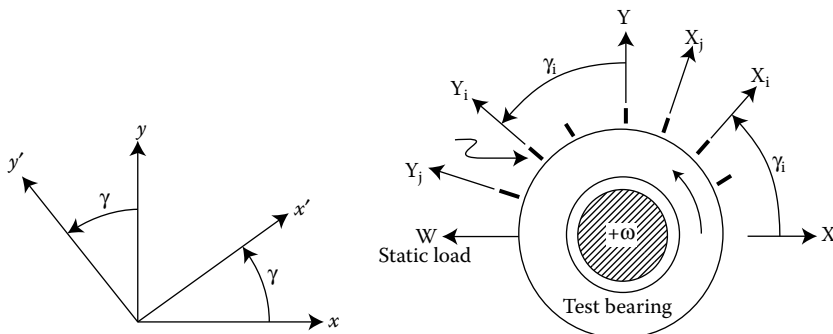
FIGURE 5.2 Tensor transformation of bearing coefficients, Equations 5.7.
