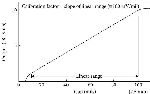
FIGURE 7.8 Typical inductance probe displacement calibration plot.
