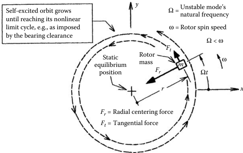
FIGURE 9.19 Growth of rotor orbit for an unstable rotor mode.
