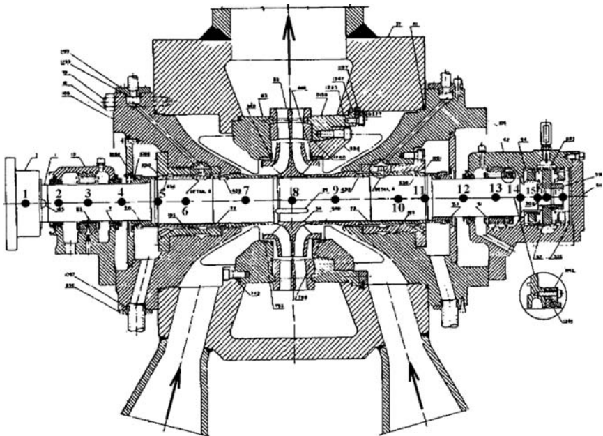
FIGURE 10.14 Nuclear feed water pump.
