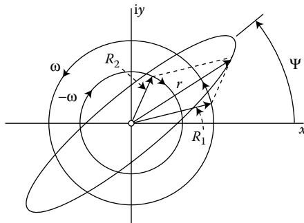
FIGURE 4.6 Elliptical orbit: the sum of two counter whirling circular orbits.
