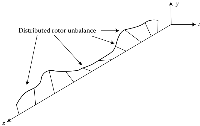
FIGURE 12.19 Isometric view of a general rotor unbalance axial distribution.
