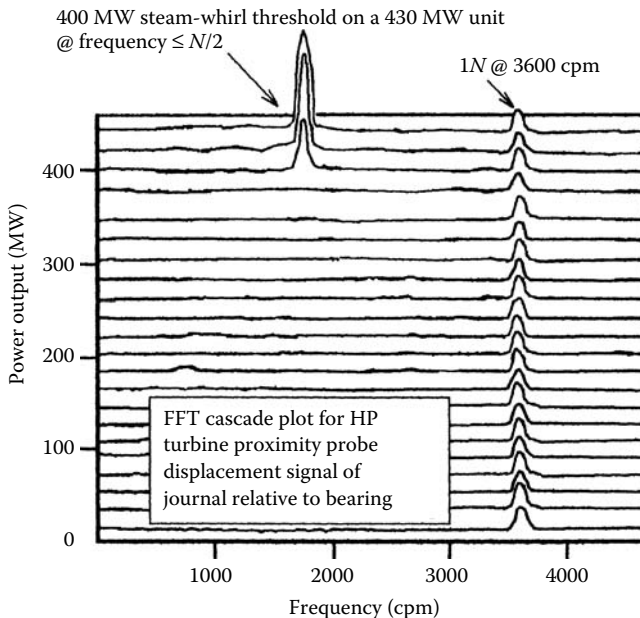
FIGURE 9.20 Steam whirl symptoms on high-pressure steam turbine. Unit should be de-rated to 400 MW pending solution of problem.
