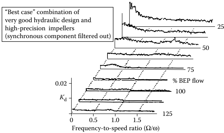
FIGURE 6.4 Spectra (rms) of normalized broadband impeller forces.
