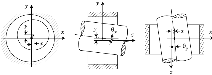
FIGURE 2.14 Radial bearing/seal radial and misalignment coordinates.
