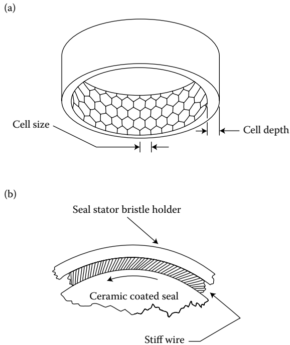
FIGURE 5.18 Recently implemented annular gas seal designs: (a) honeycomb seal and (b) brush seal.
