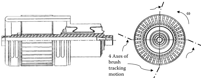
FIGURE 12.9 DC starter-generator rotor.
