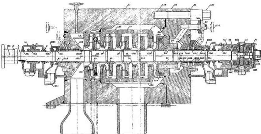
FIGURE 10.10 Variable-speed boiler feed pump of a 600 MW generating unit.
