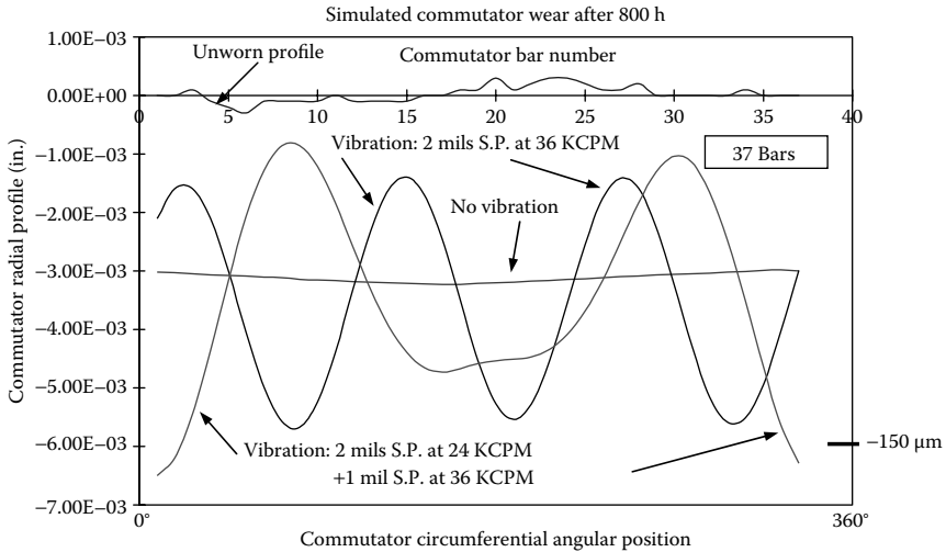
FIGURE 12.12 (See color insert following page 262.) Simulated commutator radial wear for APU DC starter-generator.
