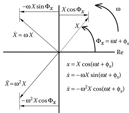
FIGURE 4.3 Complex plane view of x -displacement, velocity, and acceleration.
