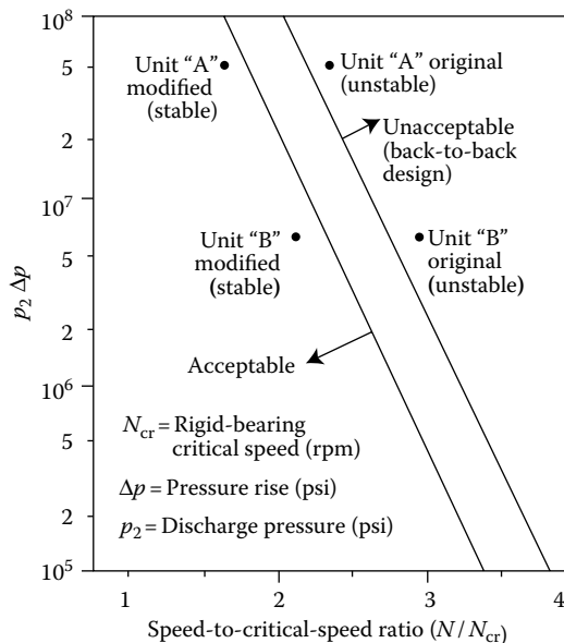
FIGURE 6.5 Criteria for rotor dynamically stable centrifugal compressors.
