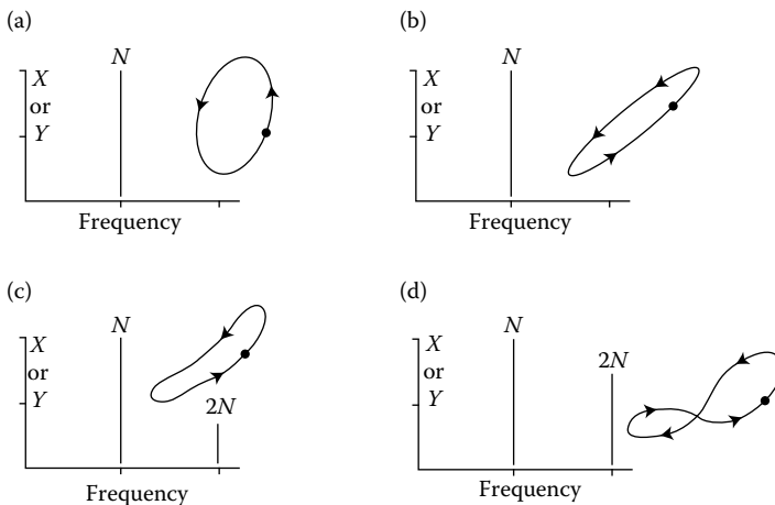
FIGURE 9.5 Filtered orbit and FFT with increasing radial load or misalignment. (a) Nominal radial load; synchronous linear motion. (b) Moderate radial load increase; synchronous linear motion. (c) Substantial radial load; nonlinear motion with some 2N . (d) Very high radial load; nonlinear motion with high 2N .
