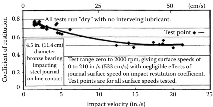
FIGURE 2.24 Bearing-on-journal impact restitution coefficient.
