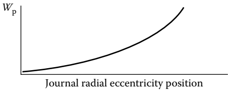
FIGURE 5.4 Tilting pad load W_p versus journal pivot radial displacement.
