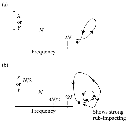
FIGURE 9.6 Changes with high radial load or misalignment during coast-down. (a) Filtered journal orbit and FFT at normal operating speed (5413 rpm). (b) Filtered journal orbit and FFT during coast-down at 4264 rpm.
