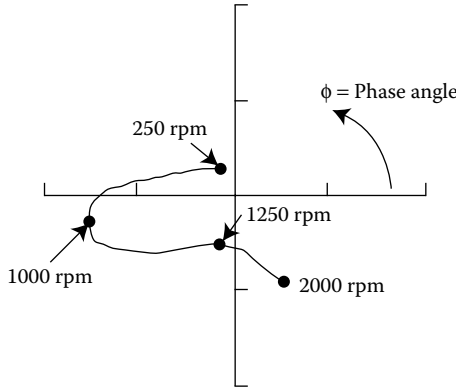
FIGURE 9.8 Polar plot of steady-state vibration amplitude and phase angle.
