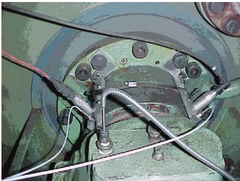
FIGURE 10.11 Proxy probe setup.
