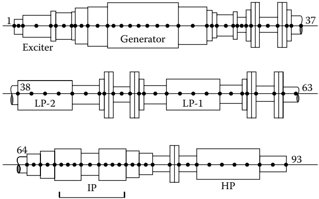
FIGURE 3.8 Layout for 93-DOF model of 800 MW 3600 rpm turbo-generator.
