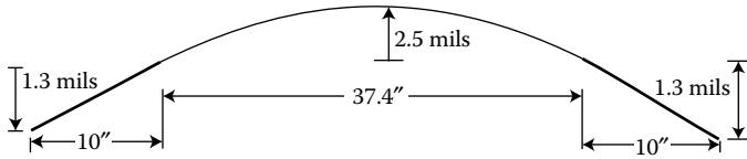
FIGURE 10.16 Computed shaft bow by sleeve-to-shaft differential expansion.
