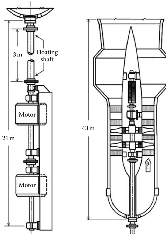
FIGURE 3.5 Altitude wind tunnel high-capacity two-stage fan.
