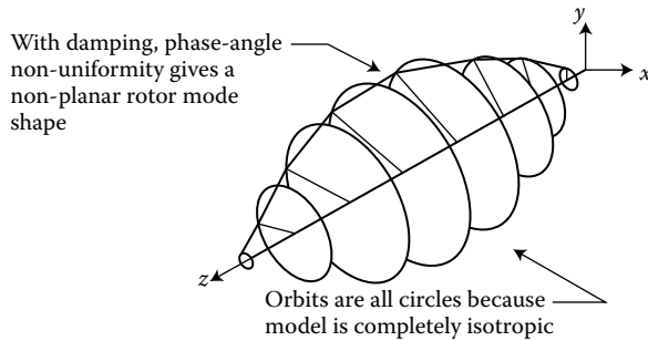
FIGURE 4.8 Isotropic model with damping gives circular orbits.
