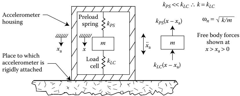
FIGURE 7.5 Elementary schematic for unidirectional accelerometer.
