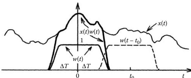
FIGURE 9.11 Time windowing of a function for WFT.
