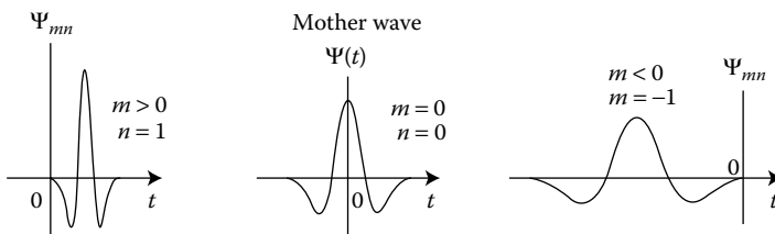
FIGURE 9.13 Two wavelets, which are dilations and translations of \Psi(t) .
