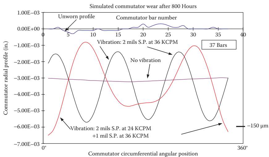
FIGURE 12.12 Simulated commutator radial wear for APU DC starter-generator.
