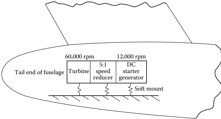
FIGURE 12.8 Commuter jet APU.
