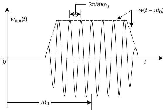
FIGURE 9.12 Illustration of a member of the function family w_{mn}(t) .
