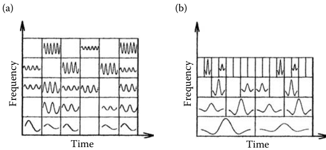
FIGURE 9.14 Time–frequency plane, comparing FT and WT: (a) WFT and (b) WT.
