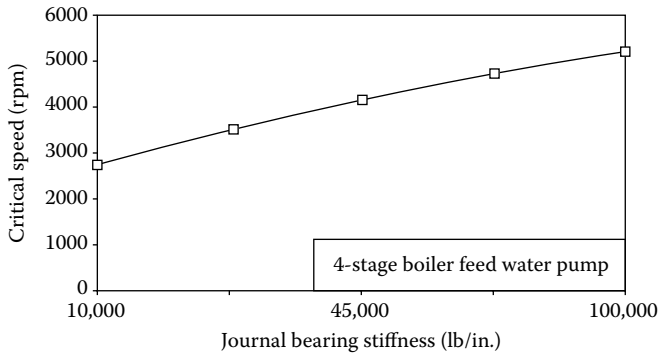
FIGURE 10.7 Computed unbalance-excited critical speed versus bearing stiffness (interposed gasket).
