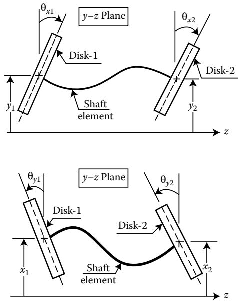
FIGURE 2.8 Basic rotor finite-element building block.
