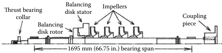
FIGURE 10.6 Rotor sectional view for a four-stage BFP.
