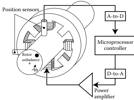
FIGURE 5.21 Active magnetic bearing schematic.
