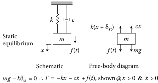
FIGURE 1.1 One-DOF linear spring-mass-damper model.
