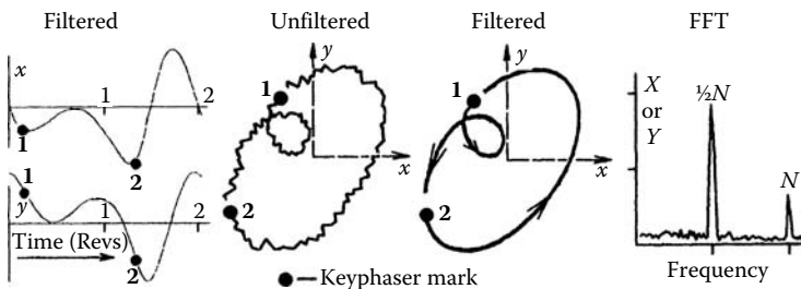
FIGURE 9.4 Measured orbit with synchronous and half synchronous components.
