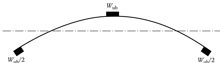
FIGURE 12.18 Unbalance vibration mode shape of a first bending critical speed.
