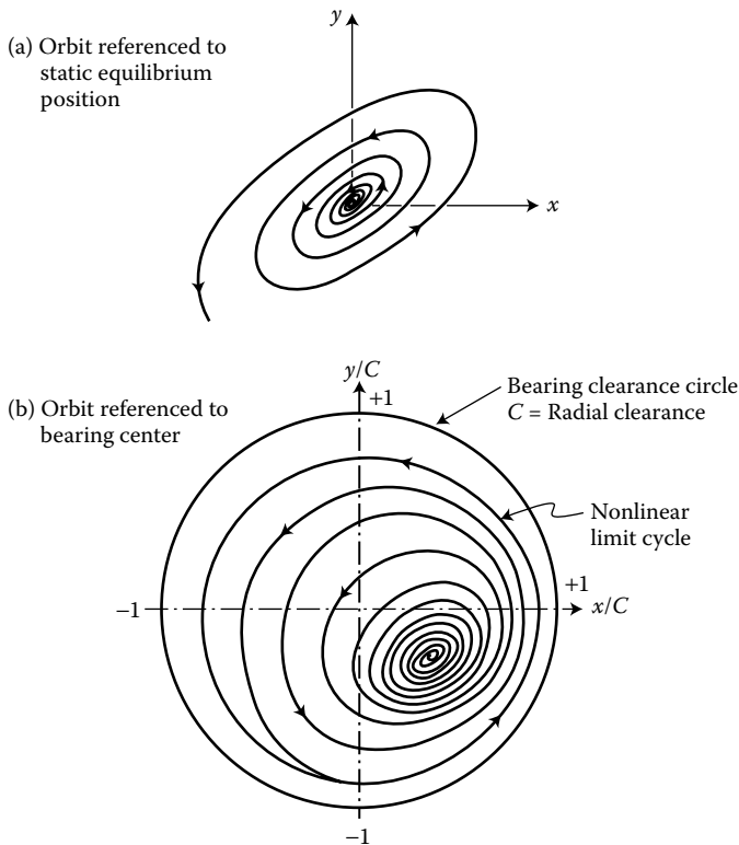
FIGURE 4.11 Transient orbital vibration build-up in an unstable condition: (a) initial linear transient build-up and (b) growth to nonlinear limit cycle.
