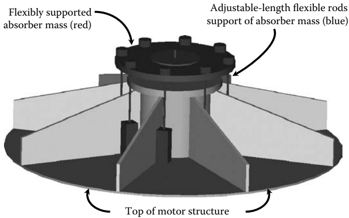
FIGURE 10.19 (See color insert following page 262.) Vibration absorber (blue and red) atop pump motor.
