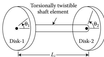
FIGURE 3.2 Rotor torsional finite-element 2-DOF building block.
