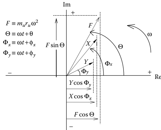
FIGURE 4.2 Complex plane representation of synchronous harmonic signals.
