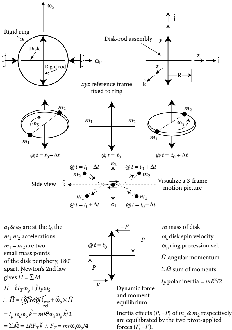
FIGURE 2.12 Illustrated explanation of the gyroscopic effect.
