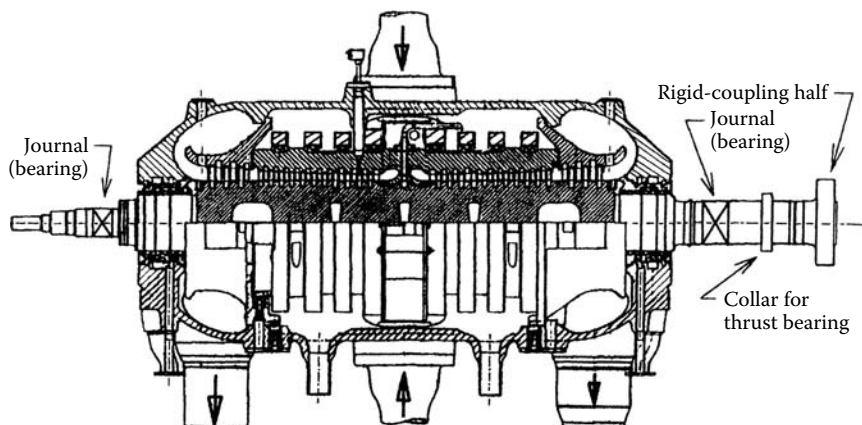
FIGURE 11.1 HP turbine section of the HP drive line of a 1300 MW 3600 rpm cross-compound steam turbo-generator.
