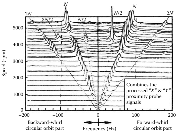
FIGURE 9.10 Cascade for field measurement case shown in Figure 9.6.
