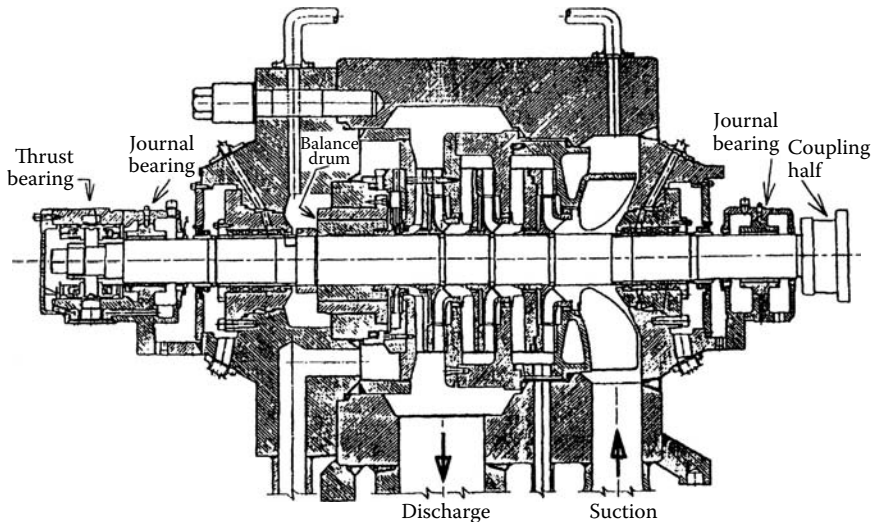
FIGURE 10.9 Assembly view of a BFP.
