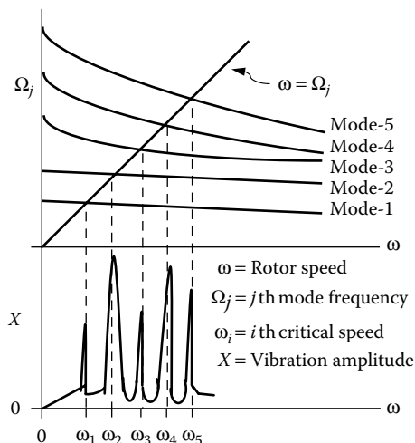
FIGURE 4.10 Campbell diagram combined with unbalance vibration.
