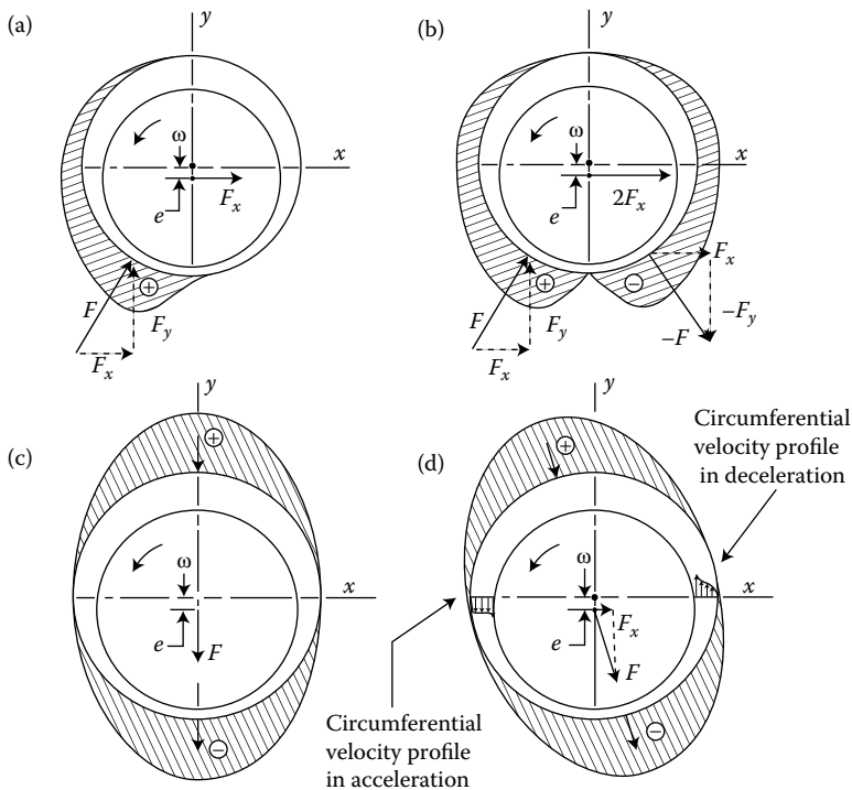
FIGURE 6.6 Circumferential pressure distributions relative to ambient: (a) journal bearing operating with atmospheric pressure (cavitation); (b) journal bearing operating with high ambient pressure (no cavitation); (c) and (d) high rotational Reynolds number fluid annulus with high ambient pressure.
