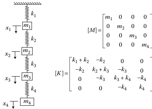
FIGURE 1.9 4-DOF lumped-mass model.
