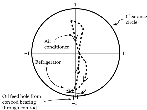
FIGURE 2.27 Wrist pin orbital trajectories from nonlinear simulations.
