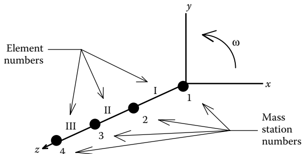
FIGURE 4.1 Proper shaft element and station input ordering.
