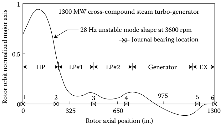
FIGURE 11.2 Steam whirl excited unstable mode of HP drive line.
