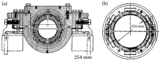
FIGURE 10.5 Turbine pivoted-pad bearing configurations: (a) OEM and (b) TRI.
