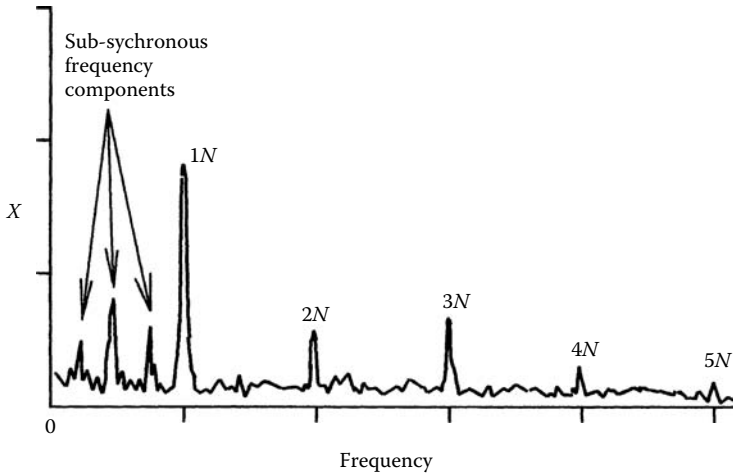
FIGURE 9.2 Example spectrum of a rotating machinery vibration signal.
