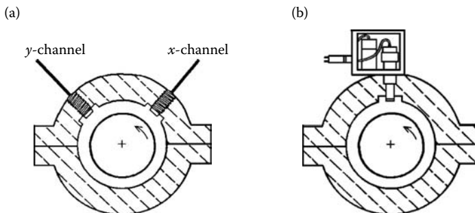
FIGURE 7.9 Proximity probe example mountings: (a) typical 2-probe @ 90^\circ placement and (b) probe with seismic sensor.
