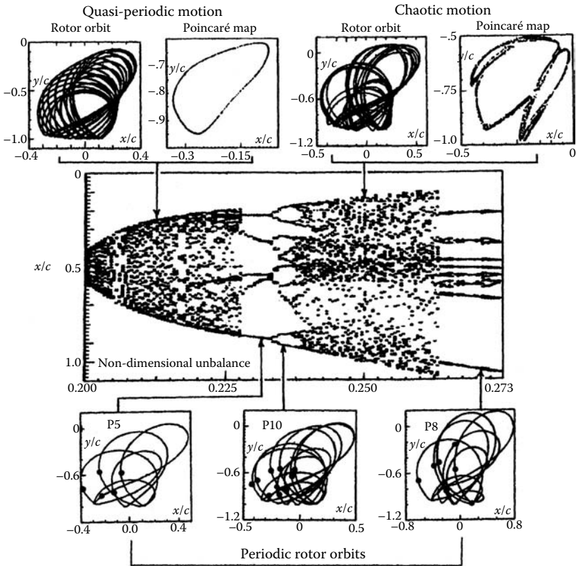
FIGURE 9.16 Rotor orbits and chaos-tool mappings for the unbalance-excited rub-impact simulation model in Figure 9.15a.
