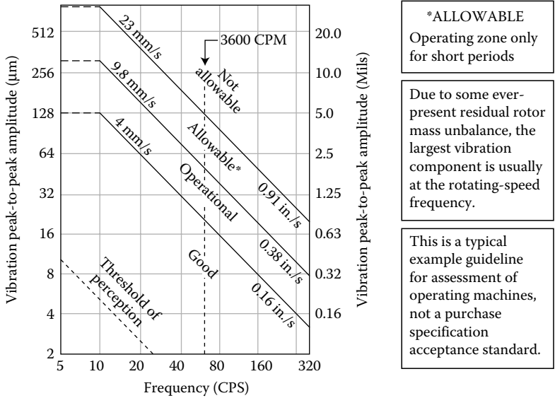
FIGURE 8.1 Bearing cap vibration displacement guideline.
