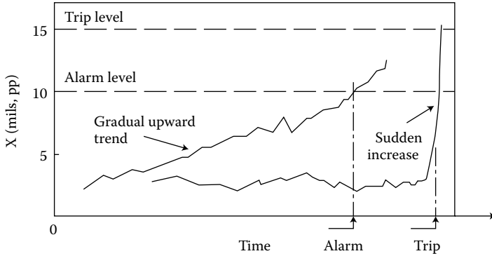
FIGURE 7.1 Tracking of a representative vibration peak amplitude over time.
