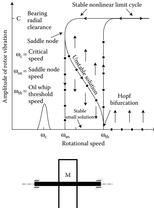
FIGURE 2.22 Journal-bearing hysteresis-loop and rotor-bearing model.
