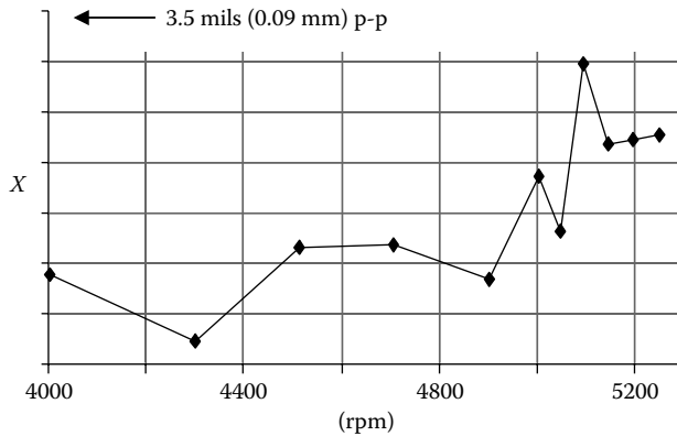
FIGURE 10.13 Boiler feed pump shaft vibration measurements.
