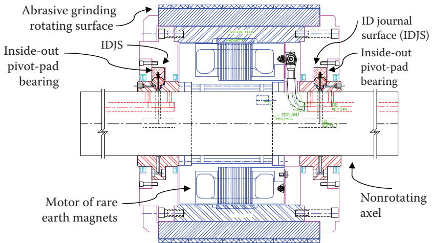
FIGURE 5.7 Next-generation centerless grinder spindle.
