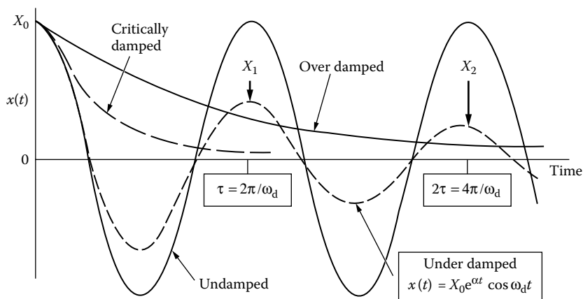
FIGURE 1.2 Motion types for the unforced 1-DOF system.
