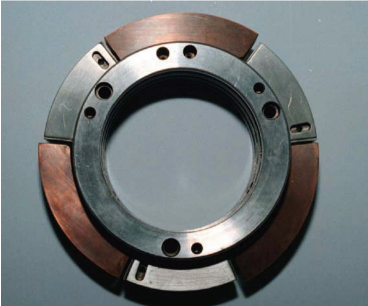
FIGURE 5.8 Photo of three-pad inside-out PPJB with three copper pads to facilitate heat removal; three steel thrust sectors.
