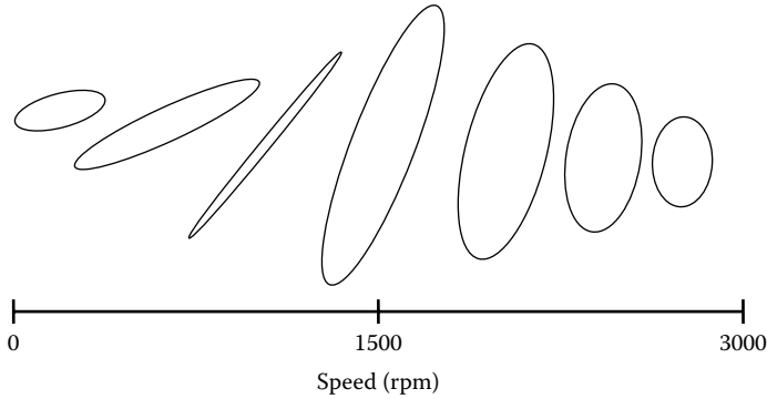
FIGURE 4.5 Orbit at a rotor station versus speed; critical speed at 1500 rpm.
