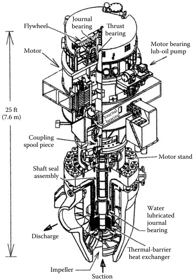
FIGURE 12.1 RCP of 100,000 gpm capacity and speed of 1200 rpm; typical PWR primary loop conditions are 2250 psi (153 bars), 550°F.
