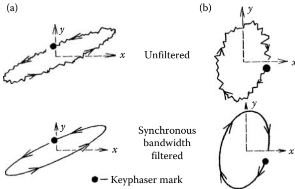
FIGURE 9.3 Illustrated examples of measured rotor synchronous orbits: (a) forward whirl and (b) backward whirl.
