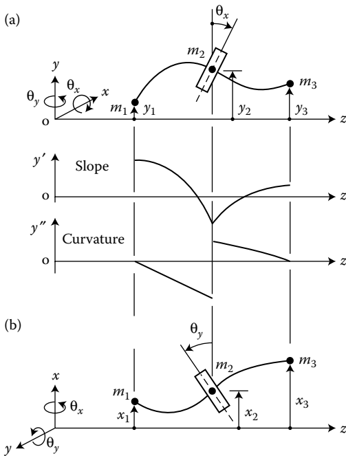
FIGURE 2.5 Rotor beam-deflection model for an 8-DOF system, with all generalized coordinates shown in their respective positive directions: (a) beam deflection, slope, and curvature in y - z plane and (b) x - z deflection only, but slope and curvature similar to (a).
