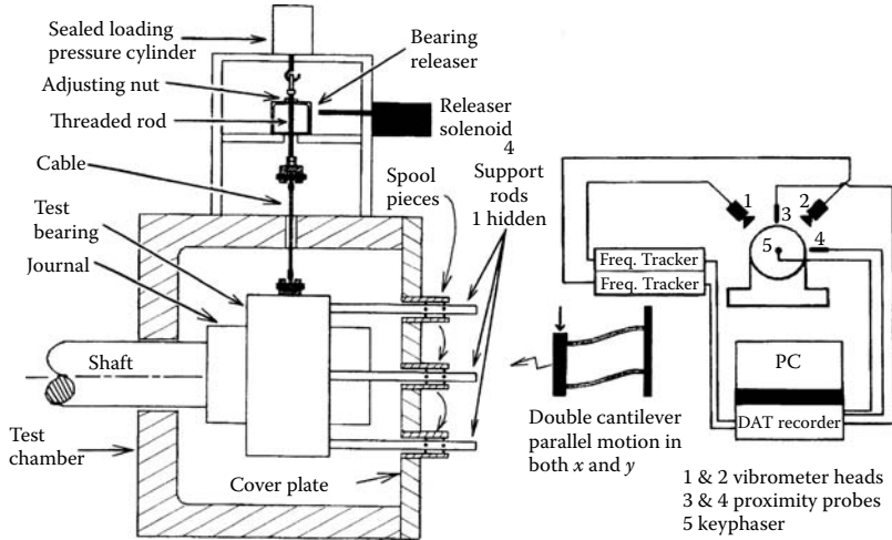
FIGURE 2.23 Test for rotor-bearing restitution coefficient measurement.
