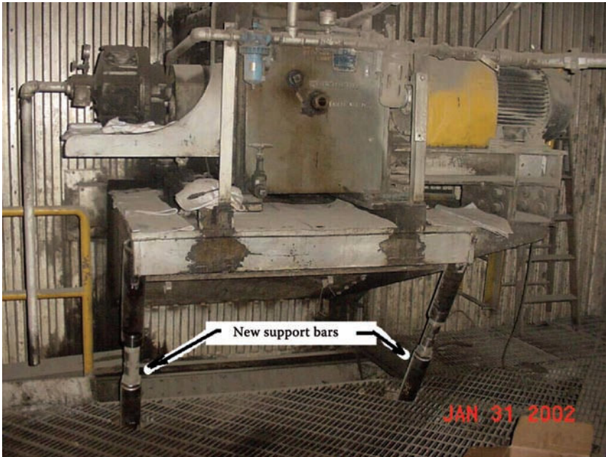
FIGURE 12.7 Air preheater drive/platform with overhang support bars.
