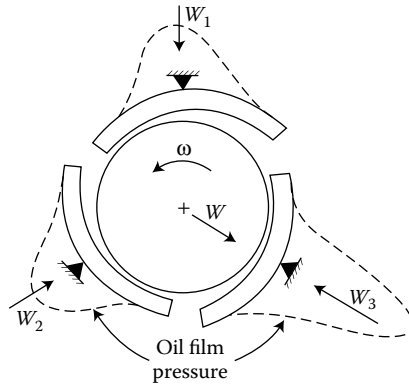
FIGURE 5.6 Illustration of preloaded tilting-pad journal bearing.
