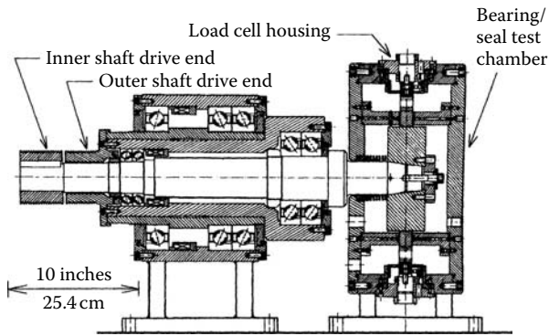
FIGURE 5.10 Double-spool-shaft spindle for bearing and seal test apparatus.
