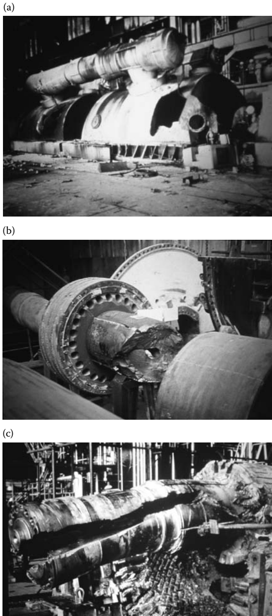
FIGURE 2.15 (See color insert following page 262.) Photos from the two 1970s catastrophic failures of large 600 MW steam turbine-generator sets. Using nonlinear rotor dynamic response computations, failures could be potentially traced to the large unbalance from loss of one or more large LP turbine blades at running speed, coupled with behavior of fixed-arc journal bearings during large unbalance. (a) LP steam turbine outer casing. (b) Brushless exciter shaft. (c) Generator shaft. (d) LP steam turbine last stage.
