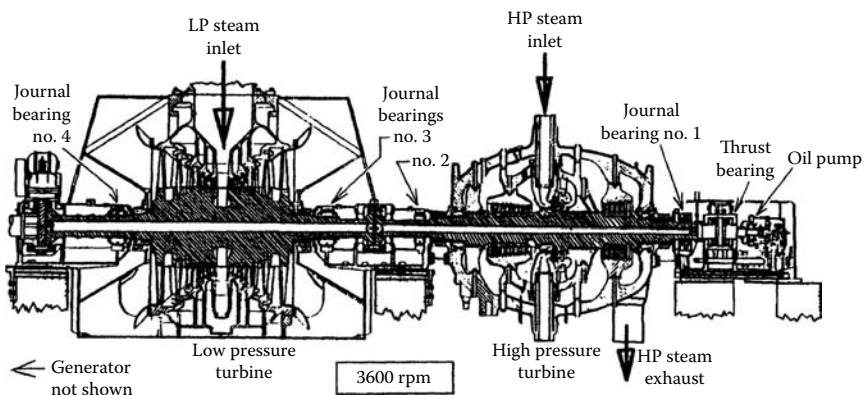
FIGURE 10.1 Cross-compound 350 MW turbo-generator, HP-LP portion.
