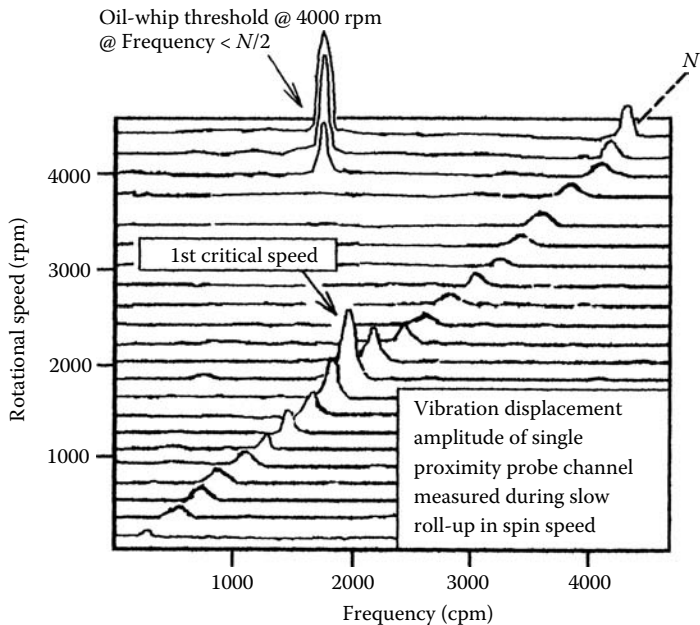
FIGURE 9.9 Cascade of passage through first critical speed to oil whip.
