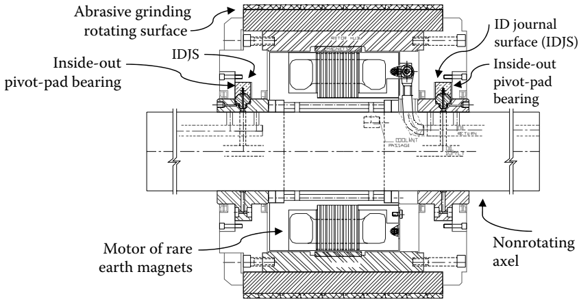
FIGURE 5.7 (See color insert following page 262.) Next-generation centerless grinder spindle.
