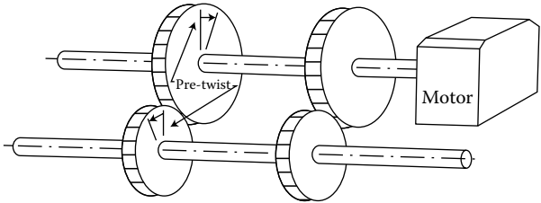
FIGURE 3.6 Conceptual illustration of a four-square gear tester.
