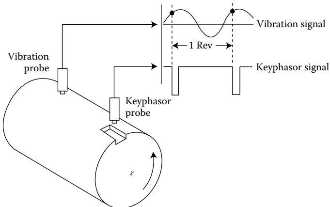
FIGURE 7.11 Vibration signals all referenced to a single keyphasor.
