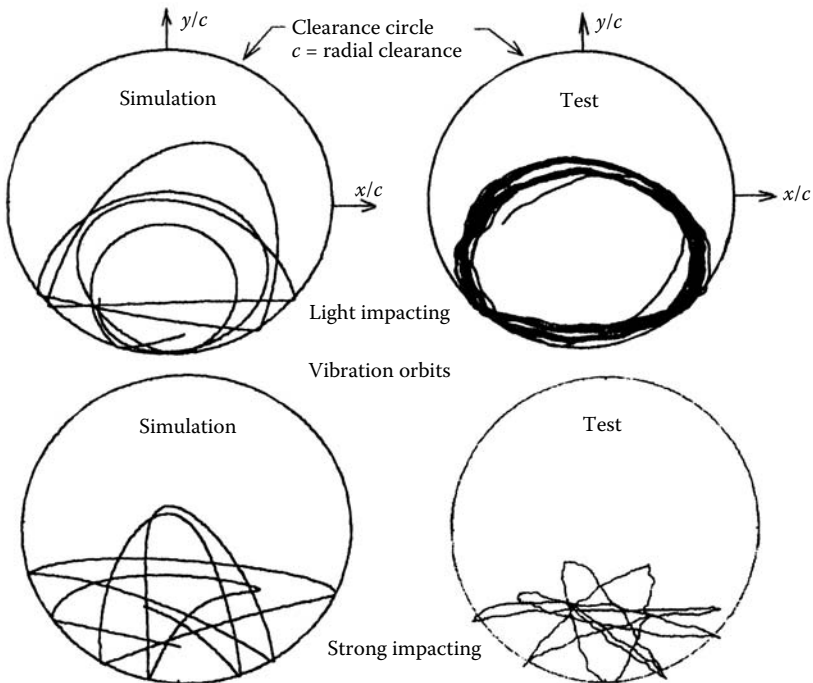
FIGURE 9.22 Unbalance induced rub-impacting on a flexible-rotor test rig.
