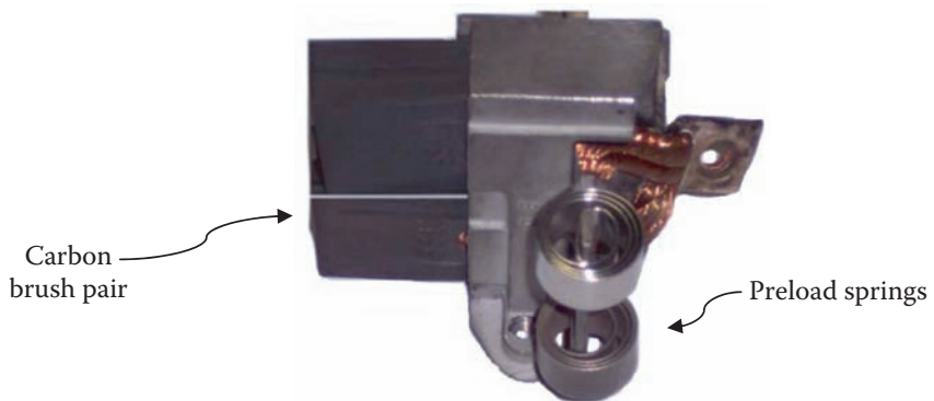
FIGURE 12.10 Carbon brush pair in holder with preload springs.
