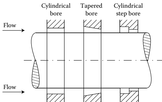
FIGURE 5.14 Ungrooved annular seals (illustrated clearances exaggerated).
