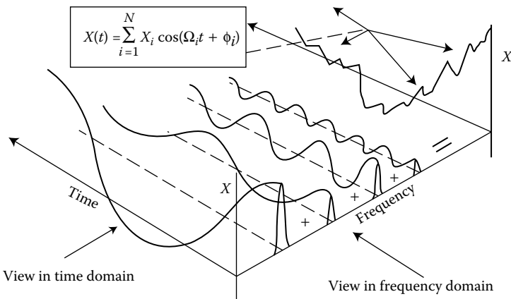
FIGURE 9.1 Illustration of an oscillatory signal's frequency spectrum.
