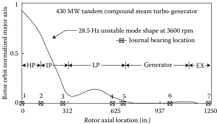
FIGURE 11.5 Oil whip/steam whirl unstable mode of complete drive line.
