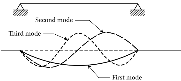
FIGURE 4.13 First three planar mode shapes for a simply supported uniform beam.
