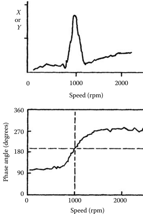
FIGURE 9.7 Bode plot of a rotor vibration signal on speed-up or coast-down.
