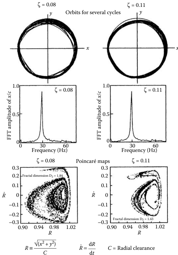
FIGURE 9.17 Poincaré mapping of chaotic response reveals small loss in damping at off-resonance condition (rub-impact model).
