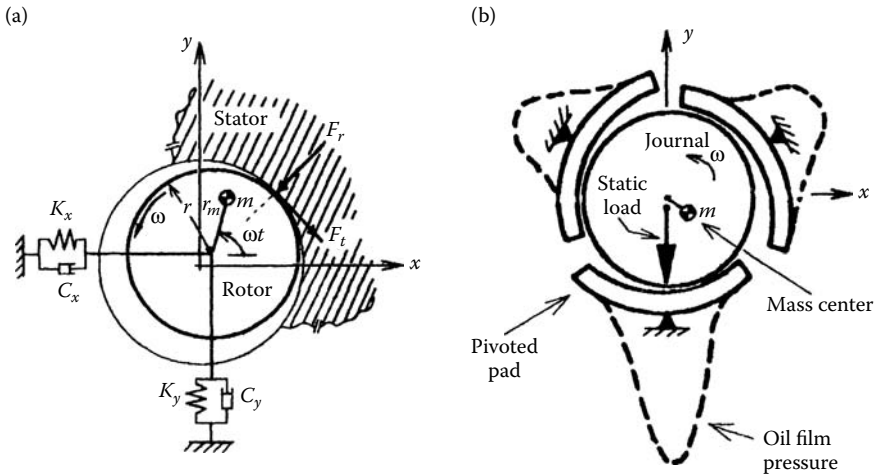
FIGURE 9.15 Simple rotor dynamics models used for chaos studies: (a) unbalance excited rub-impact and (b) three-pad pivoted-pad bearing.
