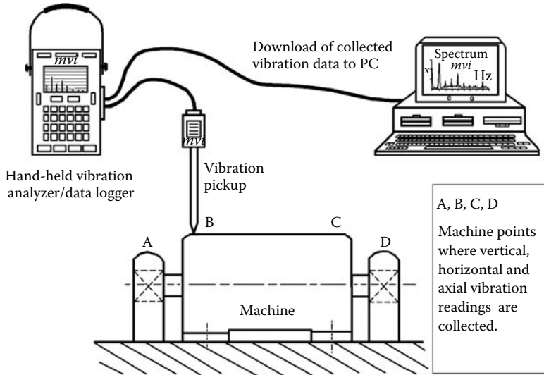
FIGURE 7.14 Portable machinery vibration analyzer and data logger.
