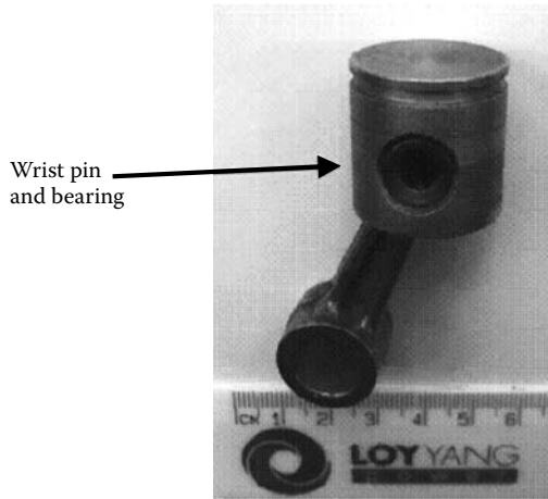
FIGURE 2.25 (See color insert following page 262.) Piston and connecting rod of a small reciprocating compressor.
