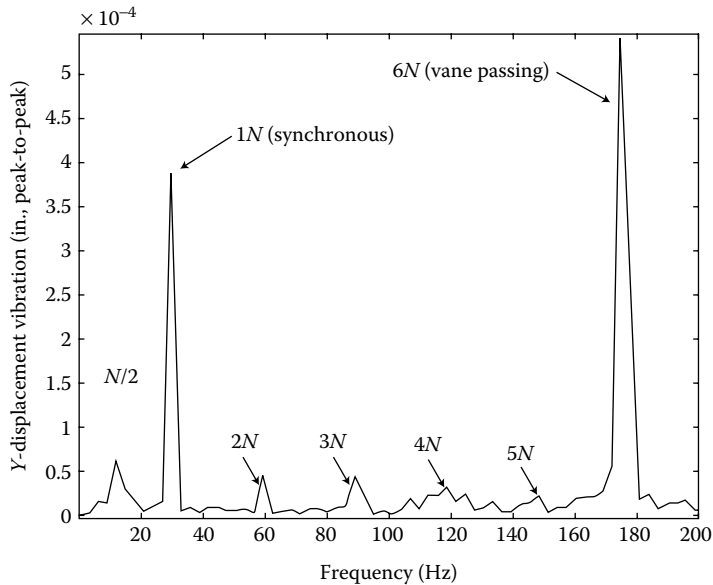
FIGURE 10.18 Shaft coupling vibration displacement spectrum.
