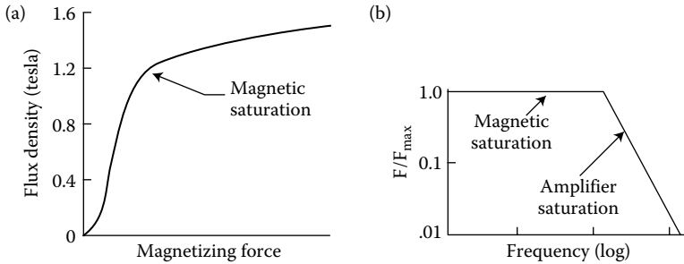
FIGURE 5.22 Magnetic bearing saturation effect load limits (Fleming, 1991).
