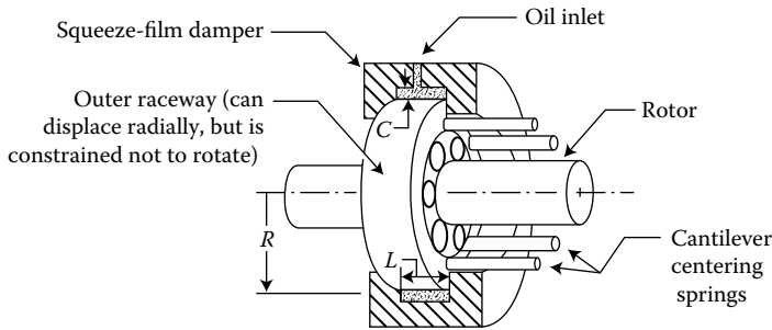
FIGURE 5.20 SFD concept with RCB and centering springs.
