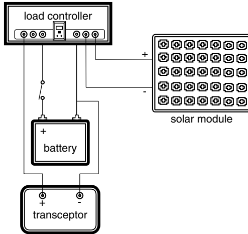
Figure 6.14 Telecommunication systems fed by solar modules.
