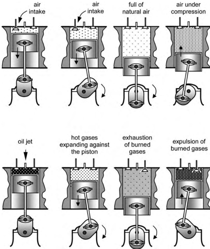
Figure A.3 Four-stroke diesel engine.
