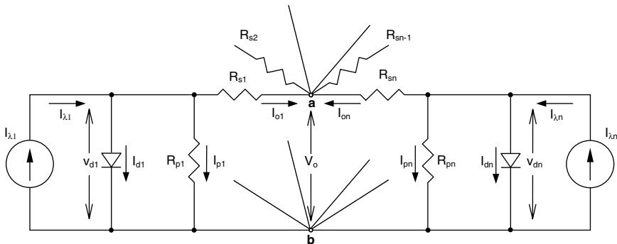
Figure 6.10 Group of identical PV cells connected in parallel.
