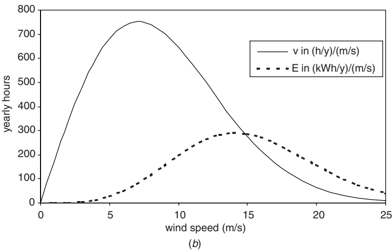
Figure 4.7 Rayleigh wind and energy density distribution ( k = 2 ): (a) c = 7 m/s; (b) c = 10 m/s.
