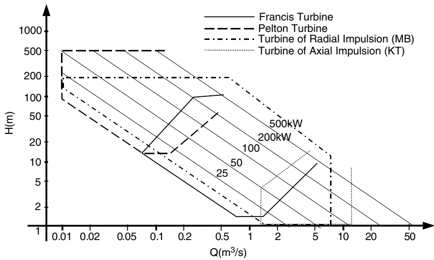
Figure 3.7 Application ranges of turbines.
