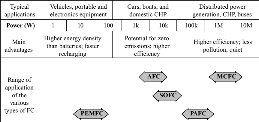
Figure 7.2 Applications of fuel cells.
