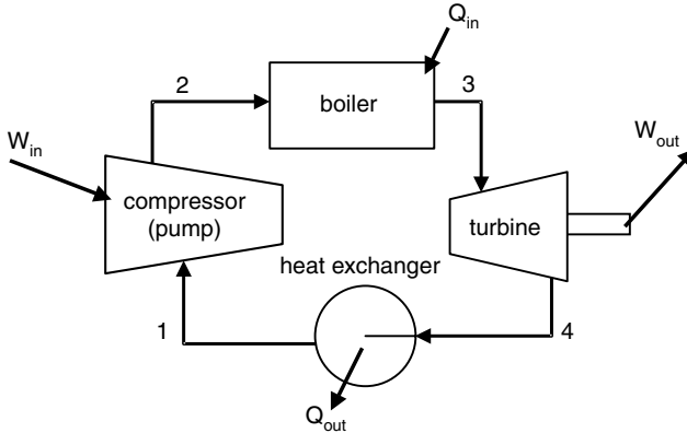
Figure 2.5 Scheme of a simple power plant.
