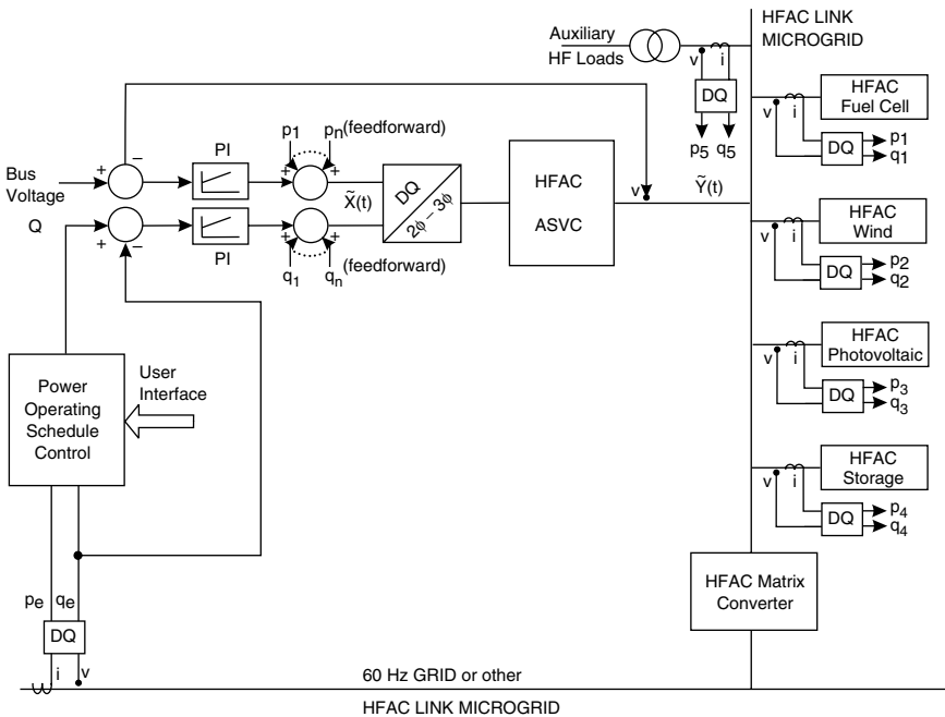
Figure 12.14 Active and reactive power flow control of an HFAC microgrid.
