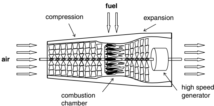
Figure 9.1 Principles of gas microturbine power conversion.
