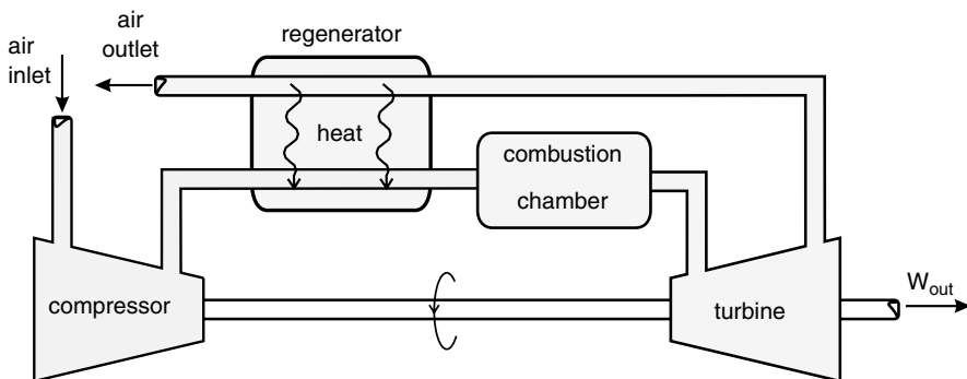
Figure 2.11 Brayton cycle–based gas turbine.
