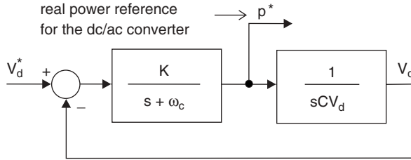
Figure 12.10 Real power tracking by dc-link voltage control.
