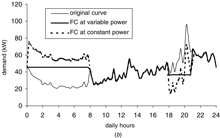
Figure 7.7 Typical residential load curves, including production of H_2 : (a) hydrogen production during off-peak hours of a weekday (from 9 p.m. to 6 a.m. the next day) in a private residence; (b) hydrogen production during the early hours of a weekday (midnight to 8 a.m.) in a condominium.
