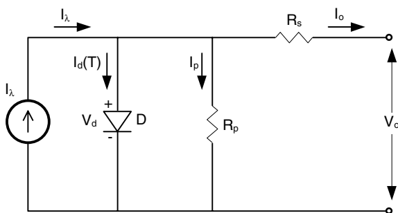
Figure 6.2 Equivalent electrical circuit of a single PV cell.
