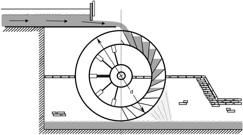
Figure 3.5 Waterwheel of upper buckets.
