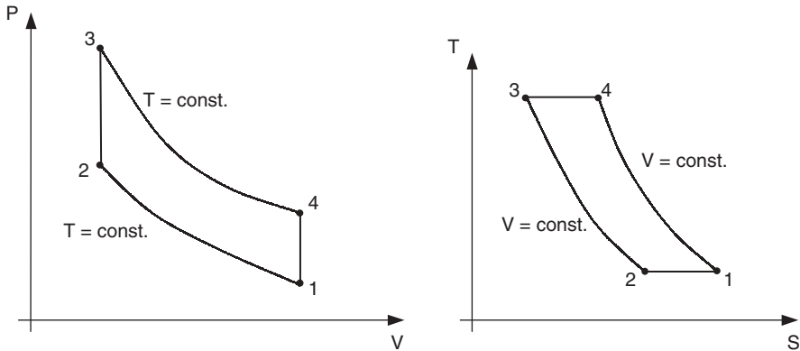
Figure C.1 P - v and T - s diagrams for the ideal Stirling cycle.
