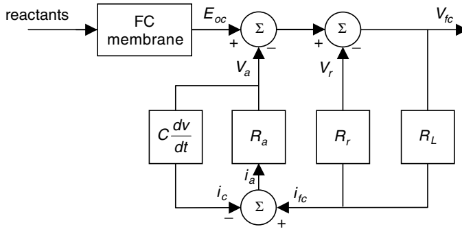
Figure 7.12 Flow diagram calculation of FC output voltage.
