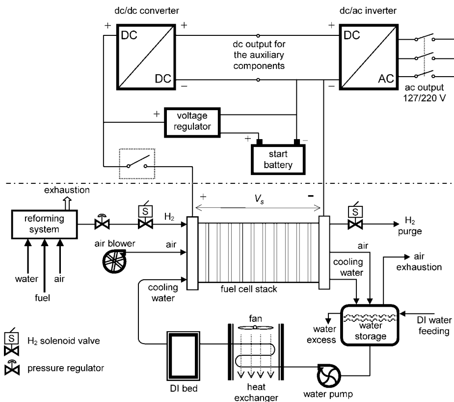
Figure 7.5 Practical outline of a small fuel cell power plant. (From Ref. [2].)
