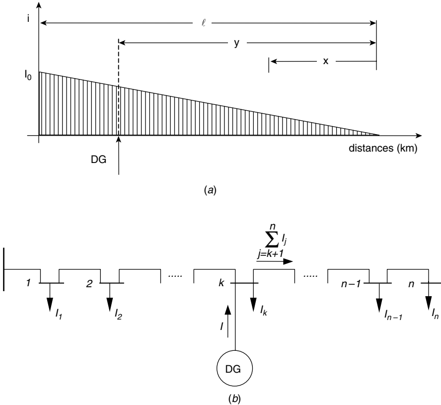
Figure 13.5 Examples of distributed loads and concentrated DG: (a) a feeder with uniformly distributed loads and DG integration; (b) a feeder with discrete loads.
