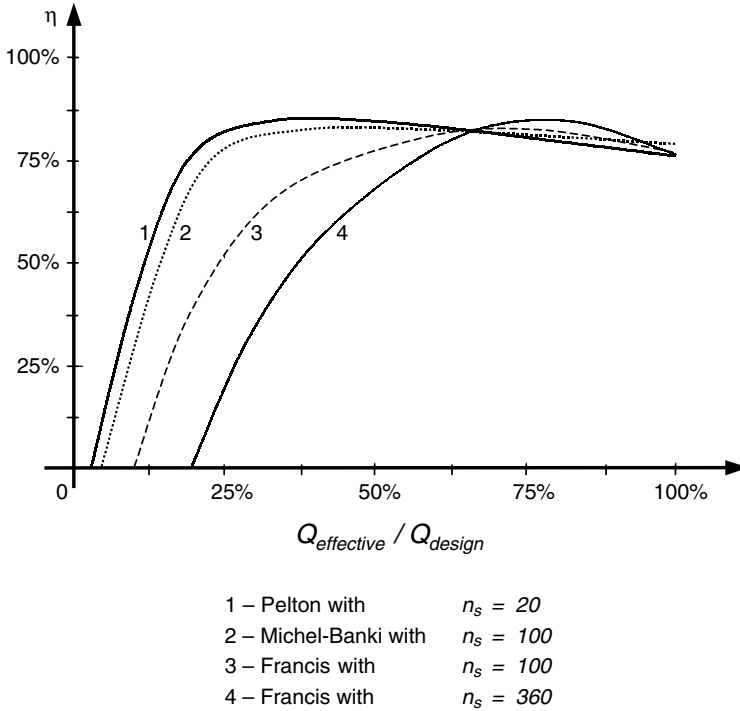
Figure 3.10 Efficiency of turbines for small hydroelectric power plants.
