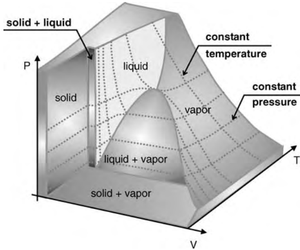
Figure 2.2 P - V - T surface for a substance.
