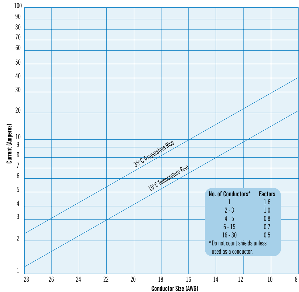
Figure 7.3—Current Ratings for Electronic Cables
