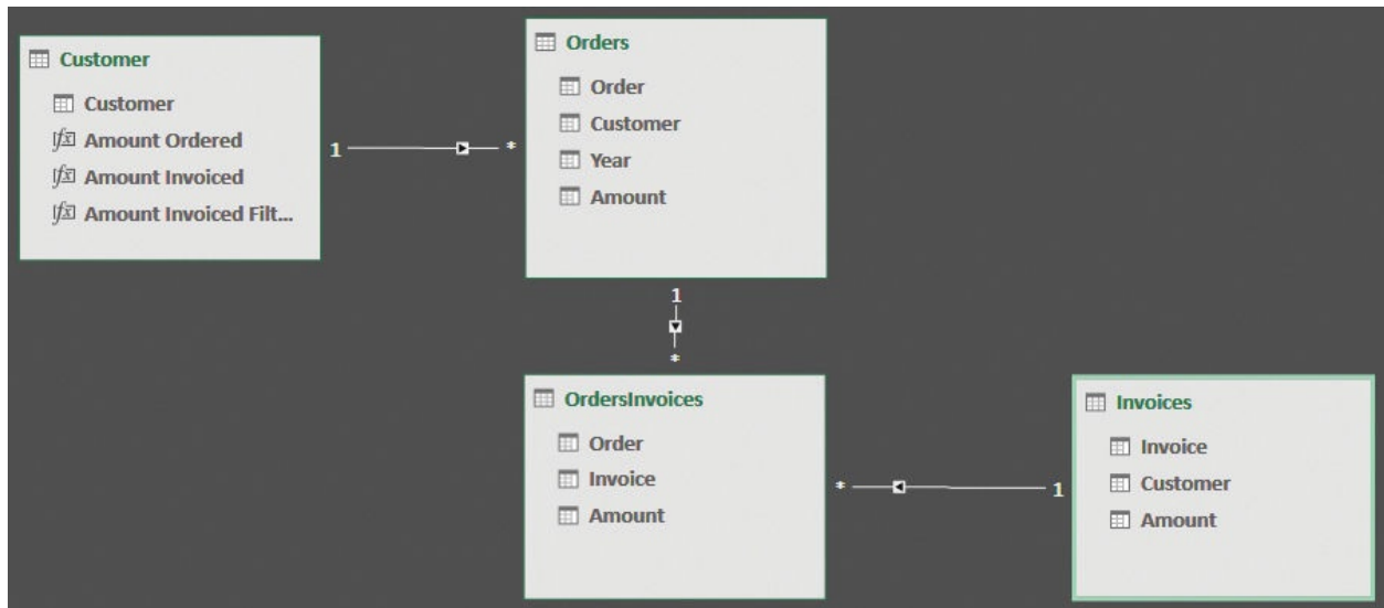
FIGURE 3-20 This structure models one order with multiple invoices, and one invoice with multiple orders, with the amount invoiced for each order.
