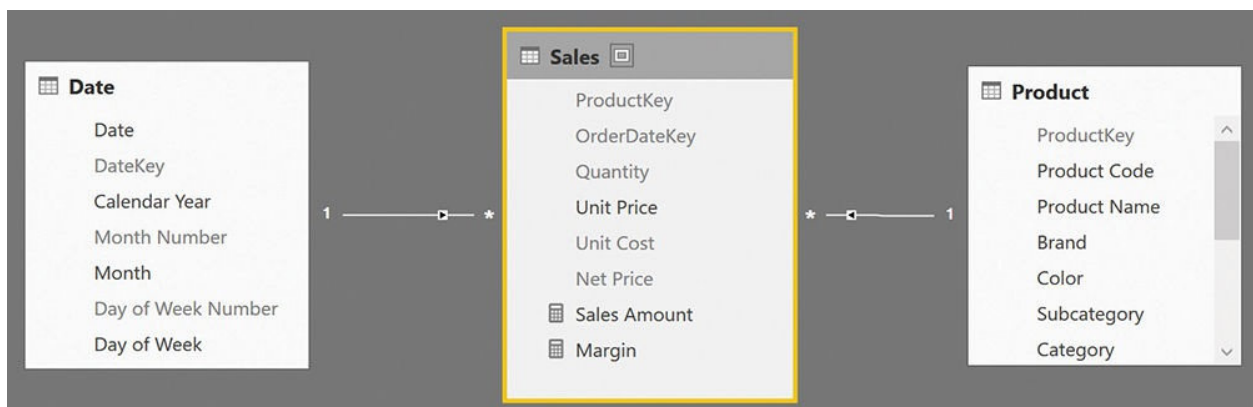
FIGURE 10-9 The data model to compute the ABC classes for products is very simple.
