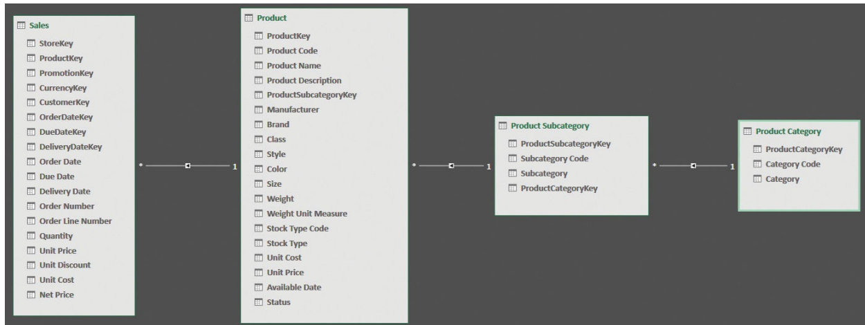
FIGURE 1-15 Product Category, Subcategory, and Product form a chain of relationships and are snowflaked.
