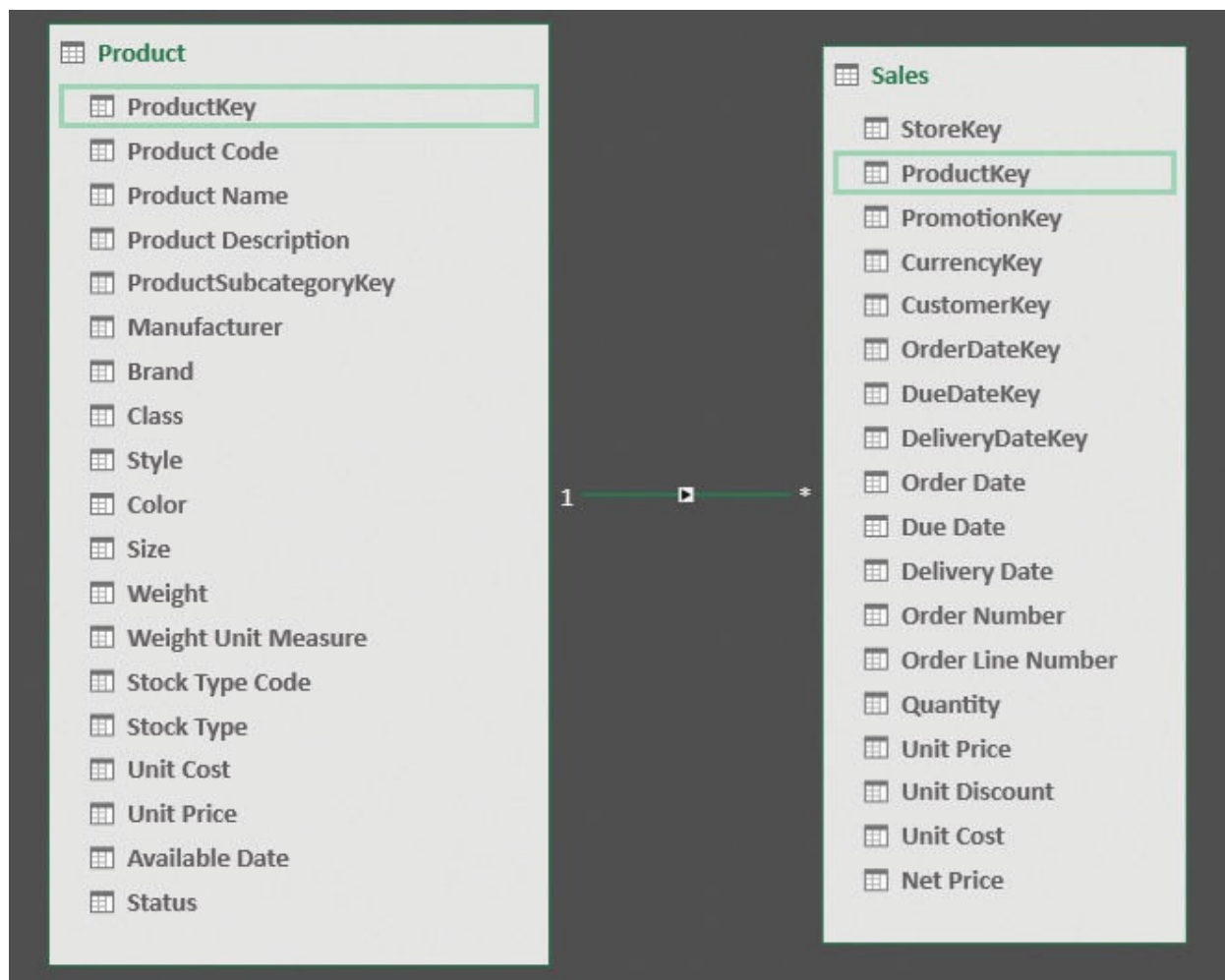
FIGURE 1-8 A relationship is represented as a line, in this case connecting the Product and Sales tables, with an indication of the side (1 for one side, * for many side).
