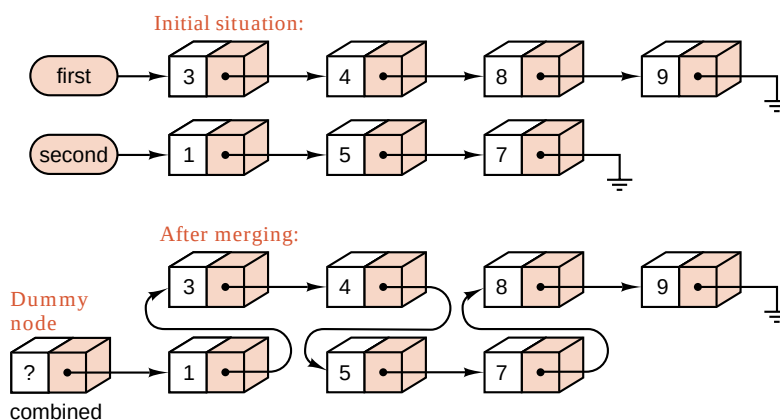
Figure 8.13. Merging two sorted linked lists
