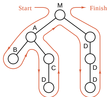
Figure 5.2. Tree of function calls
