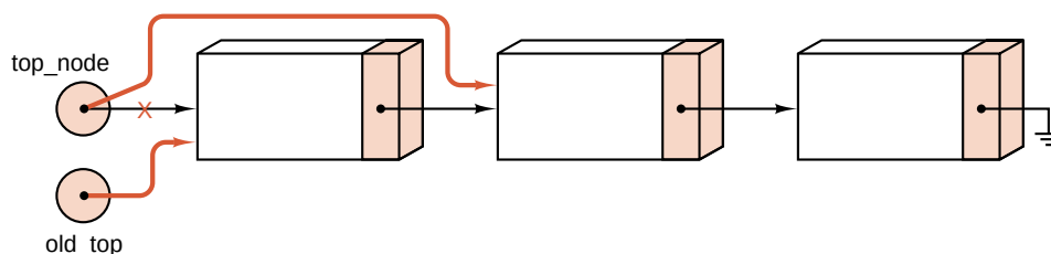
Figure 4.11. Popping a node from a linked stack
