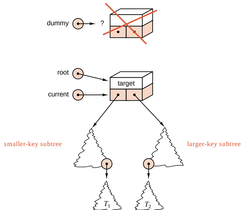
Figure 10.32. Reconnecting the subtrees
