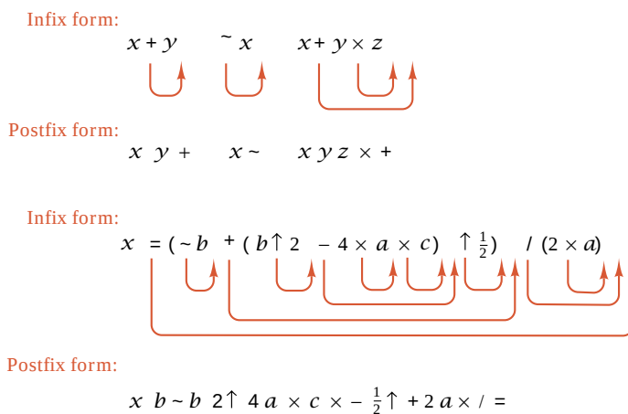
Figure 13.5. Delaying operators in postfix form
