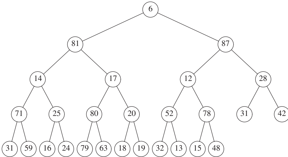
Figure 6.57 Min-max heap
