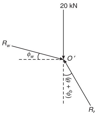
Figure 8.64 Free body diagram of block A.
