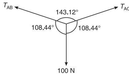
Figure 5.13 Example 5.6: Free-body diagram.
