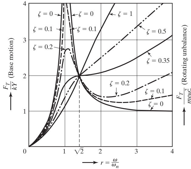
FIGURE 3.16 Force transmissibility.
