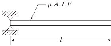
FIGURE 12.29 Pinned-free beam.
