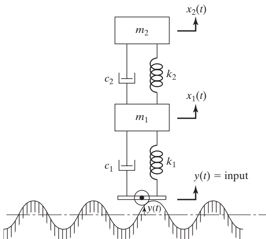
FIGURE 5.20 System with base motion.
