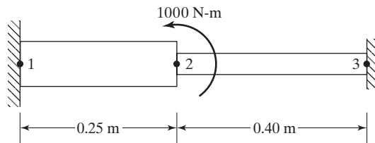
FIGURE 12.23 Stepped beam.
