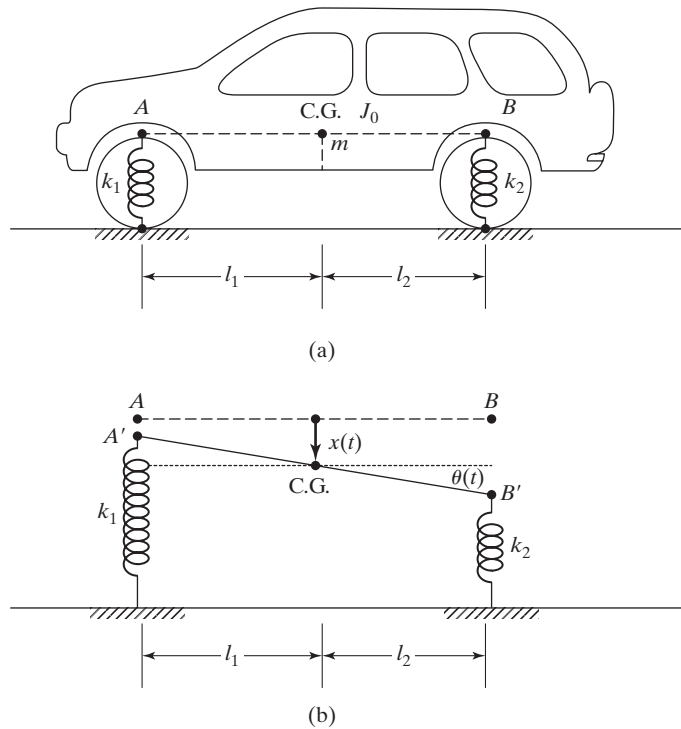
FIGURE 5.2 Car.
