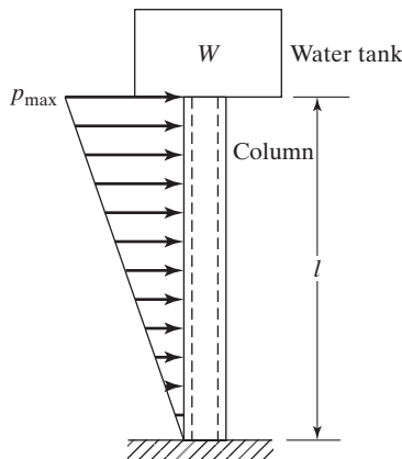
FIGURE 12.28 Water tank.
