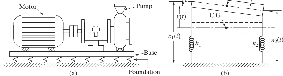
FIGURE 5.36 Motor-pump system on springs.
