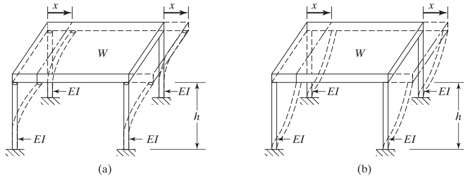
FIGURE 2.79 Building frame.
