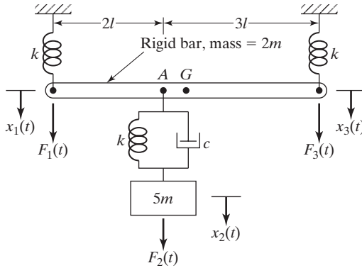
FIGURE 6.20 Three-degree-of-freedom damped system.
