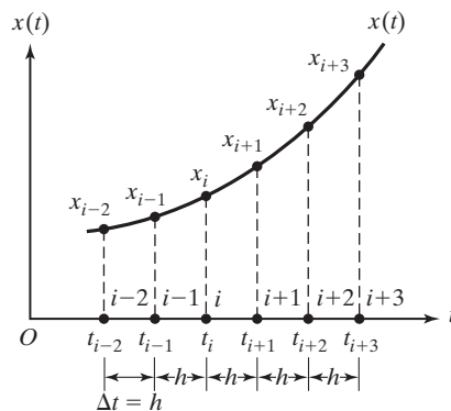
FIGURE 11.1 Grid points.
