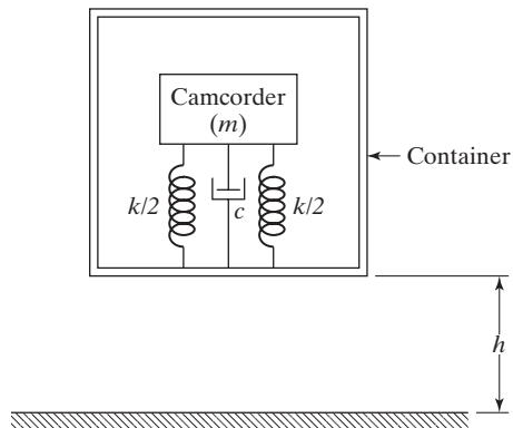
FIGURE 4.50 Dropping of container with camcorder.
