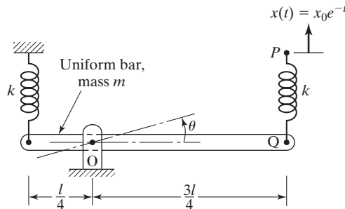
FIGURE 4.55 Rigid bar undergoing rotational motion.
