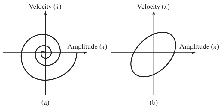
FIGURE 13.18 Attractor.
