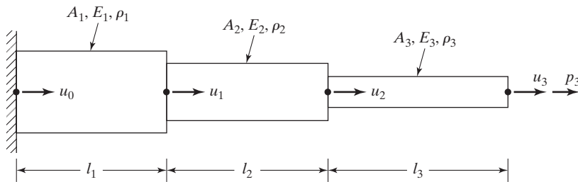
FIGURE 12.11 Stepped bar.
