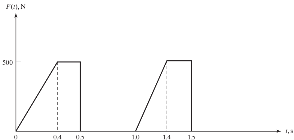
FIGURE 4.72 Periodic force.
