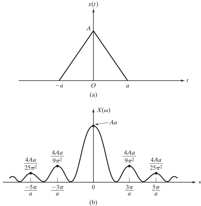
FIGURE 14.12 Fourier transform of a triangular pulse.
