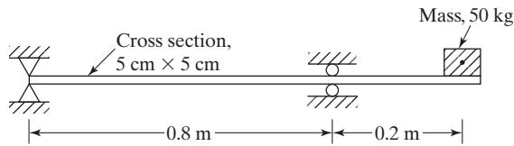
FIGURE 2.89 Beam carrying a mass.
