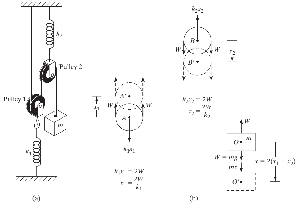
FIGURE 2.13 Pulley system.
