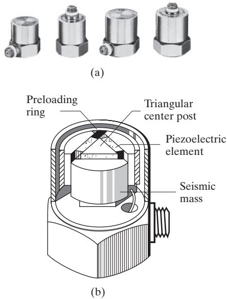
FIGURE 10.12 Accelerometers. (Brüel and Kjaer Sound and Vibration Measurement A/S.)
