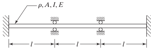
FIGURE 12.33 Fixed-fixed beam with intermediate supports.
