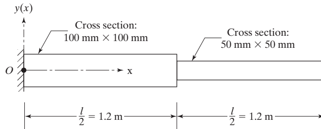
FIGURE 7.15 Stepped cantilever beam.
