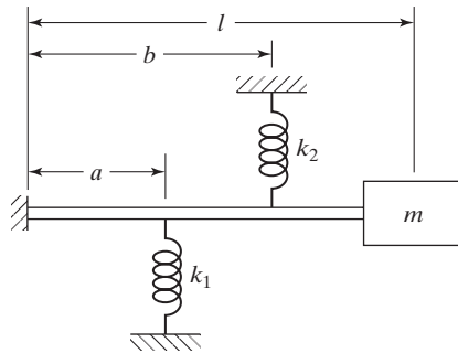
FIGURE 2.55 Elastic beam with springs and mass attached.
