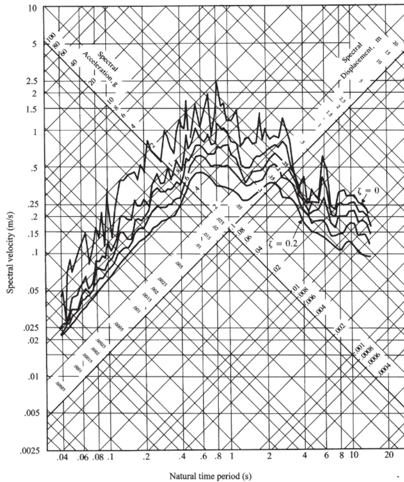
FIGURE 4.18 Response spectrum of a typical earthquake [4.12]. (Imperial Valley Earthquake, May 18, 1940; \zeta = 0, 0.02, 0.05, 0.10 , and 0.20 .) (Adapted with permission from The Shock and Vibration Digest .)
