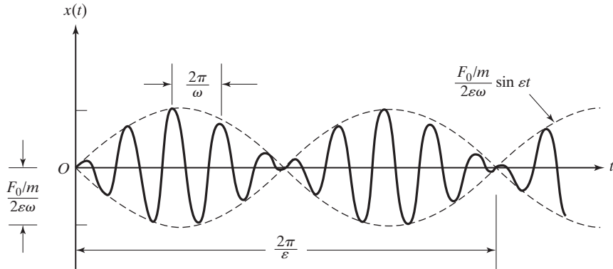
FIGURE 3.8 Phenomenon of beats.
