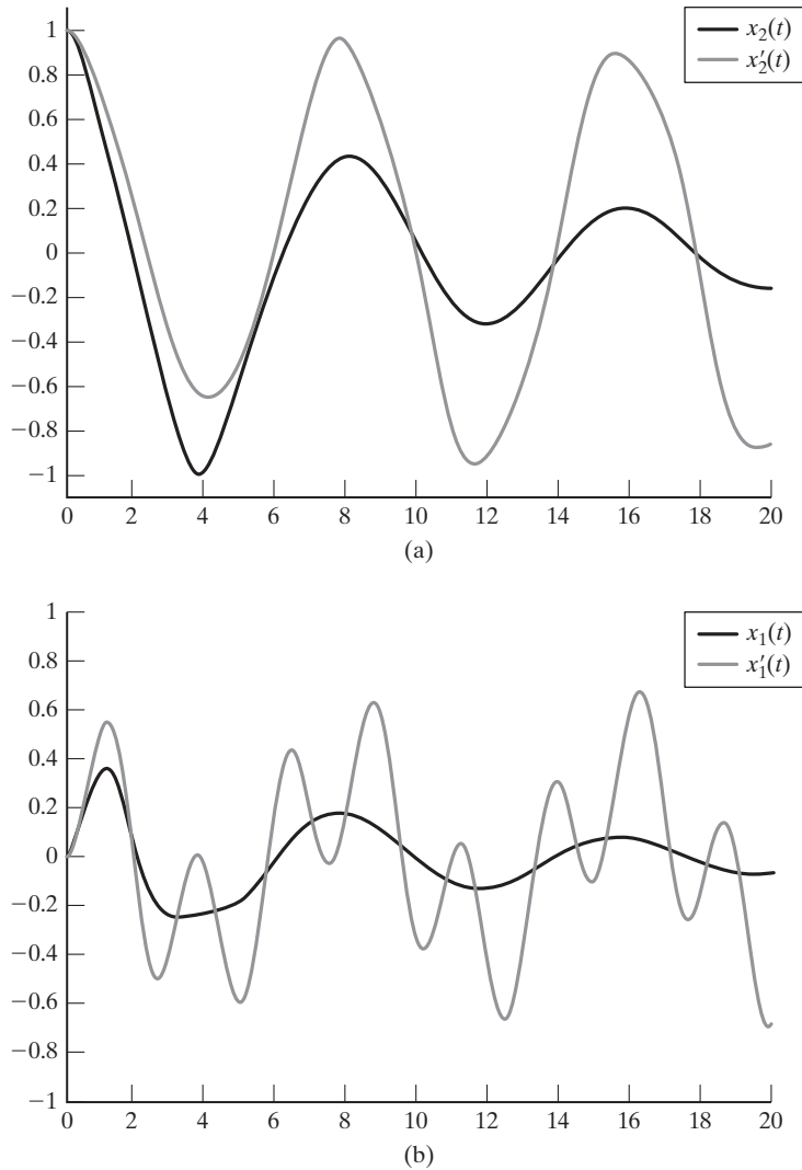
FIGURE 5.18 Free vibration response of the system.
