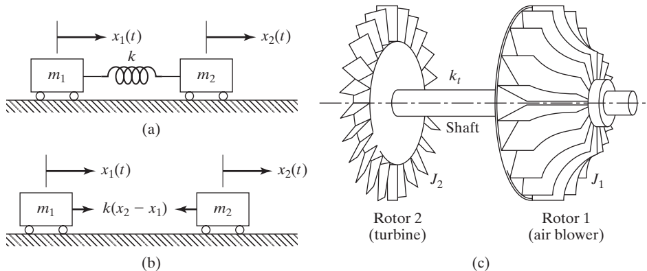
FIGURE 5.17 Semidefinite systems.
