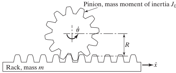
FIGURE 1.37 Translational and rotational masses in a rack-and-pinion arrangement.
