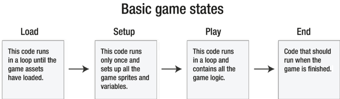
Figure 11-2. Four basic game states
