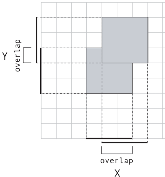
Figure A-35. The squares overlap on both axes, so we have a collision. The collision occurs on the y axis, which has the least overlap
