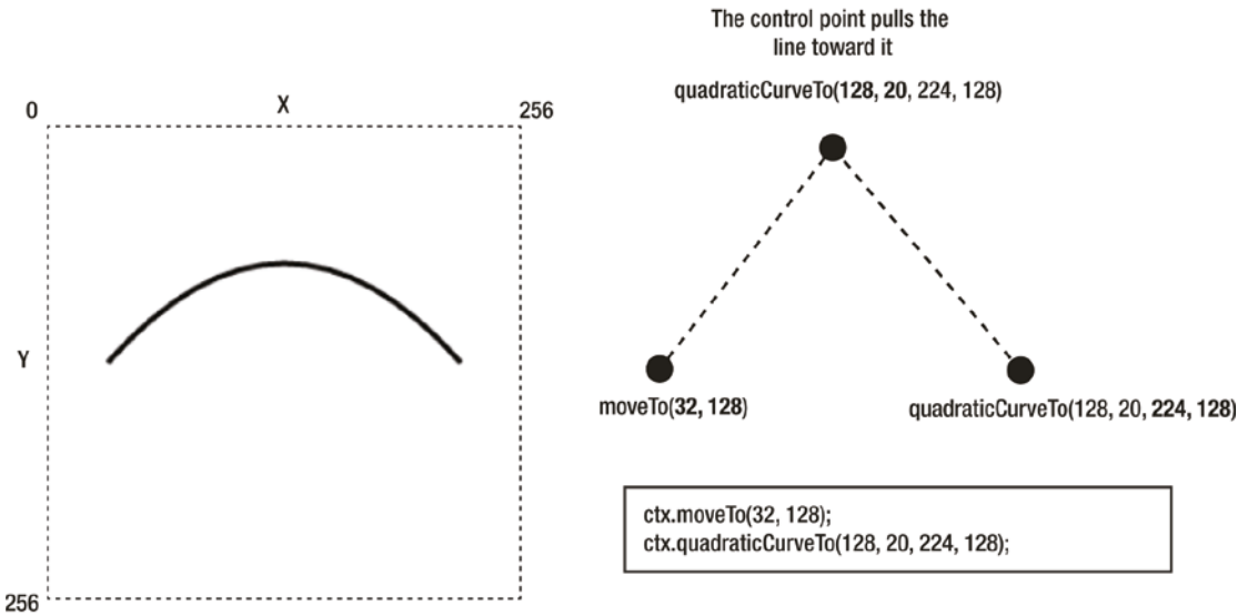
Figure 2-12. A quadratic curve
