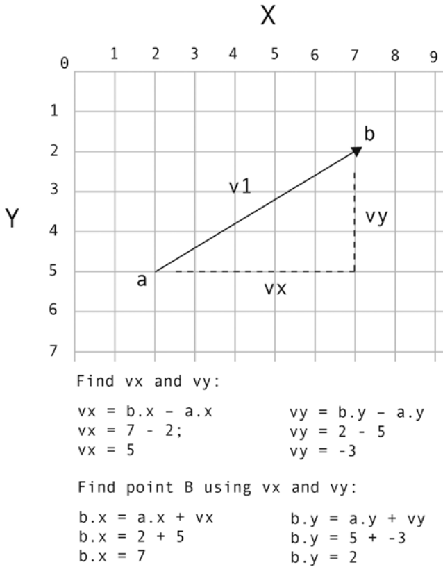
Figure A-3. The vector's x and y components: v_x and v_y
