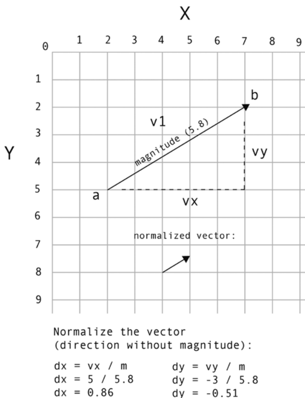
Figure A-8. Normalize the vector to help scale it to a different magnitude
