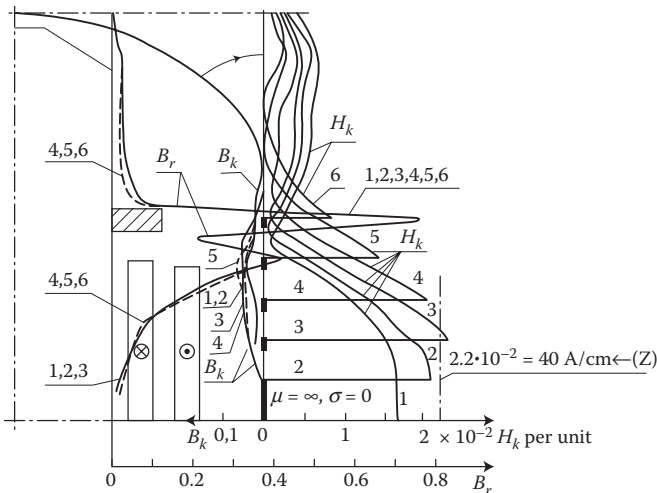
FIGURE 4.22 Two-dimensional analysis of the influence of height 1,2,3... of magnetic screen (shunt) of tank on the field H_{ms} = H_t on the surface of transformer tank walls; B_r —normal to tank, B_c —radial in windings. (Adapted from Turowski J.: Proc. of Jubilee Conference "The Transformer Production is 100 Years Old." Budapest, June 18–21, pp. 470–477 [4.26].)
