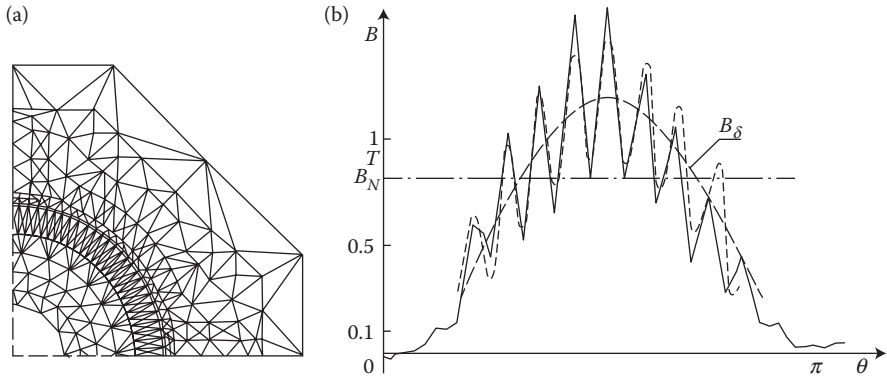
FIGURE 5.34 Calculation of flux density in the air gap of a DC motor, with the FEM: (a) the FEM mesh for the motor with compensation winding, (b) the calculated slot pulsation ——— FEM, — · — the author's formulae (5.43)—for motor without compensation windings. (Adapted from Rizzo M., Savini A., and Turowski J.: Internat. Conference on Electric Machines. ICEM'88 . Pisa, Italy. September 12–13, 1988, Vol. 1, pp. 85–88 [5.12]; Rizzo M., Savini A., and Turowski J.: Proc. of the Internat. Conference on Electric Drives ICED'88 . Polana Brasov, Romania, September 20–22, 1988, Paper 8.1–10, pp. 1–9 [5.13].)
