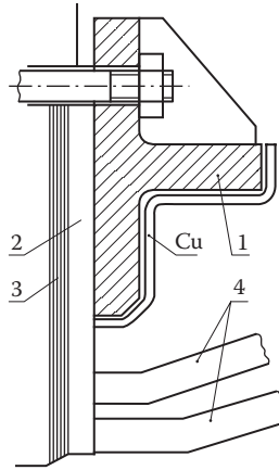
FIGURE 4.28 A copper screen of the periphery flange (1) of an 800 MVA turbogenerator, (Adapted from Doi S., Ito K., and Nonaka S.: IEEE Transactions , PAS-104(7), 1985, 1856–1862), (2) distancing plate, (3) package of stator core, (4) endwinding of the stator windings.
