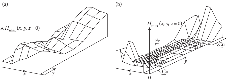
FIGURE 7.23 An interactive study of the field H_{\max} on the surface of tank of a 150 kV three-phase transformer, with the help of the RNM-3D program: (a) without any screens; (b) with partial, combined Cu screens and Fe frame (Figure 4.20b). (Adapted from Turowski J., Kopeć M., and Turowski M.: ISEF'89. Electromagnetic Fields in Electrical Engineering. COMPEL . London: James & James, 1990, pp. 113–116; and ITMA'91 . New Delhi, India [4.28].)
