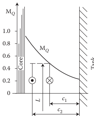
FIGURE 5.6 Variability of the equivalent coefficient M_Q of transformer winding mirror image at the surface of a solid steel wall versus the spot of measurement in a flat system. (Adapted from Kazmierski M.: An estimation of approximate methods for the analysis of electromagnetic fields in transformers. Rozprawy Elektrotechniczne , 16(1), 1970, 3–26 [5.9].)
