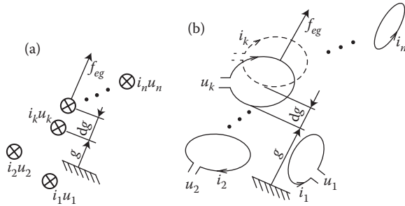
FIGURE 8.1 The virtual work f_{eg} \cdot dg in a system of: (a) conductors, (b) current circuits. (Adapted from Turowski J.: Fundamentals of Mechatronics (in Polish). AHE-Lodz, 2008 [1.20]; Turowski J. (1) (Editor and author 35%) et al.: Analysis and Synthesis of Electromagnetic Fields . (in Polish). Wroclaw: OSSOLINEUM - PAN, 1990; where §3 Reluctance network method RNM; §5 Coupled fields. (2) Computational magnetics. (in English). (J. Sykulski, editor), London: Chapman & Hall Stellenbosch, 1995 where: §4 Turowski J.: Reluctance networks RNM. and §6 Coupled Fields [1.17].)
