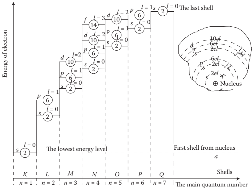
FIGURE 1.3 Diagram of permissible energy levels of electrons in a multielectron atom (with no scale regards): l —Azimuthal quantum number; s, p, d, f —subshells; ②, ⑥, and so on—maximal permitted number of electrons in a given subshell.
