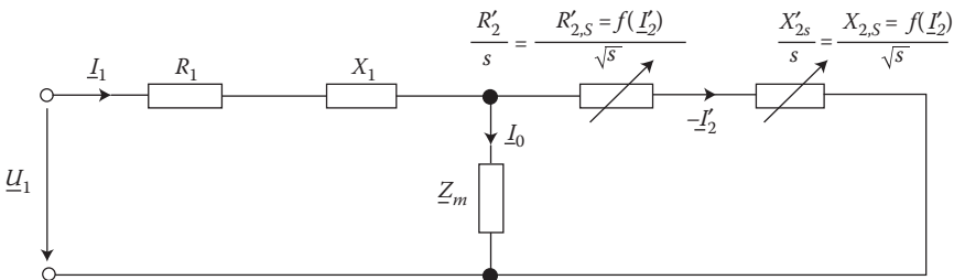
FIGURE 6.15 Equivalent circuit of induction motor with a solid steel rotor.
