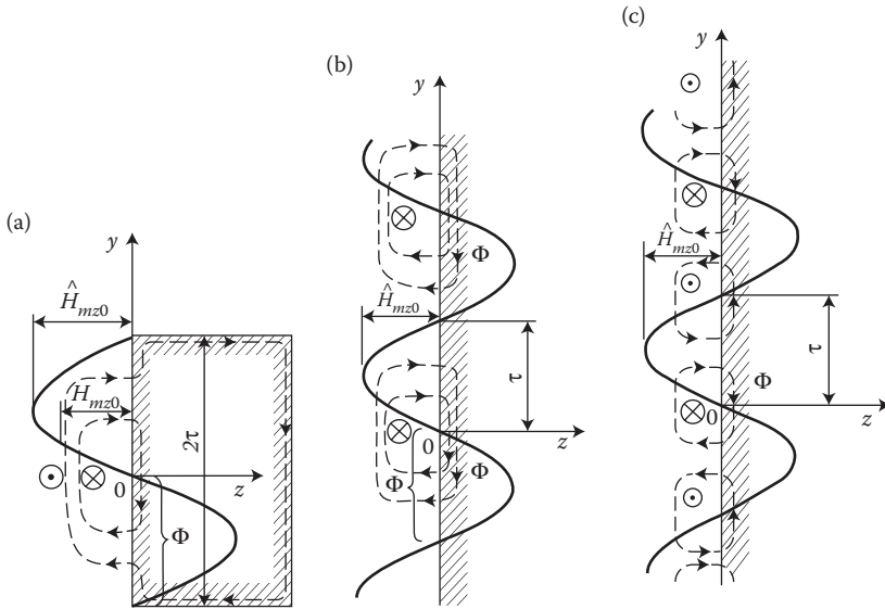
FIGURE 7.11 Typical cases of distribution of the normal component of field H_{mz0} on the surface of a steel half-space.
