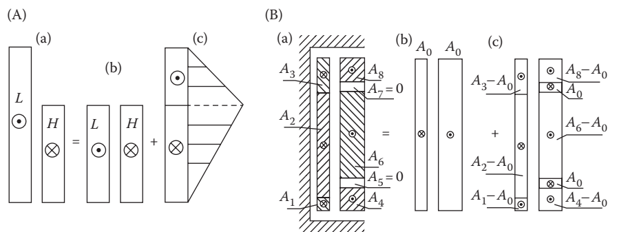
FIGURE 7.16 Division of ampere-turns of a transformer. (a) Asymmetric cylindrical winding, (b) fictitious symmetric component, and (c) fictitious sandwich component L_a = I_2 N_2 ; H_a = I_1 N_1 . (A) A simplified model with a graph of radial ampere-turns; (B) with double asymmetry.
