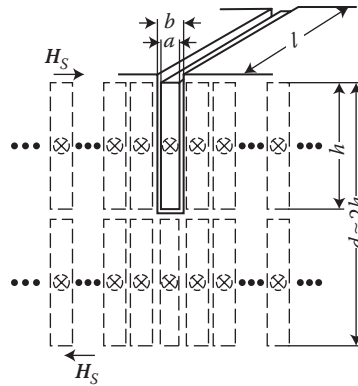
FIGURE 5.28 Multiple mirror images of a conductor in a deep-slot of an electric machine. (Adapted from Turowski J.: Wave method of calculating the screens and elements of electric machines. (in Russian). Elektricitstwo , (12), 1965, 53–58.)
