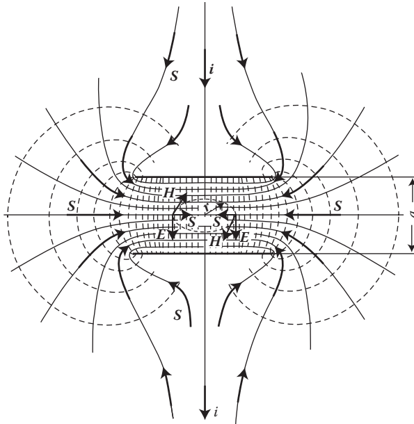
FIGURE 3.4 Distribution of power flux in a parallel-plate capacitor; \mathbf{S} —Poynting vector = power flux density (VA/m 2 ).
