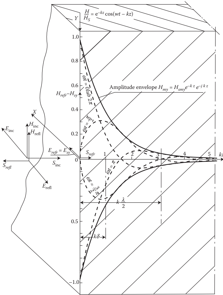
FIGURE 2.10 Penetration of electromagnetic plane wave into a metal half-space: envelopes of amplitudes and instantaneous field distributions, for several arbitrary time instants: t_1, t_2, \dots
