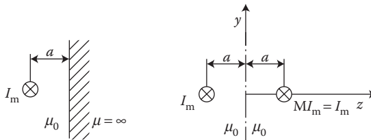
FIGURE 5.39 The full, positive ( M = +1 ) mirror image of a current.
