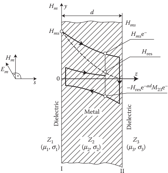
FIGURE 4.7 Reflections of the magnetic component of electromagnetic wave that impinges and penetrates a thin screen from one side.
