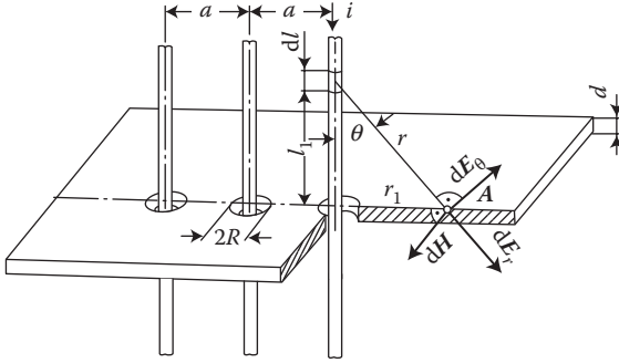
FIGURE 5.21 Components of field on the cover surface. (After Turowski J.: Losses and local overheating caused by stray fields. (in Polish). Scientific Archives of the Technical University of Lodz “ Elektryka ”, No. 11, 1963, pp. 89–179 ( Habilitation (DSc) dissertation; 1st Ministry Award ) [2.41]; Turowski J.: Losses in single and three phase transformers covers. (in Polish). Rozprawy Elektrotechniczne , (1), 1959, 87–119 [4.16].)
