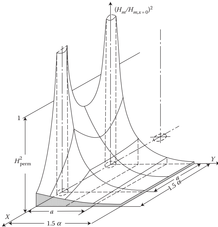
FIGURE 6.8 Distribution of active power losses on the cover of a three-phase power transformer at \mu = \text{const} ; 1—excessive heating line, 2—the distance H_{\text{perm}}^2 —the relative value permitted from the point of view of local excessive heating hazard, see Equations 9.10, 9.28 and Figure 9.2 [6.17], [7.16].
