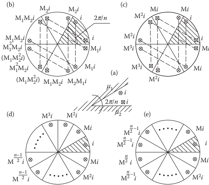
FIGURE 5.9 Mapping (simulation) of a real system: (a) (center) of currents placed between iron walls, by means of a field of fictitious currents placed in the area of \mu_r = 1 ; (b) at different saturation values \mu_1, \mu_2 of the neighboring iron walls M_1 = (\mu_{r1} - 1)/(\mu_{r1} + 1) , M_2 = (\mu_{r2} - 1)/(\mu_{r2} + 1) ; (c) at identical saturation M_1 = M_2 = M ; (d) at an odd n , (e) at an even n . (Adapted from Turowski J., Andryszczak W., and Pelikant A.: Application of the method of mirror images to calculation of the slot impedances, taking into account the saturation of the teeth. (in Polish). “ Elektryka ” Scientific Papers of Techn. University of Lodz , (74), 1983, 187–198 [5.17].)
