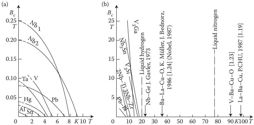
FIGURE 1.15 Dependence of critical flux density B_c on the absolute temperature T , after different sources: (a) ideal, "soft" superconductors; (b) nonideal, "hard" superconductors (Kunzler 1962) and ceramic superconductors (30–100 K).
