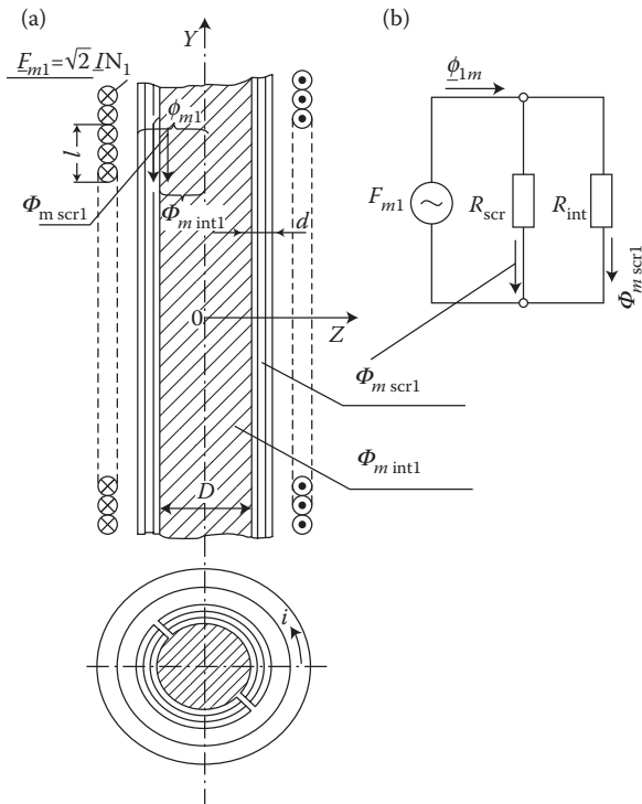
FIGURE 4.5 Longitudinal magnetic screen (shunt) of a solid steel (internal) part; \underline{F}_{m1} = \sqrt{2}IN_1 —maximum in time magnetomotive force (ampere-turns) per unit length (A/m); I —rms current; N_1 —number of turns per meter; \underline{F}_{m1} = \underline{F}_{m,scr1} + \underline{F}_{m,int1} —total maximum in time magnetic flux (Wb); \underline{F}_{m,scr1}, \underline{F}_{m,int1} —components of total flux in screen (shunt) and internal steel part, respectively; R_{scr1} —per-unit reluctance ( 1/H ) of magnetic screen (laminated shunt); R_{int1} —per-unit reluctance ( 1/H ) of the internal part made of solid steel.
