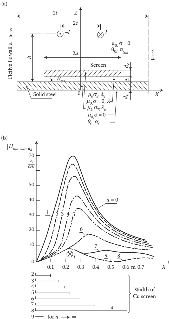
FIGURE 6.24 The calculation of power loss density P_1 = \frac{a_p}{2} \sqrt{\frac{\omega \mu_s}{2s}} \frac{|H_{ms}|^2}{2} (in W/m 2 ) in a steel wall screened partly from the field of a pair of conductors: (a) the calculation model; (b) the field on the steel surface, at z = d_k . (Adapted from Kaźmierski M. and Kersz I.: Effectiveness of longitudinal conducting screens. Part I. Electromagnetic field and stray losses. Part II. Temperature rise. (in Polish). Rozprawy Elektrot. , (2–3), 1989 [6.10].)
