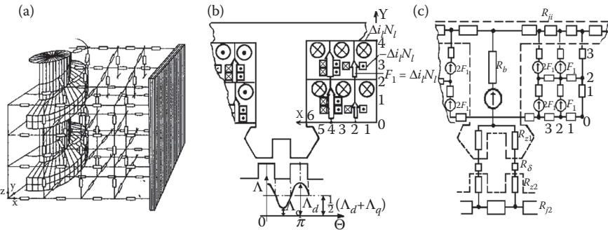
FIGURE 9.10 RNM-3D modeling of distributed field by an equivalent reluctance circuit: (a) magnetic separator of chimney smoke (Adapted from Ciosk K., Gierczak E., Mendrela E.A. Magnetic and Force Field in the Gap of Magnetic Screw Separator (in Polish). Wiadomosci Elektrotechniczne . LXII, No 6, 1994, p. 236–238.); (b) pole winding of stepping motor; (c) equivalent reluctance scheme for a wide winding. (Adapted from Turowski J.: Computational magnetics . (in English). J. Sykulski (Editor), London: Chapman & Hall Stellenbosch, 1995 where: §4) Turowski J.: Reluctance networks RNM [1.17/2].)
