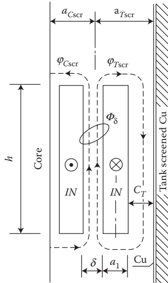
FIGURE 10.28 Distribution of the leakage flux \Phi_\delta between core and tank wall screened with Cu screens.
