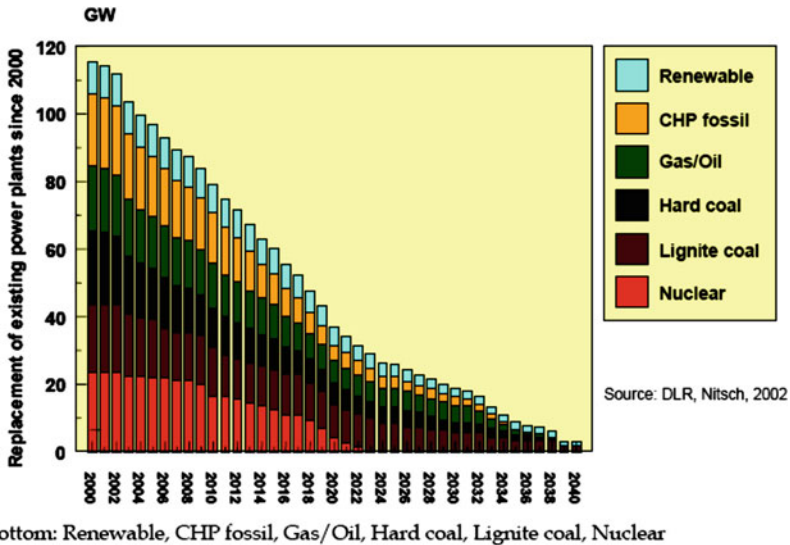
Fig. 2.51 Need for replacement of existing power plants until 2040
