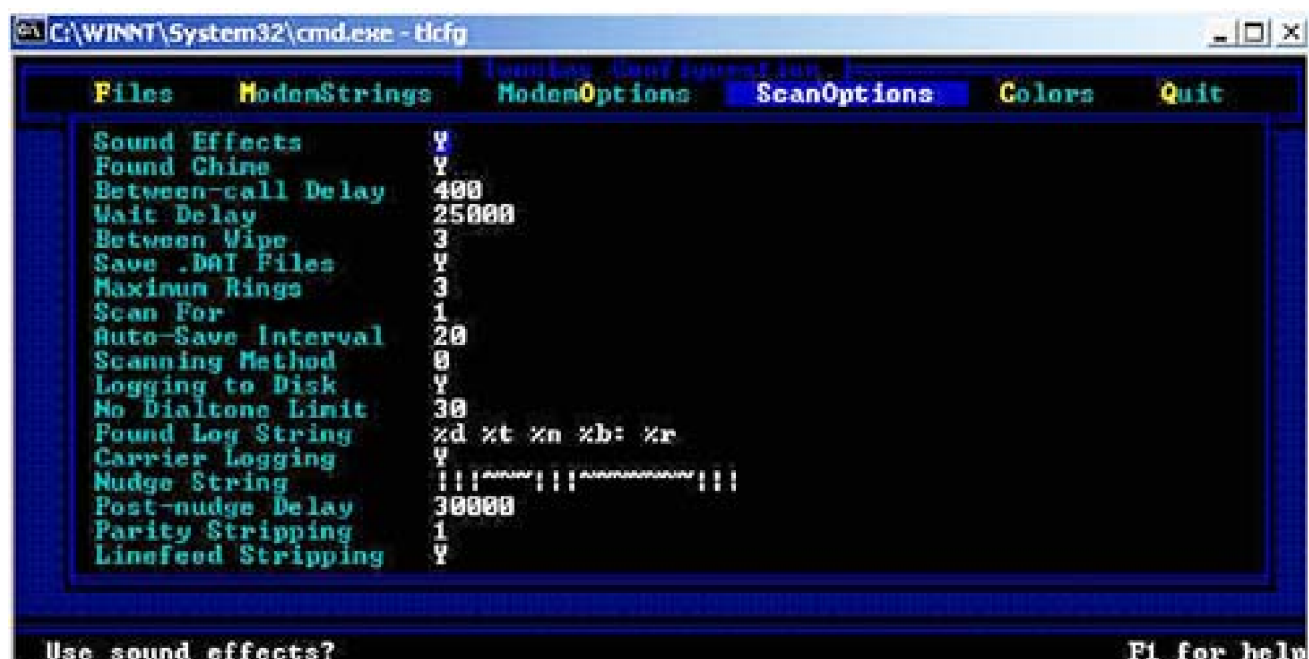
Figure 6-5. ToneLoc ScanOptions menu
