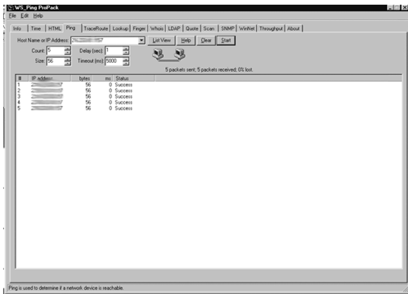
Figure 12-2. WS_Ping ProPack Ping function
