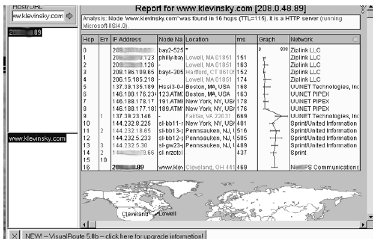
Figure 12-32. Sample traceroute with VisualRoute
