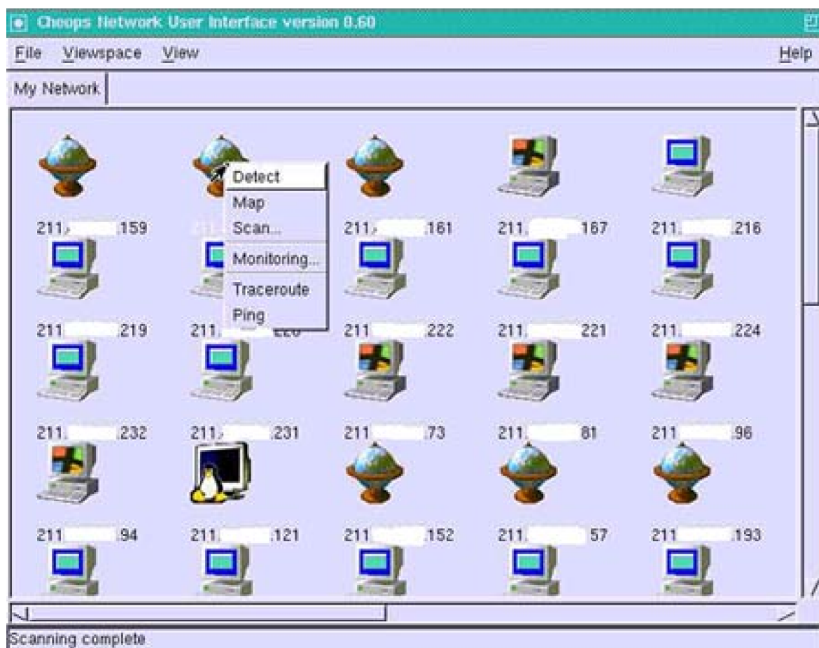
Figure 9-4. Cheops port scan results
