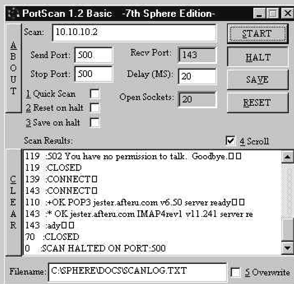
Figure 13-3. 7th Sphere Scan screen
