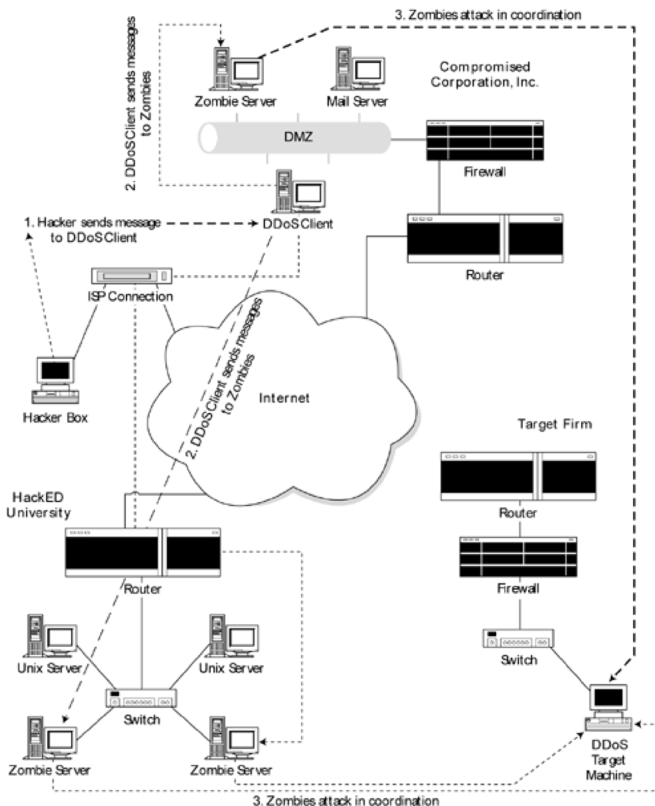
Figure 21-1. Diagram of a distributed denial-of-service attack
