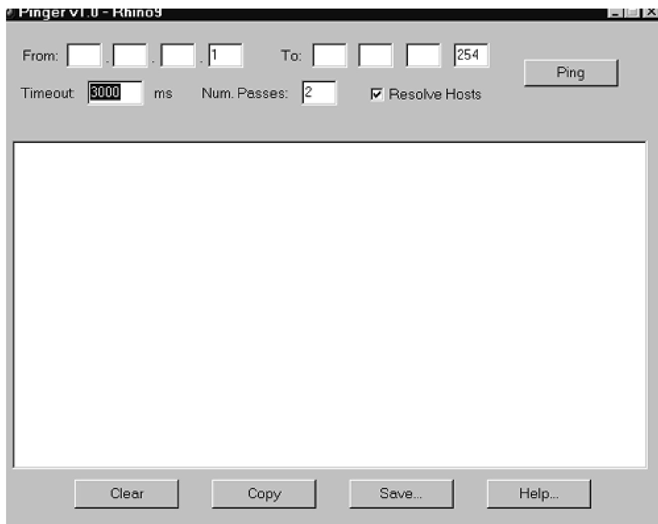
Figure 12-31. Pinger user interface
