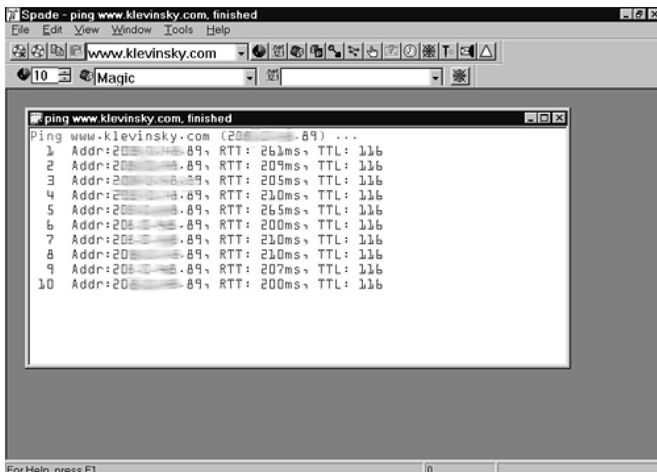
Figure 12-18. Sample Ping output in Sam Spade
