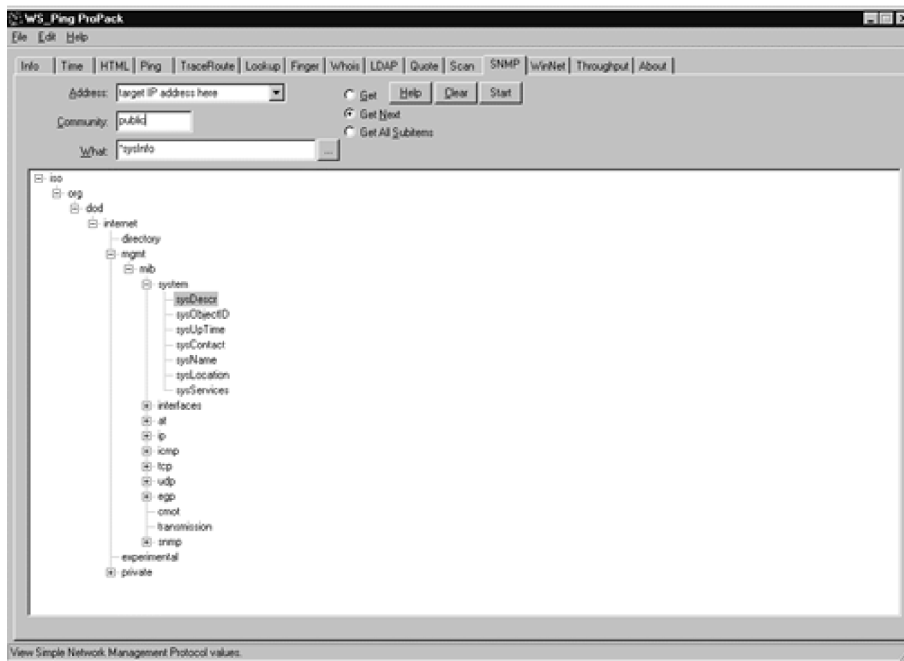
Figure 12-8. WS_Ping ProPack SNMP screen
