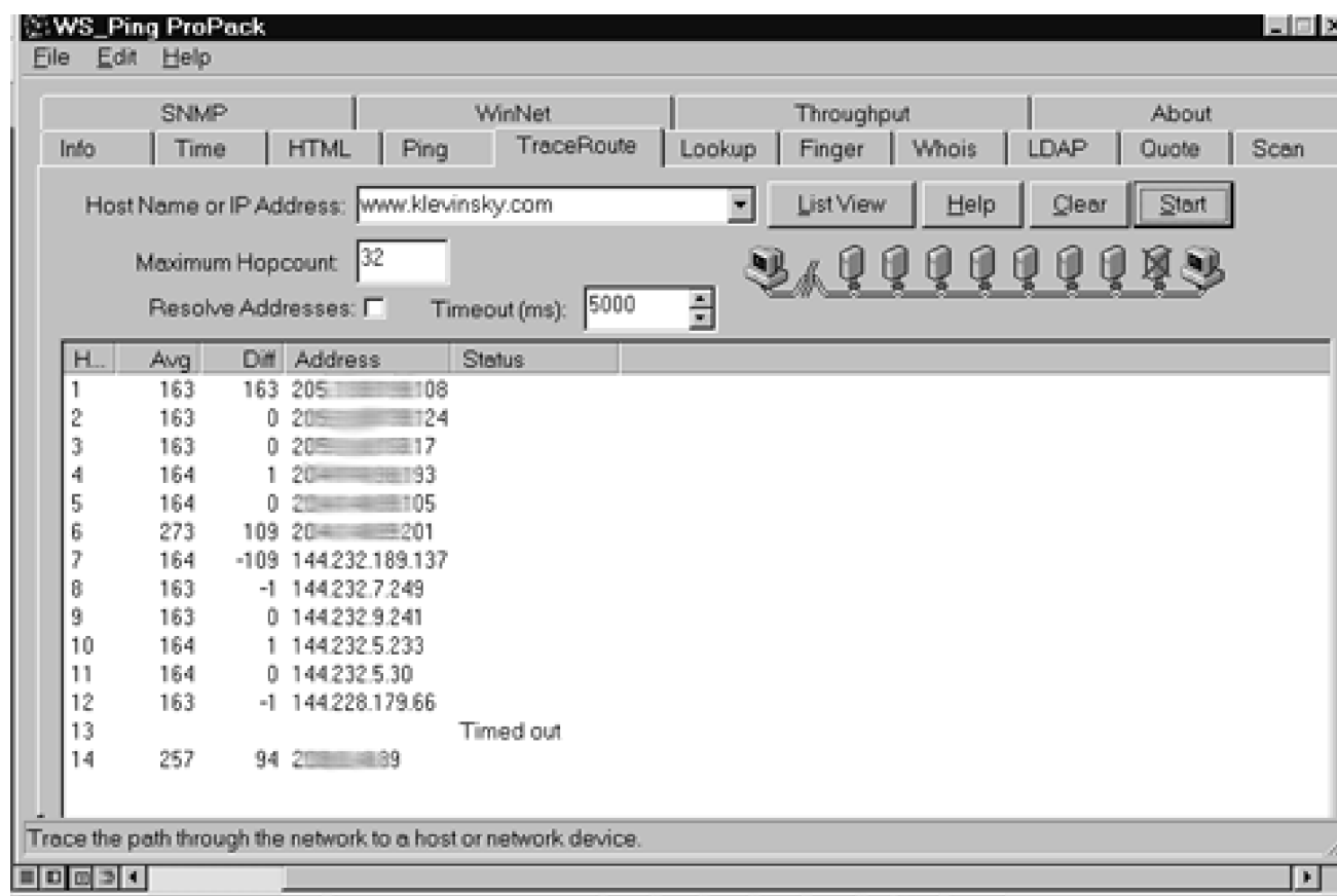
Figure 12-3. WS_Ping ProPack TraceRoute
