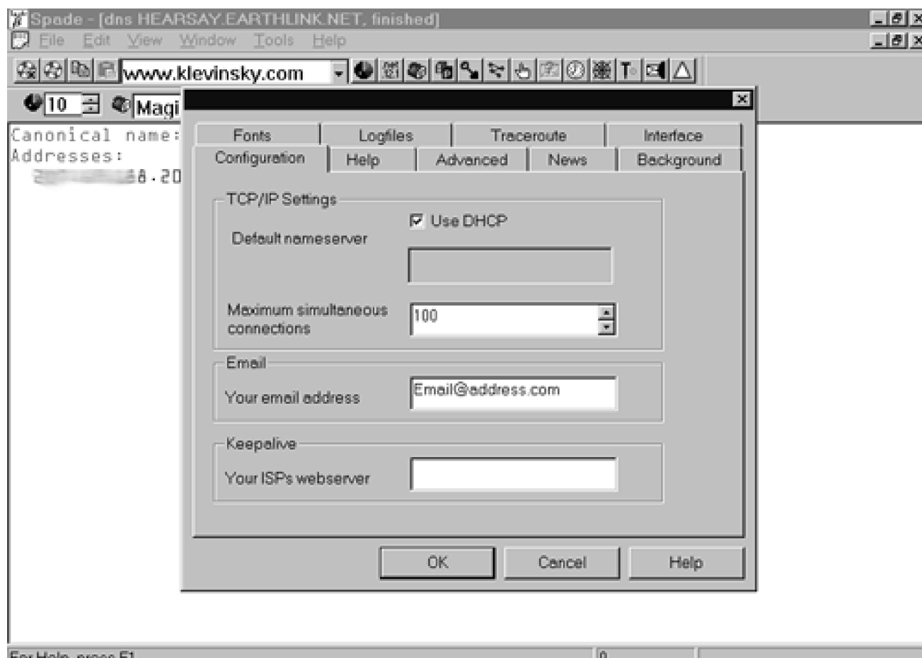
Figure 12-27. Sam Spade Advanced options screen
