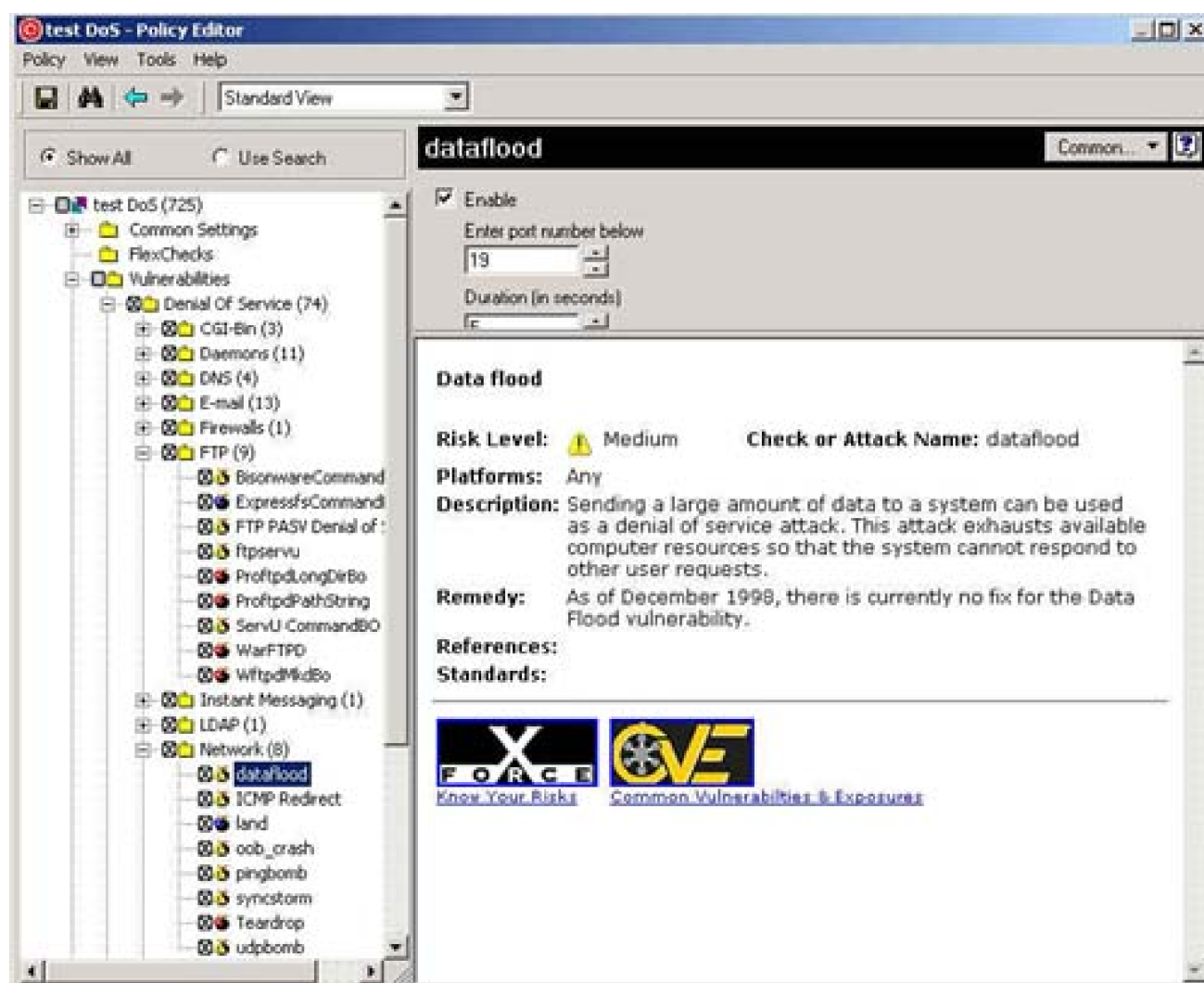
Figure 21-5. ISS Internet Scanner DoS attacks
