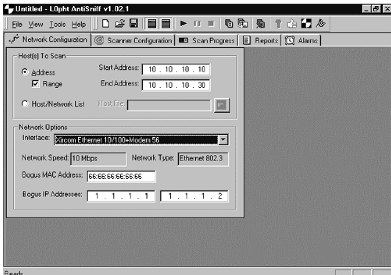
Figure 14-3. AntiSniff Scanner Configuration window
