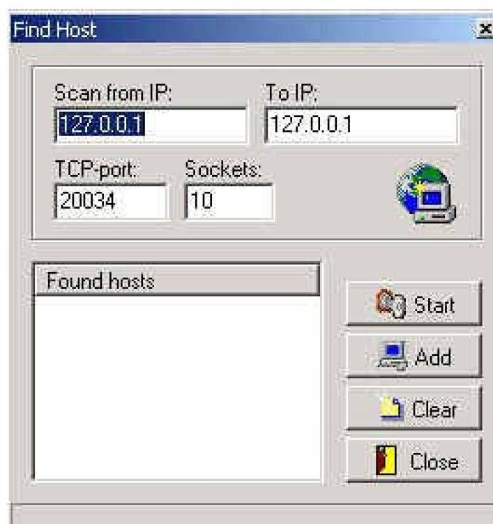
Figure 18-10. NetBus Find Host screen
