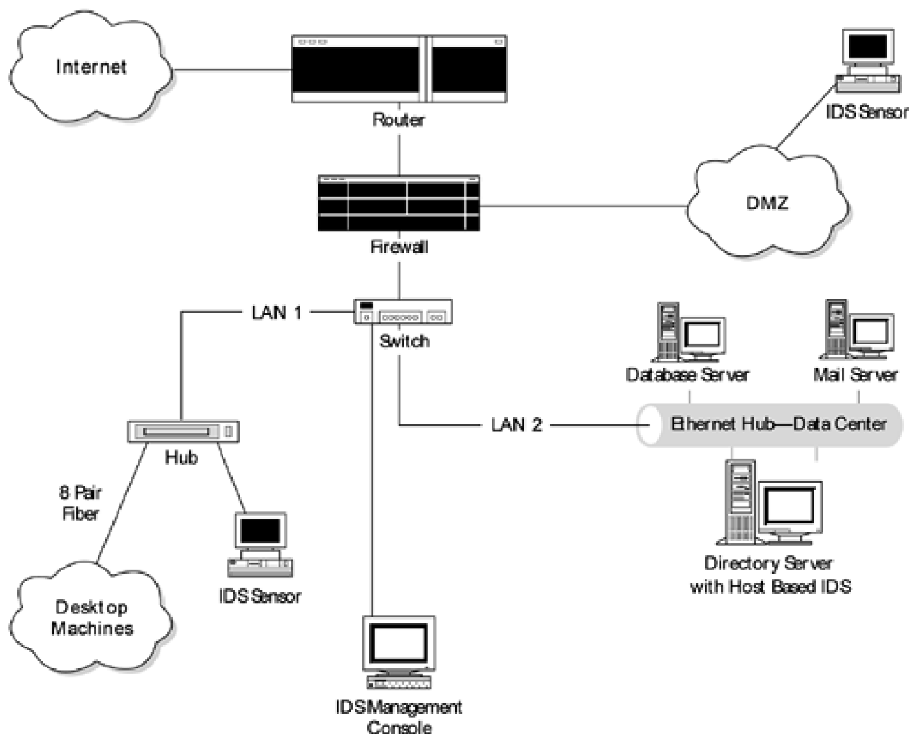
Figure 19-1. Sample architecture for an intrusion detection system
