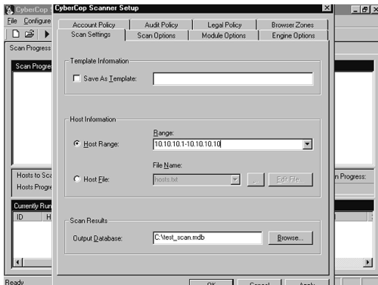
Figure 11-2. CyberCop Scanner Engine Options screen
