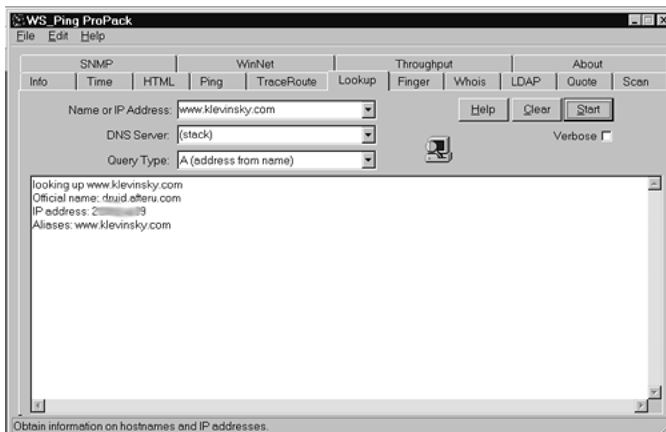
Figure 12-5. Query Type drop-down box in WS_Ping ProPack
