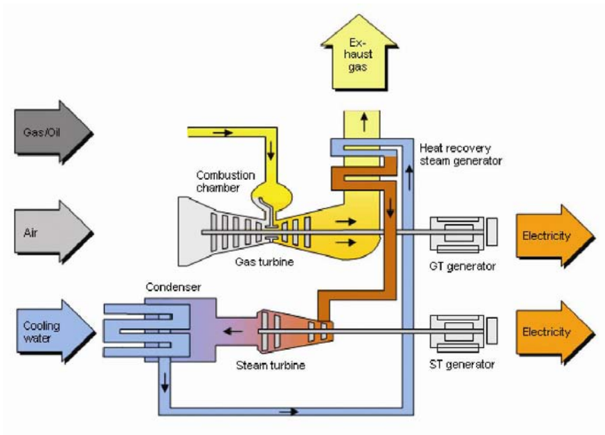
Figure 15. Process Schematic: Combined Cycle Power Plant
