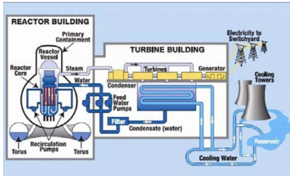
Figure 18. Process Schematic: Boiling Water Reactor (BWR)
