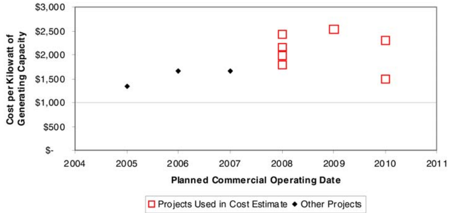
Wind Project Cost Trends
