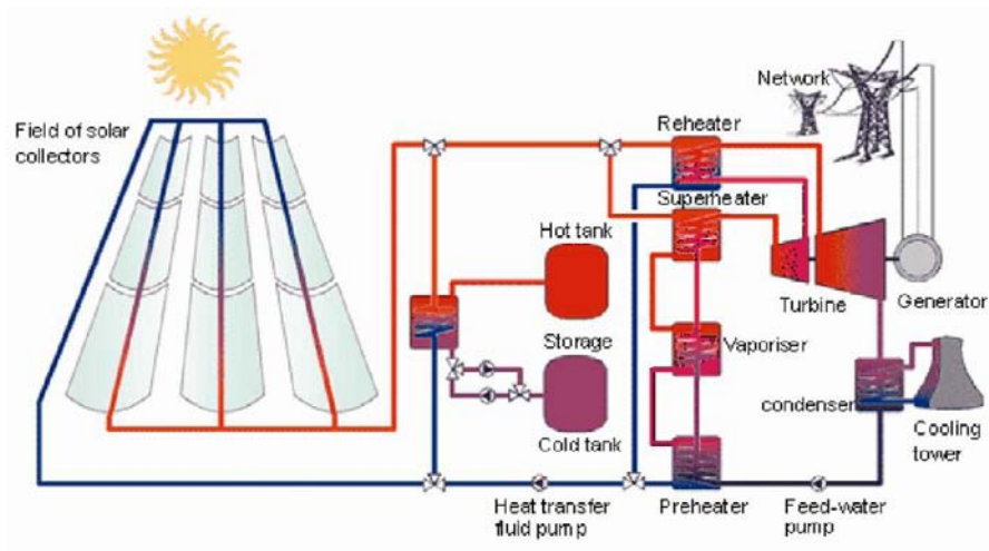
Figure 25. Process Schematic: Parabolic Trough Solar Thermal Plant
