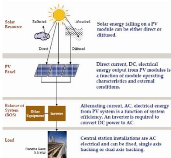
Figure 28. Process Schematic: Central Station Solar Photovoltaic Power
