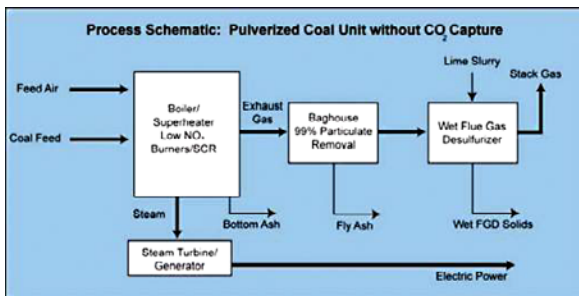
Figure 9. Process Schematic: Pulverized Coal without Carbon Capture
