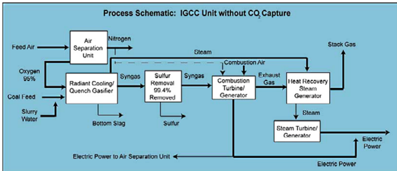
Figure 12. Process Schematic: IGCC without Carbon Capture
