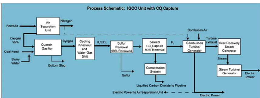
Figure 13. Process Schematic: IGCC with Carbon Capture
