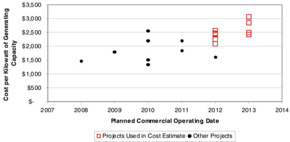
Pulverized Coal Project Cost Trends
