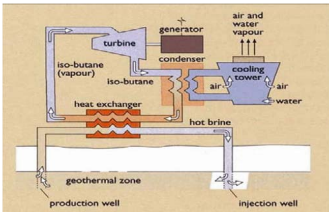
Figure 23. Process Schematic: Binary Cycle Geothermal Plant
