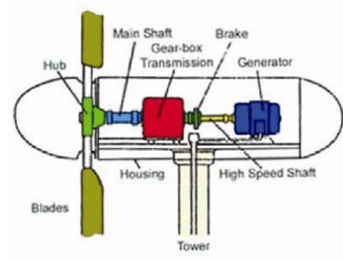
Figure 20. Schematic of a Wind Turbine
