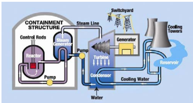
Figure 17. Process Schematic: Pressurized Water Reactor (PWR)
