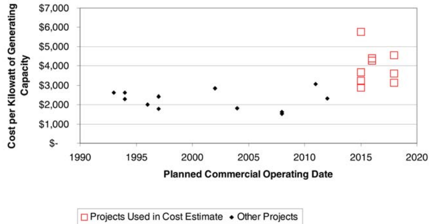
Nuclear Project Cost Trends
