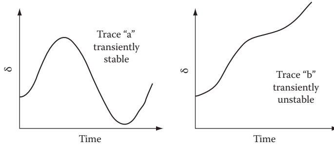
FIGURE 9.1 Plots showing the trajectory of generator rotor angle through time for transient stable and transiently unstable cases.
