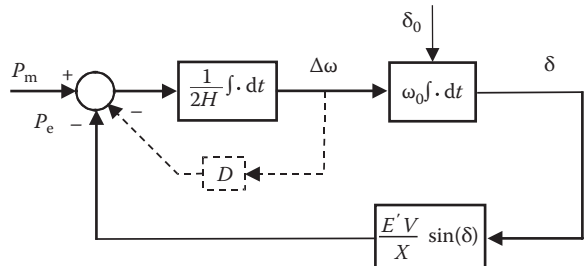
FIGURE 13.3 Simplified block diagram of generator electromechanical dynamics.
