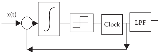
FIGURE 5.3 Delta modulator and error.
