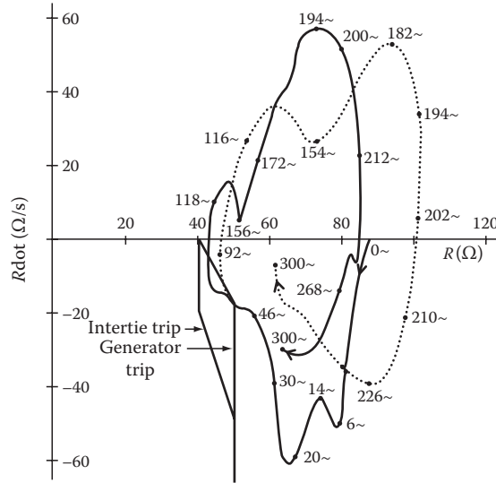
FIGURE 13.7 R - \dot{R} phase plane for loss of Pacific HVDC Intertie (2000 MW). Solid trajectory is without additional generator tripping. Dashed trajectory is with additional 600 MW of generator tripping initiated by the R - \dot{R} controller generator trip switching line. (From Haner, J.M. et al., IEEE Trans. Power Delivery , PWRD-1, 35, 1986.)
