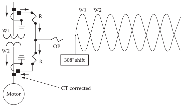
FIGURE 6.17 Corrected connection.
