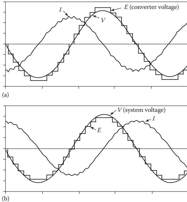
FIGURE 19.21 (a) STATCOM capacitive operation and (b) STATCOM inductive operation. (From Erinmez, I.A. and Foss, A.M., (eds.), Static synchronous compensator (STATCOM), Working Group 14.19, CIGRE Study Committee 14 , Document No. 144, August 1999.)
