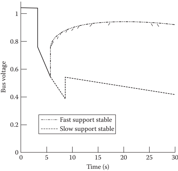
FIGURE 11.9 Simulation of voltage collapse.
