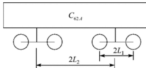
Fig. 6.13 Geometric dimension of the commonly used vehicles in China
