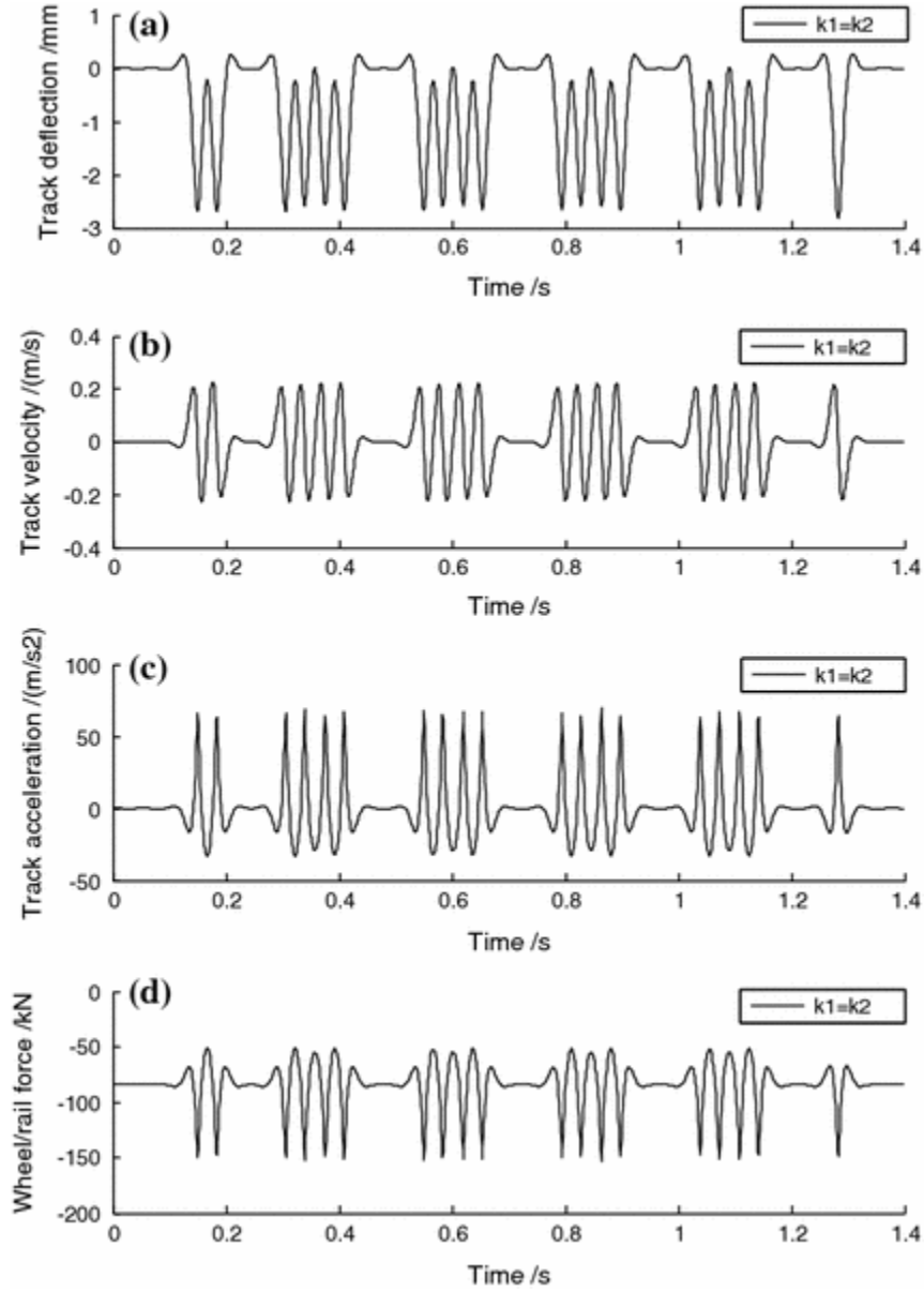
Fig. 2.10 Time history of the track deflection, velocity, and acceleration as well as the wheel-rail force at the point of stiffness abrupt change ( k_1 = k_2 , a = 1 \text{ mm} )
