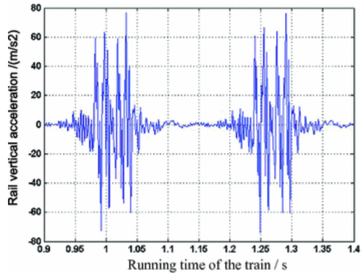
Fig. 9.14 Time history of the rail vertical acceleration
