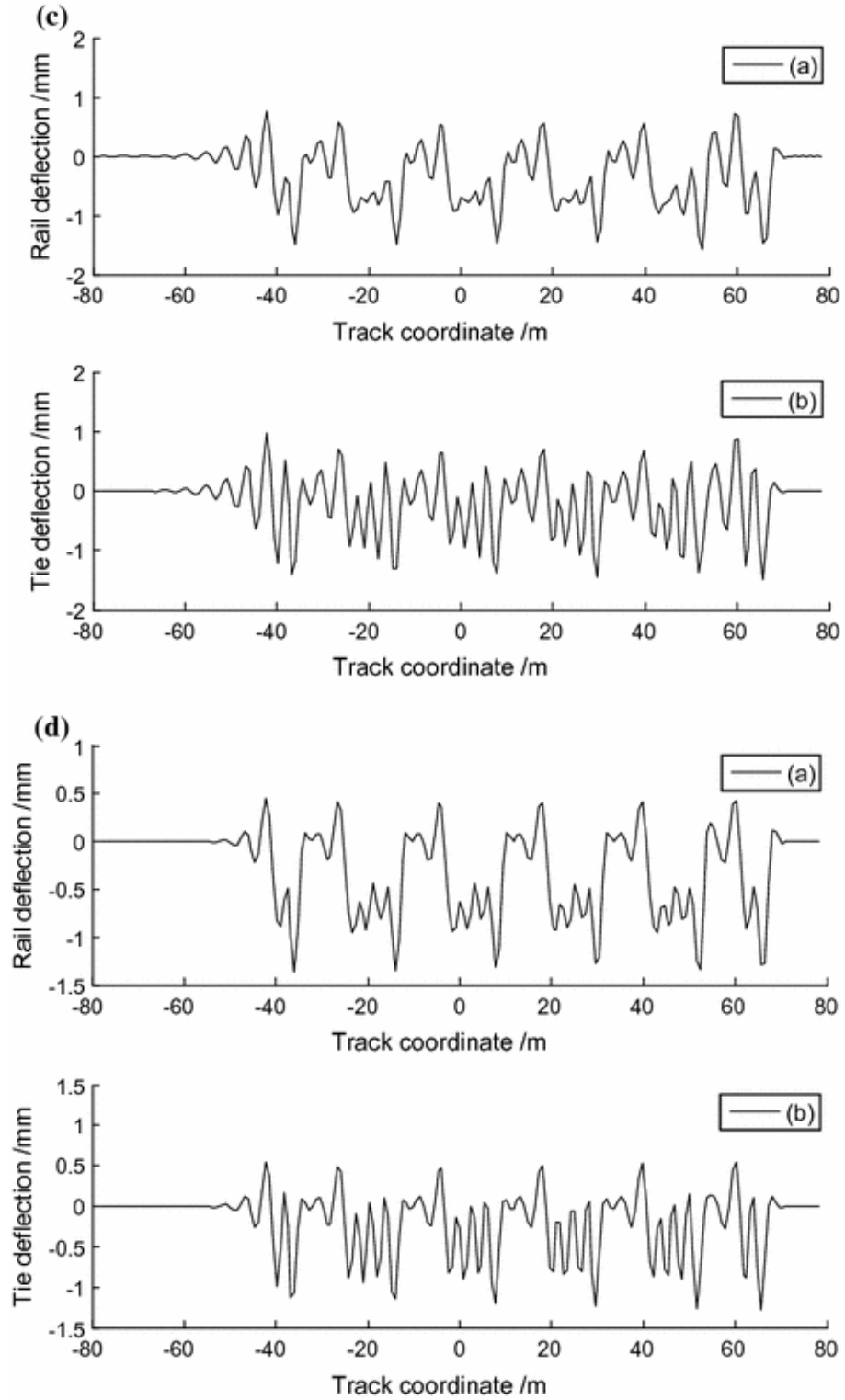
Fig. 3.12 Effect of the track foundation damping on track vibration (E_s = 2 \times 50 \text{ MN/m}^2; k_p = 2 \times 100 \text{ MN/m}^2; c_r = 2 \times 50 \text{ kN s/m}^2; V = 149 \text{ m/s}) . a
