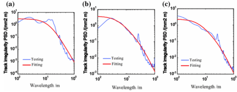
Fig. 5.4 The fitting curve of irregularity power spectrum for ballast track over subgrade of Hefei-Wuhan passenger-dedicated line . a Profile irregularity. b Alignment irregularity. c Cross level irregularity
