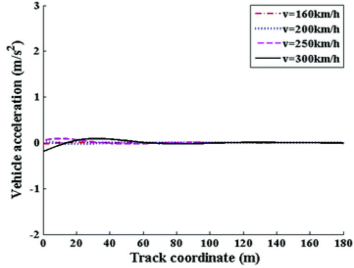
Fig. 12.4 Influence of train speeds on vertical acceleration of car body
