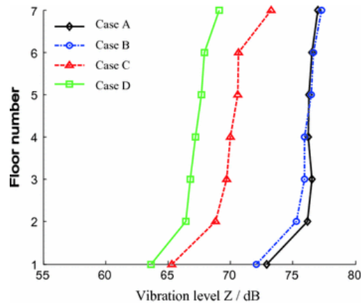
Fig. 15.23 Vibration level Z of each floor when both subways operate (Case A: both subways with integrated ballast track; Case B: subway 1 with floating slab track ; Case C: subway 2 with floating slab track; and Case D: both subways with floating slab track)
