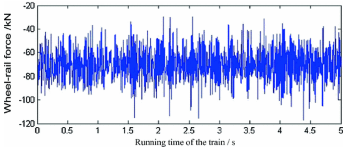
Fig. 10.24 Time history of the wheel-rail contact force
