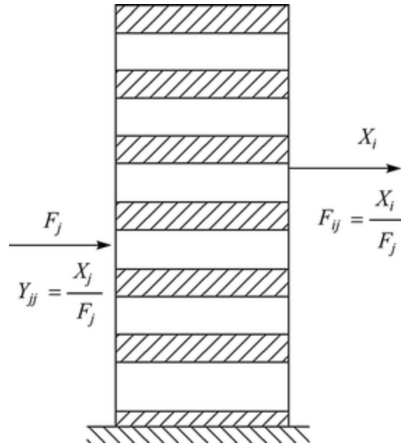
Fig. 4.1 The concept of admittance
