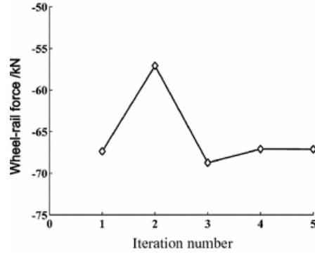
Fig. 7.10 Iteration process for wheel-rail contact force at time t
