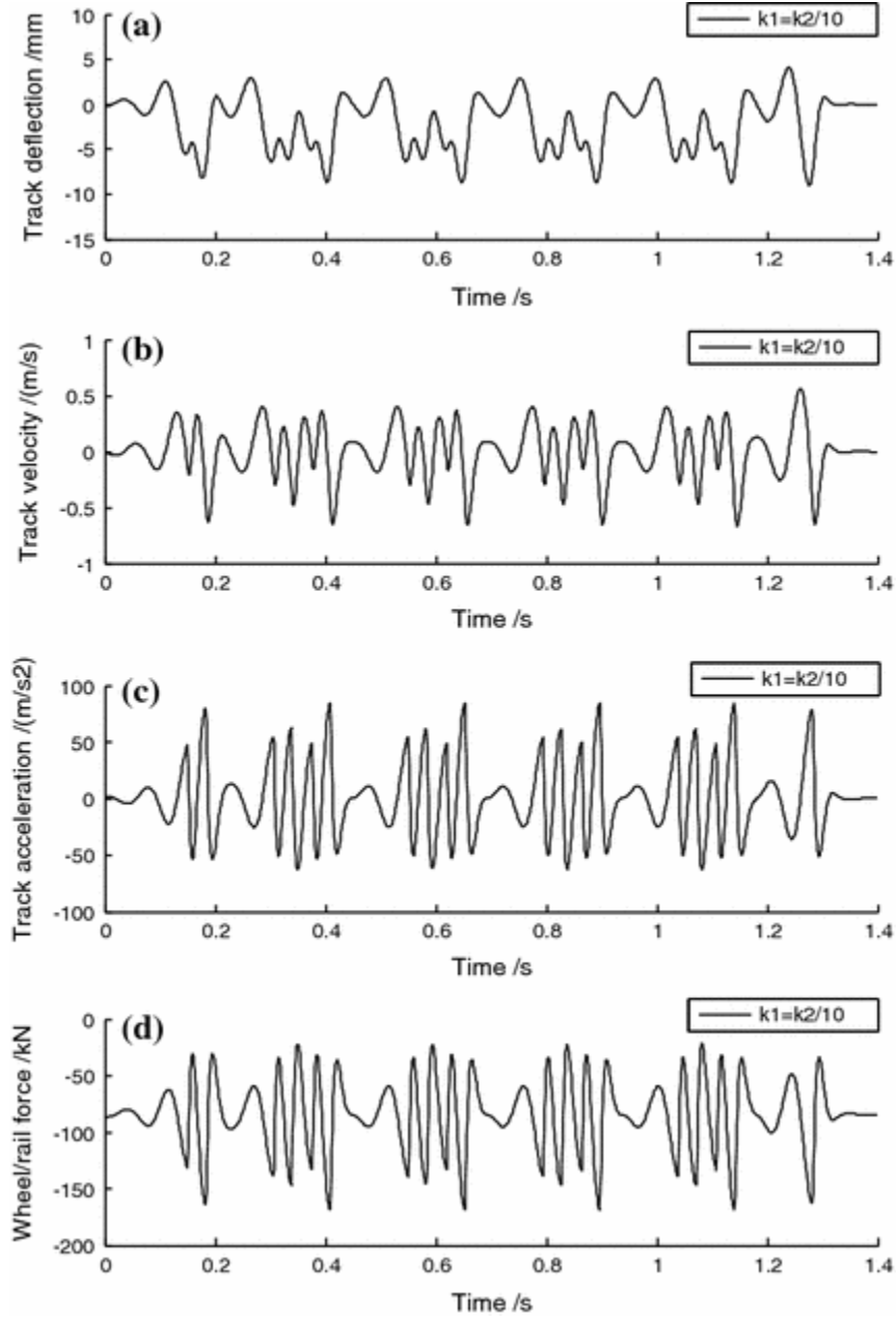
Fig. 2.13 Time history of the track deflection, velocity, and acceleration as well as the wheel-rail force at the point of stiffness abrupt change ( k_1 = \frac{k_2}{10} , a = 1 \text{ mm} )
