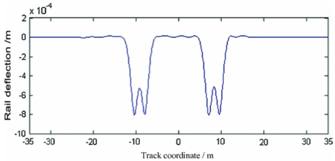
Fig. 10.14 Rail vertical displacement along the track direction
