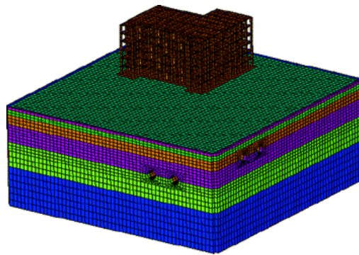
Fig. 15.15 3D finite element model of track-overlapping tunnels -ground-building
