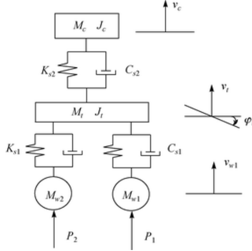
Fig. 6.11 Vehicle model of half a car with primary and secondary suspension system
