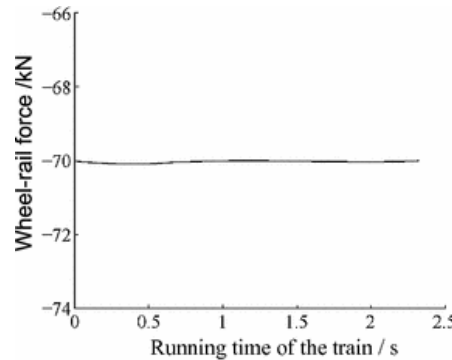
Fig. 7.13 Time history of wheel-rail contact force for convergence precision 1.0 \times 10^{-7}
