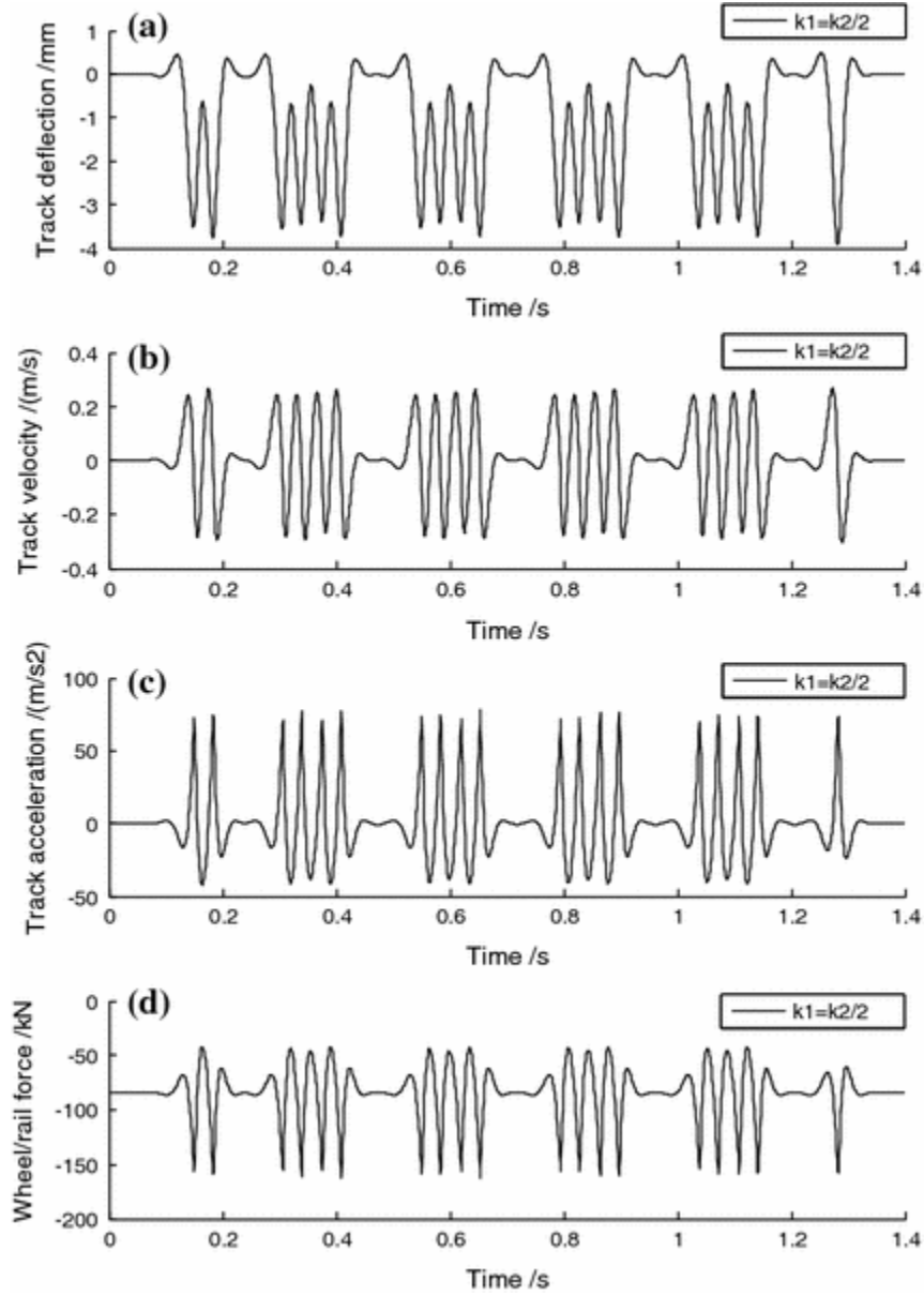
Fig. 2.11 Time history of the track deflection, velocity, and acceleration as well as the wheel-rail force at the point of stiffness abrupt change ( k_1 = \frac{k_2}{2} , a = 1 \text{ mm} )
