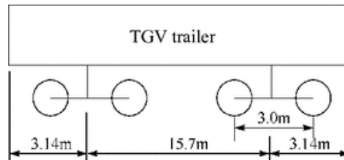
Fig. 6.17 TGV medium- and high-speed trailer
