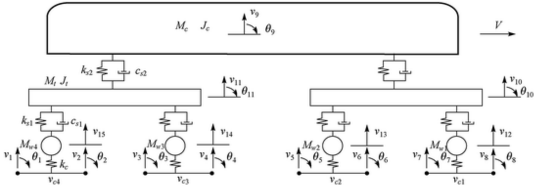
Fig. 9.4 Vehicle element model
