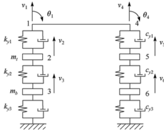
Fig. 9.1 Three-layer ballast track element model
