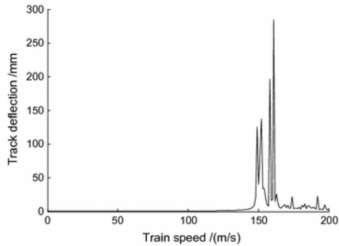
Fig. 3.3 The corresponding maximum track vibration deflection for different train speeds ( E_s = 2 \times 50 \text{ MN/m}^2 )
