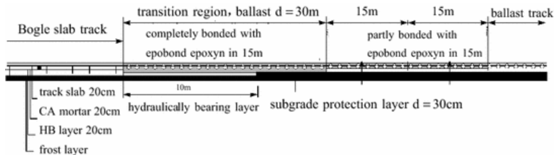
Fig. 14.11 Transition section between the ballast track and German Bögle slab track on subgrade
