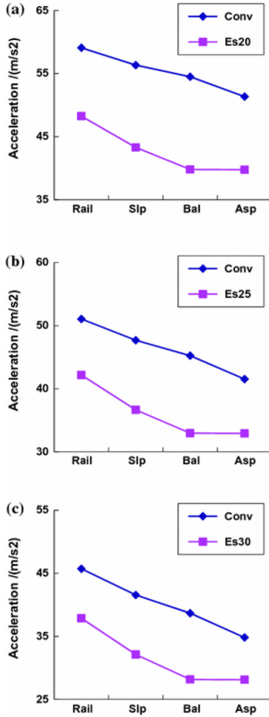
Fig. 3.27 Influence of subgrade module E_s with C_a = 20\% and H_a = 20\text{ cm} on accelerations of the track ( Slp sleeper, Bal Ballast, Asp Asphalt, Conv Conventional ballast track with soft subgrade, E_s subgrade module). a E_s = 20 MPa. b E_s = 25 MPa. c E_s = 30 MPa
