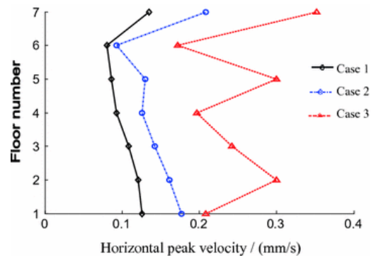
Fig. 15.19 Vibration velocity of each floor along the synthetic direction without vibration reduction measures (Case 1: a single operation of subway 1 with integrated ballast bed; Case 2: a single operation of subway 2 with integrated ballast bed; and Case 3: simultaneous operation of both subways with integrated ballast bed)
