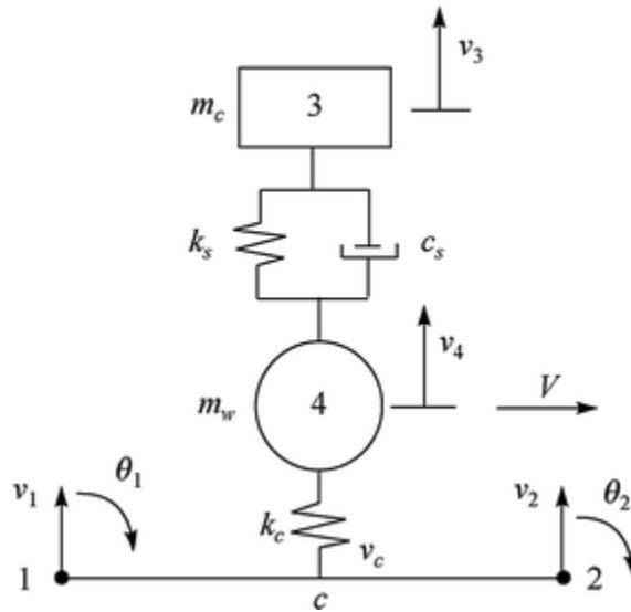
Fig. 8.2 Moving element model of a single wheel with primary suspension system
