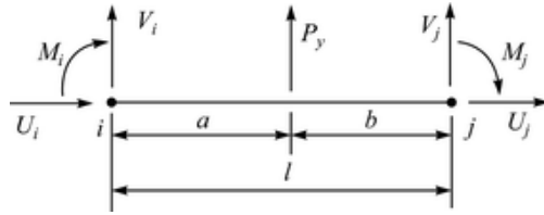
Fig. 6.3 Vertical concentrated load on beam element
