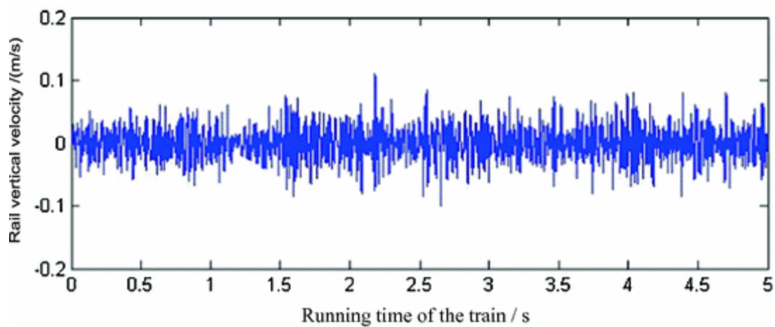
Fig. 10.17 Time history of the rail vertical velocity
