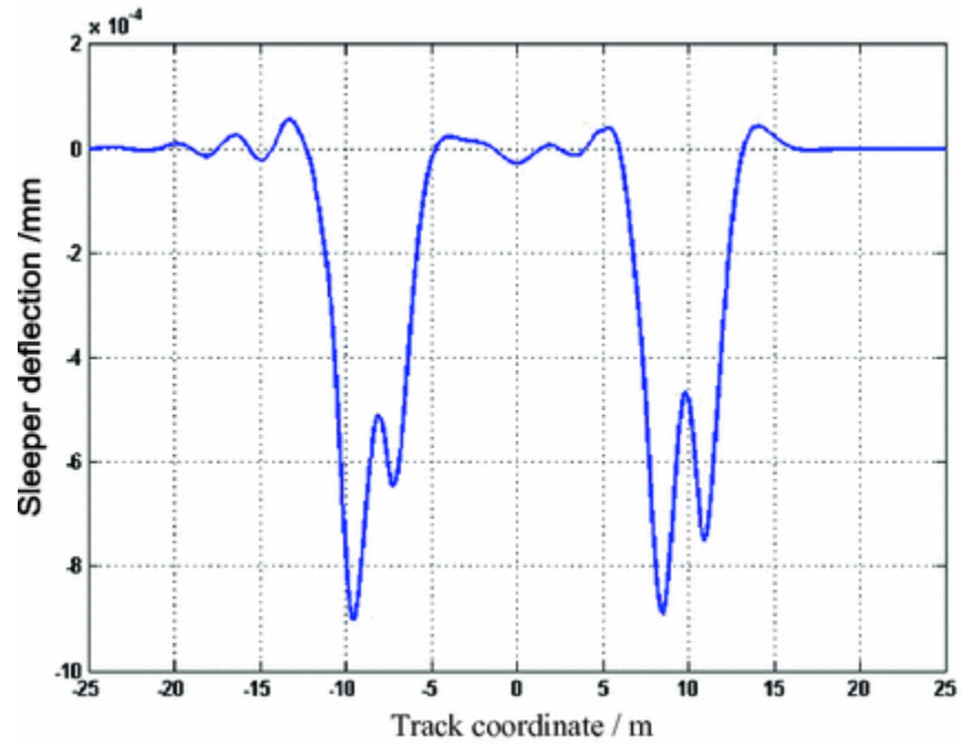
Fig. 9.13 Sleeper deflection along the track
