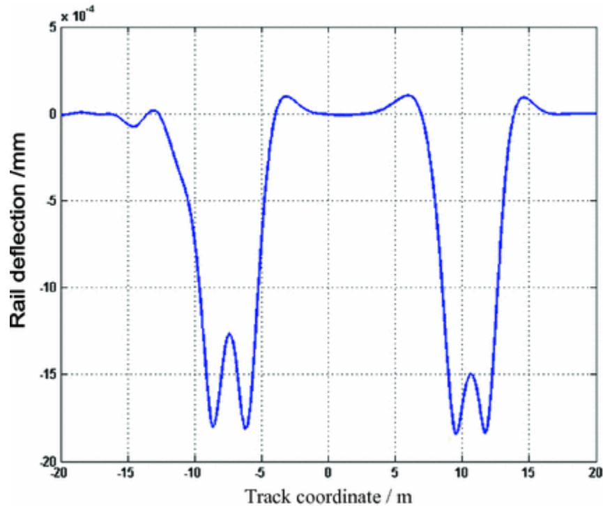
Fig. 9.12 Rail deflection along the track
