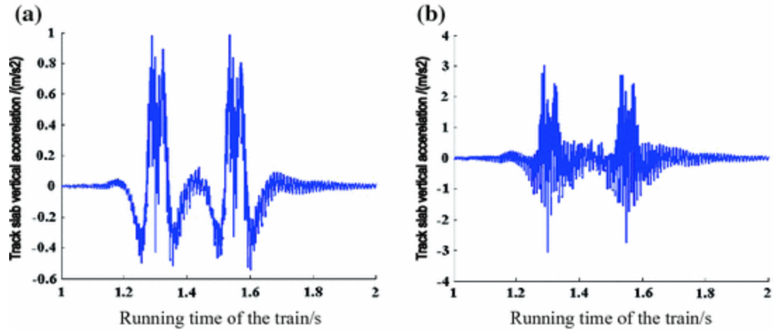
Fig. 13.13 Influence of different rail pad and fastener damping on the track slab vertical acceleration. a C_p = 3.63 \times 10^4 \text{ N s/m} . b C_p = 10 \times 10^5 \text{ N s/m}
