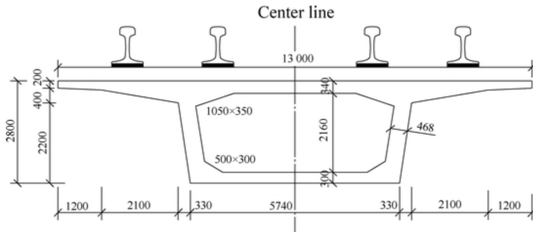
Fig. 4.5 Geometrical dimensions of box girder cross section
