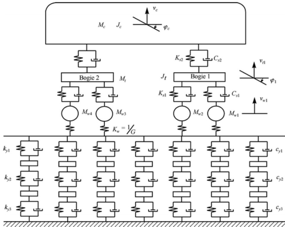
Fig. 6.5 Computing model of the vehicle-track system
