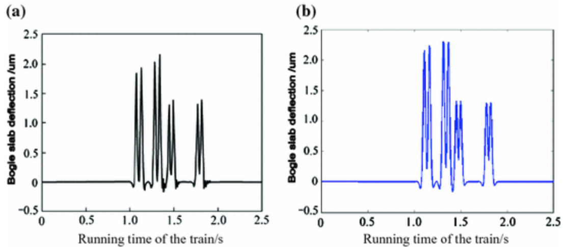
Fig. 13.4 Time history of the Bögle slab vertical displacements. a Results with FEM. b Results with the proposed method
