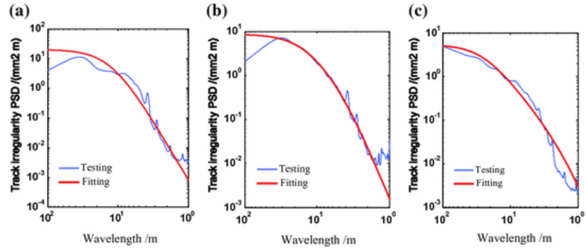
Fig. 5.5 The fitting curve of irregularity power spectrum for ballast track over bridge of Hefei-Wuhan passenger-dedicated line track irregularity of passenger-dedicated line. a Profile irregularity. b Alignment irregularity. c Cross level irregularity
