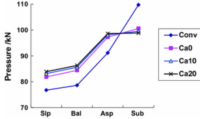
Fig. 3.25 Influence of rubber content C_a with H_a = 20 cm and E_s = 20 MPa on pressures on the track ( Slp sleeper, Bal Ballast, Asp Asphalt, Sub Subgrade, Conv Conventional ballast track with soft subgrade, C_a Rubber content of the asphalt layer )
