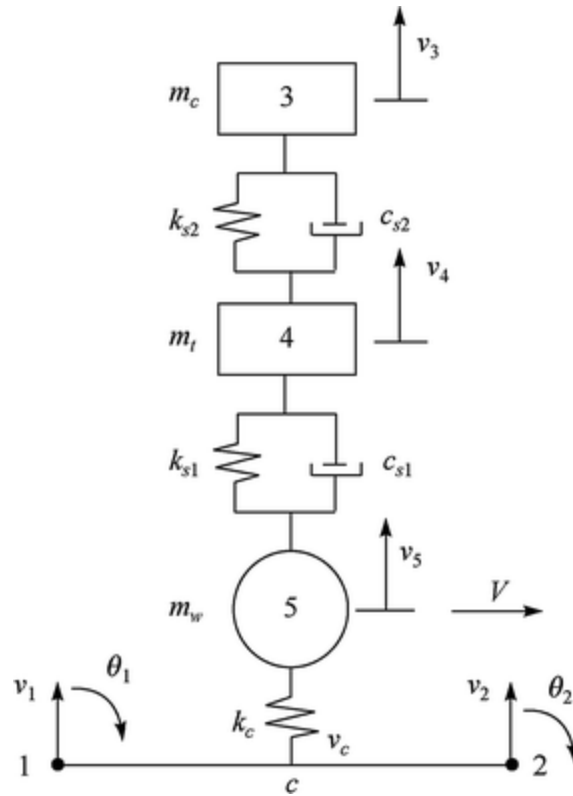
Fig. 8.3 Moving element model of a single wheel with primary and secondary suspension systems
