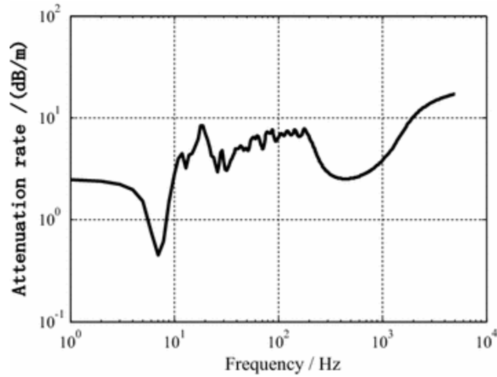
Fig. 4.21 The calculated track vibration attenuation rate
