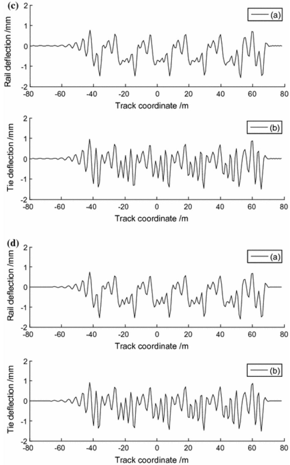
Fig. 3.11 Effect of the rail pad and fastener damping on track vibration (E_s = 2 \times 50 \text{ MN/m}^2; k_p = 2 \times 100 \text{ MN/m}^2; c_s = 2 \times 50 \text{ kN s/m}^2; V = 149 \text{ m/s}) . a
