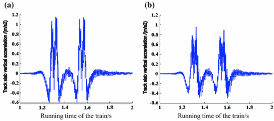
Fig. 13.18 Influence of different CA mortar stiffness on the track slab vertical acceleration. a K_{CA} = 3.0 \times 10^8 \text{ N/m} . b K_{CA} = 3.0 \times 10^9 \text{ N/m}
