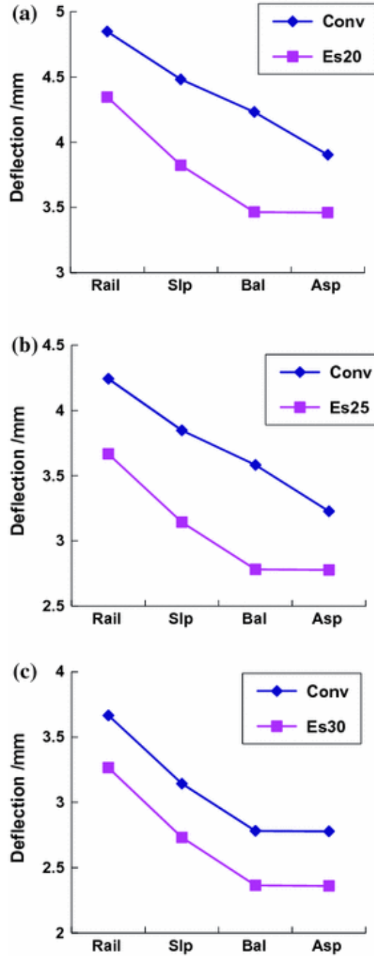
Fig. 3.26 Influence of subgrade module E_s with C_a = 20\% and H_a = 20 cm on deflections of the track ( Slp sleeper, Bal Ballast, Asp Asphalt, Conv Conventional ballast track with soft subgrade, E_s subgrade module). a E_s = 20 MPa. b E_s = 25 MPa. c E_s = 30 MPa
