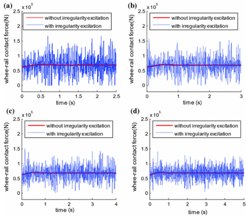
Fig. 7.15 Time history of the wheel-rail contact force with different train speeds in wheel-rail linear contact model. a At the speed of 350 km/h, b at the speed of 300 km/h, c at the speed of 250 km/h, and d at the speed of 200 km/h
