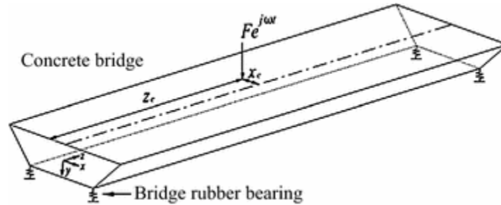
Fig. 4.3 The elevated bridge structure model
