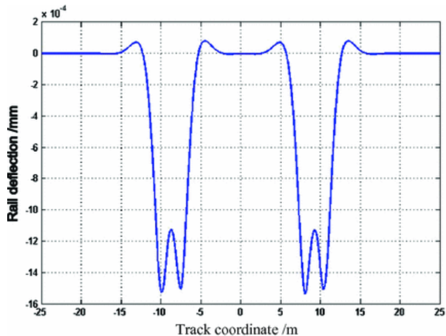
Fig. 9.7 Rail deflection along the track
