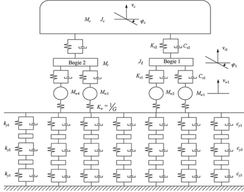
Fig. 7.1 Computation model for the vehicle-track coupling system
