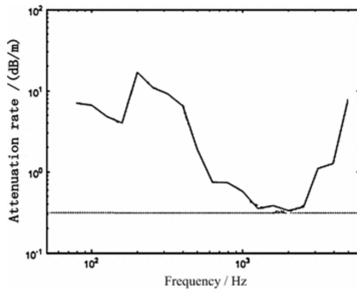
Fig. 4.22 The measured track vibration attenuation rate
