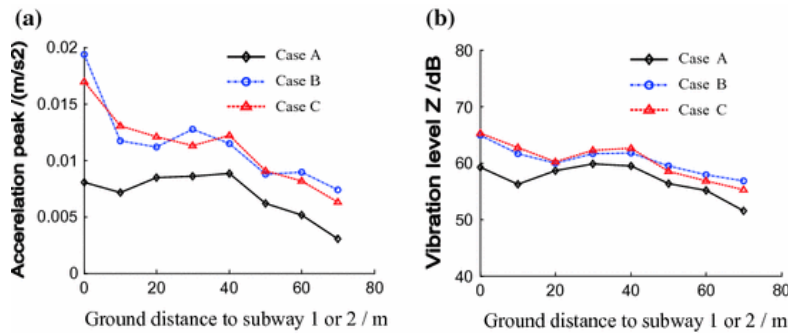
Fig. 15.7 Acceleration peak and vibration level Z attenuate with distance. a Acceleration peak. b Vibration level Z
