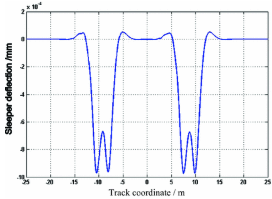
Fig. 9.8 Sleeper deflection along the track
