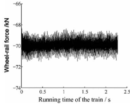
Fig. 7.13 Time history of wheel-rail contact force for convergence precision 1.0 \times 10^{-7}
