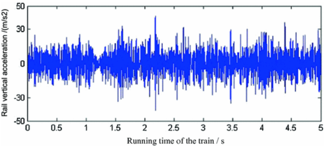
Fig. 10.20 Time history of the rail vertical acceleration
