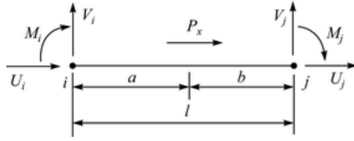
Fig. 6.4 Longitudinal concentrated load on beam element
