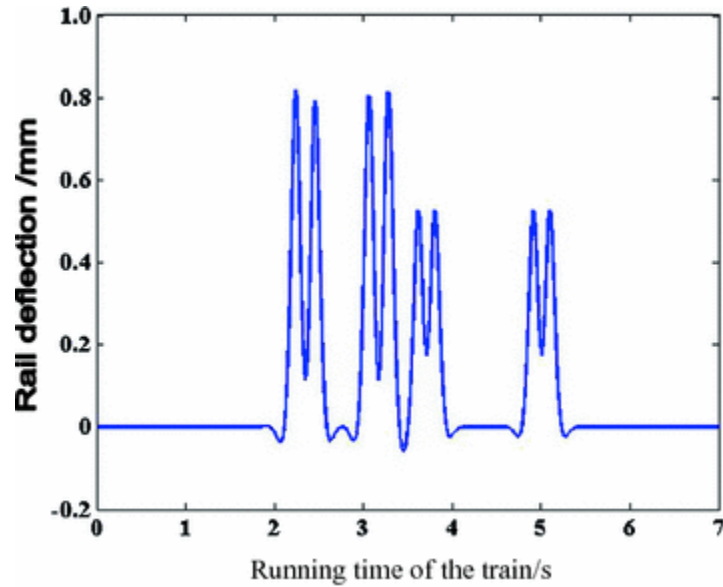
Fig. 13.1 Time history of the rail deflection
