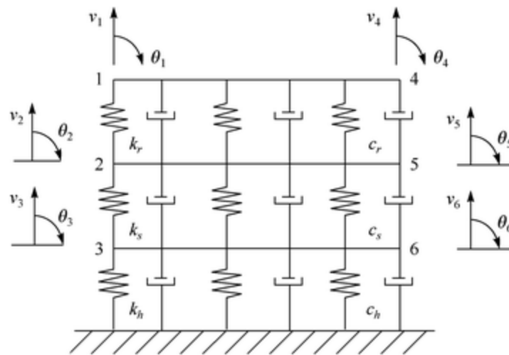
Fig. 10.5 CRTS II slab track element model
