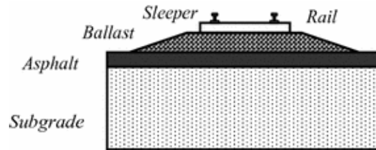
Fig. 3.18 Cross section of the ballast track with asphalt trackbed over soft subgrade
