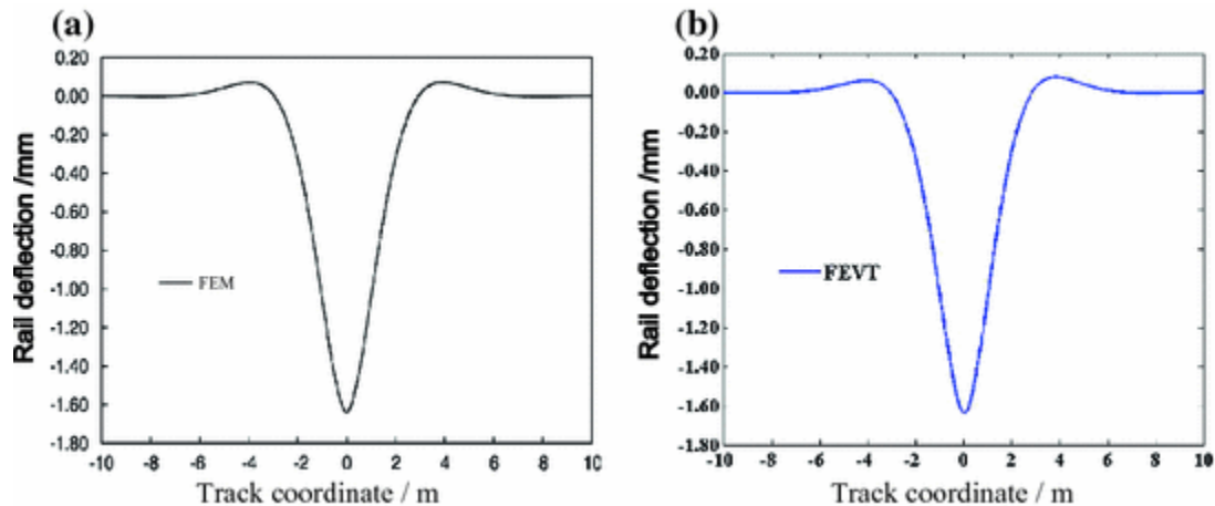
Fig. 9.6 Rail deflection distribution along the track direction. a Calculated result of finite element and b calculated result of the vehicle and track element
