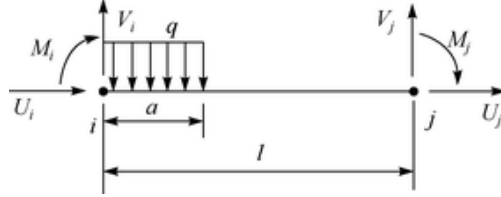
Fig. 6.2 Uniformly distributed load on beam element
