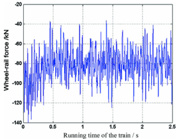
Fig. 9.16 Time history of the wheel-rail contact force
