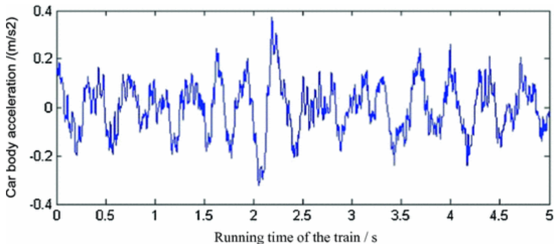
Fig. 10.23 Time history of the car body acceleration
