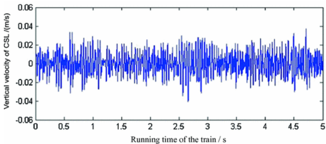
Fig. 10.18 Time history of the track slab vertical velocity
