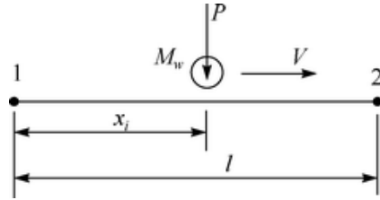
Fig. 6.9 Position of the wheelset on the rail
