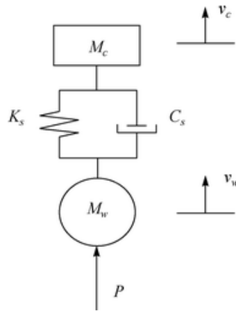
Fig. 6.10 Vehicle model of a single wheel with primary suspension system
