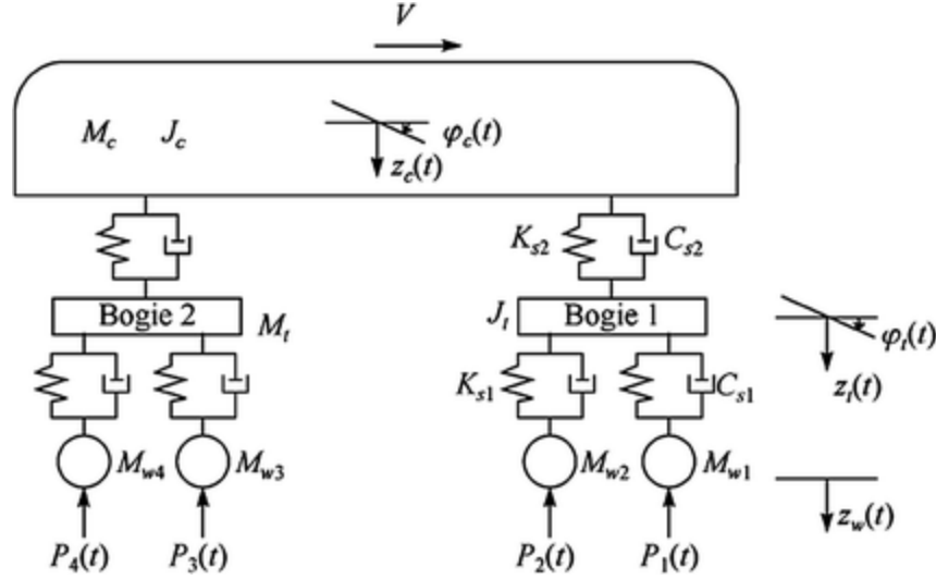
Fig. 11.3 A vehicle model with primary and secondary suspension systems
