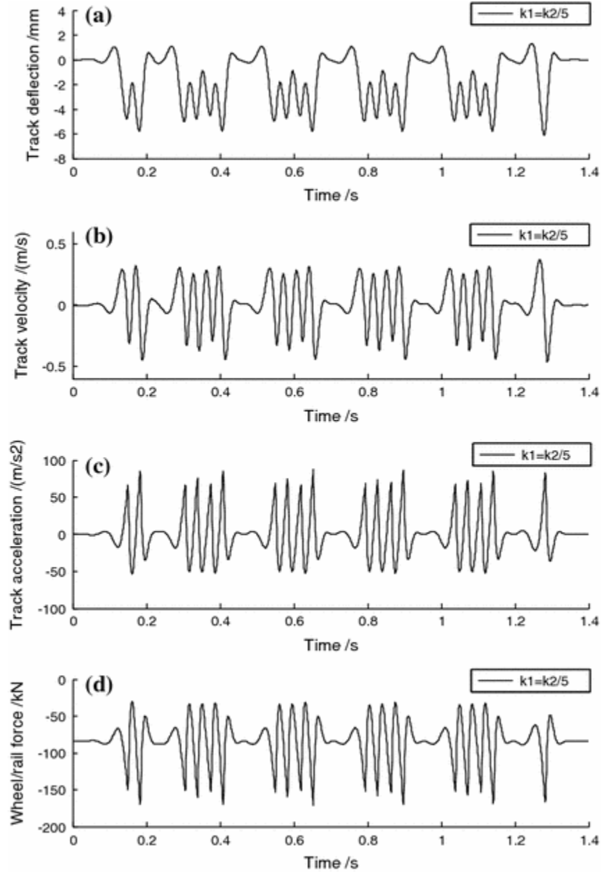
Fig. 2.12 Time history of the track deflection, velocity, and acceleration as well as the wheel-rail force at the point of stiffness abrupt change ( k_1 = k_2/5 , a = 1 mm)
