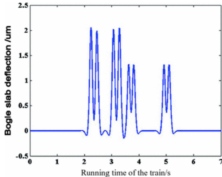
Fig. 13.2 Time history of the Bögle slab deflection
