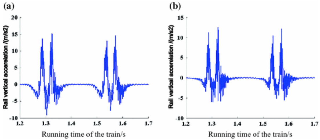
Fig. 13.7 Influence of different rail pad and fastener stiffness on the rail vertical acceleration. a K_p = 2 \times 10^7 N/m. b K_p = 1.2 \times 10^8 N/m
