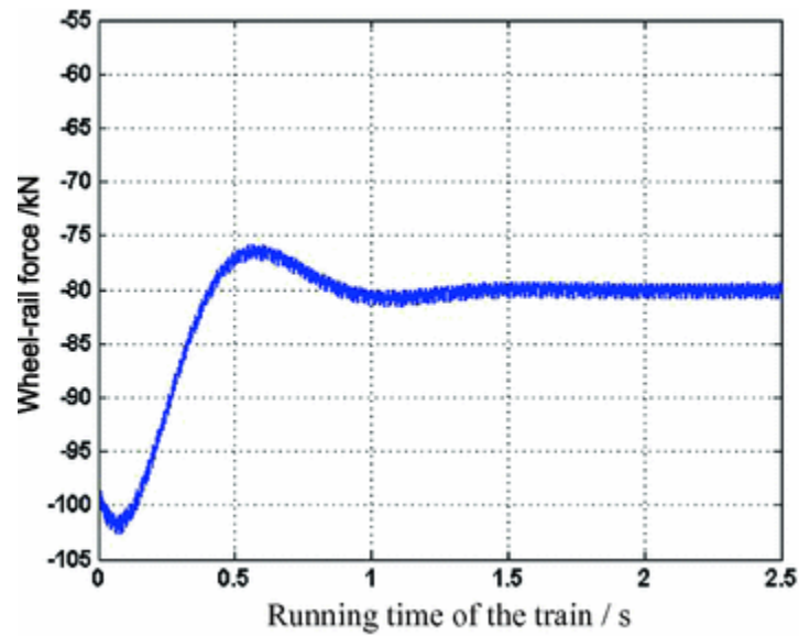
Fig. 9.11 Time history of the wheel-rail contact force
