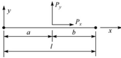
Fig. 6.7 Vertical and longitudinal concentrated forces on rail
