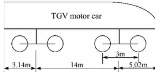
Fig. 6.16 TGV medium- and high-speed motor car
