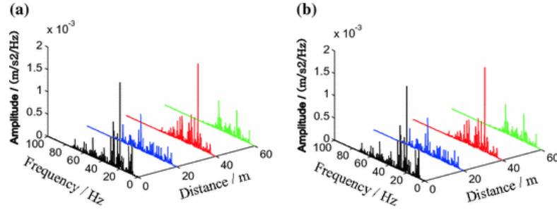
Fig. 15.11 Vibration acceleration amplitude-frequency curves. a Case 3. b Case 6
