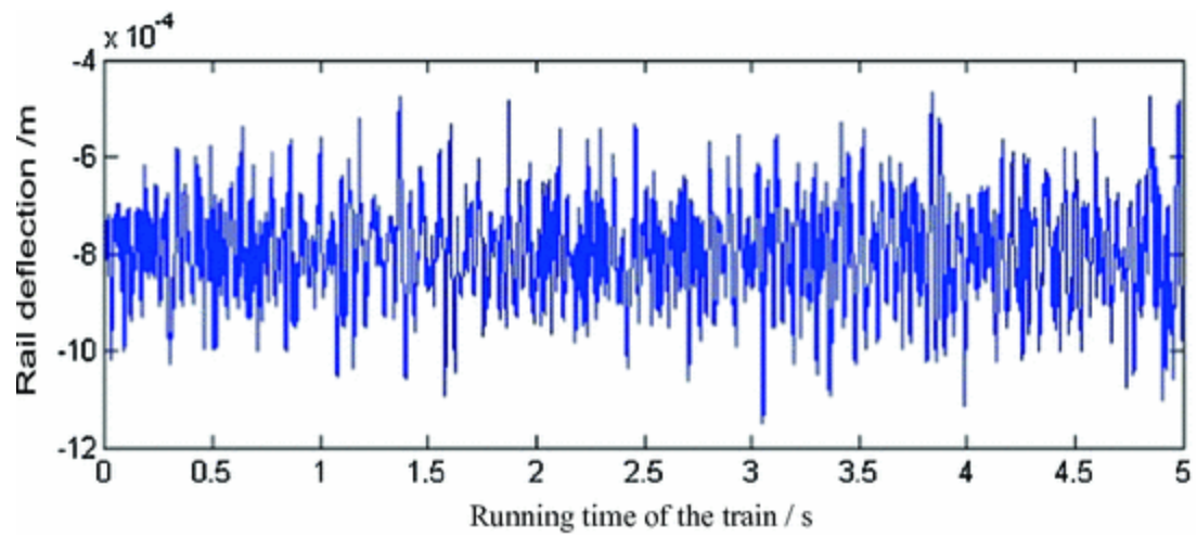
Fig. 10.11 Time history of the rail vertical displacement
