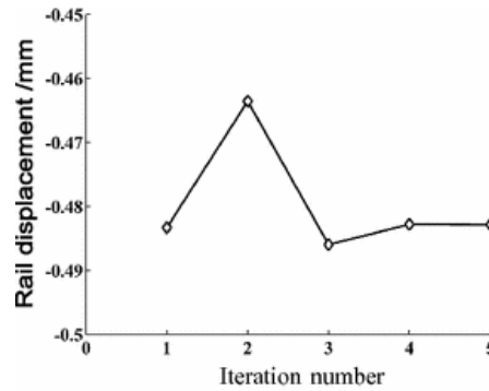
Fig. 7.11 Iteration process for rail displacement at wheel-rail contact point at time t
