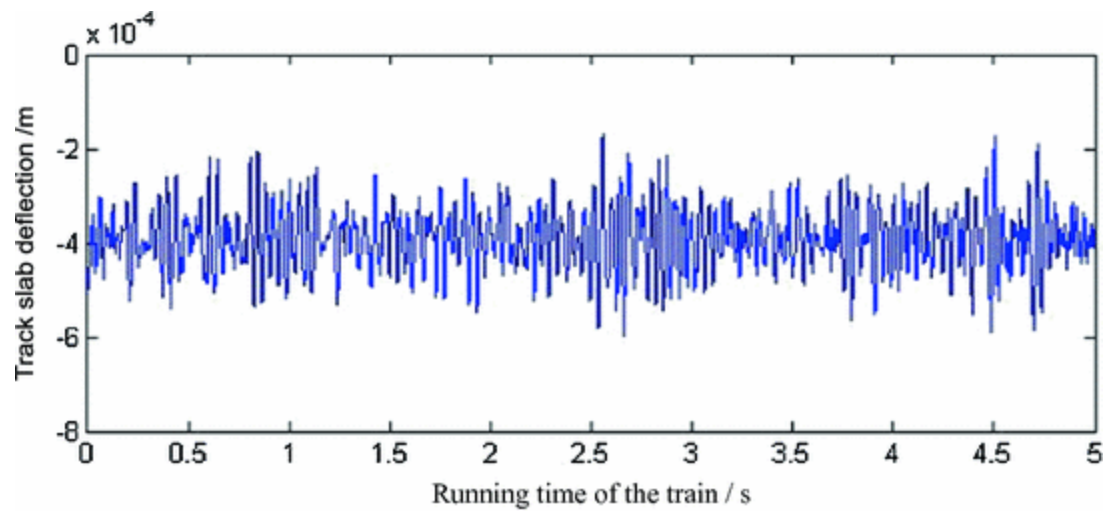
Fig. 10.12 Time history of the slab vertical displacement
