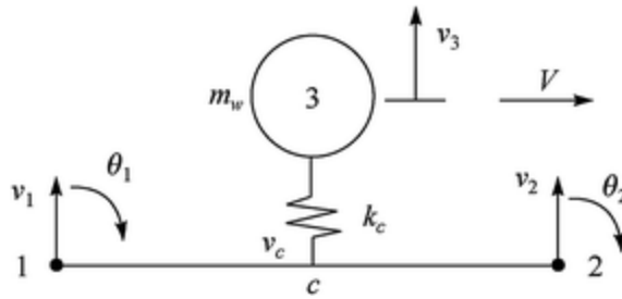
Fig. 8.1 Moving element model
