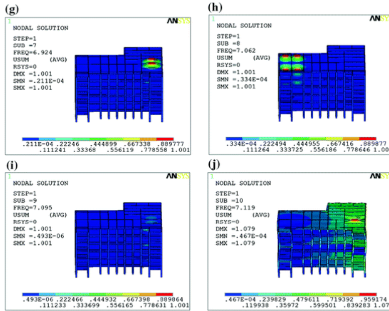
Fig. 15.16 The first 10 vibration mode of the building. a The first order. b The second order. c The third order. d The 4th order. e The 5th order. f The 6th order. g The 7th order. h The 8th order. i The 9th order. j The 10th order
