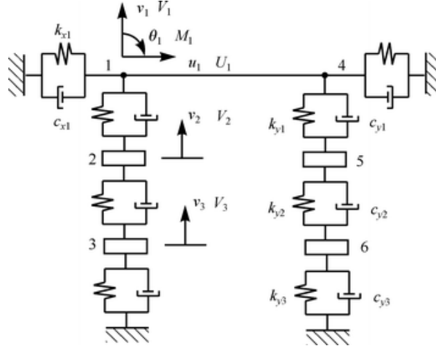
Fig. 6.6 Generalized beam element of track structure
