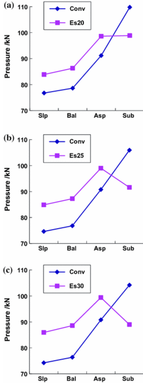
Fig. 3.28 Influence of subgrade module E_s with C_a = 20\% and H_a = 20 cm on pressures on the track (Slp sleeper, Bal Ballast, Asp Asphalt, Sub Subgrade, Conv Conventional ballast track with soft subgrade, E_s subgrade module). a E_s = 20 MPa. b E_s = 25 MPa. c E_s = 30 MPa
