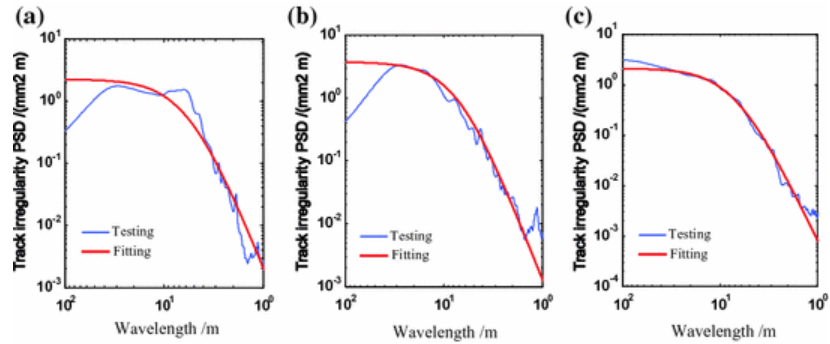
Fig. 5.6 The fitting curve of irregularity power spectrum for ballast track in tunnel of Hefei-Wuhan passenger-dedicated line . a Profile irregularity. b Alignment irregularity. c Cross level irregularity
