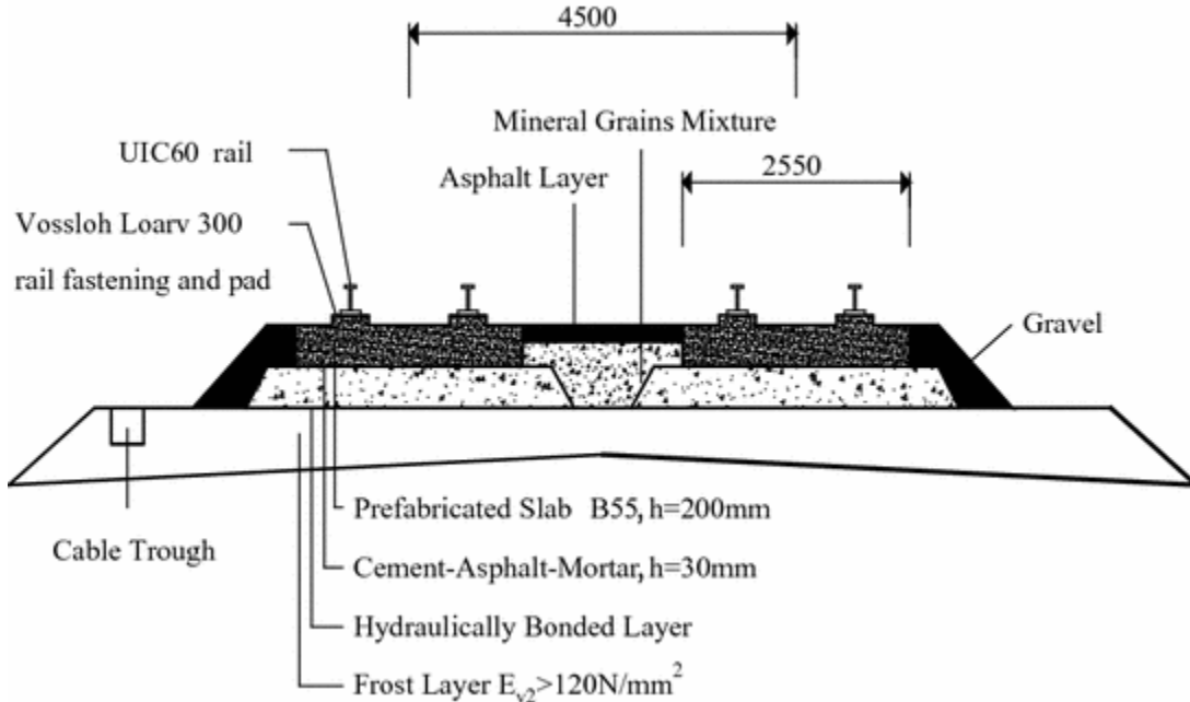
Fig. 10.1 CRTS II slab track
