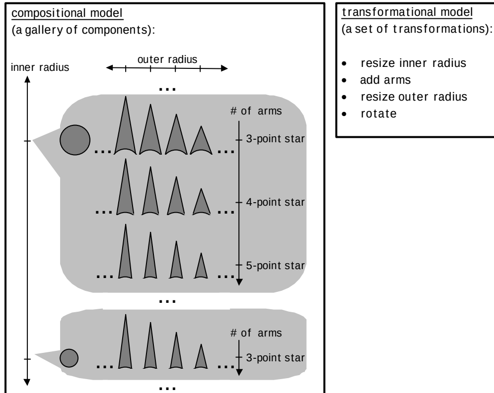
Figure 54 Implementing the domain model of the star concept using the compositional model (on the left) and the transformational model (on the right)
