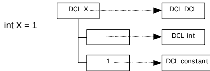
Figure 87 Source tree of int X = 1 ;
