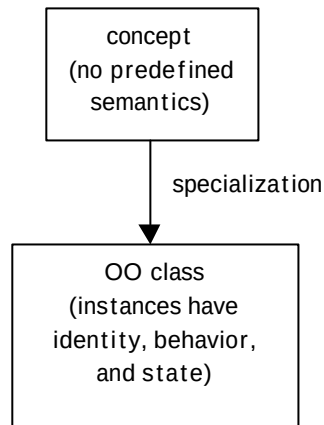
Figure 21 Difference between a concept and an OO class
