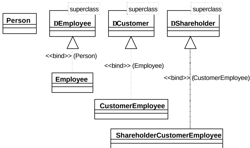
Figure 45 Implementation of an extension point with three or-features using parameterized inheritance (the classes Customer , Shareholder , and ShareholderEmployee and ShareholderCustomer are not shown)
