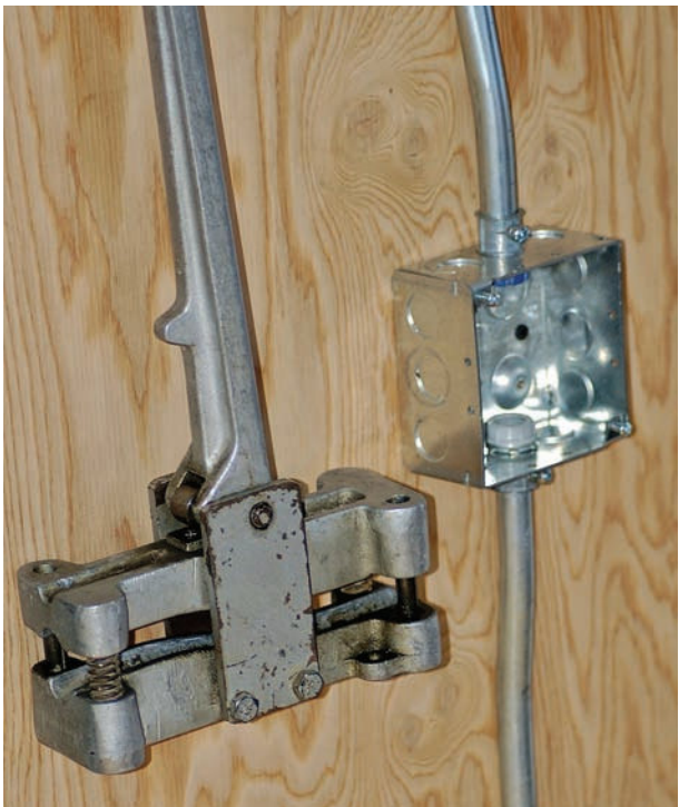
FIGURE 7-10 A 4 × 4 box with an offset bender.
