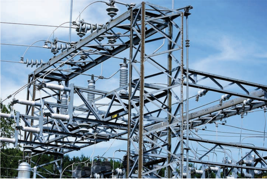
FIGURE 15-2 The substation is the source of local power, and the utility controls all lines that emanate from it.
