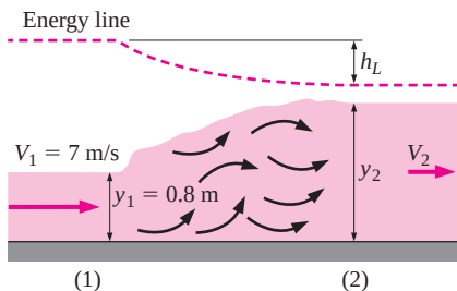
FIGURE 13-35 Schematic for Example 13-7.
