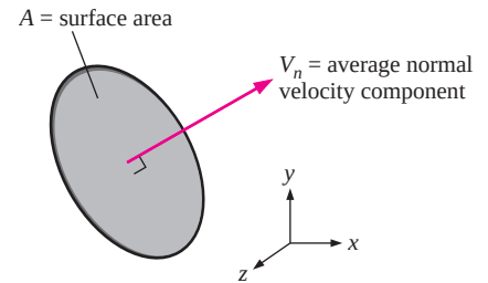
FIGURE 9-4 The mass flow rate through a surface is equal to \rho V_n A .
