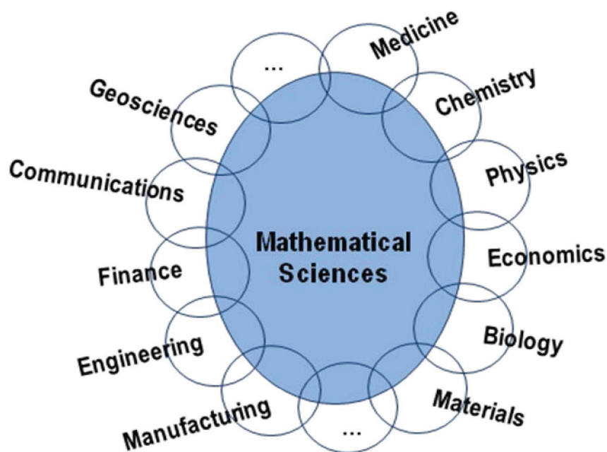
FIGURE 3-1 The mathematical sciences and their interfaces. SOURCE: Adapted from National Science Foundation, 1998, Report of the Senior Assessment Panel for the International Assessment of the U.S. Mathematical Sciences , NSF, Arlington, Va.
