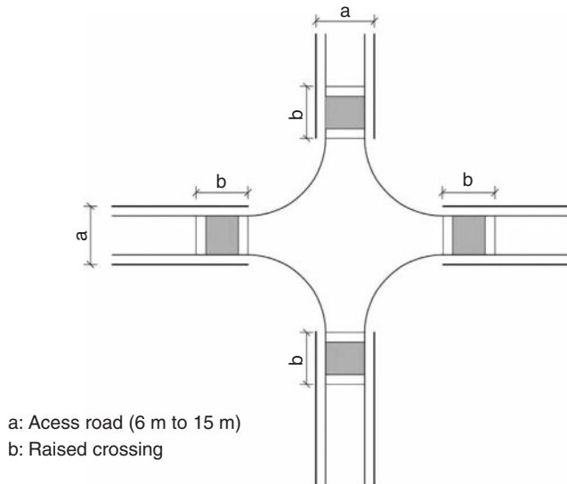
Figure 18.2 Example of unsignalized junctions.
