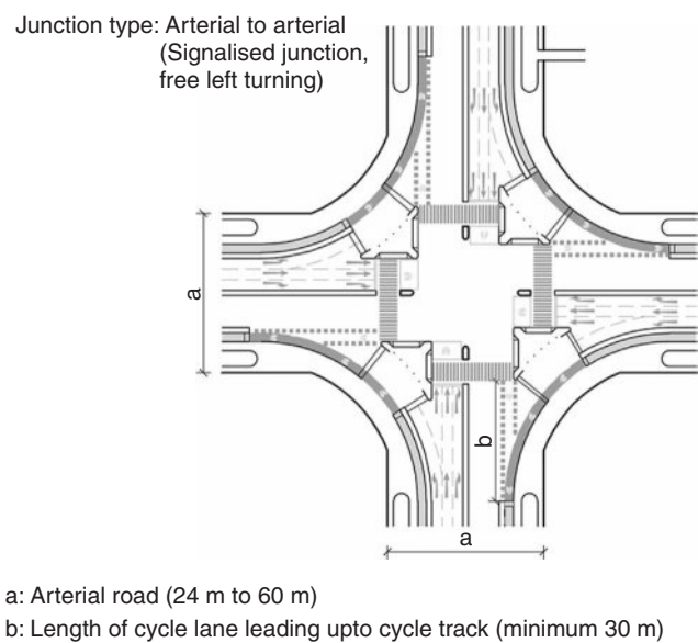
Figure 18.3 Example of Signalized junctions.
