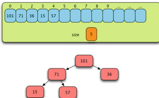
Fig. 9.12 Just Before Phase II
