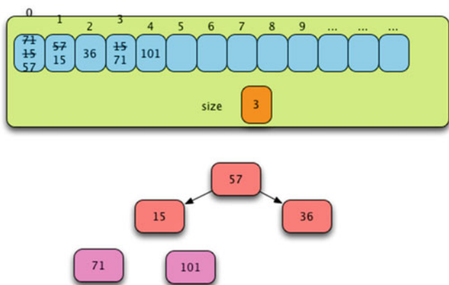
Fig.9.15 After the Second Pass of Phase II
