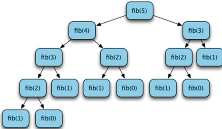
Fig. 5.7 Computing fib(5)
