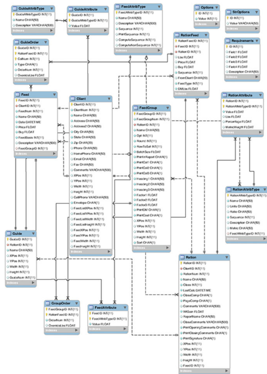
Fig. 11.1 Dairy Database Entity Relationship Diagram
