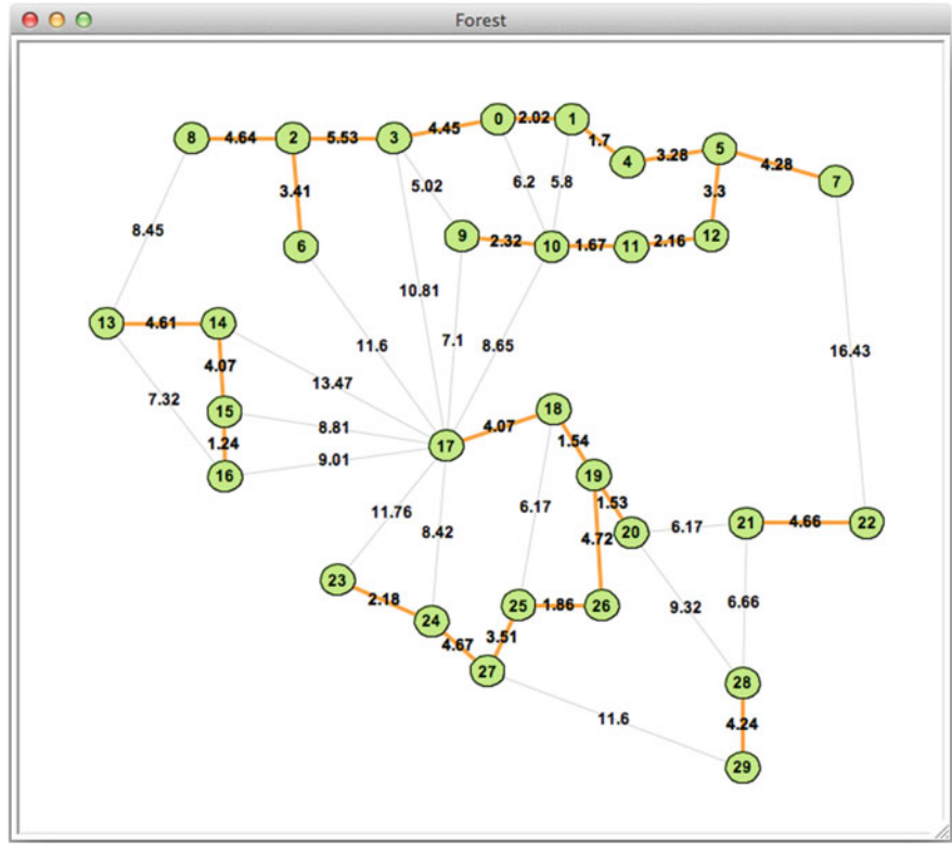
Fig. 7.7 Kruskal's: Snapshot 2
