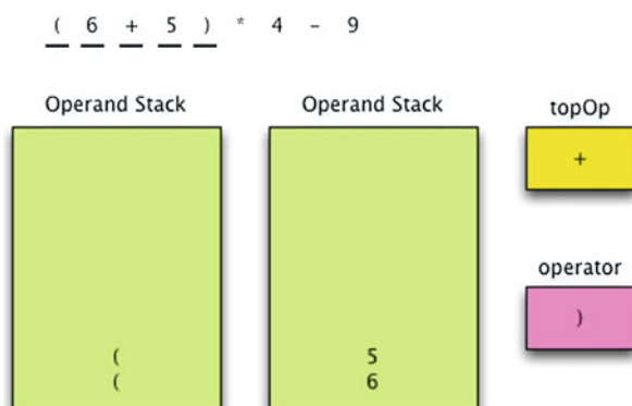
Fig.4.15 Infix Evaluation Step 1
