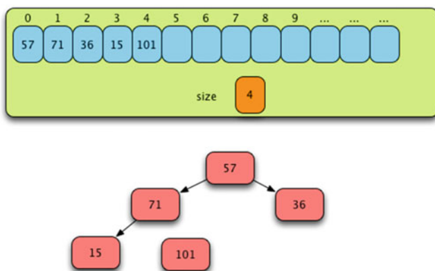
Fig. 9.13 After Swapping First and Last Values
