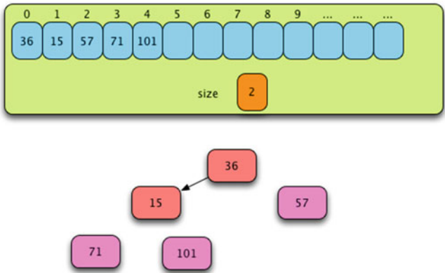
Fig. 9.16 After the Third Pass of Phase II
