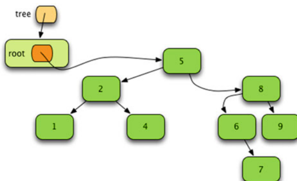
Fig. 6.12 The Final BinarySearchTree Object Contents
