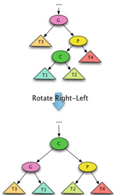
Fig. 10.11 Splay Tree Double-Left Rotate
