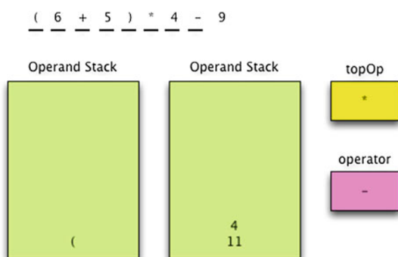
Fig.4.16 Infix Evaluation Step 2
