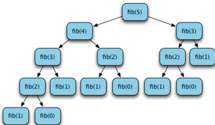
Fig. 6.1 The Call Tree for Computing \text{fib}(5)
