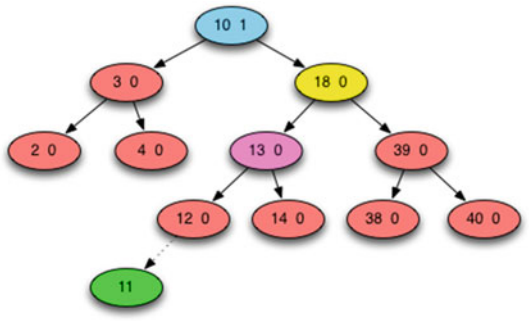
Fig. 10.4 AVL Tree Case 3B—Double Rotation
