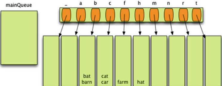
Fig.4.25 Radix Sort Step 8—1st letter
