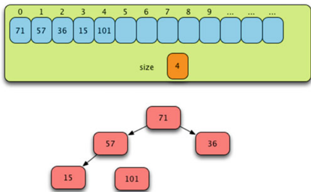
Fig.9.14 After the First Pass of Phase II
