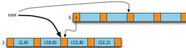
Fig. 11.16 After Deleting the Item Containing 18
