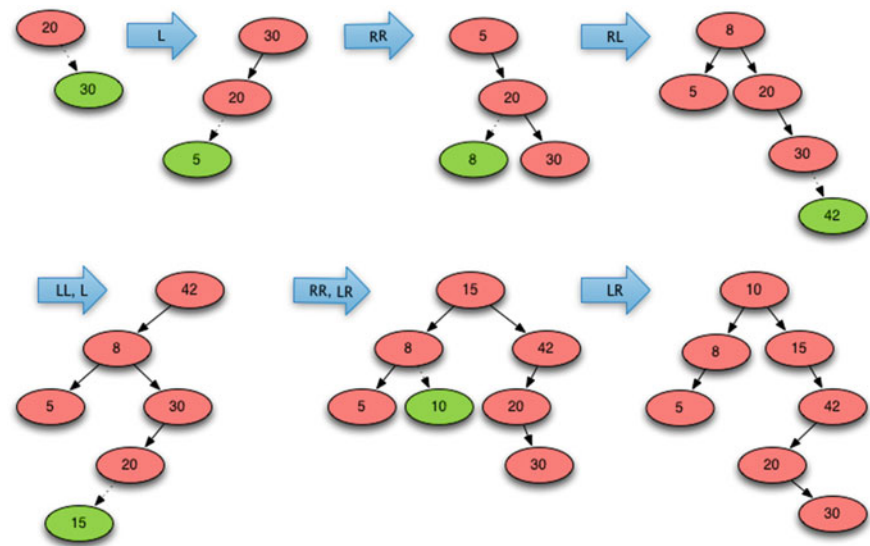
Fig. 10.14 Splay Tree Example
