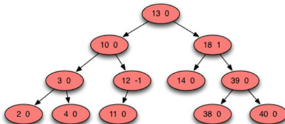
Fig. 10.6 AVL Tree Case 3B Step 2 Rotate Away
