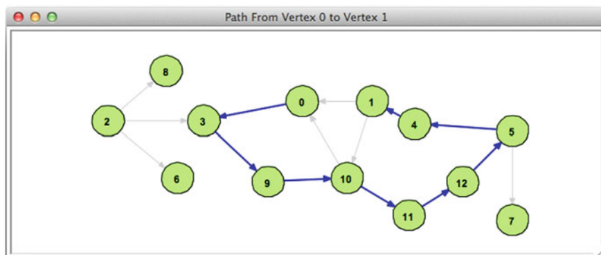
Fig. 7.4 A Path from Vertex 0 to Vertex 1
