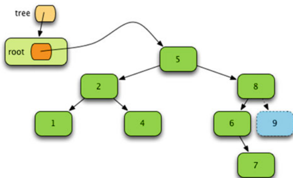
Fig. 6.13 The Tree After Deleting 9
