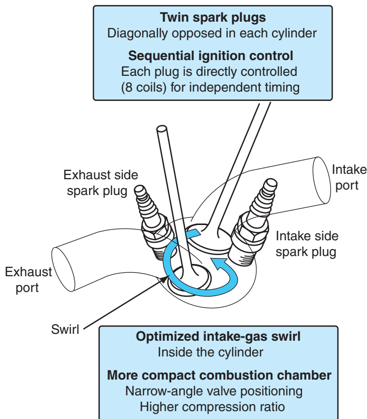
Figure 7-24 The intelligent-Dual & Sequential Ignition (i-DSI) system has eight ignition coils, eight spark plugs that can fire sequentially or simultaneously, and is totally controlled by the PCM.
