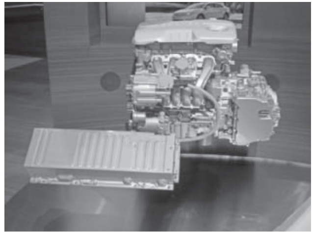
Figure 7-8 The main components of a GM eAssist system.
