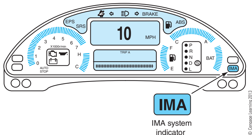
Figure 10-38 When the IMA warning lamp remains lit after the engine is started, the control system has detected a problem.
