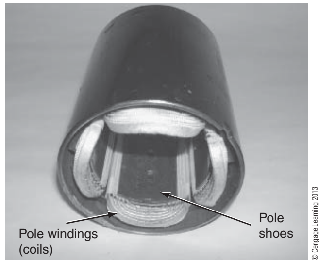
Figure 3-10 The field (pole) windings are secured to the inside of the motor's housing.
