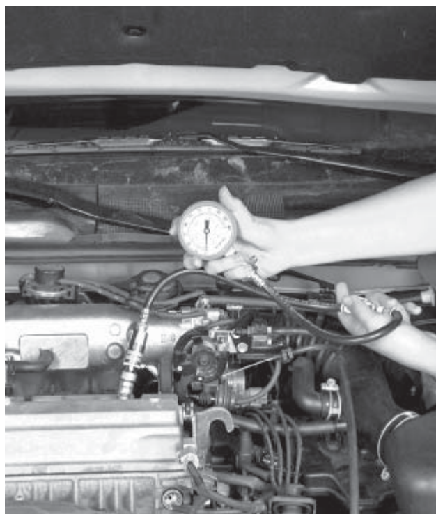
Figure 10-39 A compression tester connected to a cylinder.
