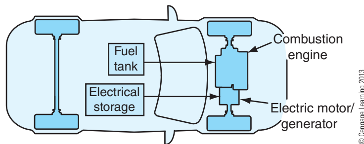
Figure 1-11 The motor/generators drive the wheels and absorb the vehicle's kinetic energy during slow-down and braking.
