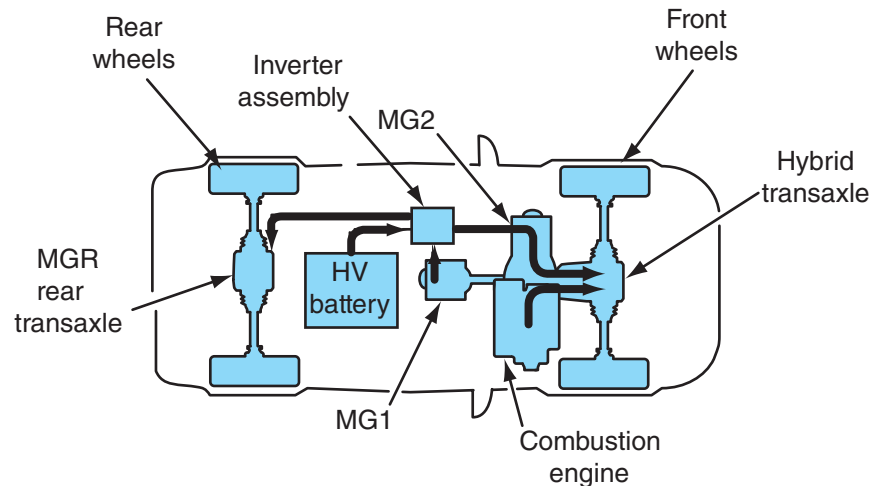
Figure 8-36 During full-throttle acceleration, the vehicle is powered by the engine, MG2, and MGR. Electrical power for MG2 and MGR comes from the battery pack and MG1.
