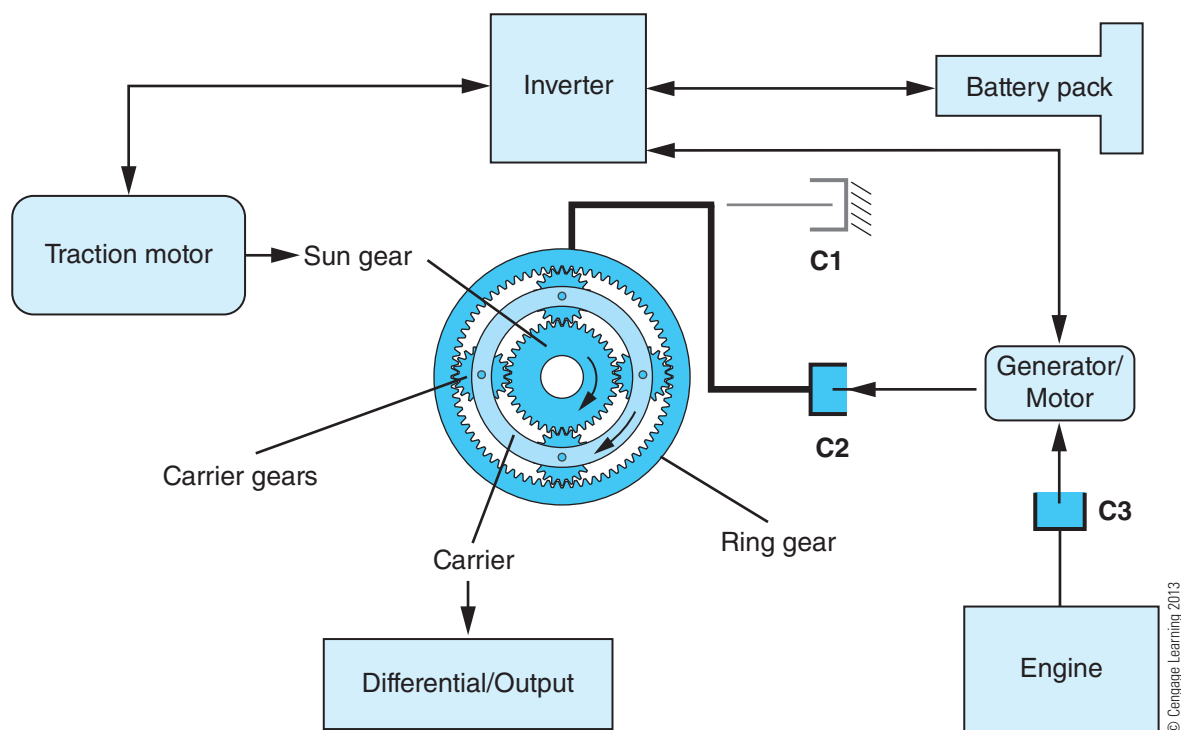
Figure 6-35 Power flow while the Volt is operating in the Extended Range, Charge Sustaining, High-Speed, Two Motors mode.
