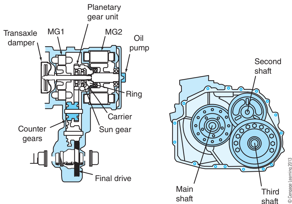
Figure 10-48 A compound gear set-equipped Toyota transaxle.
