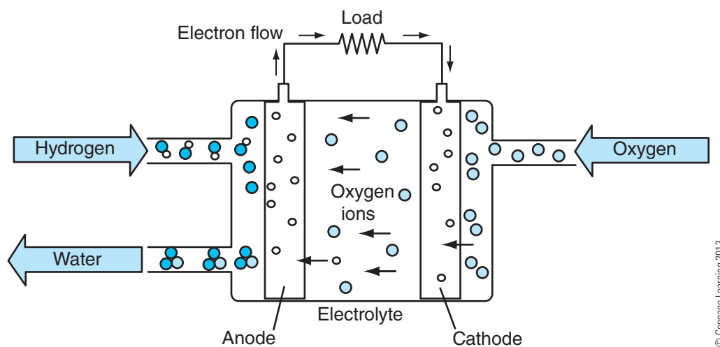
Figure 11-7 A solid oxide fuel cell (SOFC).
