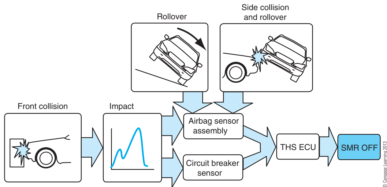
Figure 10-18 Through the use of sensors, high-voltage systems are shut down when a collision is detected.
