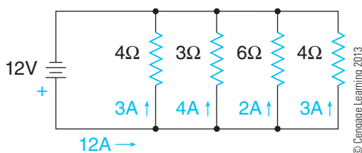
Figure 2-12 The characteristics of a parallel circuit.
