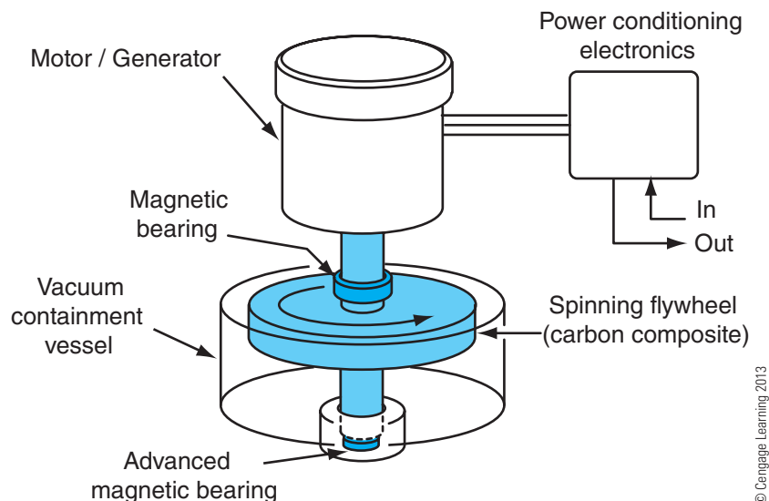
Figure 5-6 Basic construction of a flywheel energy storage system.
