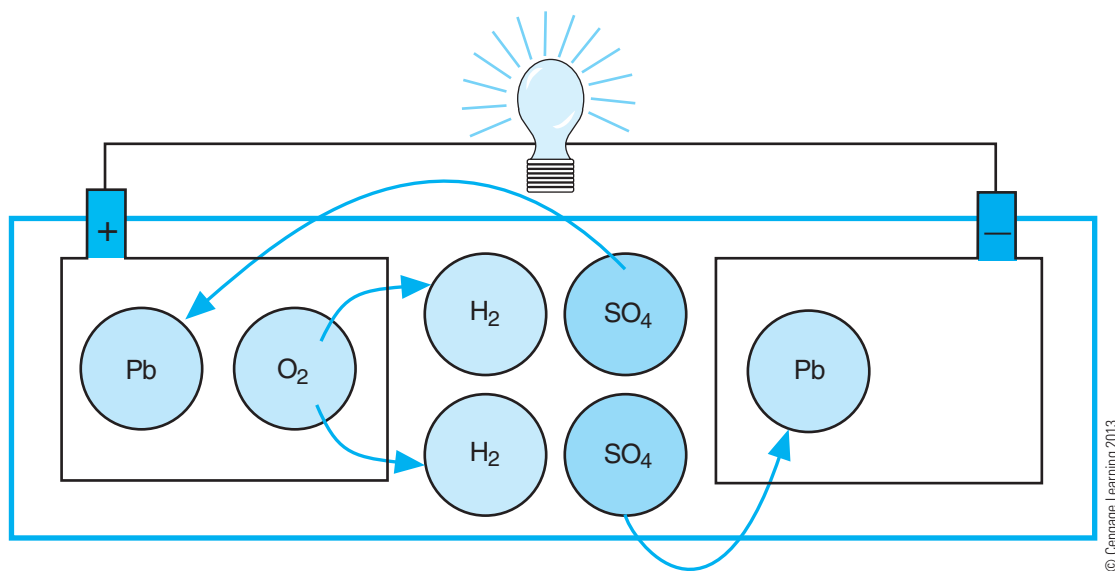
Figure 4-23 The chemical reaction during discharge of a lead-acid battery.
