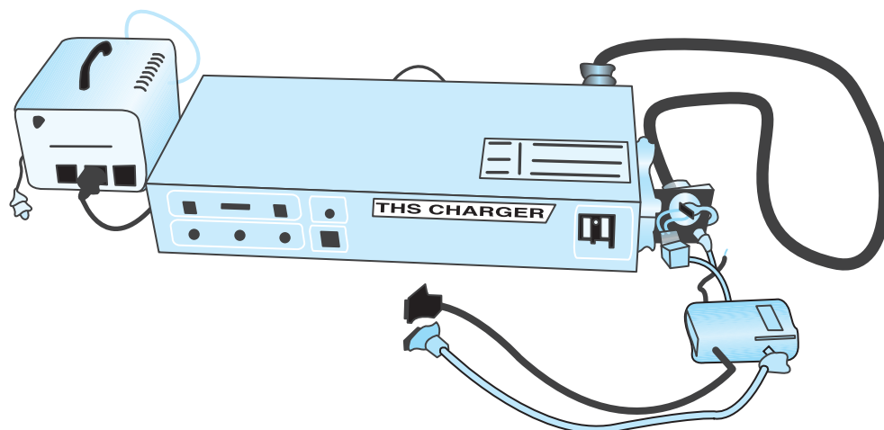
Figure 10-27 The high-voltage battery charger for Toyota hybrids. There are two output cables, one for the battery pack and the other to operate the 12V system for the battery-cooling fans and computer.
