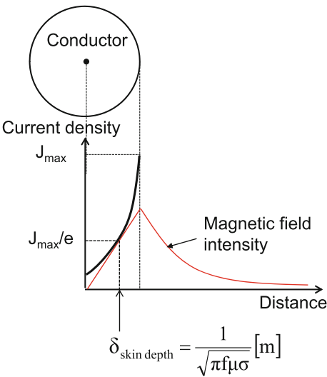
Fig. 5.8 Cutaway view of magnetic field within a round conductor
