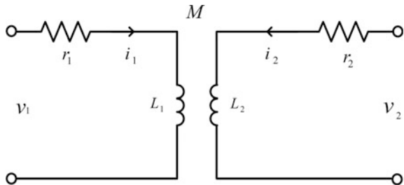
Fig. 7.4 Equivalent circuit model of wireless power transfer system
