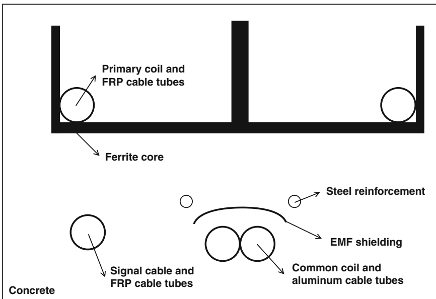
Fig. 6.2 Front view of power supply cable module
