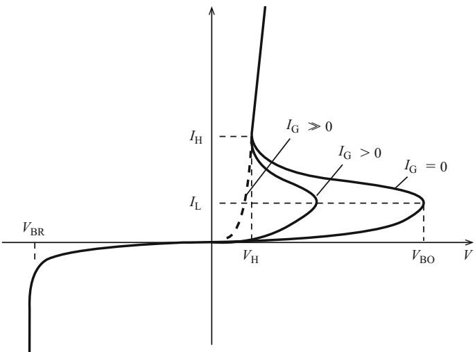
Fig. 8.6 Voltage–current characteristics of thyristor [4]
