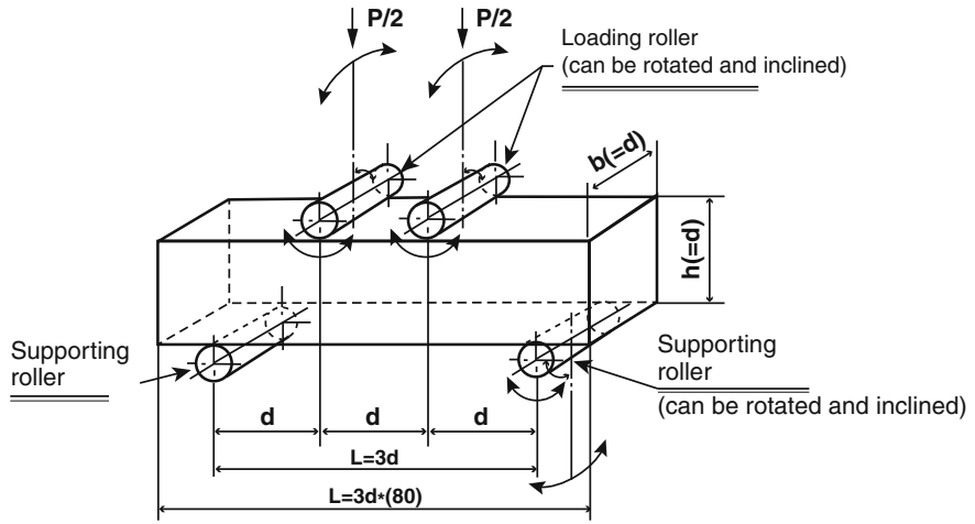
Fig. 23.6 Example of trisection point load device
