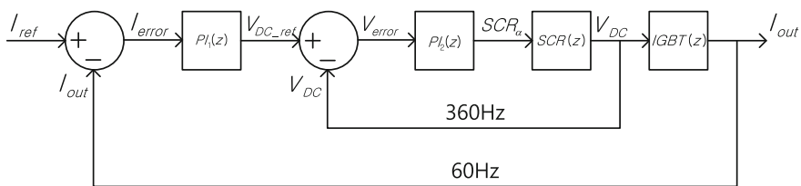
Fig. 10.4 Control algorithm block diagram
