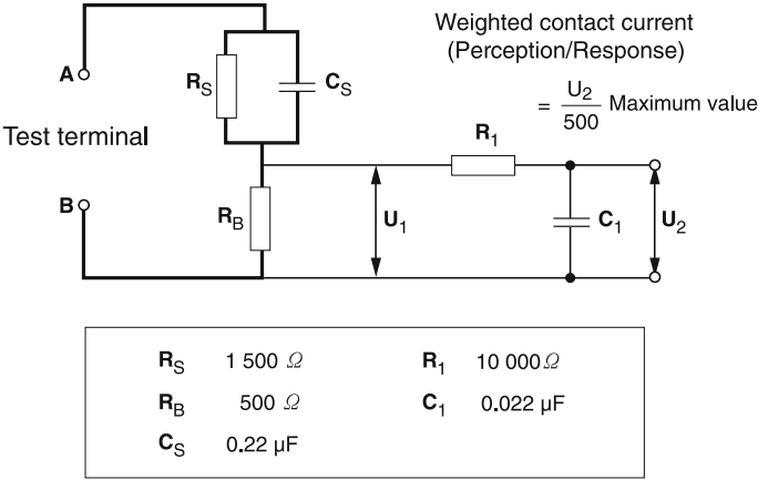
Fig. 23.2 Leakage current test
