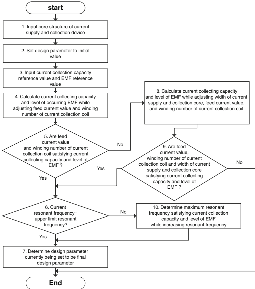
Fig. 4.8 Flow chart of optimal design method for power transfer system using a magnetic resonance scheme
