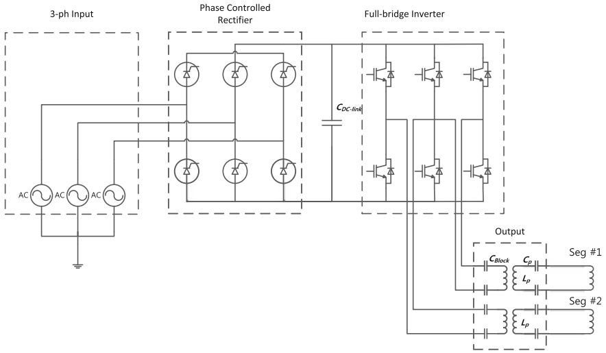
Fig. 10.3 Power circuit of OLEV infrastructure system
