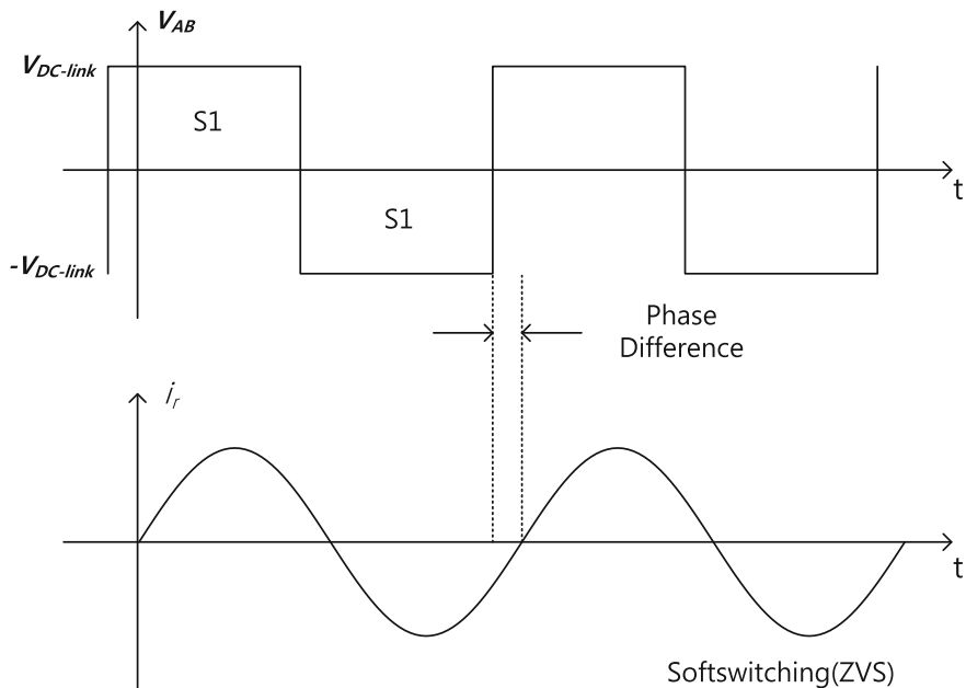
Fig. 10.5 Steady-state inverter switching
