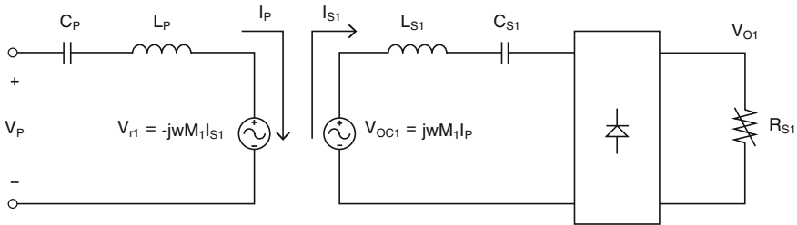
Fig. 12.5 Series-series resonance circuit
