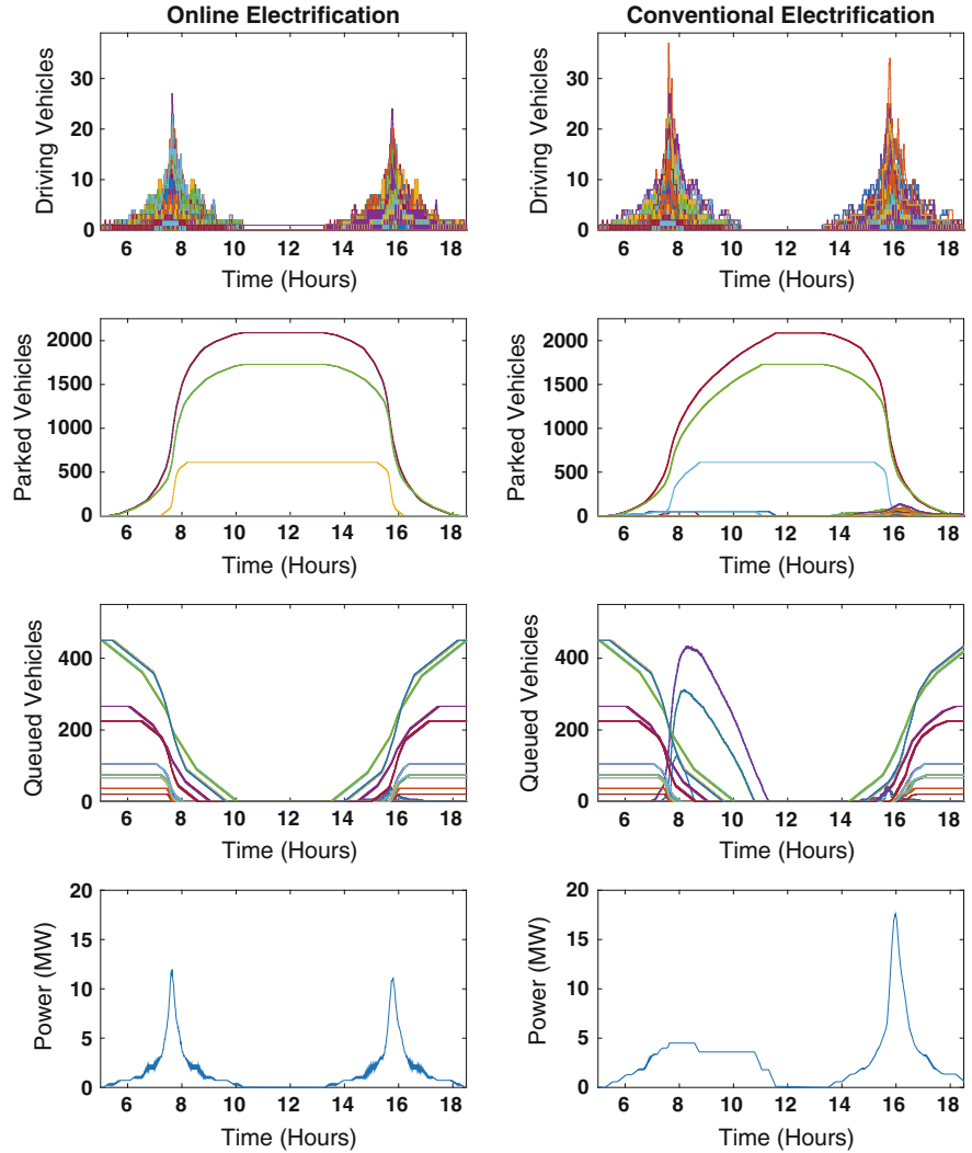
Fig. 20.2 Simulation results of the Symmetrica test case for online and conventional transportation-electrification
