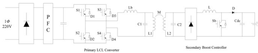
Fig. 18.3 Topology of wireless power transfer system for electric carrier application
