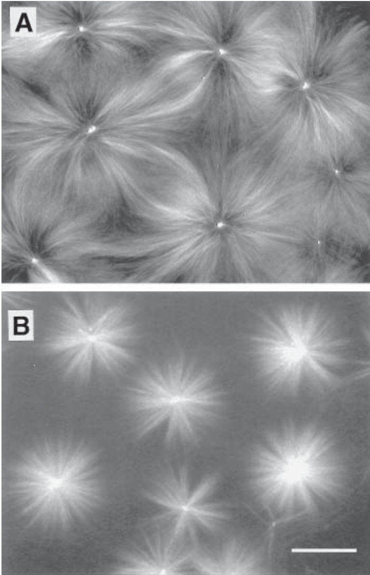
Fig. 2. Microtubule asters organized by kinesin complexes (A) and by NCD complexes (B). In these two cases, self-organization of microtubules and motors produce asters. However, because the two motor proteins have opposite directionality the asters formed have opposite polarity (manuscript in preparation). In asters organized by kinesin complexes, the plus end of the microtubules is in the center, whereas organization of microtubules by NCD complexes produces asters with minus ends in the center. The images are taken in dark field. Scale bar: 50 \mu\text{m} .
