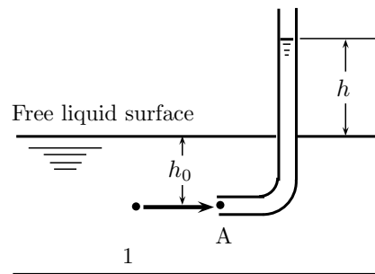
Figure 6.39 | Simple pitot tube.
