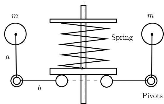
Figure 3.60 | Hartnell governor.
