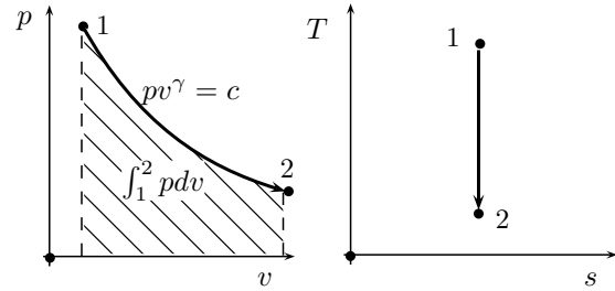
Figure 8.42 | Adiabatic process.
