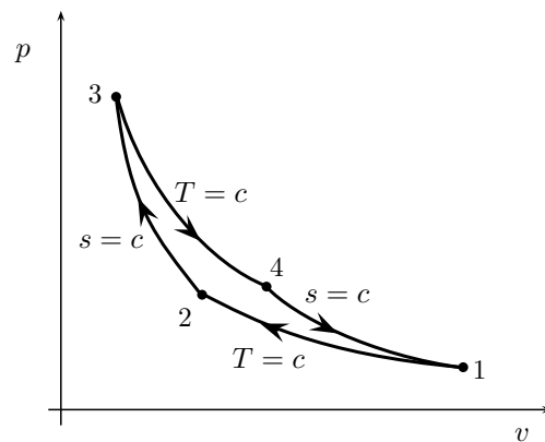
Figure 8.21 | Carnot cycle.
