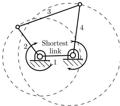
Figure 3.6 | Drag-link mechanism.
