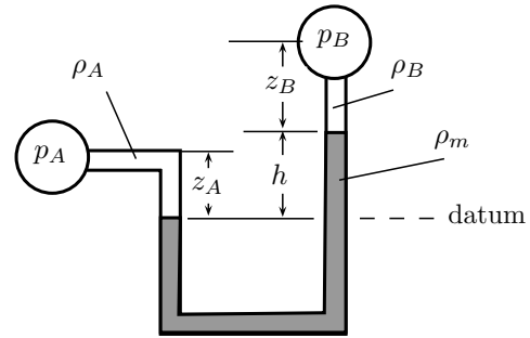
Figure 6.14 | Manometer.
