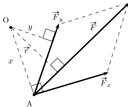
Figure 1.3 | Varignon's theorem.
