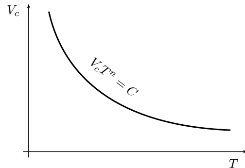
Figure 14.10 | Tool life versus cutting velocity.
