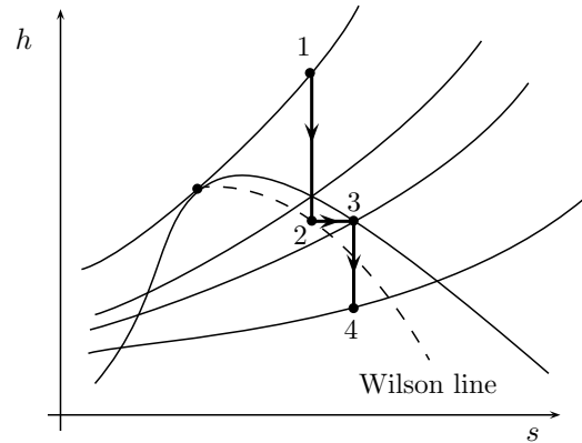
Figure 9.14 | Saturated flow.
