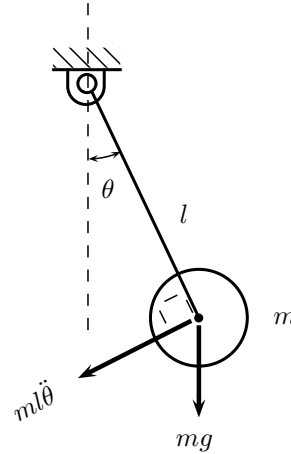
Figure 4.12 | Pendulum.
