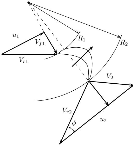
Figure 9.66 | Velocity diagram.
