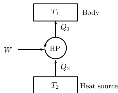
Figure 8.20 | Cyclic heat pump.
