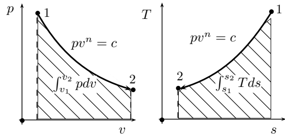
Figure 8.38 | Polytropic process.
