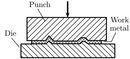
Figure 12.12 | Embossing.
