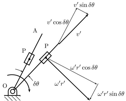
Figure 3.23 | Coriolis component.
