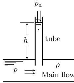
Figure 6.13 | Piezometer.
