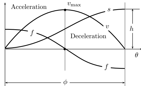
Figure 3.27 | Simple harmonics.
