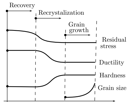
Figure 10.8 | Grain boundary modification.
