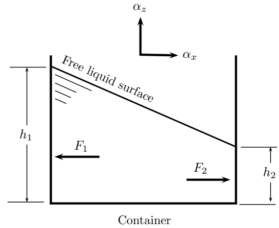
Figure 6.21 | Linear acceleration.
