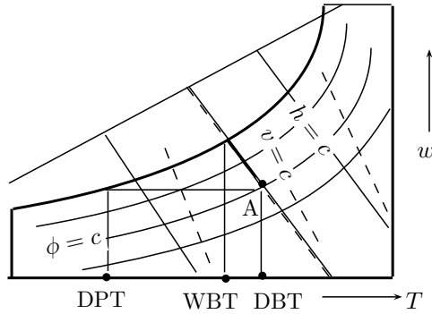
Figure 9.53 | Psychrometric chart.
