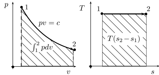
Figure 8.41 | Isothermal process.
