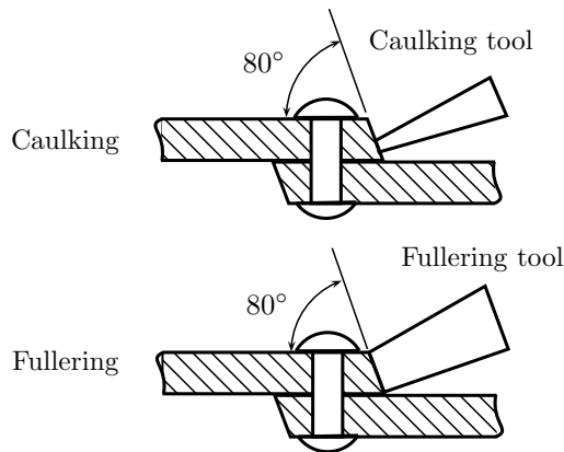
Figure 5.14 | Caulking and fullering.
