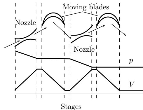
Figure 9.26 | Pressure compounded stages.
