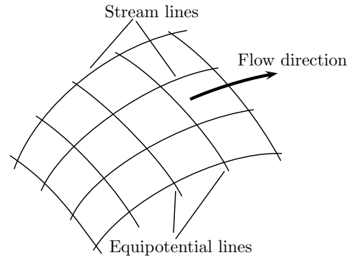
Figure 6.29 | Flow net.
