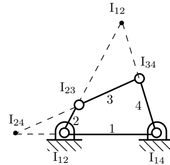
Figure 3.20 | Four-bar mechanisms.
