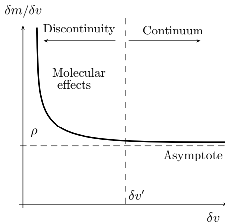
Figure 8.1 | Concept of continuum.
