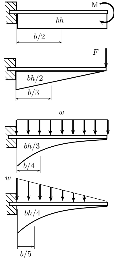
Figure 2.32 | Moment diagram by parts.
