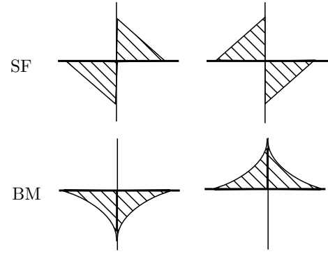
Figure 2.18 | Relationship between SF and BM.
