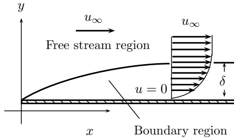
Figure 6.45 | Boundary layer.
