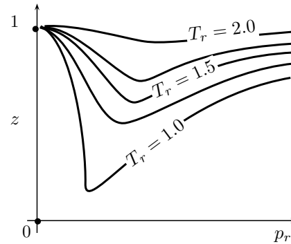
Figure 8.35 | Reduced compressibility factor.
