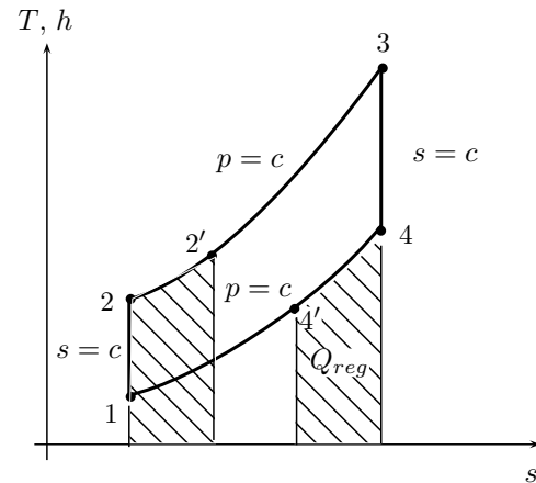
Figure 8.51 | Regeneration on T - s plane.
