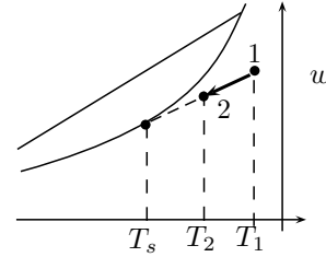
Figure 9.55 | By-pass factor.
