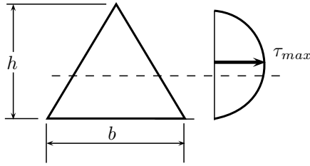
Figure 2.28 | Shear stress in triangular section.
