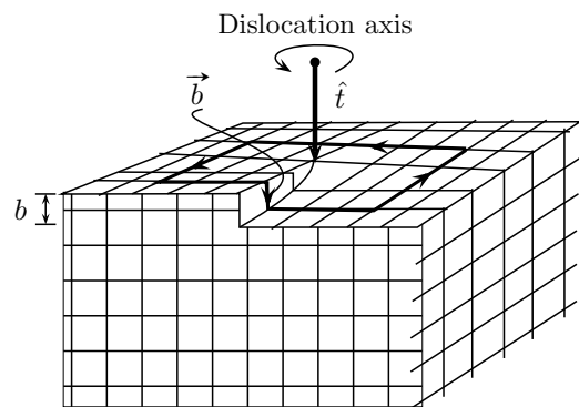
Figure 10.7 | Screw dislocation.
