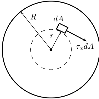
Figure 2.34 | Torsion of shaft.
