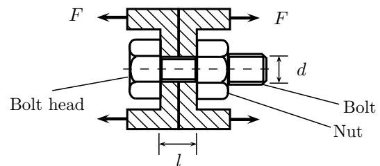
Figure 5.24 | Elastic analysis of bolted joints.
