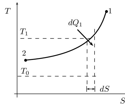
Figure 8.32 | Work on T-S diagram.
