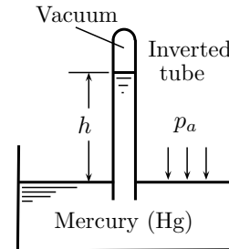
Figure 6.12 | Barometer.
