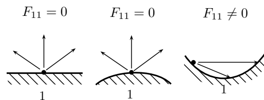
Figure 7.20 | Shape factors.
