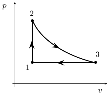
Figure 9.39 | Lenoir cycle.
