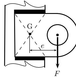
Figure 5.20 | Eccentrically loaded welds.
