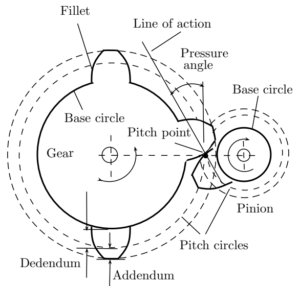
Figure 3.31 | Gear terminology.
