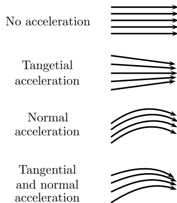
Figure 6.25 | Stream lines and acceleration.
