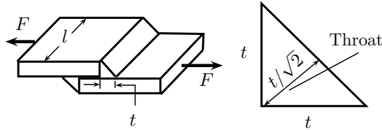
Figure 5.19 | Fillet weld.
