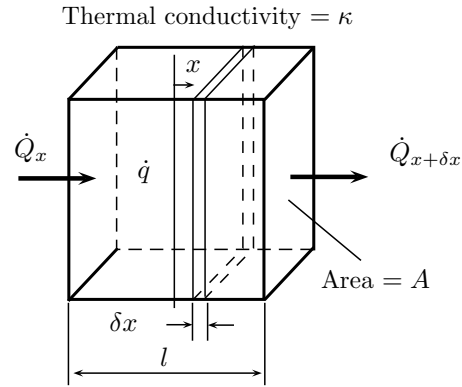
Figure 7.7 | Conduction with heat generation.
