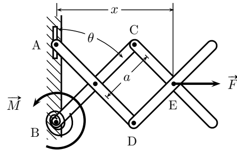
Figure 1.21 | Lazy tong mechanism.
