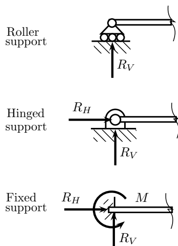
Figure 2.16 | Support reactions.
