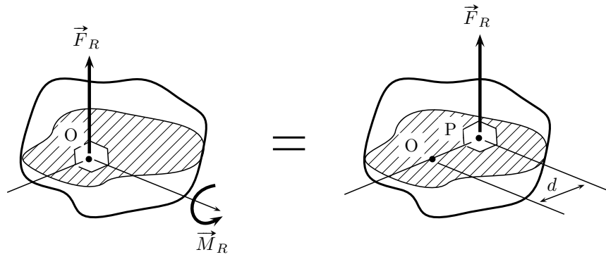
Figure 1.6 | Single resultant force.
