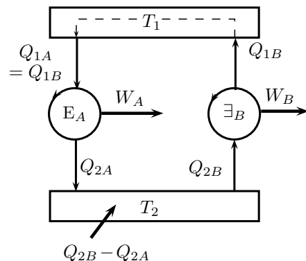
Figure 8.23 | Engine E_A and heat pump \exists_B .
