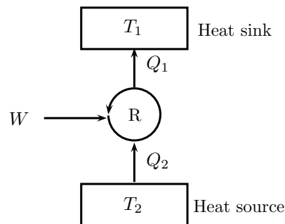
Figure 8.19 | Cyclic refrigerator.
