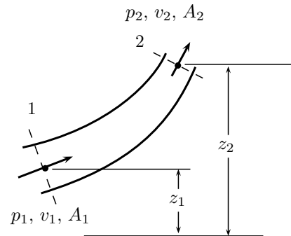
Figure 6.33 | Bernoulli's equation.
