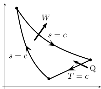
Figure 8.25 | Impossible cycle.
