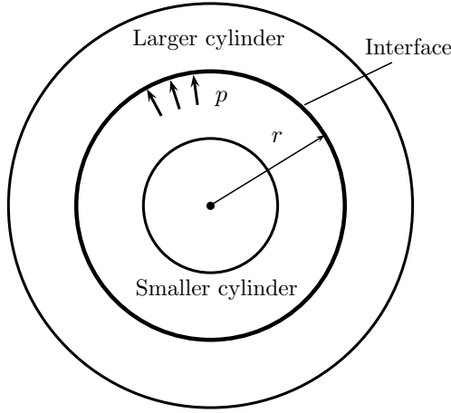
Figure 2.42 | Compound cylinder.
