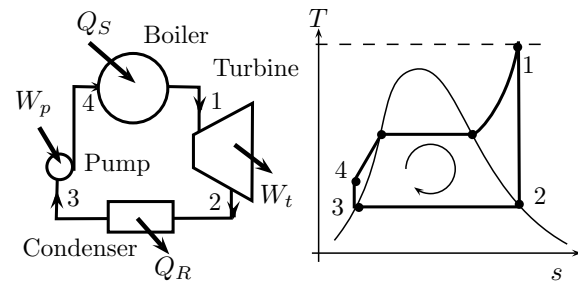
Figure 9.15 | Rankine cycle.
