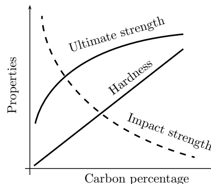
Figure 10.18 | Effect of carbon on steels.
