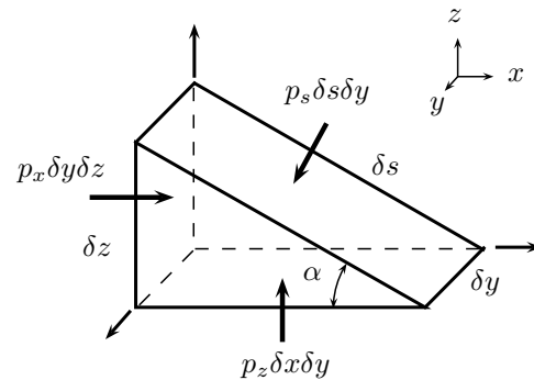
Figure 6.10 | Pascal's law.
