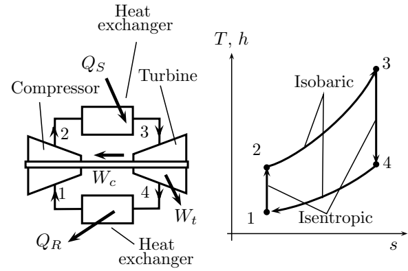
Figure 8.47 | Brayton cycle.
