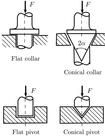
Figure 3.56 | Flat and conical pivots.
