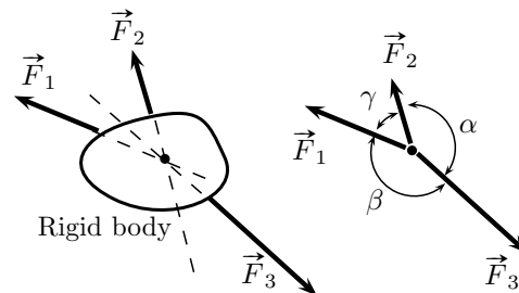
Figure 1.10 | Lami's theorem.
