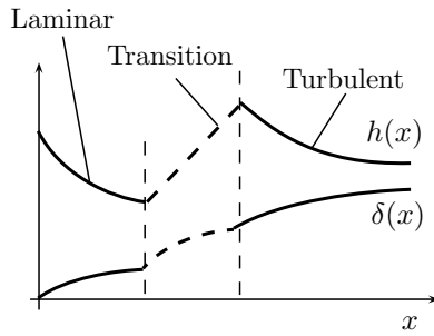
Figure 7.14 | Variation of \delta and h .
