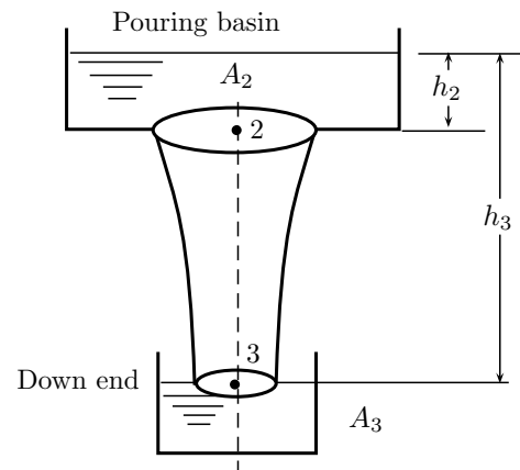
Figure 11.3 | Aspiration effect.
