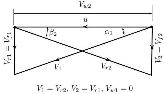
Figure 9.25 | Maximum efficiency.
