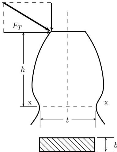
Figure 5.28 | Gear teeth as cantilever.
