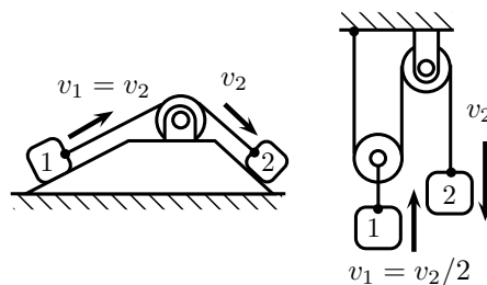
Figure 1.17 | Dependent motion of two particles.
