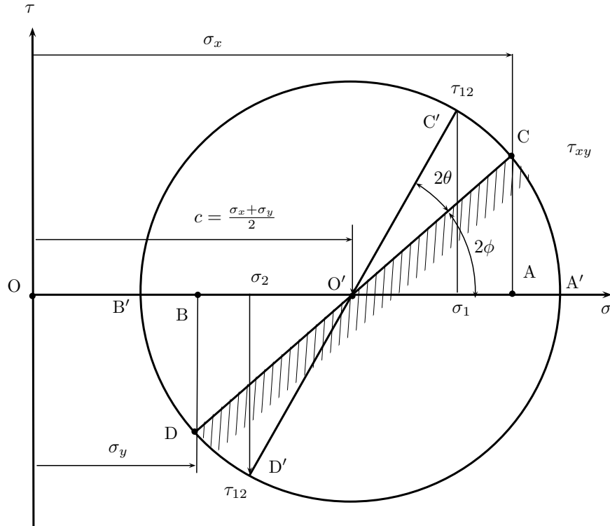
Figure 2.12 | Mohr's circle of stresses.
