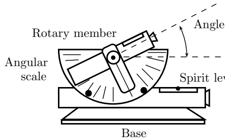
Figure 15.5 | Clinometer.
