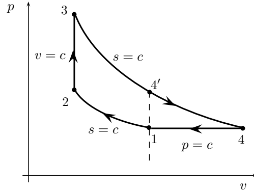
Figure 9.40 | Atkinson cycle.
