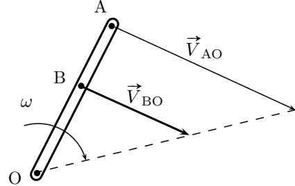
Figure 3.17 | Velocity of an intermediate point.
