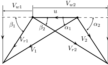
Figure 9.24 | Velocity triangle (50% reaction).
