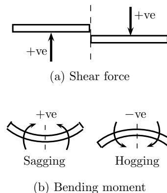
Figure 2.17 | Sign conventions for SF and BM.
