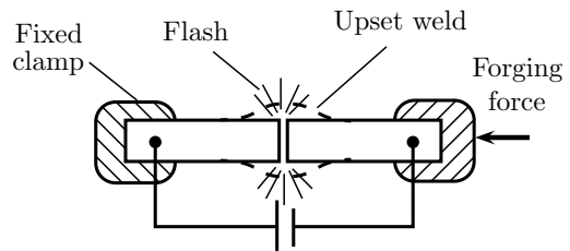
Figure 13.7 | Flash welding.
