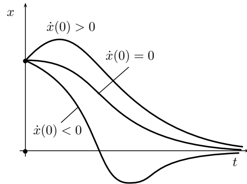
Figure 4.16 | Aperiodic motion ( \xi = 1 ).
