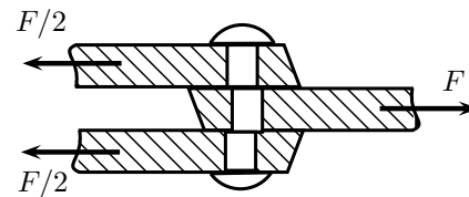
Double shear
