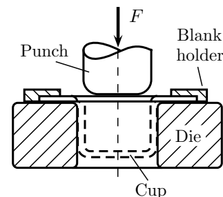
Figure 12.8 | Drawing.
