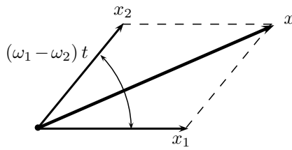
Figure 4.2 | Superposing waves.
