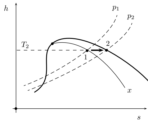
Figure 9.7 | Throttling calorimeter.
