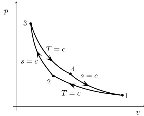
Figure 9.31 | Carnot cycle.
