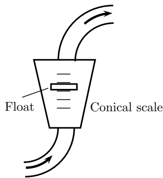
Figure 6.37 | Rotameter.
