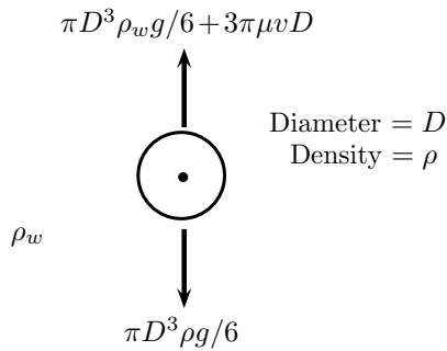
Figure 6.43 | Stokes' law.
