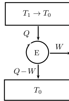
Figure 8.31 | Work from a finite body.
