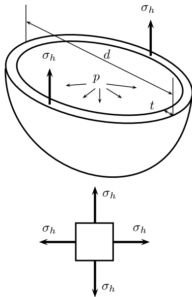
Figure 2.45 | Thin-walled sphere.
