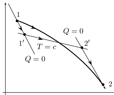
Figure 8.26 | Reversible paths.
