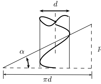
Figure 3.54 | Helix angle of screw threads.
