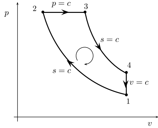
Figure 9.36 | Diesel cycle.
