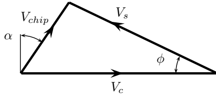
Figure 14.5 | Orthogonal cutting.
