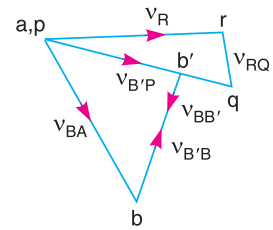
(b) Velocity diagram.
