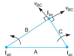
Fig. 6.7. Aronhold Kennedy's theorem.
