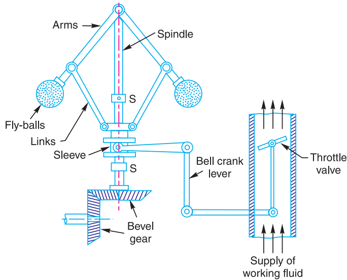
Fig. 18.1. Centrifugal governor.
