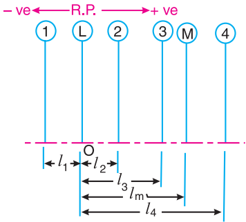
(a) Position of planes of the masses.
