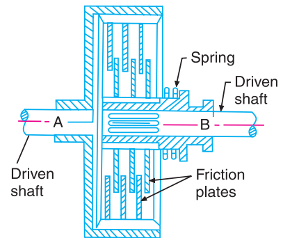
Fig. 3.7. Friction clutch.
