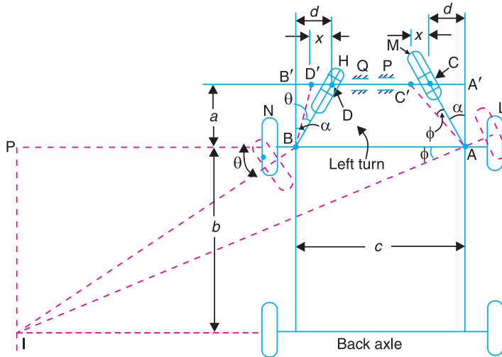
Fig. 9.16. Davis steering gear.
