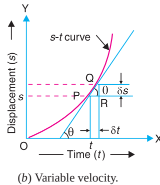
Fig. 2.1. Graphical representation of displacement with respect to time.
