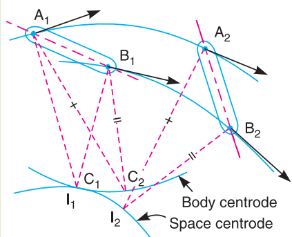
Fig. 6.3. Space and body centroides.
