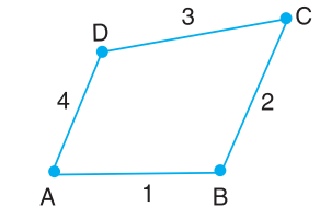
Fig. 5.10. Kinematic chain with all binary joints.
