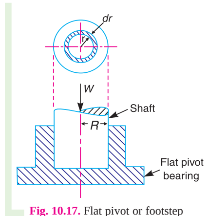
Fig. 10.17. Flat pivot or footstep bearing.
