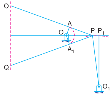
Fig. 9.8. Grasshopper mechanism.
