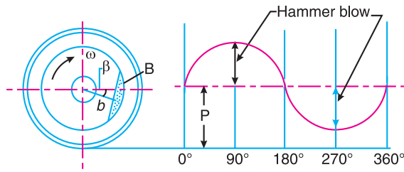
Fig. 22.6. Hammer blow.
