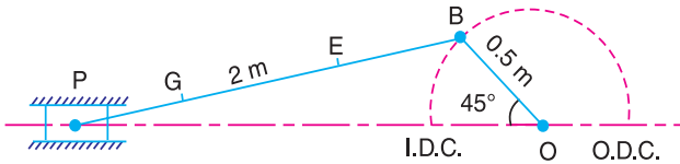
(a) Space diagram.
