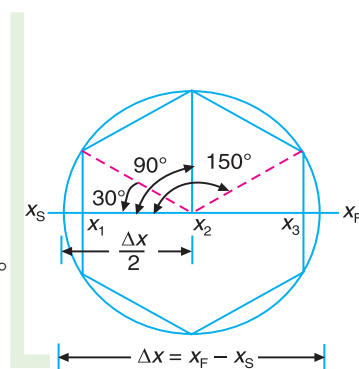
Fig. 25.5. Graphical method for determining three precision points.
