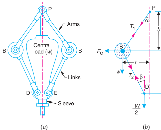
Fig. 18.3. Porter governor.
