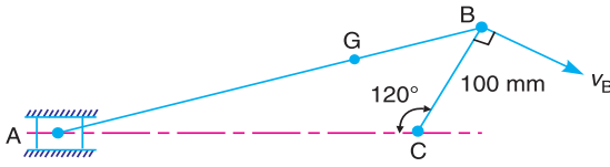
(a) Space diagram.
