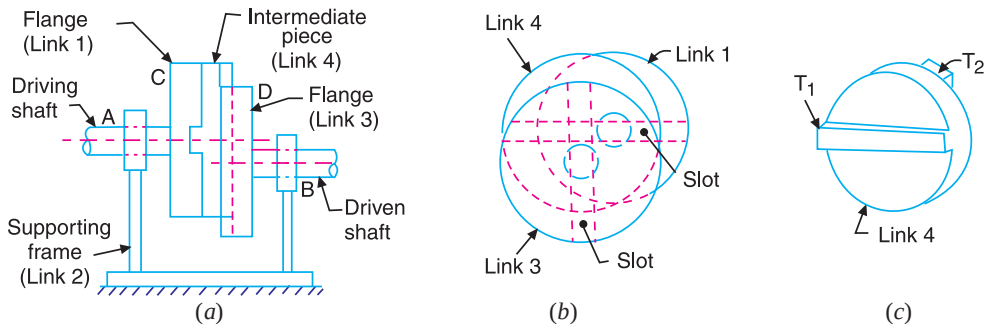
Fig. 5.36. Oldham's coupling.
