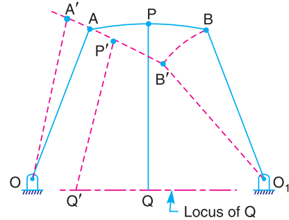
Fig. 9.10. Roberts mechanism
