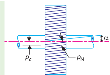
Fig. 12.15. Helical gear.
