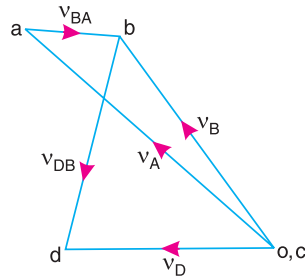
(b) Velocity diagram.
