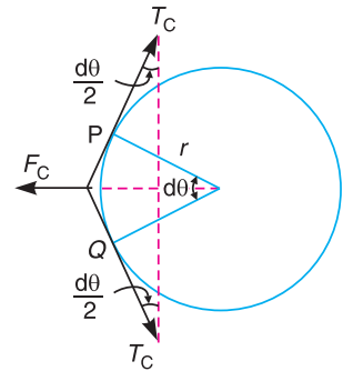
Fig. 11.17. Centrifugal tension.
