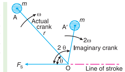
Fig. 22.16. Secondary force.
