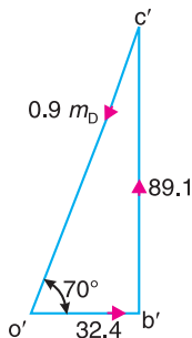
(c) Couple polygon.
