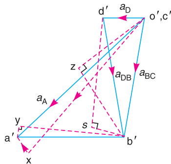
(c) Acceleration diagram.
