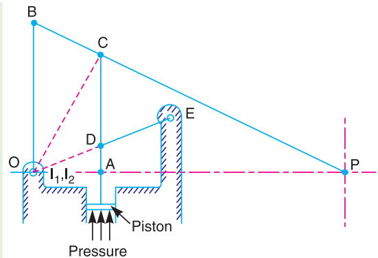
Fig. 9.12. Cross-by indicator.
