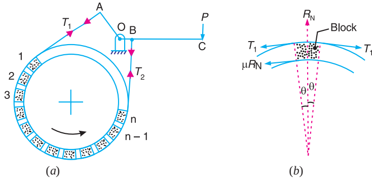
Fig. 19.20. Band and block brake.
