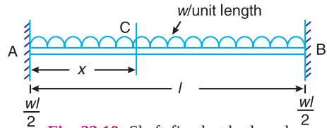
Fig. 23.10. Shaft fixed at both ends carrying a uniformly distributed load.
