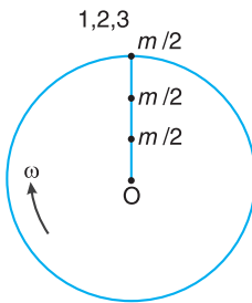
(a) Direct primary cranks.
