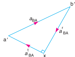
(b) Acceleration diagram.
