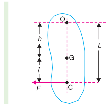
Fig. 4.6. Centre of percussuion.
