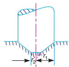
Fig 10.19. Trapezoidal pivot bearing.
