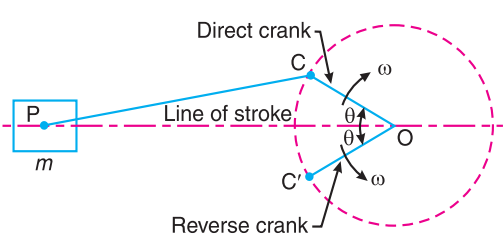
Fig. 22.27. Reciprocating engine mechanism.
