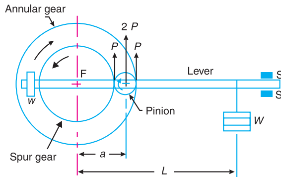
Fig. 19.33. Epicyclic train dynamometer.
