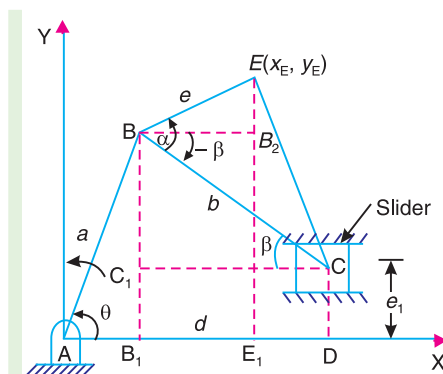
Fig. 25.4 Slider crank mechanism with coupler point.
