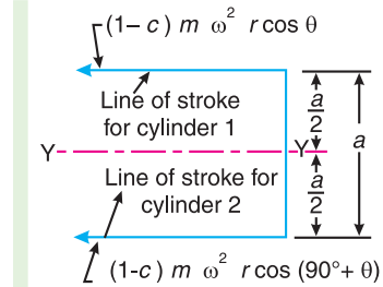
Fig. 22.5. Swaying couple.
