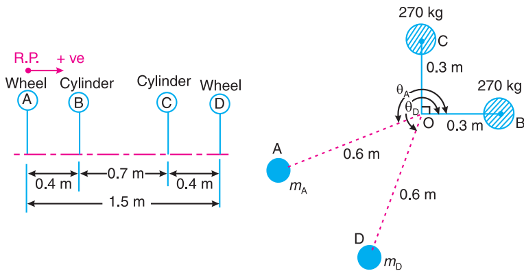
(a) Position of planes.
