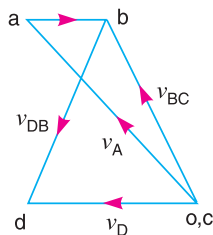
(b) Velocity diagram.
