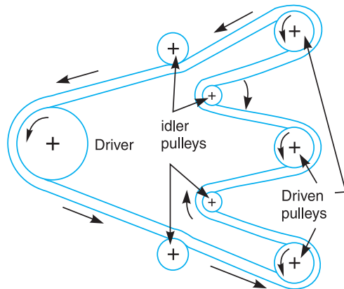
(b) Belt drive with many idler pulleys.
