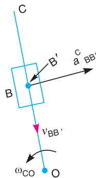
(c) Direction of coriolis component.
