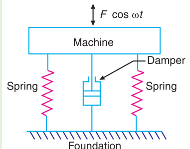
Fig. 23.22. Vibration isolation.
