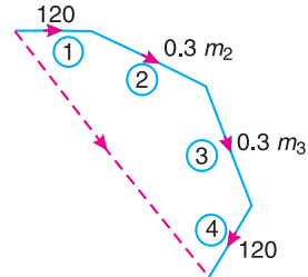
(f) Secondary force polygon.
