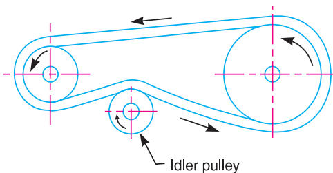
(a) Belt drive with single idler pulley.
