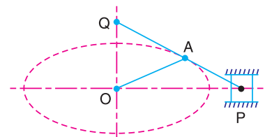
Fig. 9.7. Modified Scott-Russel mechanism.
