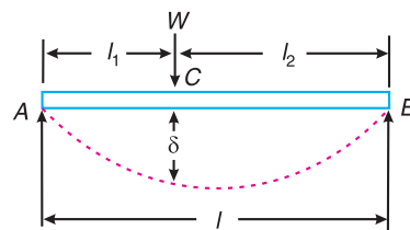
Fig. 23.6. Simply supported beam with a point load.
