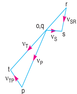
(b) Velocity diagram.
