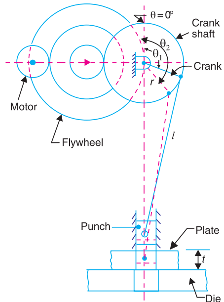
Fig. 16.22. Operation of flywheel in a punching press.
