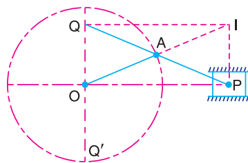
Fig. 9.5. Scott Russell's mechanism.
