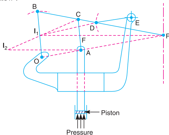
Fig. 9.13. Thompson indicator.
