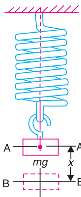
Fig. 4.4. Closely-coiled helical spring.
