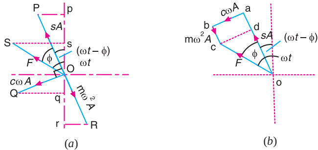
Fig. 23.20. Graphical method.
