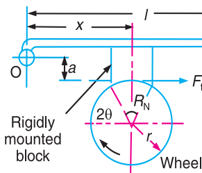
(a) Clockwise rotation of brake wheel.
