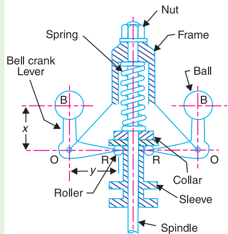
Fig. 18.18. Hartnell governor.
