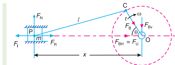
Fig. 22.1. Reciprocating engine mechanism.
