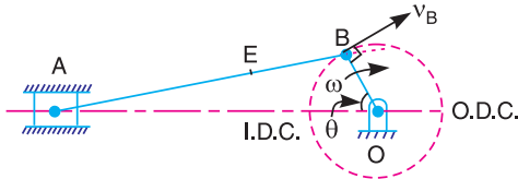
(a) Slider crank mechanism.
