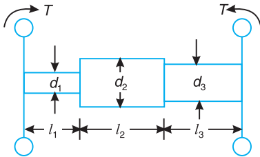
(a) Shaft of varying diameters.
