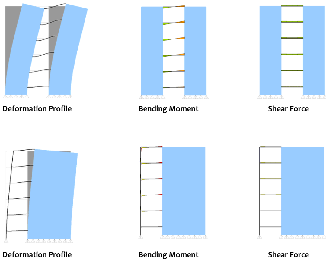
Figure 3.44: Buildings with structural walls: Long structural walls are more efficient than a number of short ones
