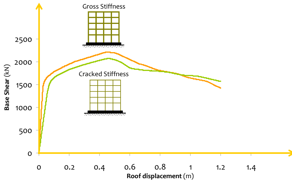
Figure 4.76: Influence of using Cracked Cross-Section Properties in RC buildings: Overall deformability is not affected
