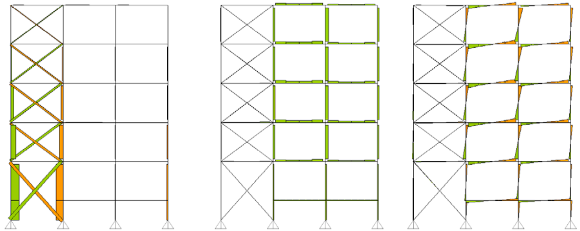
Building D
