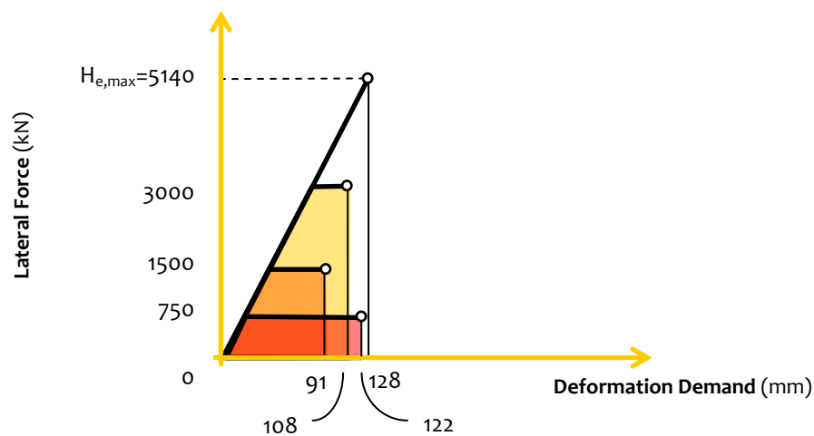
Figure 4.58: Deformation Demand on Building with T=1s subjected to 1999 Chamoli earthquake ground motion: Reducing the yield strength, increases the deformation demand
