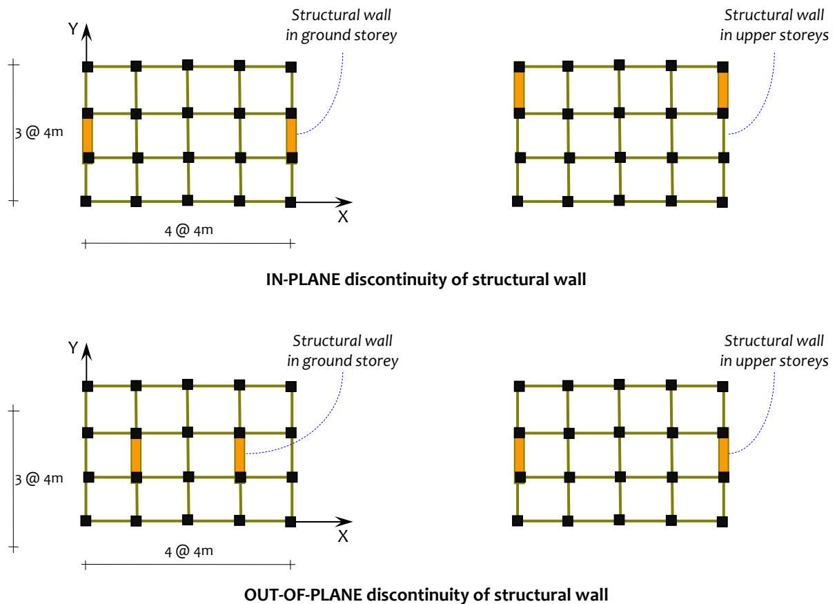
Figure 3.82: Discontinuing structural wall in lower storeys: In-plane and out-of-plane discontinuity of structural walls
