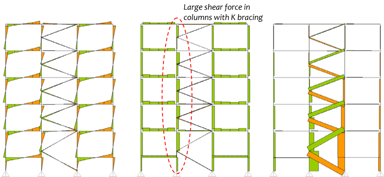
K-BRACES
