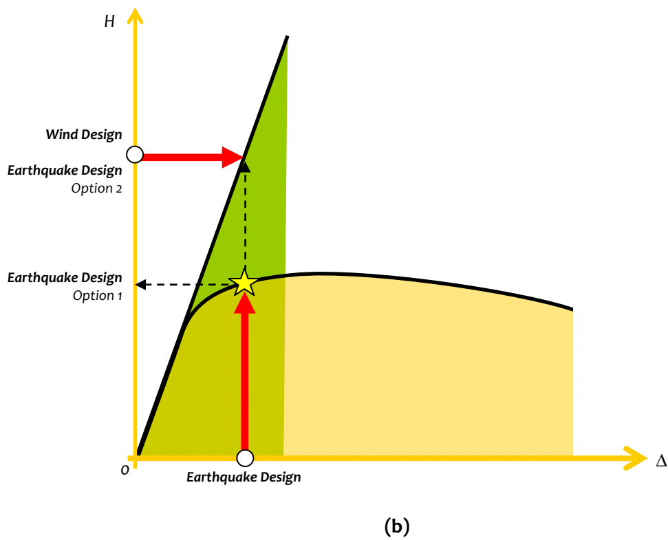
Figure 1.7: Displacement Loading versus Force Loading: Earthquake shaking imposes displacement loading on the building, while all other hazards impose force loading on it
