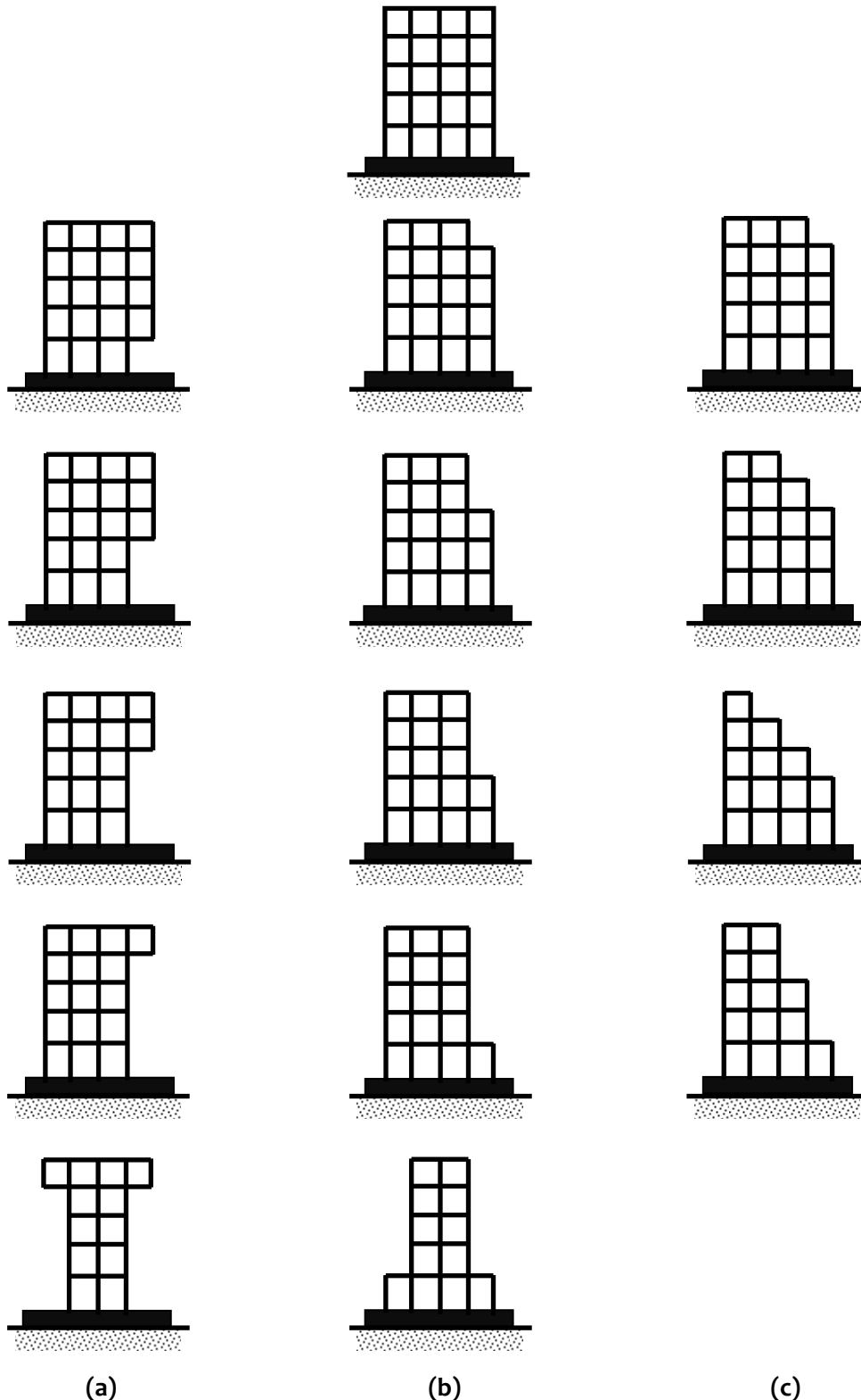
Figure 3.100: Buildings with vertical irregularity in overall geometry: (a) Set-back buildings, and (b) & (c) Step-back buildings
