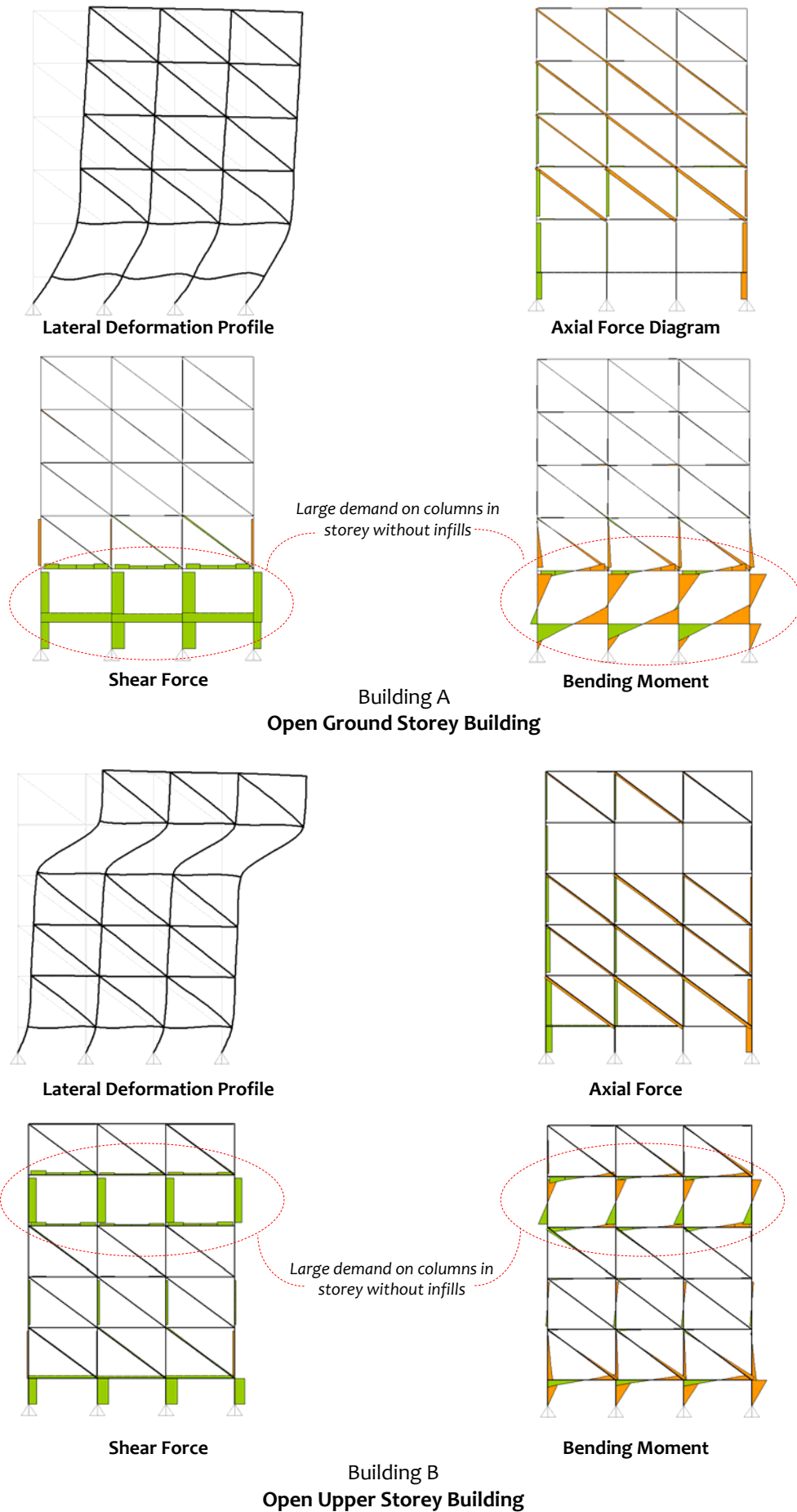
Figure 3.94: Masonry infilled frame: Discontinuity of infill in one storey cause significant demand on the columns in the storey
