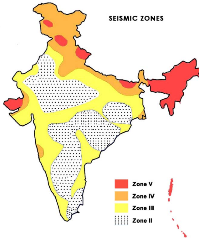
Figure 2.1: Sketch of Seismic Zone Map of India: sketch based on the seismic zone of India map given in IS:1893 (Part 1) - 2007
