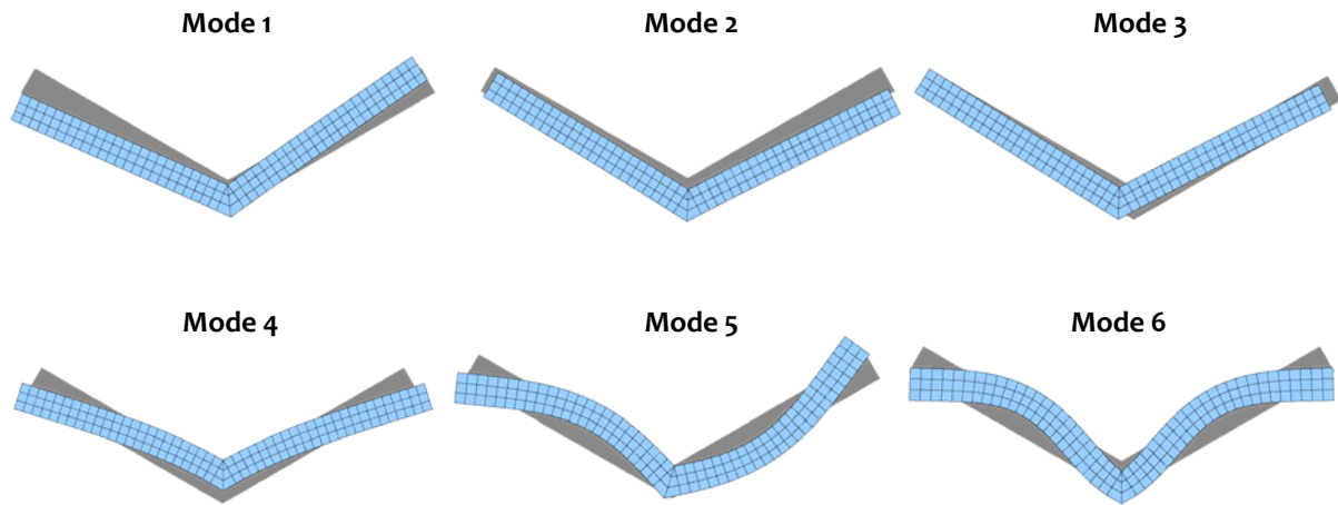
Figure 3.8: Modes of oscillation: First six modes of oscillation in building with V-plan shape
