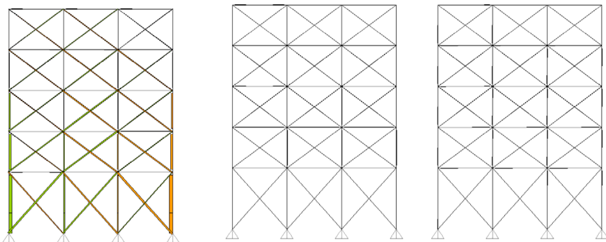
Building F
