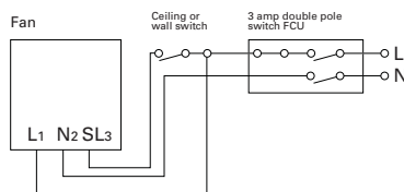
Diagram 2b Fan with Timer
