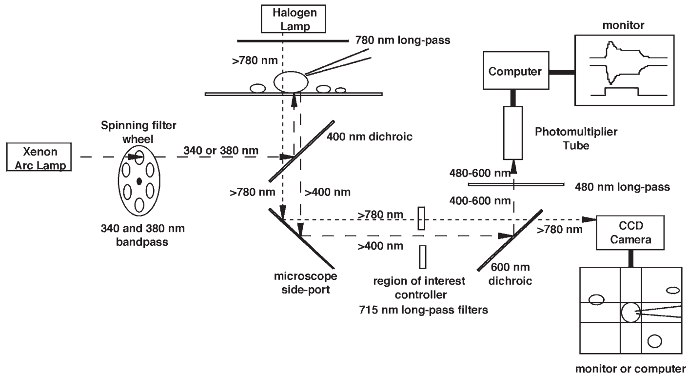
Fig. 1. Schematic representation of the filters and wavelengths within a single cell photometry setup using fura-2 as the \text{Ca}^{2+} indicator. The long dashed lines illustrate the wavelengths for excitation of fura-2 and detection of its emission by a photomultiplier tube. The short dashed lines show the path and wavelengths for simultaneous monitoring of a transmitted light image by a CCD camera. A custom region-of-interest controller with 715-nm long-pass filters permits visualization of the entire field of view. Redrawn from reference (48), with permission.
