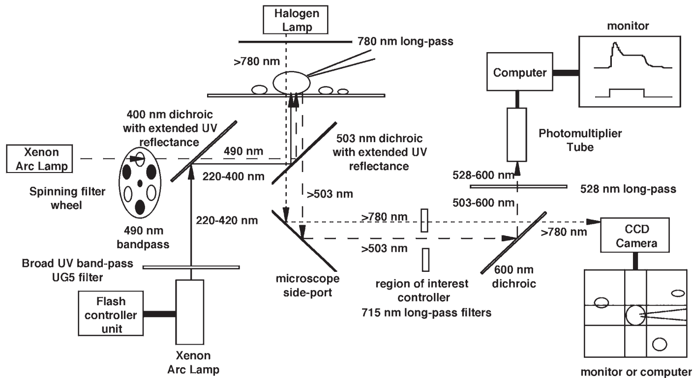
Fig. 2. Schematic representation of the filters and wavelengths within a combined flash photolysis and single-cell photometric setup. The long dashed lines illustrate the wavelengths for excitation of fluo-3 or Oregon Green 488 BAPTA-1 and detection of its emission by a photomultiplier tube. The short dashed lines show the path and wavelengths for simultaneous monitoring of a transmitted light image. The solid lines show the excitation wavelengths for flash photolysis of caged compounds.
