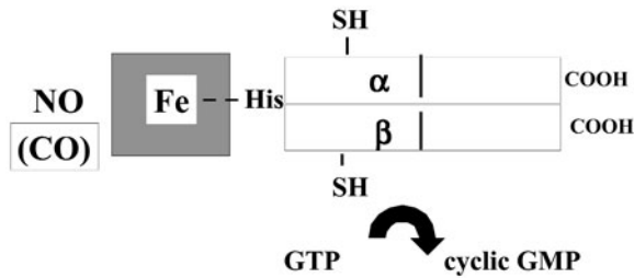
Fig. 2. The activation of soluble guanylyl cyclase by nitric oxide (and carbon monoxide).
