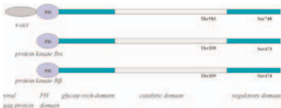
Fig. 3. Structure of protein kinase B. Platelets contain the protein kinase B \alpha and - \beta isoforms differing slightly in the position of the phosphorylation sites. Both contain a pleckstrin homology (PH) domain for binding to the plasma membrane (modified from ref. 7).
