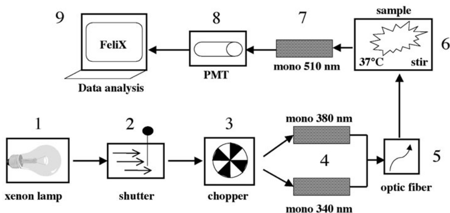
Fig. 2. Spectrofluorometer hardware system with dual excitation wavelengths. The illumination produced by the xenon arc lamp (1) first encounters a rotating chopper disk (3), which alternates the direction of the incident beam to one of two monochromators, one set at 340 nm, the other at 380 nm (4), via a focusing mirror. A shutter (2) is included to protect the sensitive PMT detector (8) from excessive light. The two separate monochromator outputs are collected by a quartz fiberoptic bundle that focuses the excitation light onto the sample (5). The sample holder is designed to accommodate a 10-mm-wide square cuvet and has a provision for sample stirring and for variable temperature (6). The sample compartment is attached to the emission monochromator (510 nm) and the photon counts are measured using a PMT (8). The fluorescence spectrometer is linked to a computer equipped with an acquisition system and appropriate software (9), for example FeliX (Photon Technology International Inc. Princeton, NJ).
