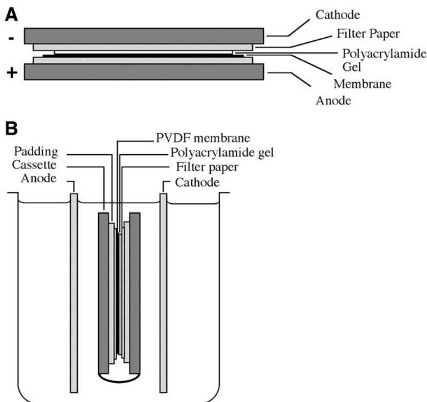
Fig. 1. Schematic representation of typical apparatus for Western blotting. (A) Semi-dry blotting is performed in a transfer cell comprising two large plate electrodes. Buffer-soaked filter papers are placed on the anode, followed by a PVDF or nitrocellulose membrane, the SDS-PAGE gel, and more pieces of soaked filter paper. Following the placement of the cathode, electrophoretic transfer is performed by supplying power to the unit. Proteins, which are coated in negatively charged SDS, migrate toward the anode and are captured on the membrane. (B) The same principle applies to wet Western blotting, except that the sandwich of filter papers, gel, and membrane are submerged in a large tank of buffer between the anode and the cathode, and power supplied.
