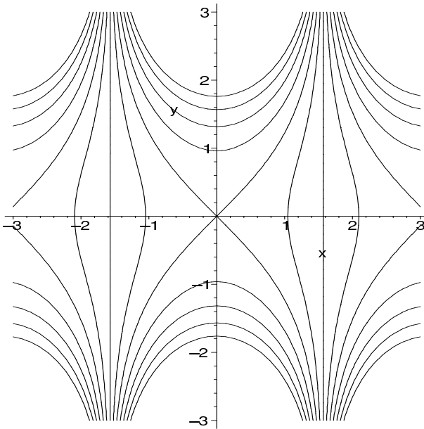
FIGURE 3.3: Steepest descent lines for \text{Re}[i \cos(x + iy)] .
