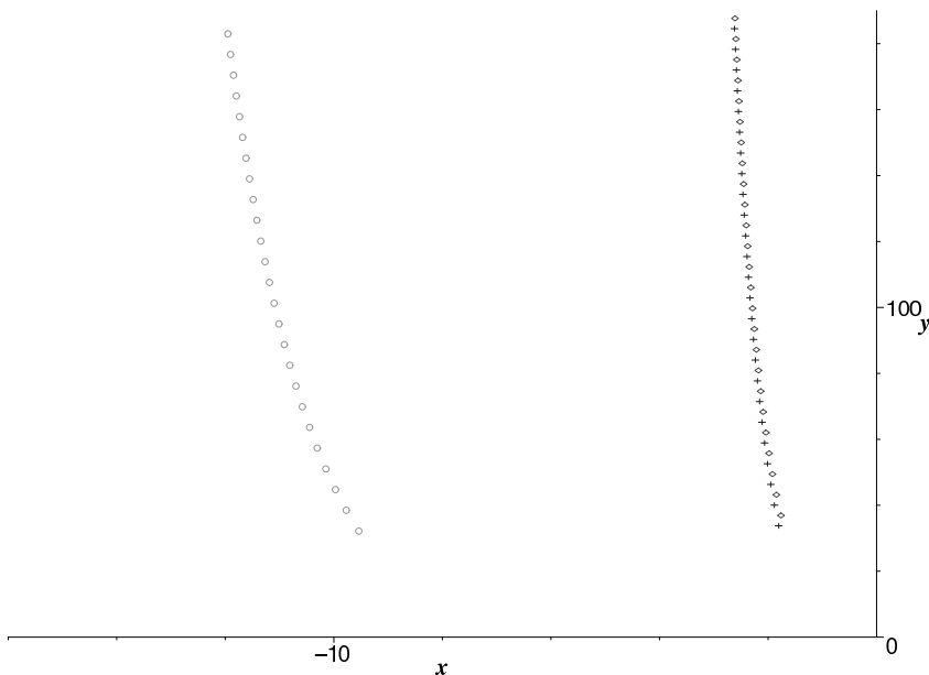
FIGURE 6.4: Poles of (4.85) for C = -12 ( \diamond ) and C = 12 ( + ), calculated via (6.70). The light circles are on the second line of poles for to C = -12 .
