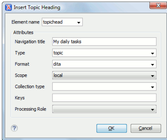
Figure 210: Insert Topic Heading Dialog
