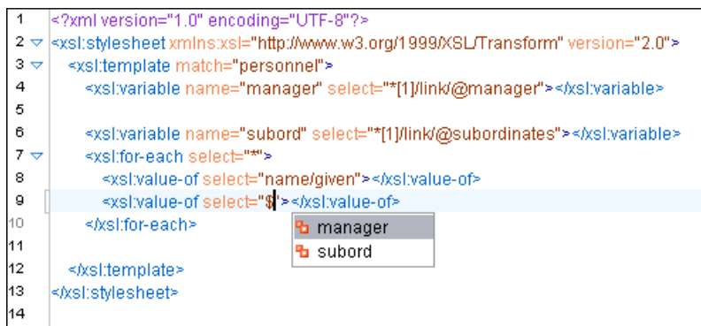
Figure 104: Content Completion in the test Attribute
