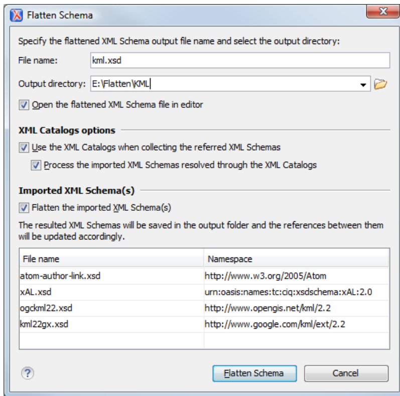
Figure 155: Flatten Schema Dialog
