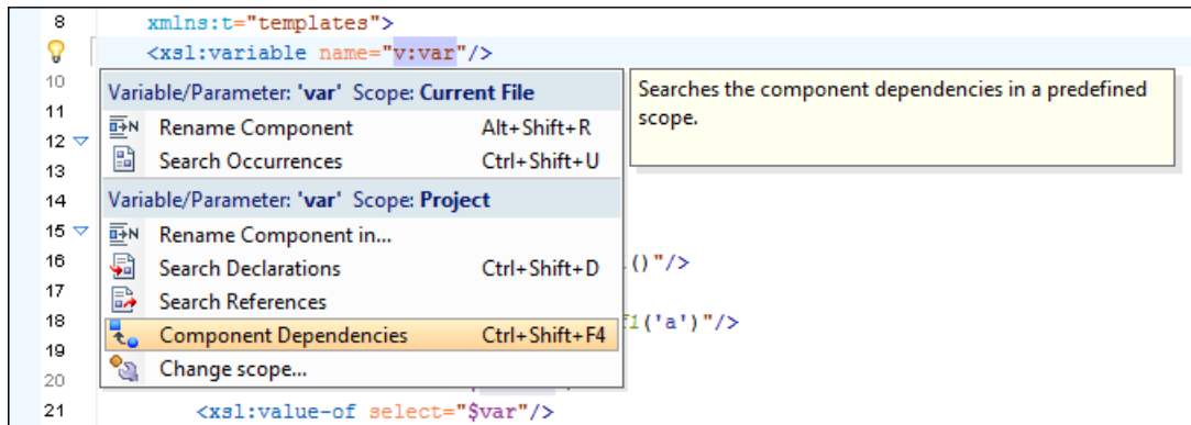
Figure 124: XSLT Quick Assist Support - Component Actions
