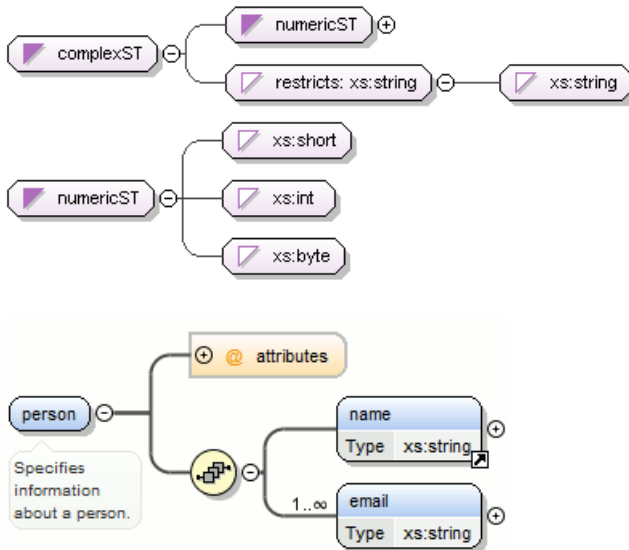
Figure 137: Extracting a Global Complex Type
