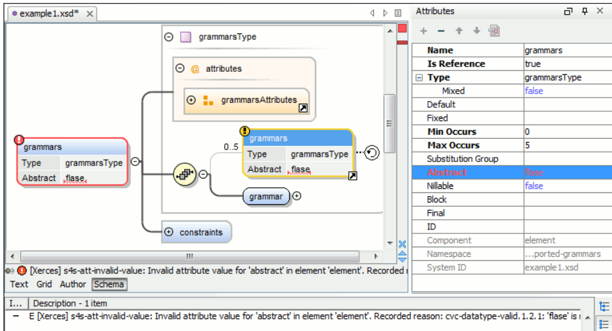
Figure 132: XML Schema Validation
