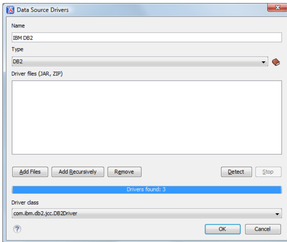
Figure 312: Data Source Drivers Configuration Dialog
