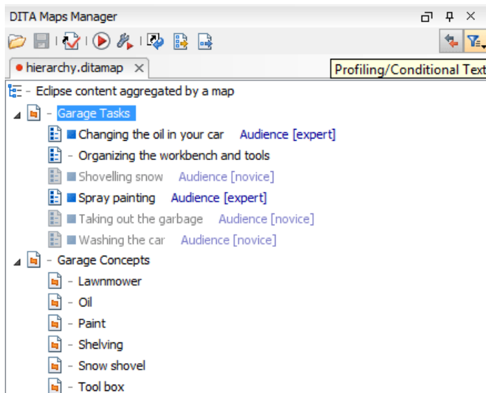
Figure 219: Profiling in DITA Maps Manager
