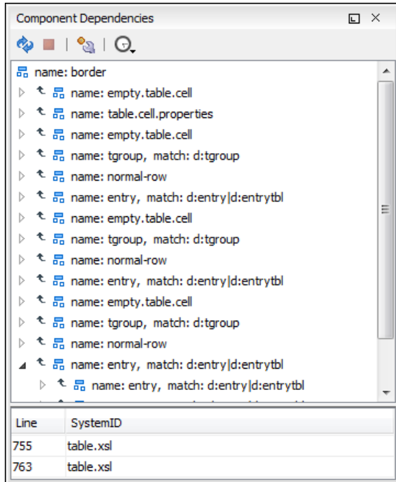
Figure 122: Component Dependencies View - Hierarchy for table.xsl
