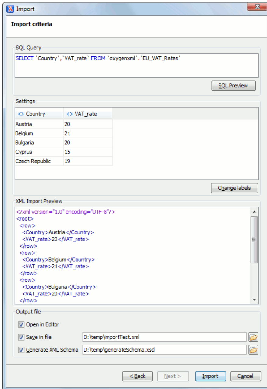
Figure 335: Import from Database Criteria Dialog
