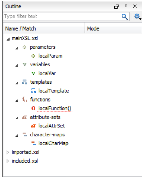
Figure 112: The XSLT Outline View
