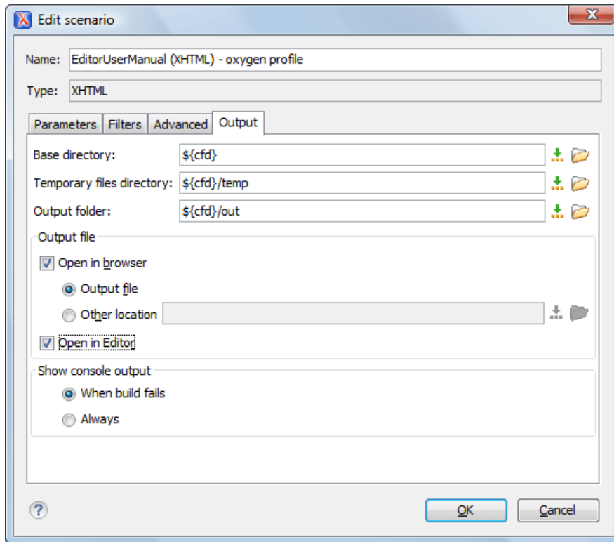
Figure 274: Output settings tab
