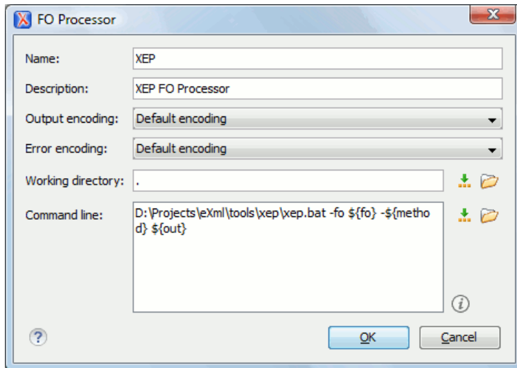
Figure 406: The External FO Processor Configuration Dialog
