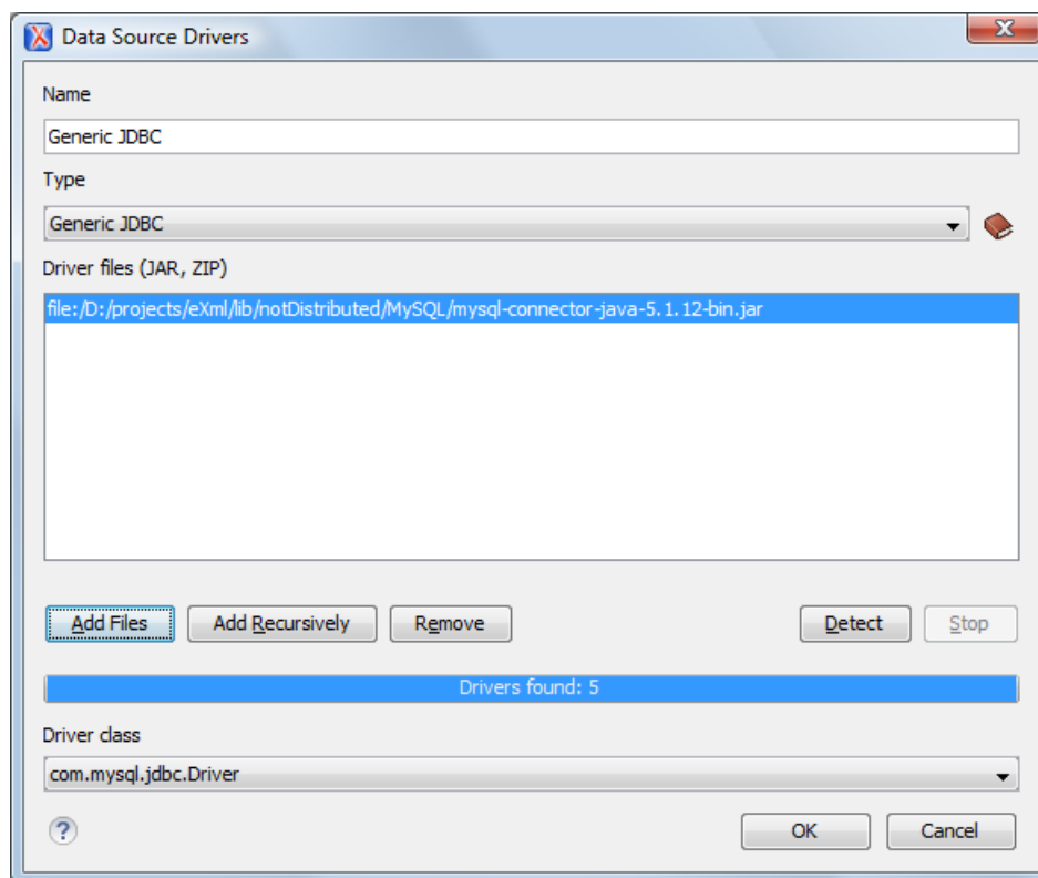
Figure 314: Data Source Drivers Configuration Dialog
