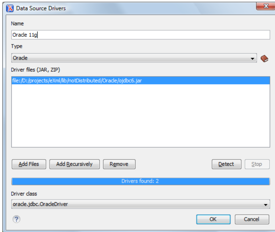
Figure 410: The Data Sources Drivers Dialog
