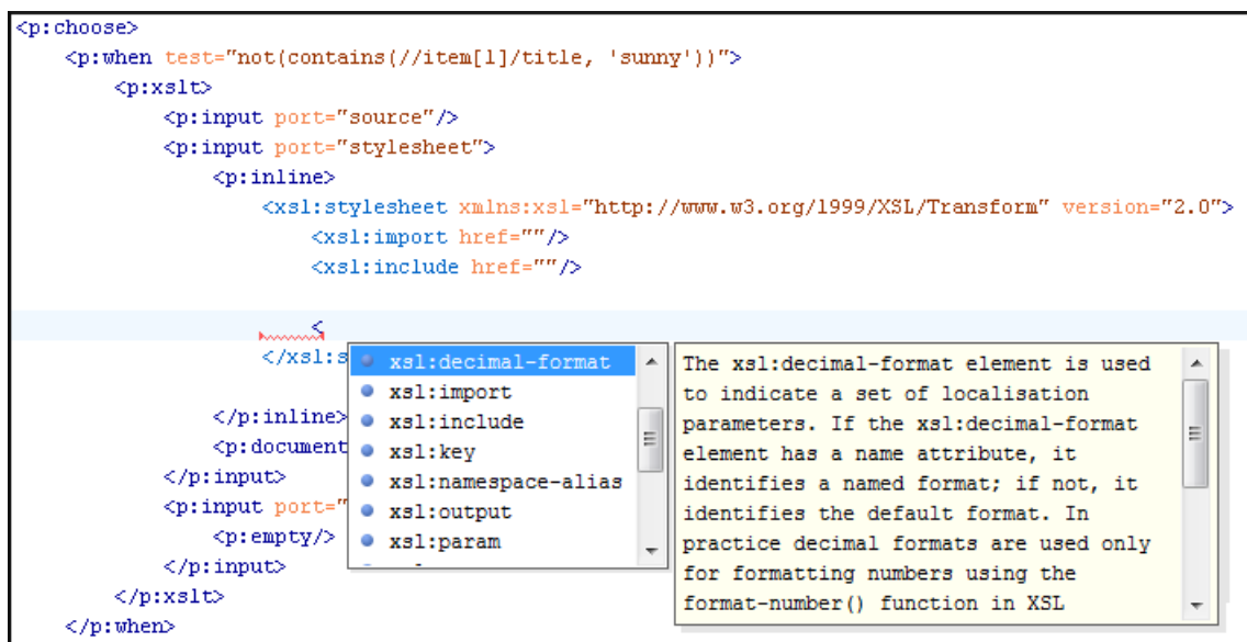
Figure 197: XProc Content Completion
