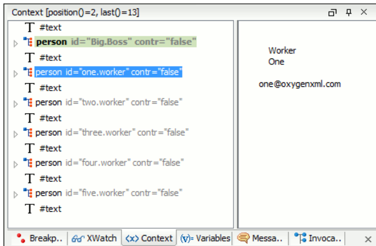
Figure 295: The Context node view
