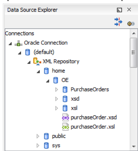
Figure 329: Browsing the Oracle XML DB Repository
