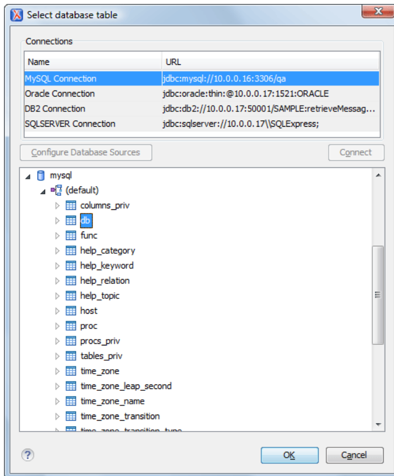
Figure 334: Select Database Table Dialog
