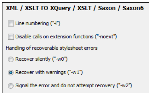
Figure 402: The Saxon 6 XSLT Preferences Panel
