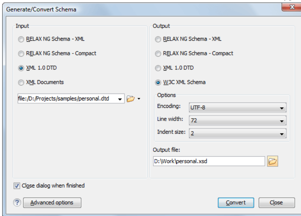
Figure 94: Convert a Schema to Other Schema Language
