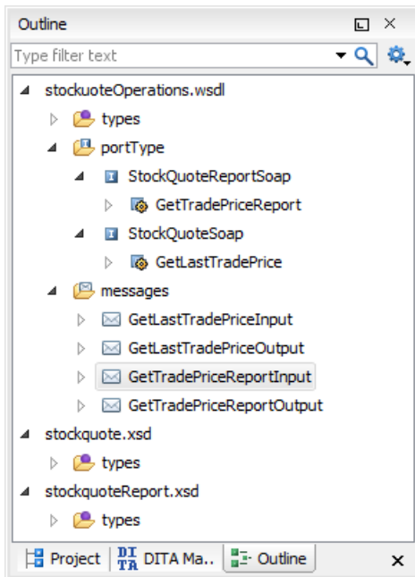
Figure 165: The WSDL Outline View
