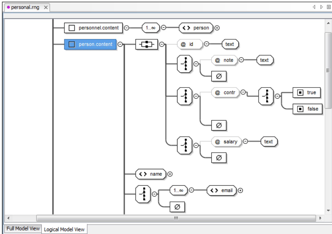
Figure 183: Logical Model View for a Relax NG Schema
