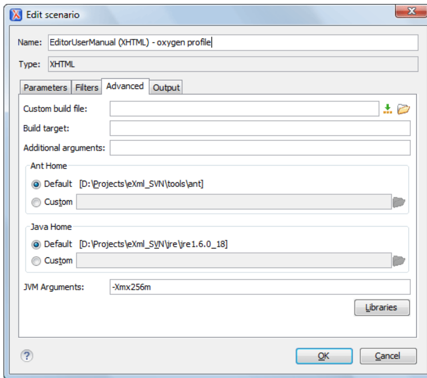
Figure 214: Advanced settings tab
