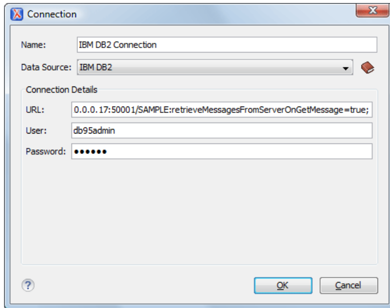
Figure 317: The Connection Configuration Dialog
