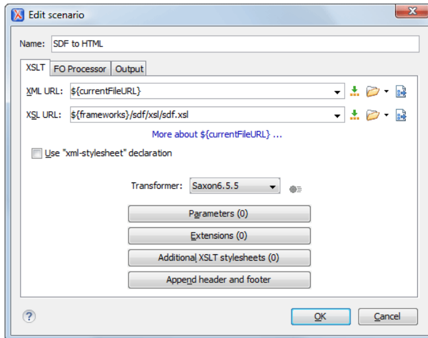
Figure 257: Configuring a transformation scenario
