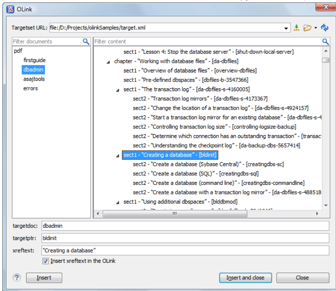
Figure 225: Insert OLink Dialog
