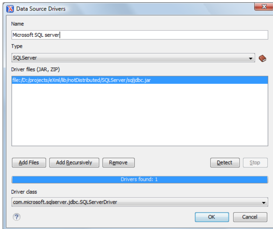
Figure 313: Data Source Drivers Configuration Dialog
