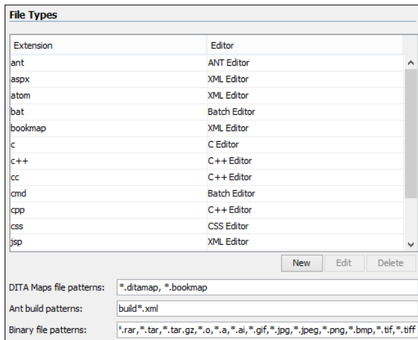
Figure 425: The File Types Preferences Panel
