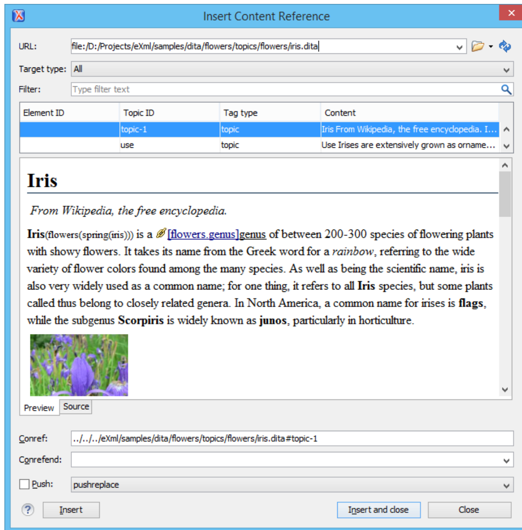
Figure 233: Insert Content Reference Dialog
