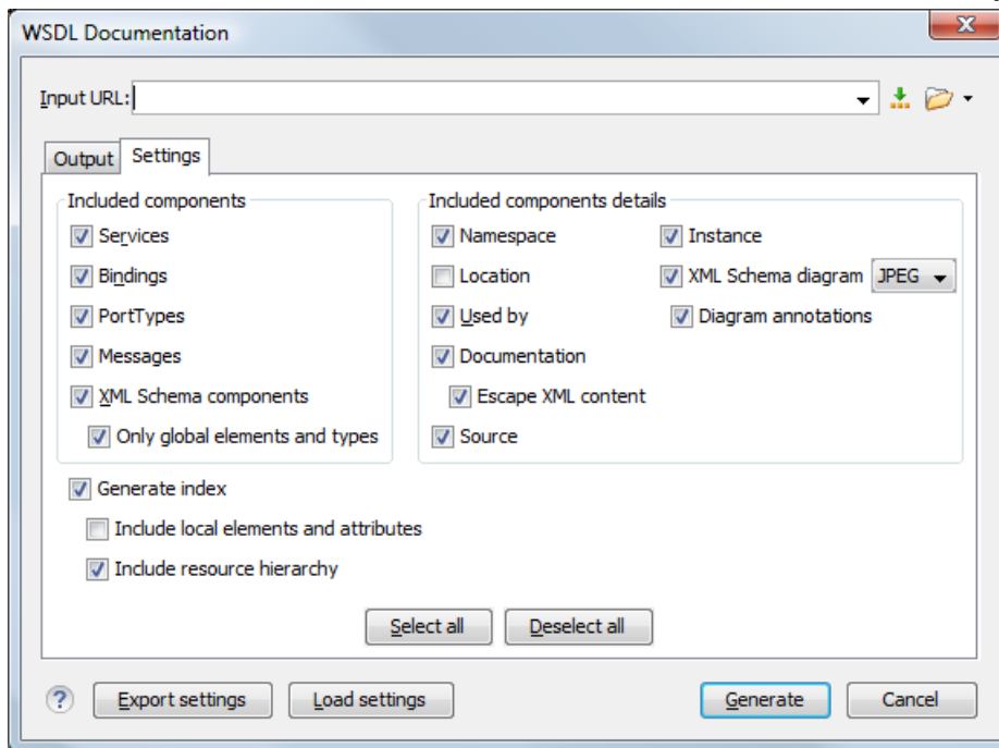
Figure 174: The Settings Panel of the WSDL Documentation Dialog
