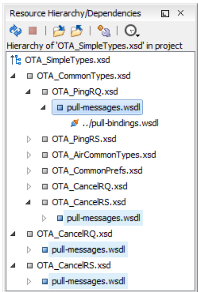
Figure 170: Resource Hierarchy/Dependencies View
