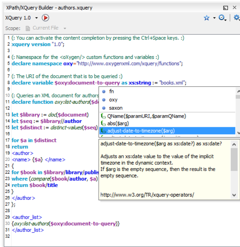
Figure 281: The XPath/XQuery Builder View
