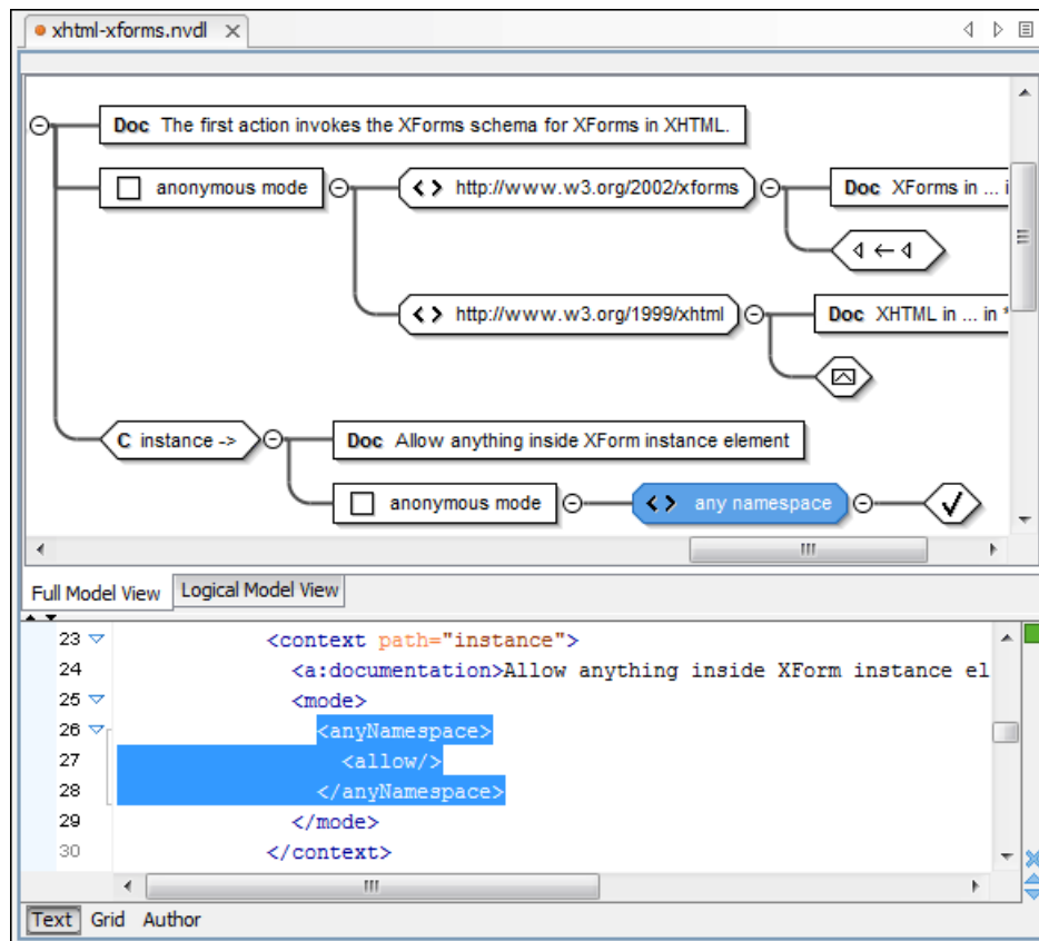
Figure 189: NVDL Schema Editor - Full Model View
