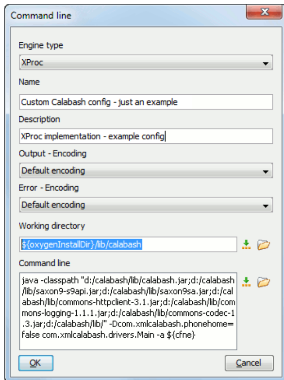
Figure 401: Creating an XProc external engine
