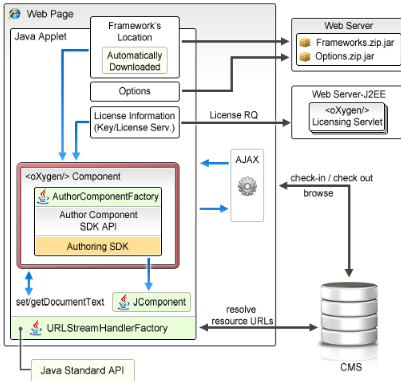
Figure 270: Oxygen XML Editor Author Component deployed as a Java applet
