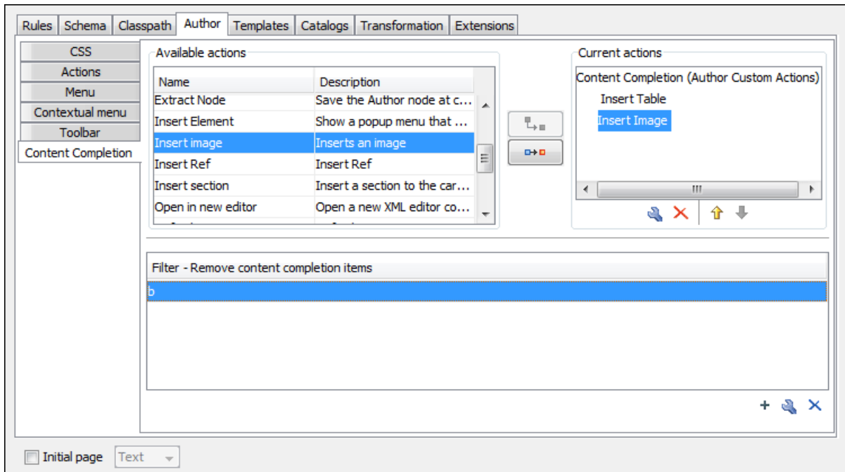
Figure 249: Customize Content Completion
