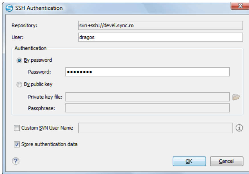
Figure 342: User & Private key authentication dialog
