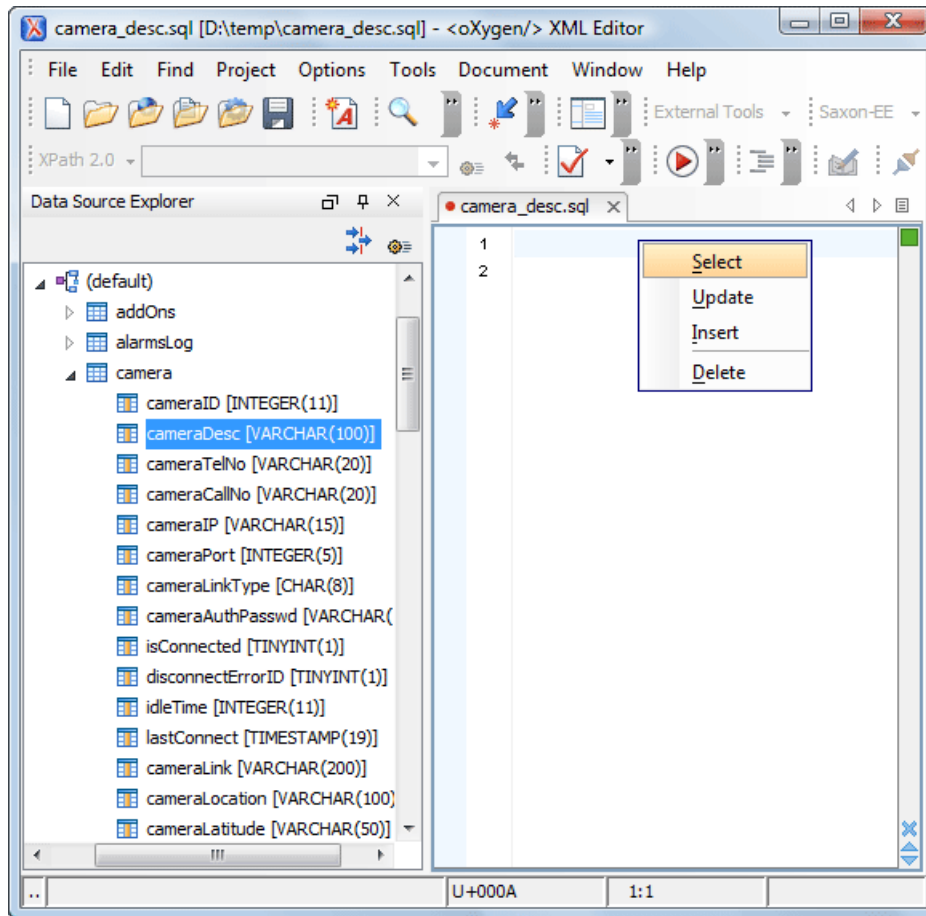
Figure 327: SQL statement editing with DND
