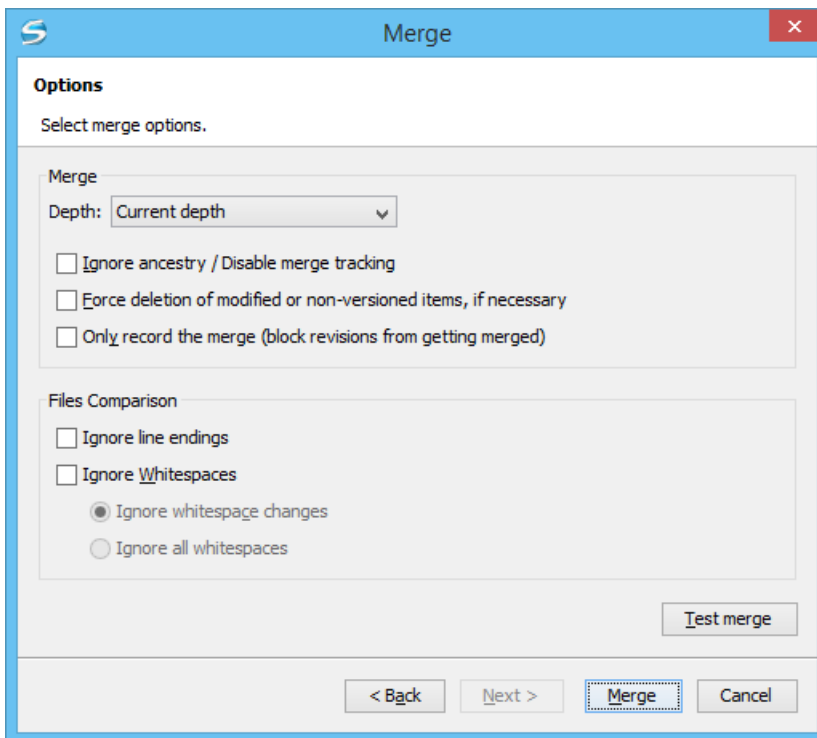
Figure 359: The Merge Wizard - Advanced Options
