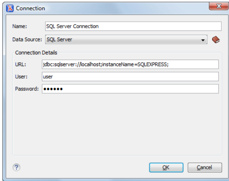
Figure 319: The Connection Configuration Dialog
