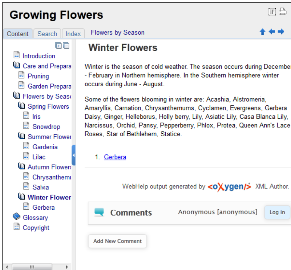
Figure 228: The layout of the Feedback-Enabled WebHelp System
