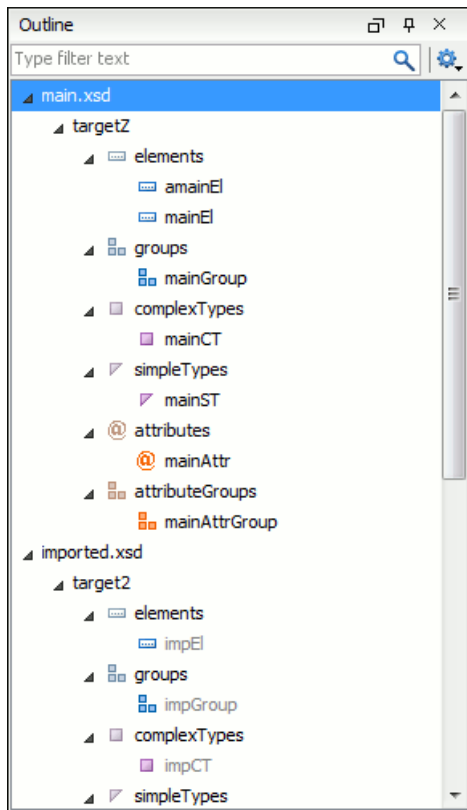
Figure 138: The Outline View for XML Schema
