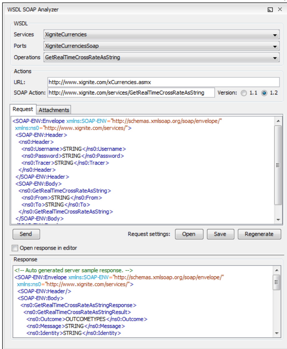
Figure 178: WSDL SOAP Analyser
