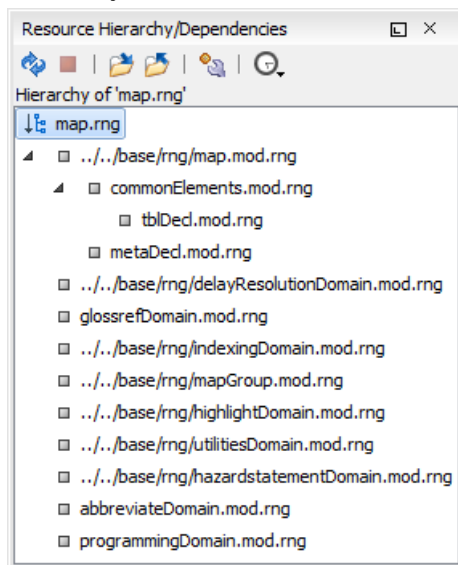
Figure 185: Resource Hierarchy/Dependencies View - hierarchy for map.rng
