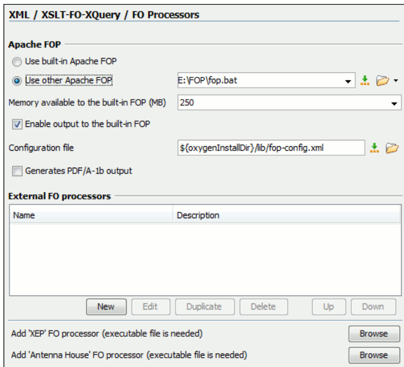
Figure 405: The FO Processors Preferences Panel
