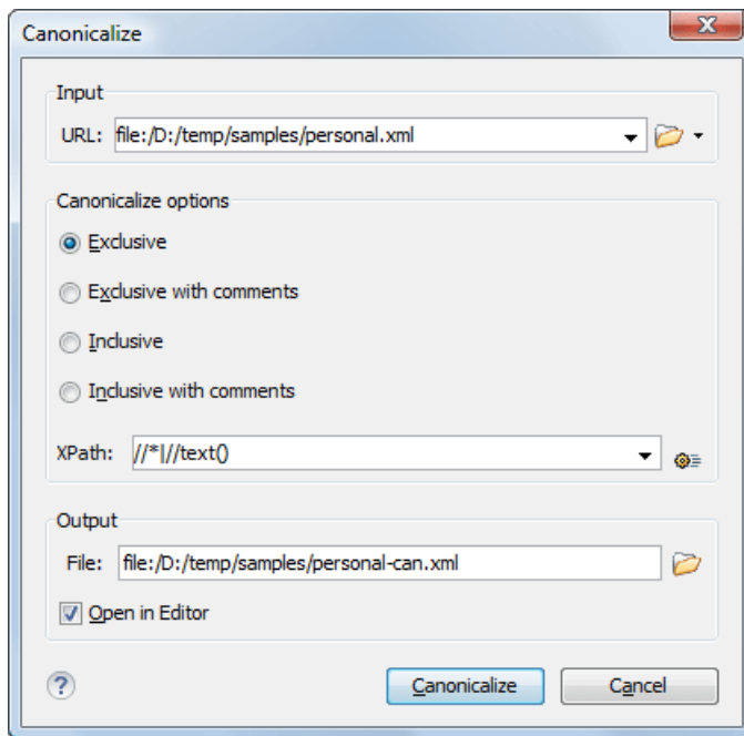
Figure 394: Canonicalization settings dialog
