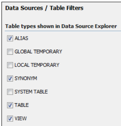
Figure 413: Table Filters Preferences Panel
