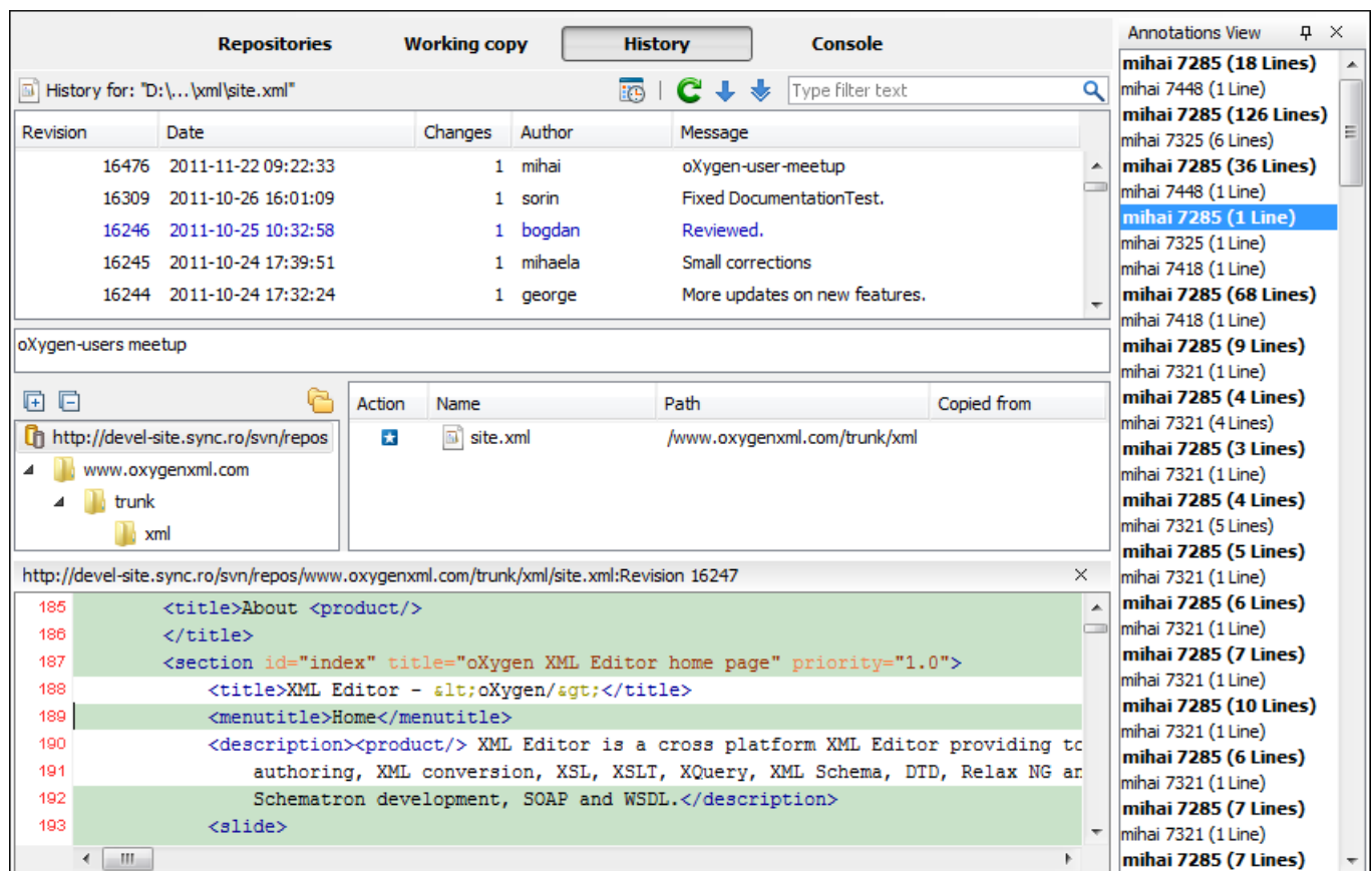
Figure 380: The Annotations View
