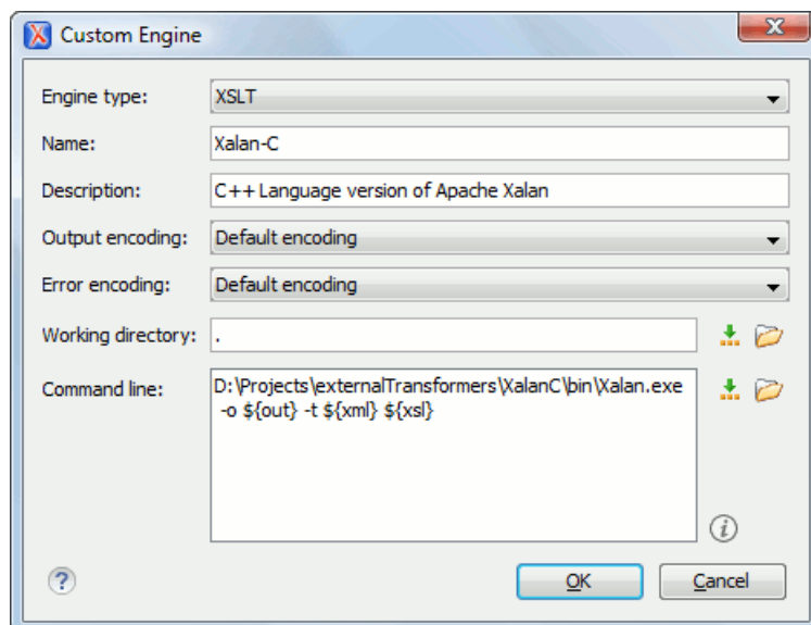
Figure 407: Parameters of a Custom Engine
