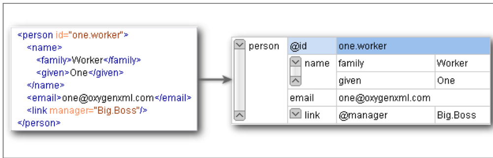
Figure 15: Copying XML Data into Grid
