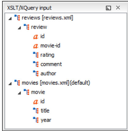
Figure 285: XQuery Input view
