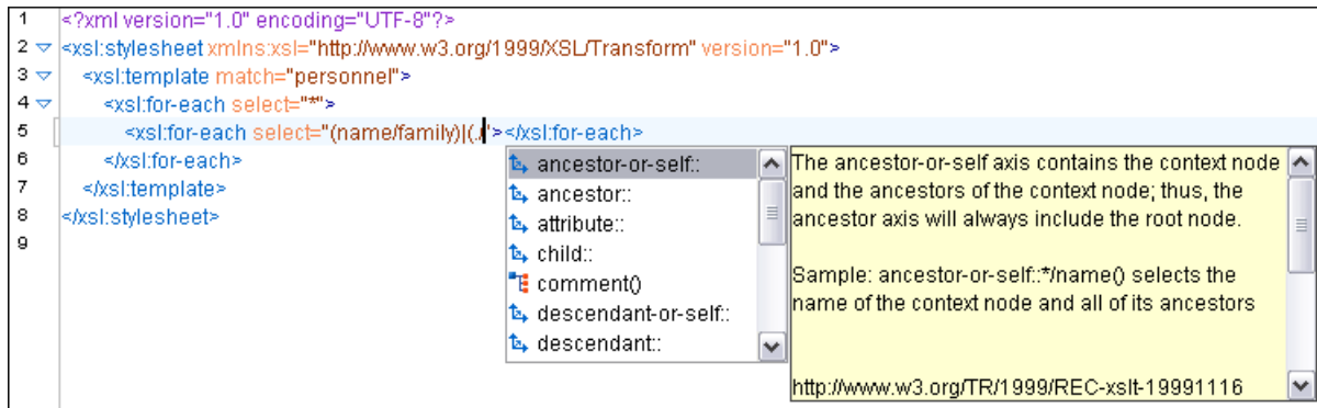
Figure 102: Content Completion in the select Attribute
