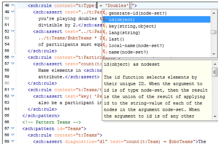
Figure 198: XSLT extension functions in Schematron schemas documents
