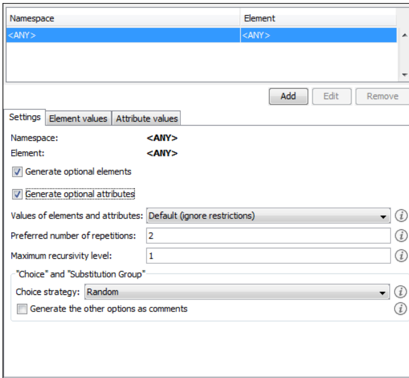
Figure 157: The Generate Sample XML Files Dialog
