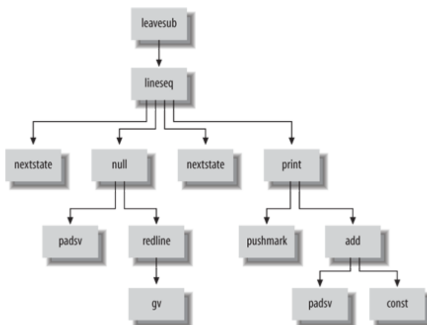
Figure 1-5. Bytecode tree
