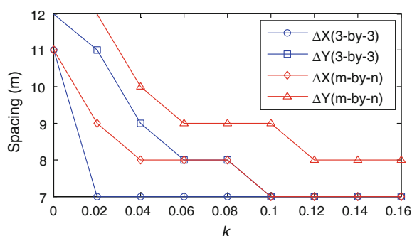
Fig. 25 Most narrow tracker spacing that minimizes the cost function with DNI data from TMY3
