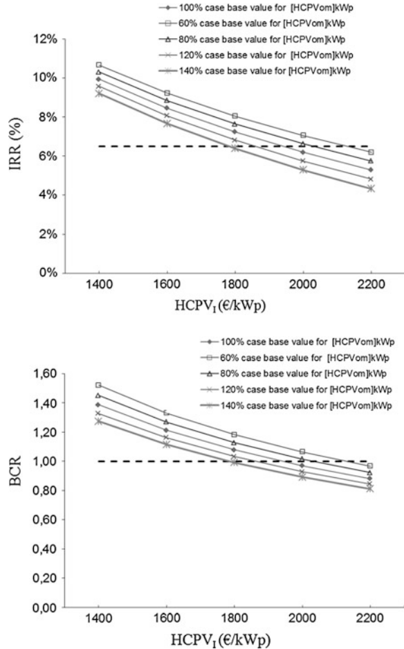
Fig. 12 IRR ( top panel ) and BCR ( bottom panel ) as a function of initial investment cost for variations of normalized-per-kWp annual operation and maintenance cost. For each figure the rest of parameters are those of base case in Table 2. The horizontal dashed line shows the threshold of economic feasibility for both criteria, i.e., d = WACC = 6.5\% ( top panel ), and BCR = 1 ( bottom panel )
