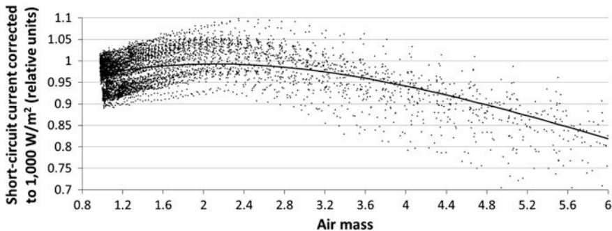
Fig. 4 Short-circuit current corrected to 1000 \text{ W/m}^2 of irradiance and normalized to the rated short-circuit current at Concentrator Standard Test conditions versus air mass for an HCPV module measured outdoors at Jaén, south of Spain, during an experimental campaign of 8 months as well as regression curve modelled as a fourth-order polynomial. The module was composed of five series-connected GaInP/GaInAs/Ge solar cells, with one squared flat Fresnel lens per cell with 625\times concentration factor, passively cooled through a finned heat exchanger. Air mass was calculated from the registered values of sun elevation angle with a pressure correction based on Jaén's altitude
