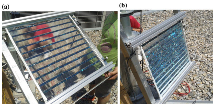
Fig. 3 The effect of the angle of incidence on the amount of beam solar radiation that reaches the PV cells concentrating PV glass pane: (a) at low incidence angles the PV cells receive only the solar radiation which is directly incident onto their surface. The remaining radiation penetrates behind the glass pane, (b) at high incidence angles the larger part of beam solar radiation is reaching the PV cells either directly or after total internal reflection at the prismatic surface
