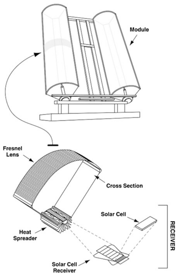
Fig. 6 Linear-focus Fresnel lens CPV system [3]
