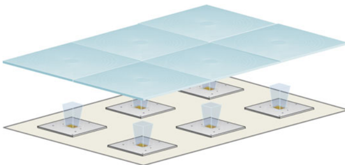
Fig. 2 Schematic of an HCPV module
