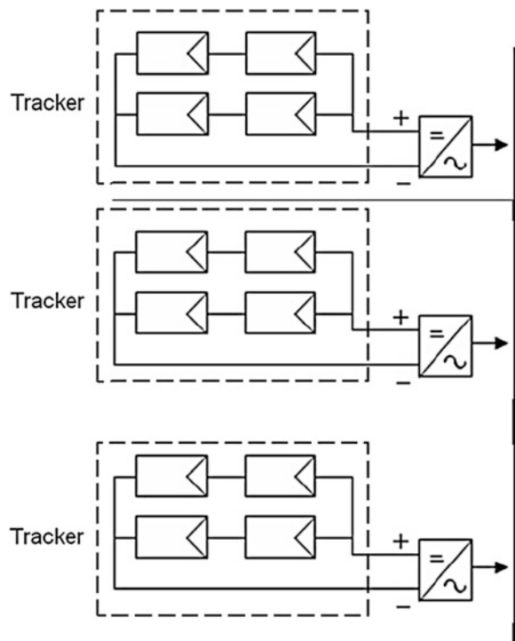
Fig. 13 Tracker oriented inverter configuration
