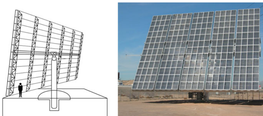
Fig. 7 Pedestal-mounted two-axis tracker for point-focus Fresnel lens PV concentrator ( courtesy of IEC62108 and Amonix )
