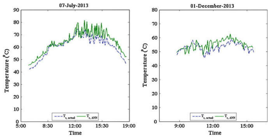
Fig. 4 Left Actual cell temperature versus predicted cell temperature by the ANN-based model for a summer day (07 July 2013). Right Actual cell temperature versus predicted cell temperature by ANN-based model for a winter day (01 December 2013)
