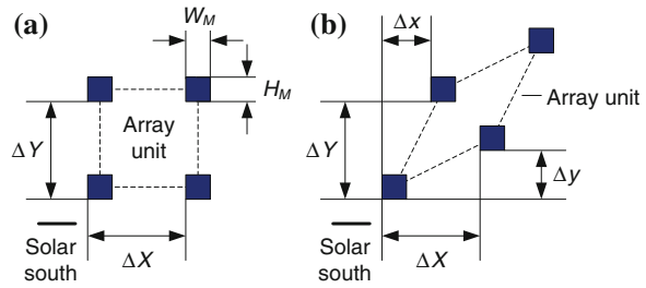
Fig. 18 Two types of tracker array units. a Rectangular array unit. b Quadrangular array
