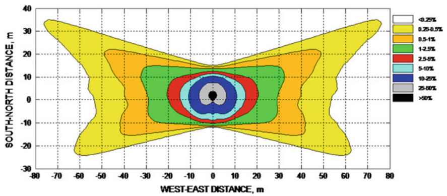
Fig. 19 Percentages of shading annual direct irradiation losses on a tracker caused by another tracker. Trackers dimensions are 11.5 \times 8.8 m. Typical direct normal irradiance data and sun position angles of Aguascalientes, México, were used for the calculations
