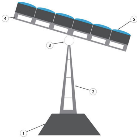
Fig. 11 Main parts of a pedestal solar tracker to HCPV system: 1 Base and embedding in the ground. 2 Picket for raising the structure and avoiding collisions during movement. 3 Mechanical and control systems in charge of the tracker movement. 4 Mechanical structure to support the solar modules and their weight. 5 HCPV solar modules
