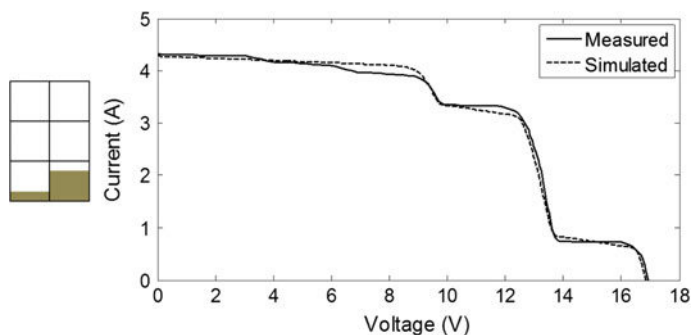
Fig. 14 Example of measured and simulated I–V curves for the module A. The shading pattern for the module is represented at the left side . Module A uses GaInP/GaInAs/Ge solar cells with 500\times concentration factor provided by flat Fresnel lenses
