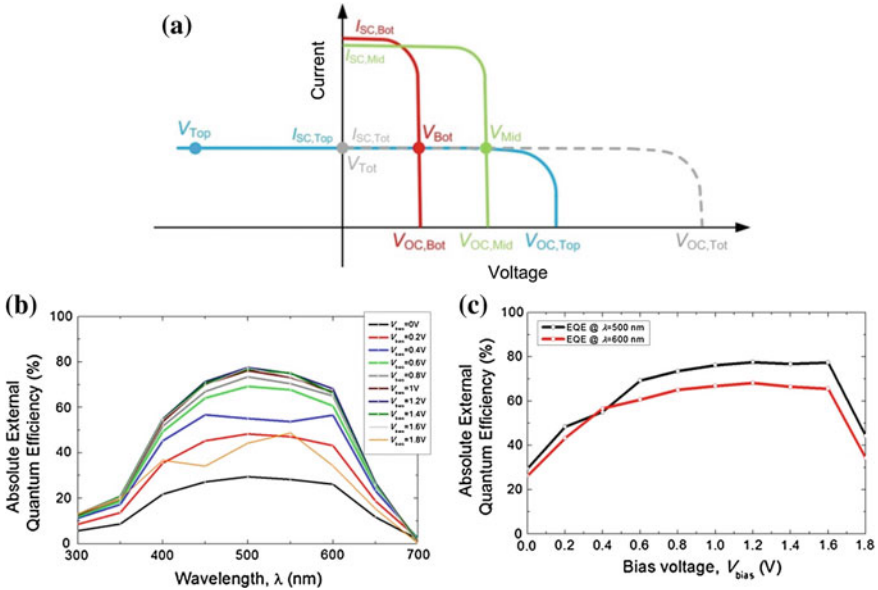
Fig. 5 a Sketch of the I-V curves of the MJSC (dashed gray) as well as from each of the other subcells. The top cell of the triple-junction cell is represented with a solid blue line, the middle cell with a green solid line, and the bottom cell with a red solid line. b QE as a function of V_{ext} . c QE at \lambda = 500 nm and \lambda = 600 nm as a function of V_{ext} from 0 V to 1.8 V (color in online)
