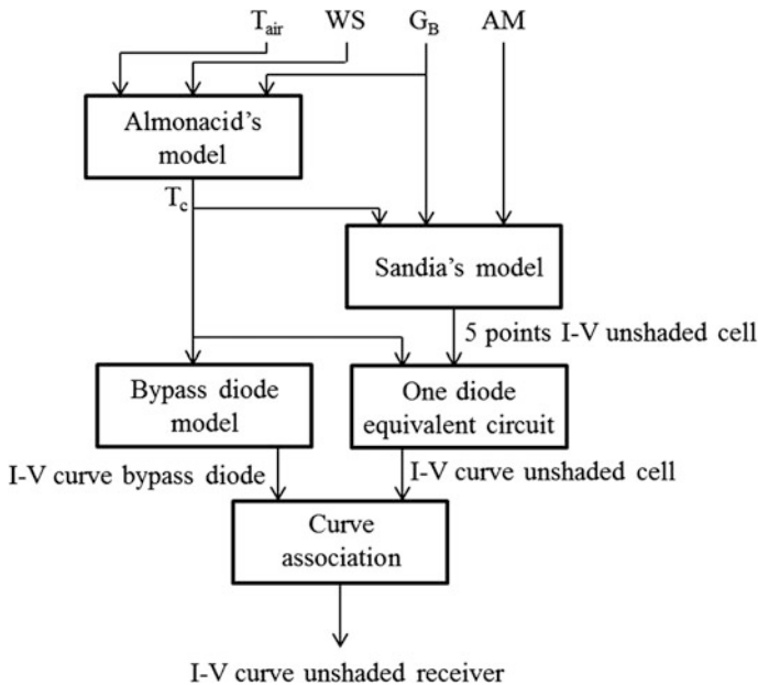
Fig. 12 Scheme of the unshaded receiver block
