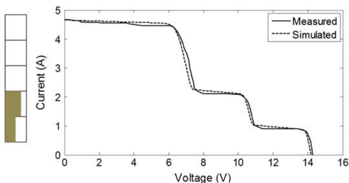
Fig. 15 Example of measured and simulated I–V curves for the module B. The shading pattern for the module is represented at the left side . Module B uses GaInP/GaInAs/Ge solar cells with 625\times concentration factor provided by flat Fresnel lenses
