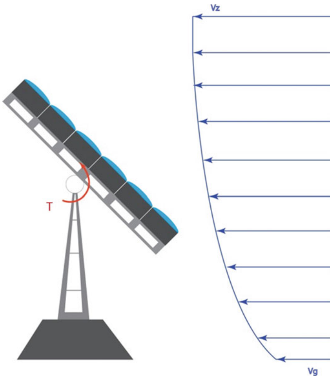
Fig. 13 Torques caused by external aerodynamic forces
