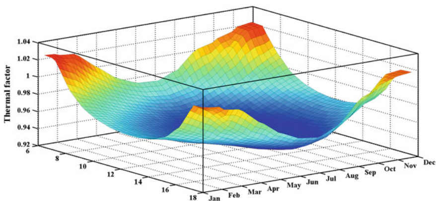
Fig. 10 Simulated annual TF for an LM GaInP/GaInAs/Ge solar cell with an SOG Fresnel lens as primary optics in Granada, southern Spain. The system has a geometric concentration of 700\times , an optical efficiency of 85 %, and a cell efficiency under reference conditions of 38.5 %
