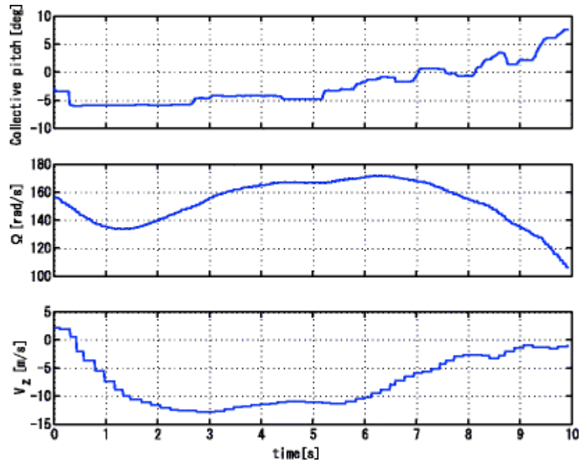
Fig. 6.5 Experimental data of autorotation
