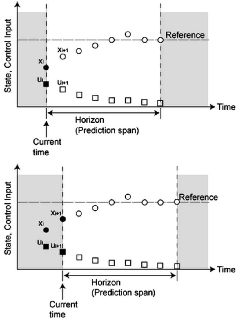
Fig. 9.5 Concept of model predictive control
