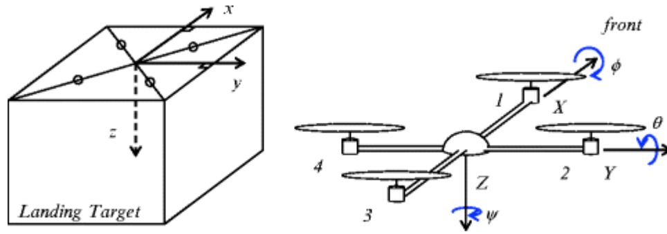
Fig. 13.6 The coordinate system
