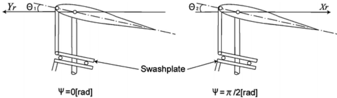
Fig. 5.13 Cyclic pitch angle
