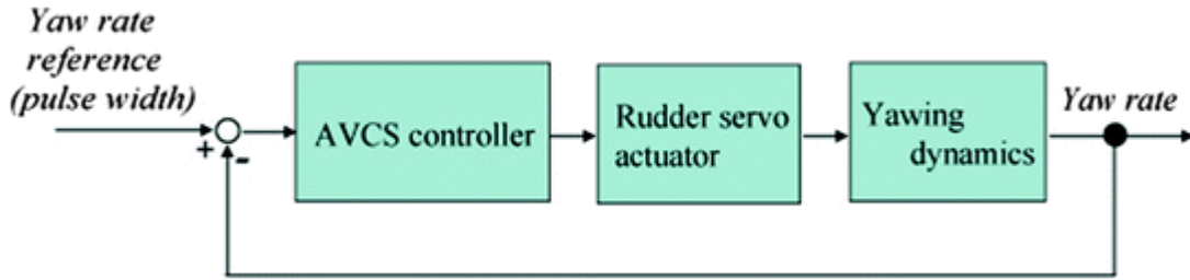
Fig. 2.8 Yawing dynamics with AVCS control system
