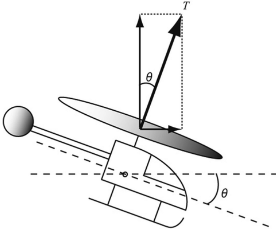
Fig. 2.10 Decomposition of thrust
