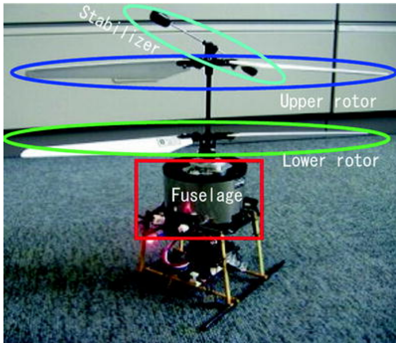
Fig. 2.2 Overview of coaxial-rotor helicopter
