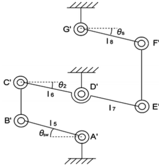
Fig. 5.7 Swashplate to stabilizer link (Link2)
