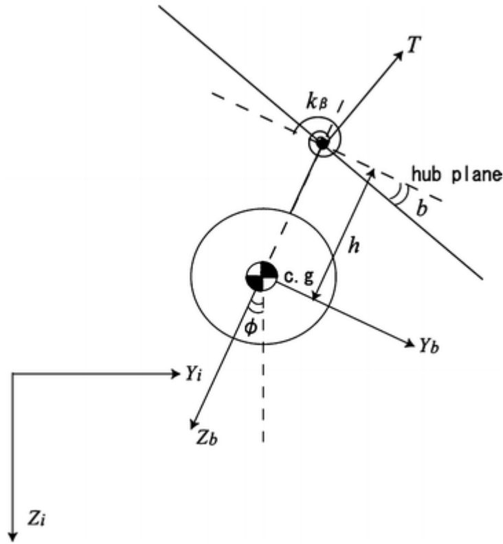
Fig. 5.15 Forces and moments
