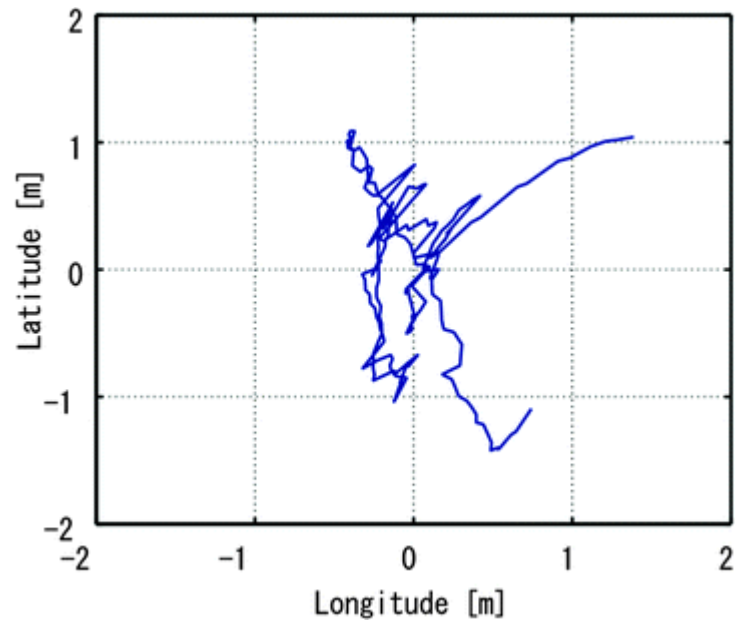
Fig. 5.36 Hovering result of SST-Eagle
