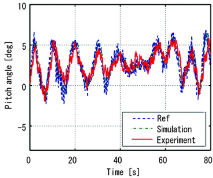
Fig. 5.27 Pitch response of SST-Eagle
