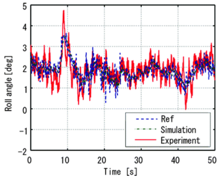
Fig. 5.28 Roll response of SF40
