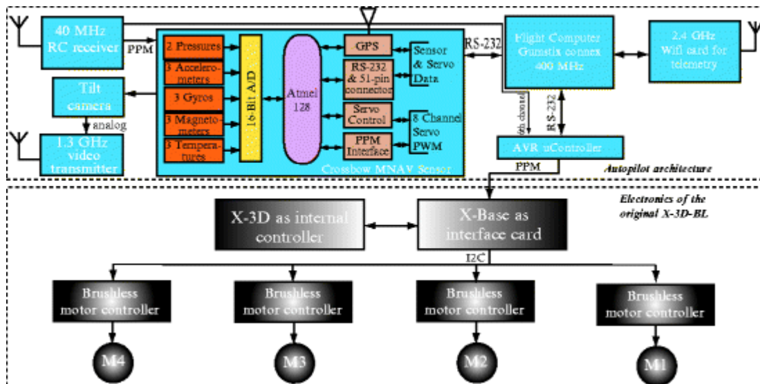
Fig. 8.5 Embedded architecture of the autopilot
