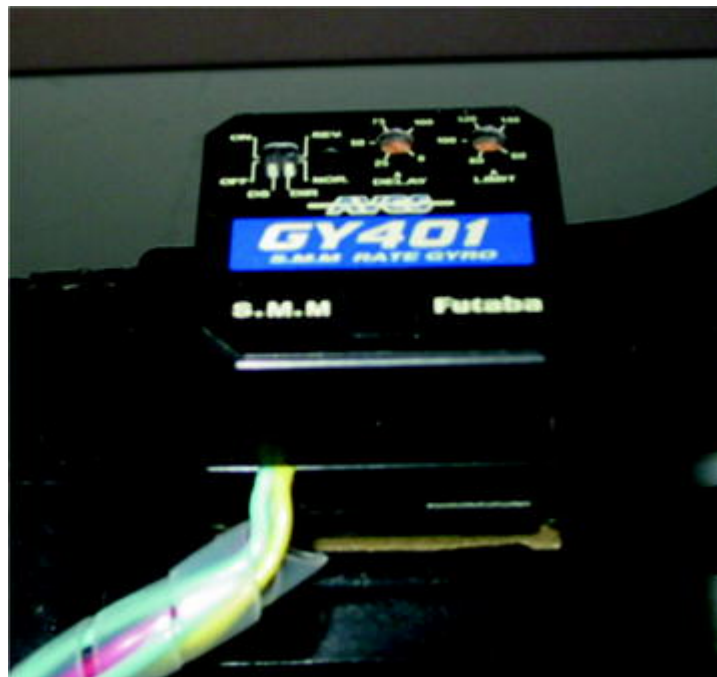
Fig. 4.10 Overview of rate gyro
