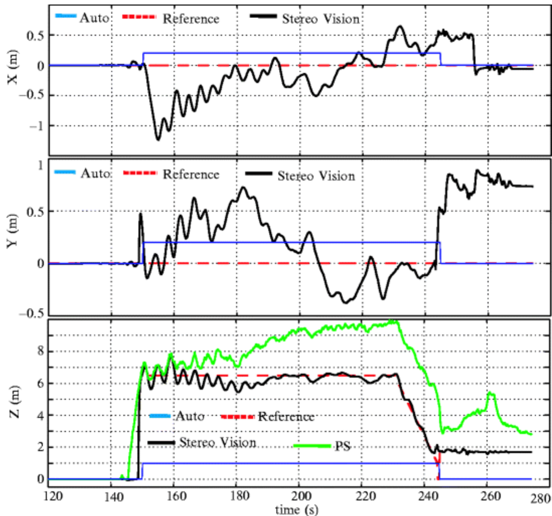
Fig. 10.17 Automatic landing based on stereo vision measurements
