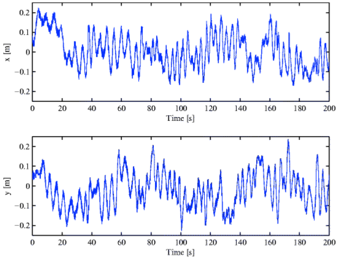
Fig. 13.12 Time variation of the position (raw data)
