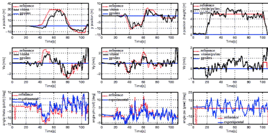
Fig. 12.13 Reference velocity trajectories tracking using optic flow
