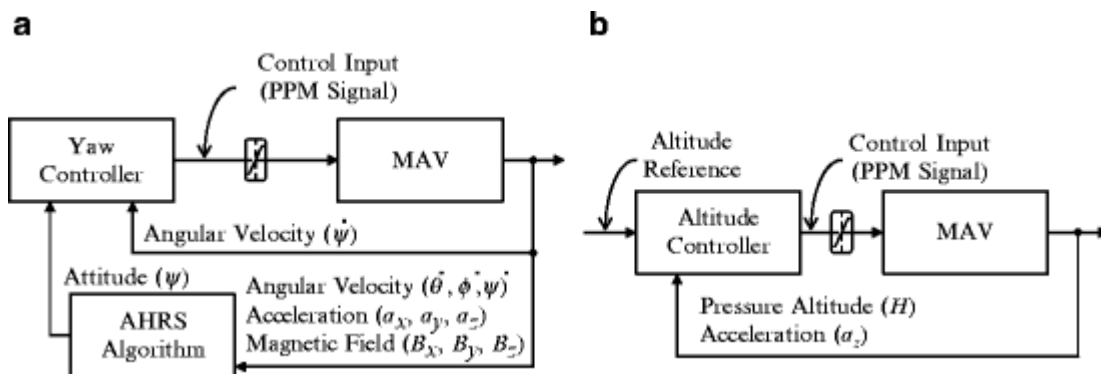
Fig. 13.9 Block diagram: (a) yaw (heading) control loop, (b) z (altitude) control loop
