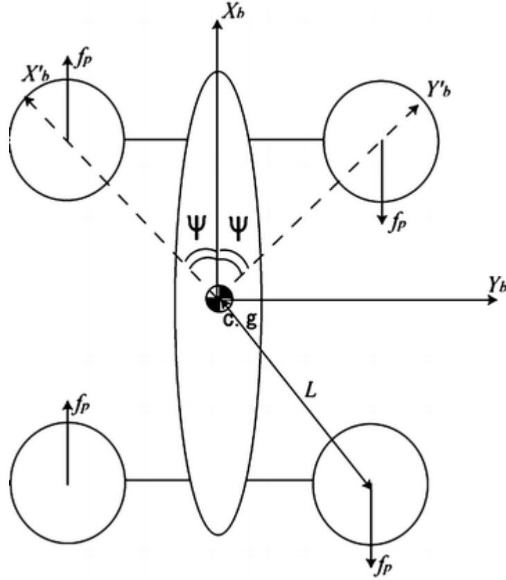
Fig. 4.6 Simplified model of QTW-UAV
