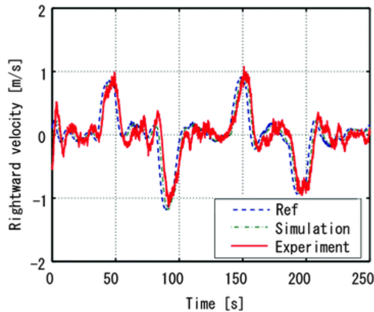
Fig. 5.35 Rightward velocity of SF40
