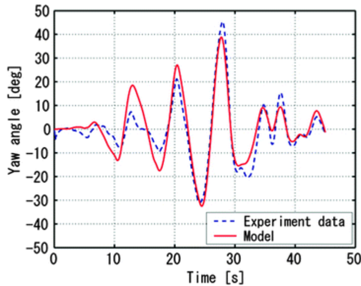
Fig. 4.8 Comparison of yaw angle
