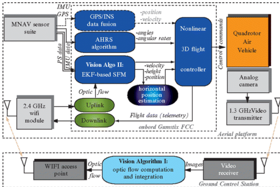
Fig. 10.5 Real-time architecture of the optic flow-based autopilot
