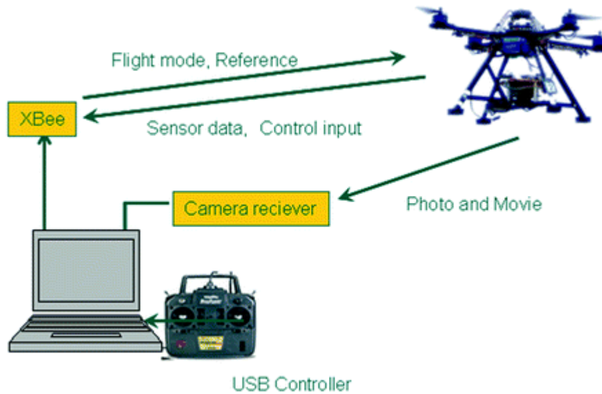
Fig. 3.9 Image of the data transmission
