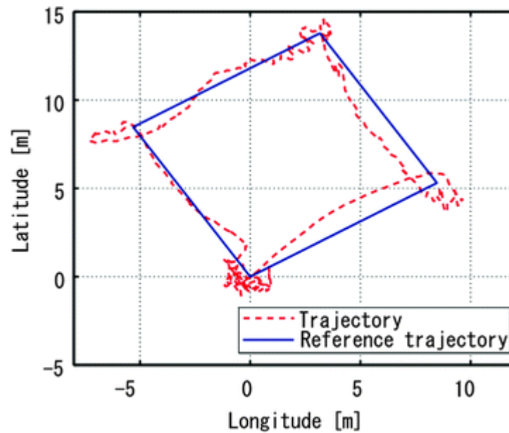
Fig. 5.38 Horizontal movement of S-ST-Eagle
