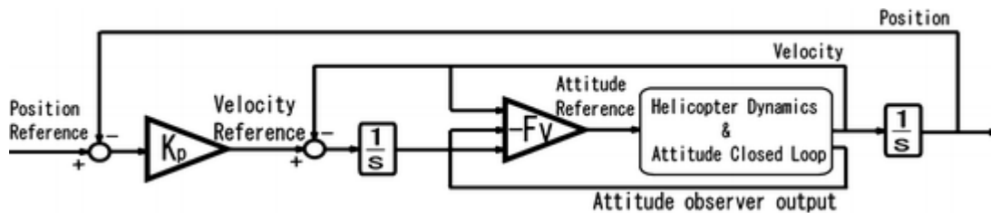
Fig. 5.23 Control System
