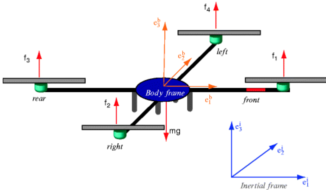
Fig. 8.2 Rigid body dynamics and the associated frames
