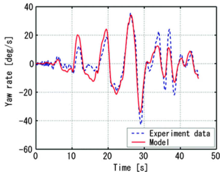
Fig. 4.7 Comparison of yaw rate
