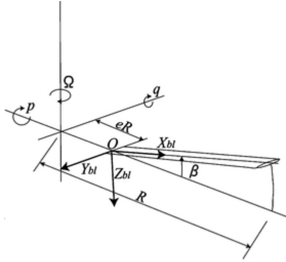
Fig. 5.10 Single flapping blade with body rotation
