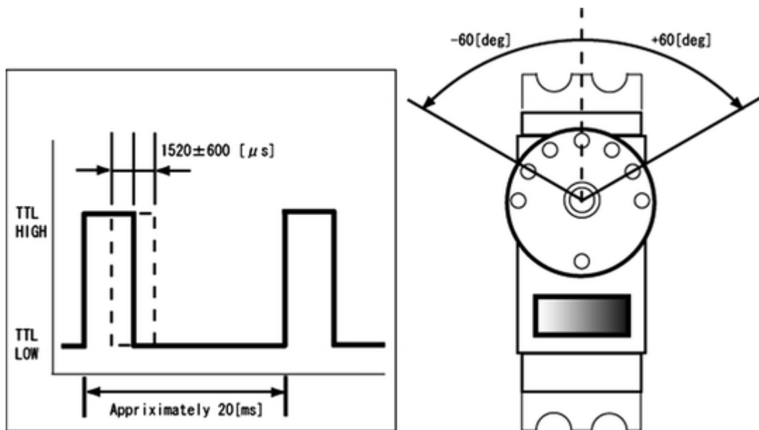
Fig. 2.5 Servomotor actuator
