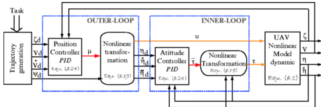
Fig. 8.3 Structure of the inner–outer loop-based controller
