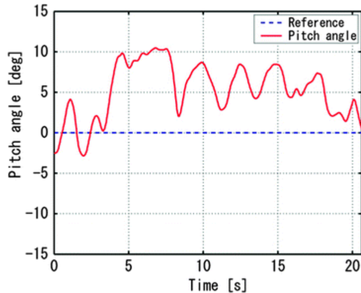
Fig. 4.17 Pitch response (tilt angle = 20^\circ )
