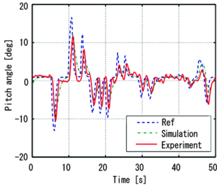
Fig. 5.31 Pitch response of SF125
