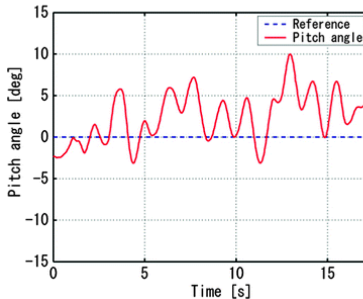
Fig. 4.16 Pitch response (tilt angle = 10^\circ )
