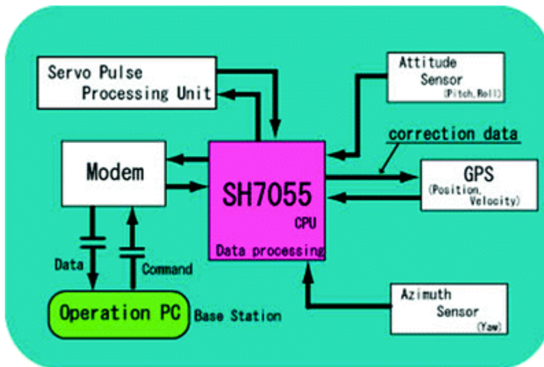
Fig. 2.16 Block diagram of control device
