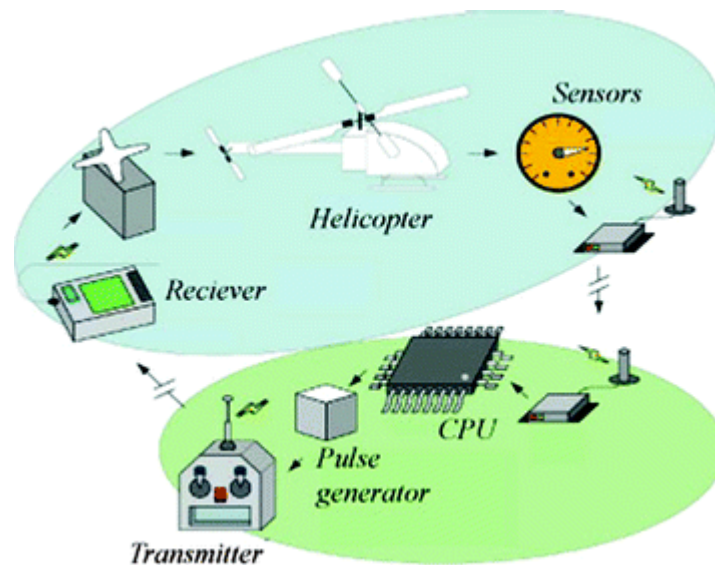
Fig. 2.14 Host-based control system
