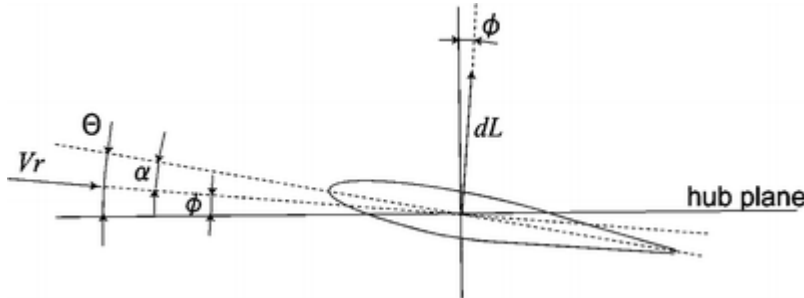
Fig. 5.12 Angle of attack
