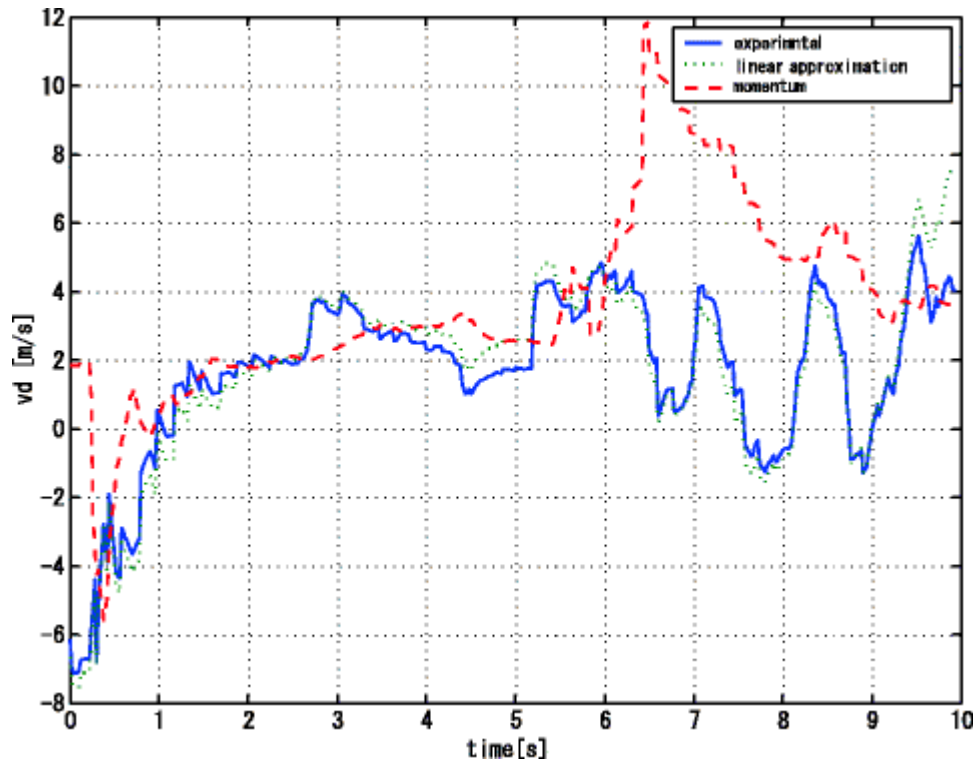
Fig. 6.8 Induced velocity (experimental, approximated, momentum theory)
