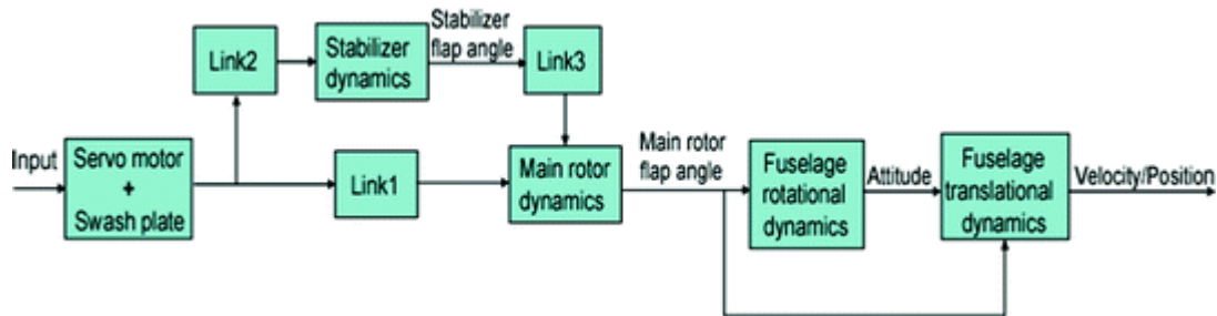
Fig. 5.1 Block diagram of helicopter system
