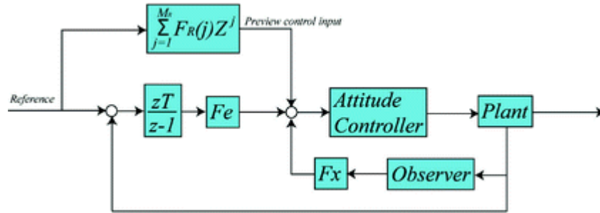
Fig. 2.13 Block diagram of optimal preview control
