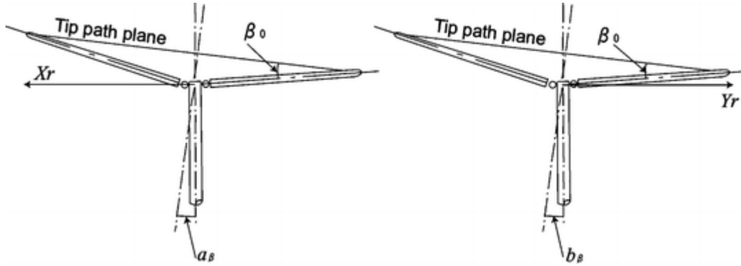
Fig. 5.14 Blade coning
