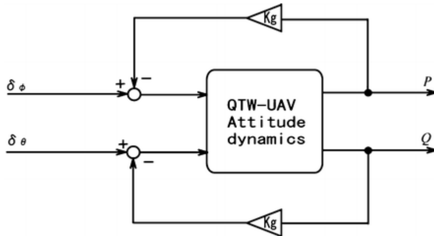
Fig. 4.9 Gyro system
