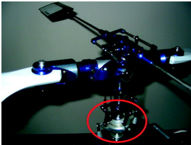
Fig. 2.3 Swash plate of single-rotor helicopter
