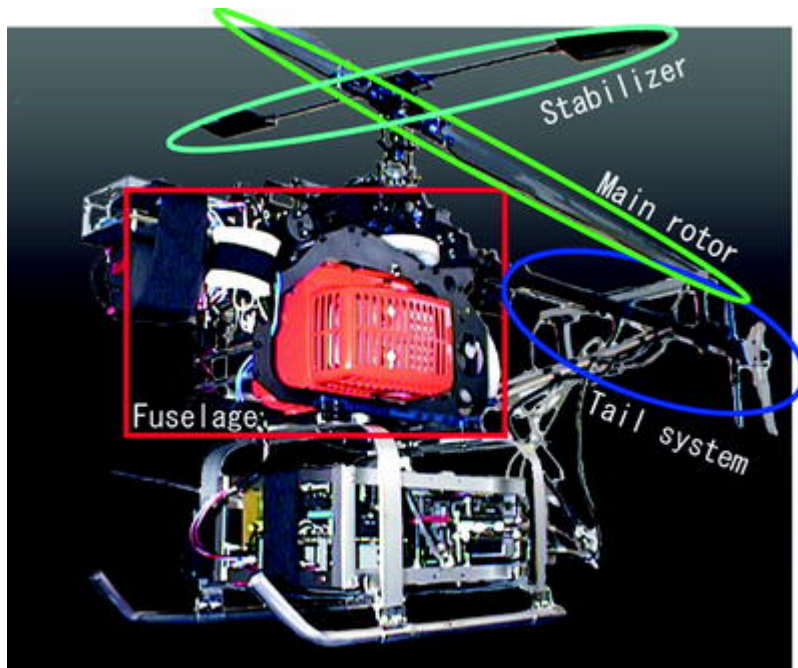
Fig. 2.1 Overview of single-rotor helicopter
