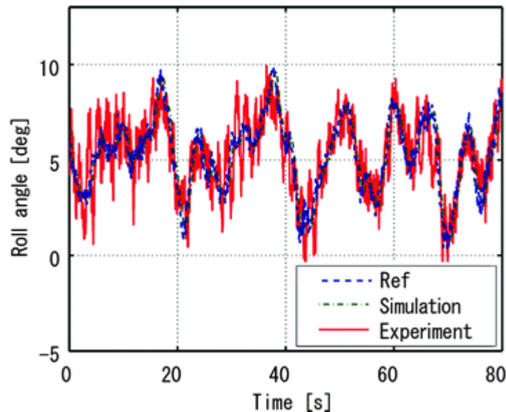
Fig. 5.26 Roll response of SST-Eagle
