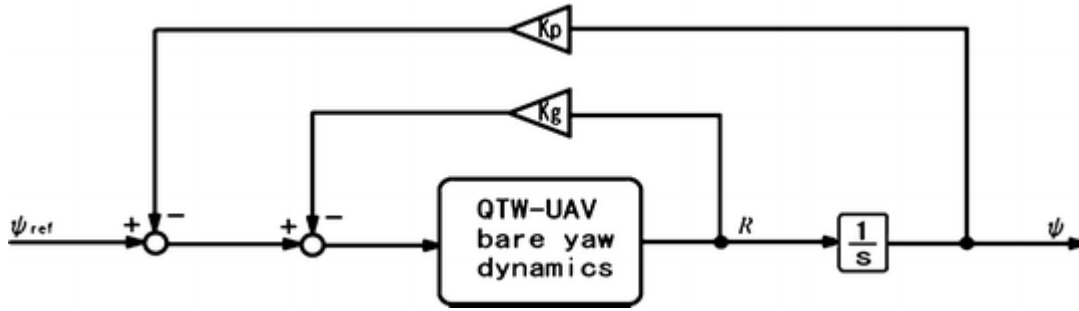
Fig. 4.12 Control system of yaw axis
