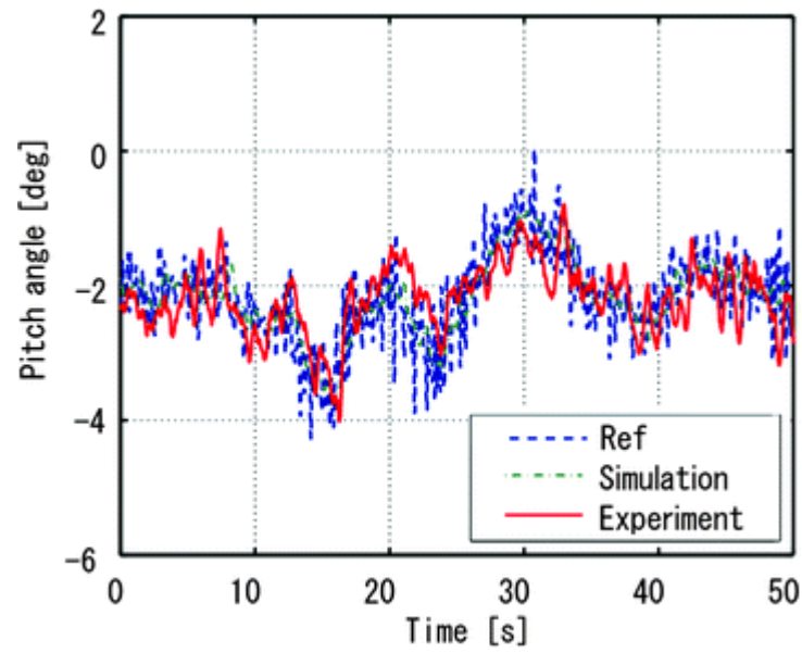
Fig. 5.29 Pitch response of SF40
