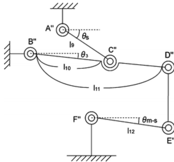
Fig. 5.8 Stabilizer to main rotor link (Link3)
