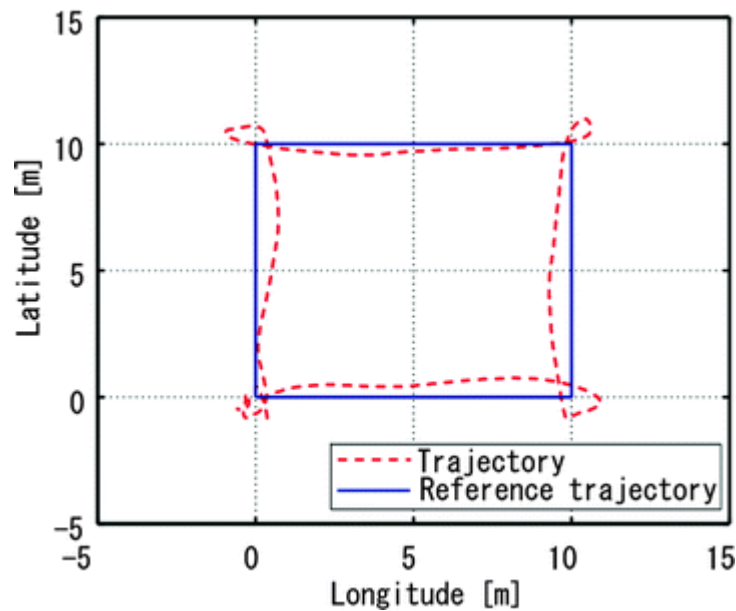
Fig. 5.39 Horizontal movement of SF40
