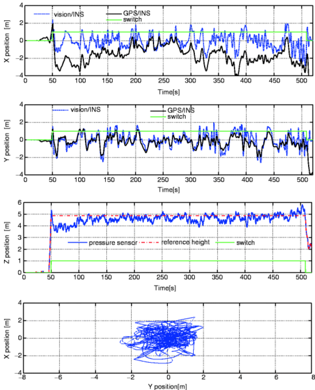
Fig. 10.12 MAV position during vision-based autonomous hovering
