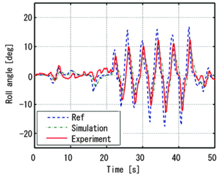
Fig. 5.30 Roll response of SF125
