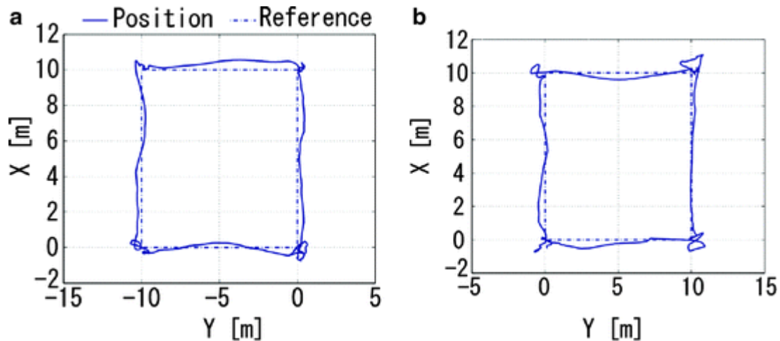
Fig. 9.12 Experimental result of the square trajectory guidance control (a) XY plot (weak windy condition). (b) XY plot (windy condition)
