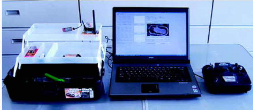
Fig. 3.7 Photo of Ground Control Station (GCS)
