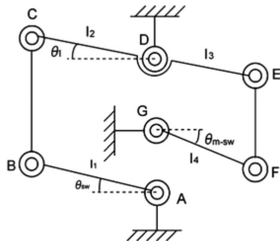
Fig. 5.6 Swashplate to main rotor link (Link1)
