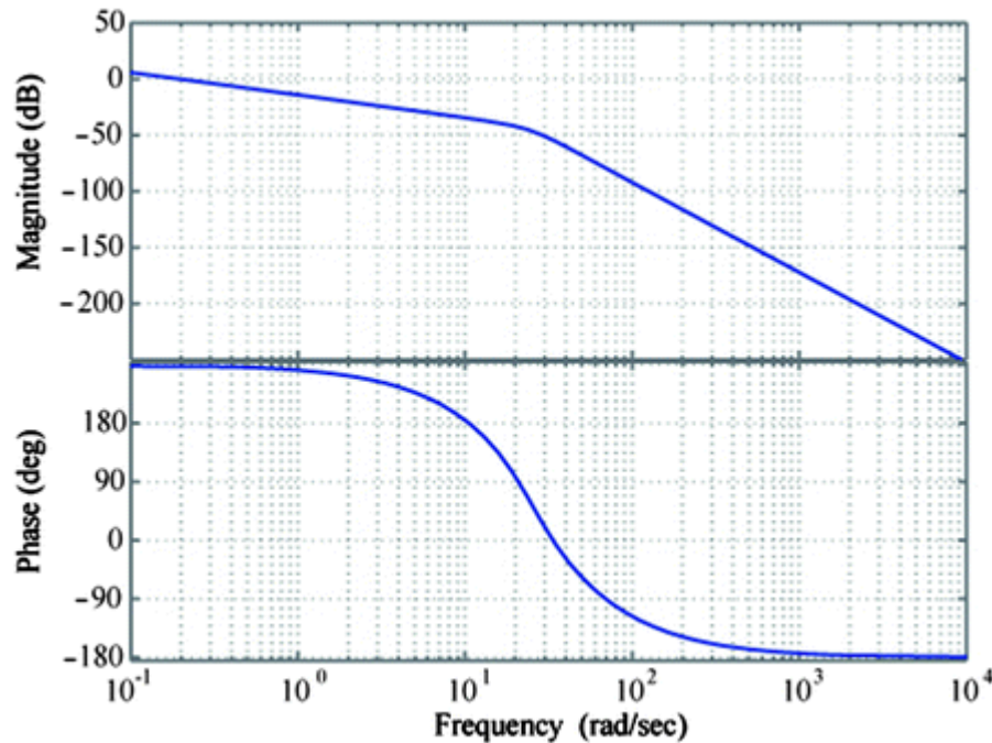
Fig. 2.7 Bode diagram of pitch model
