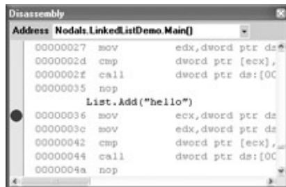
Figure 17-3: The Disassembly window with a breakpoint set
