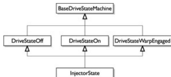
Figure 13-7: The class maintains the current state of the injector at all times by referencing a state object
