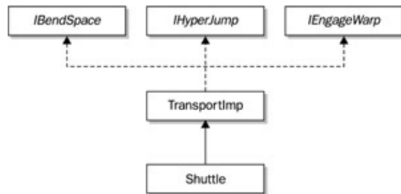
Figure 10-5: Implementing the interface in another class for access by indirection
