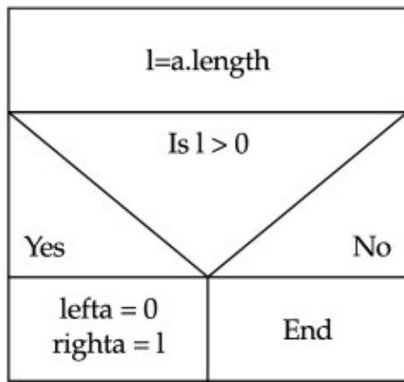
Figure 6-3: NS Chart for designing the process to step through the array
