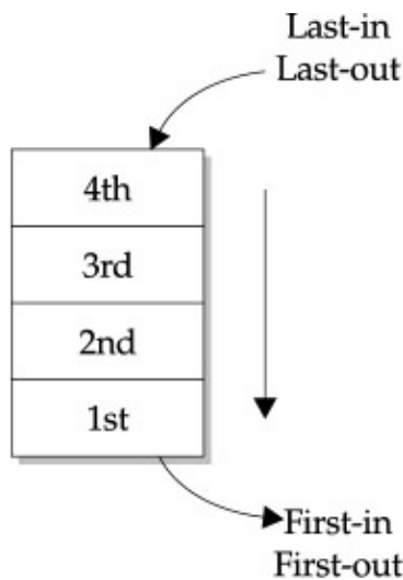
Figure 12-2: Objects in a queue can only be accessed first-in, first-out from the front of the queue. The specification for a queue is one of the easiest specs you'll ever need to prepare. Why? Look around you. From the moment you wake up to the moment you go to bed, you are standing in queues. For example, we have two showers between a three-member family, yet I still have to stand in line every morning just to get five minutes under spray. As soon as the object (me) hits the bathroom, it encounters a queue.
