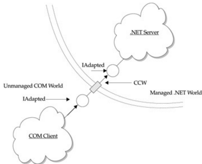
Figure 14–4: Bridging the COM (unmanaged) reality to .NET
