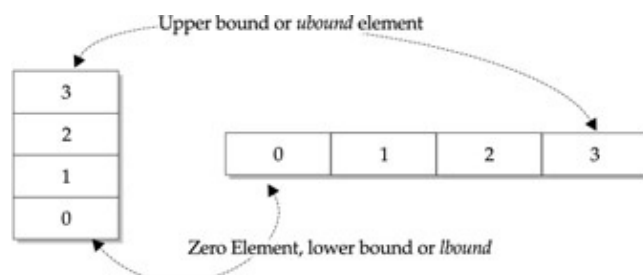
Figure 12–3: A simple one-dimensional array
