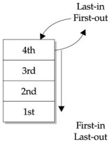
Figure 12-1: Objects on a stack can only be accessed last-in, first-out from the end of the stack. A stack is also known as a push-down store , and the implementation of a stack on a silicon wafer works the same way as stacking waffles on a plate in the kitchen. We take off from the stack the last item we placed onto it; hence, the term "push-down." If you need a waffle or a plate from a stack, you would not pull one out from under the stack; the stack would probably topple.
