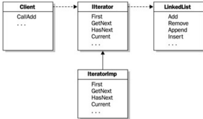
Figure 10–6: The class that instantiates a LinkedList object also instantiates a reference to an Iterator interface in order to access the functionality of the Iterator for the list in question
