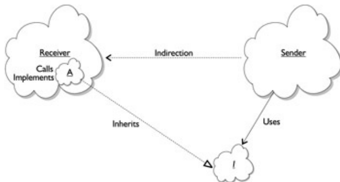
Figure 14-6: The Adapter object is a subclass or inner (composite) class of the Adaptee
