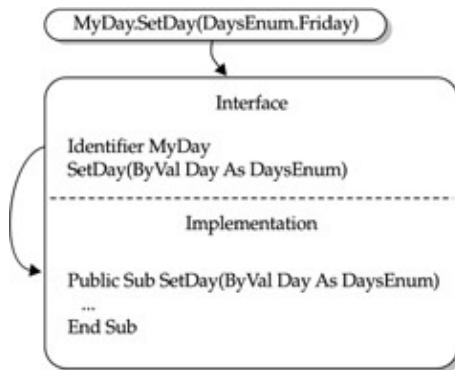
Figure 10–2: The implicit interface and the implementation behind it Visual Basic and all .NET languages implicitly provide the interface for the implementation in standard classes. You might not be thinking about the interface when you create a class and begin coding a method, but you are actually providing an interface on-the-fly. Object Pascal or Delphi source files make you more aware of the interface in every unit. For every class, you must first declare the interface as follows:
