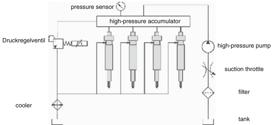
Fig. 4.11 Schematic representation of a common rail system
