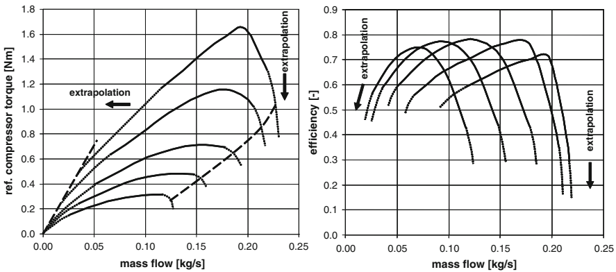
Fig. 8.24 Extrapolation of compressor torque and efficiency along speed lines
