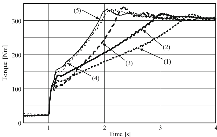
Fig. 10.24 Concept-comparison for a charged four-cylinder engine
