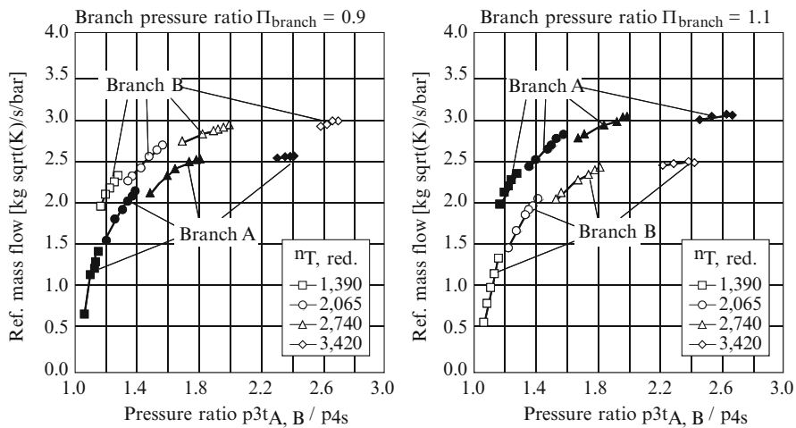
Fig. 8.34 Mass flow map of a twin-scroll turbine for branch pressure ratios 0.9 and 1.1 (Abdel Hamid et al. 2002)
