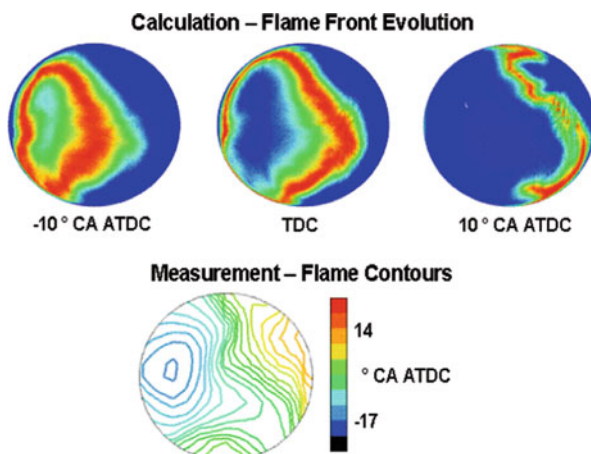
Fig. A.17 Comparison of calculated flame front position in the cylinder head gasket plane of a 2-valve SI-engine with measured flame contours
