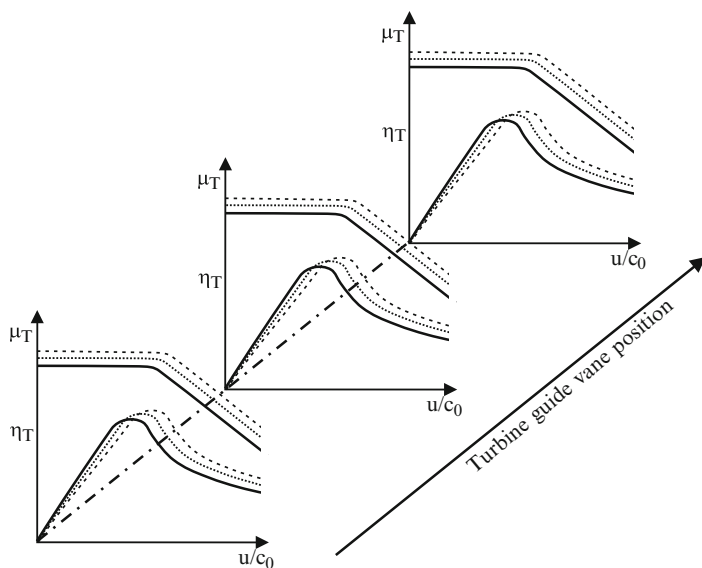
Fig. 8.32 Map of a turbine with an adjustable diffuser
