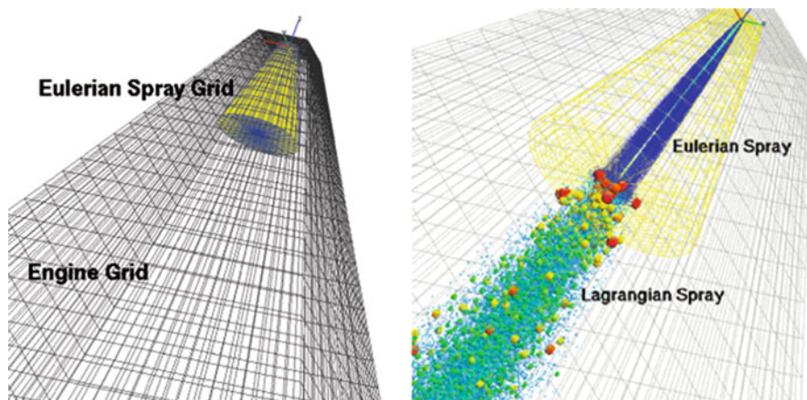
Fig. A.11 Schematics of the embedded grid approach ( left ) and representative result of the ACCI coupled Eulerian/Lagrangian spray treatment ( right ) (Edelbauer et al. 2006)
