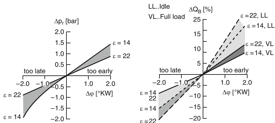
Fig. 3.24 Influence of angle error on the energy balance ( left ) and the friction mean pressure ( right ) (diesel engine)
