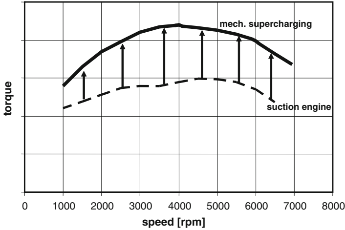
Fig. 8.7 Torque profile of a mechanically charged SI engine
