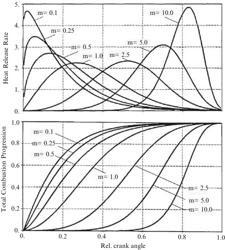
Fig. 7.12 Vibe substitute heat release rate for different Vibe shape coefficients
