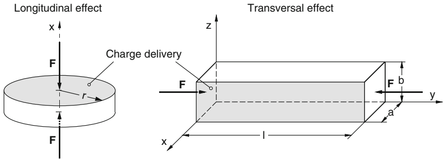
Fig. 3.4 Measuring elements for the longitudinal and transversal effect
