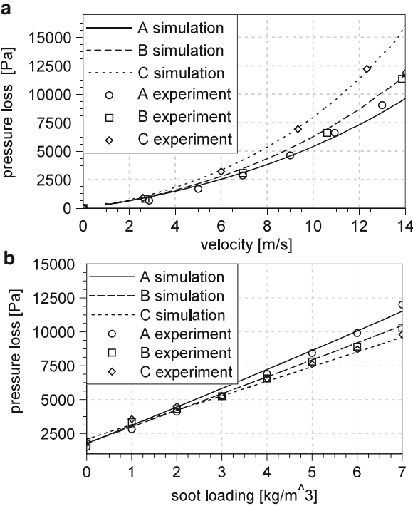
Fig. 9.9 Pressure loss for diesel particulate filters with different channel diameter ratios (inlet/outlet: A > B > C ) measured and calculated for empty filters ( top ) and for loaded filters ( bottom ). (calculations from Wurzenberger and Kutschi 2007, measurements according to Ogyu et al. 2004)
