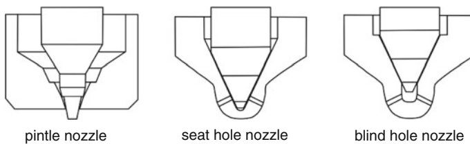
Fig. 4.14 Injection nozzle designs
