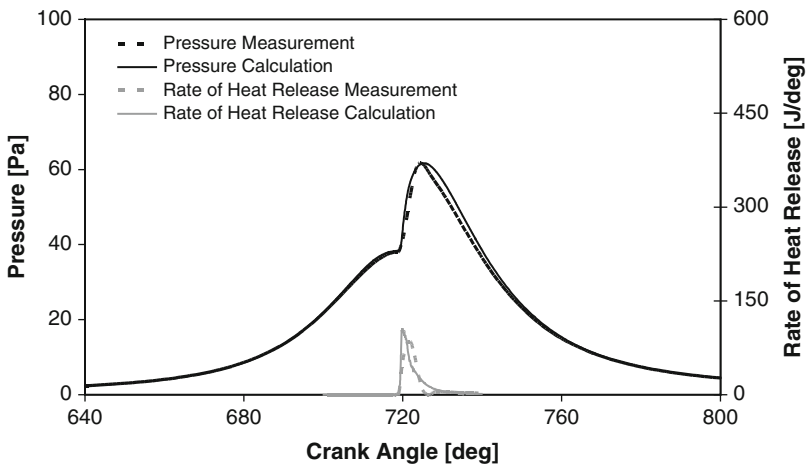
Fig. A.15 Comparison of calculated and measured cylinder pressure evolution and heat release rate for HCCI-type diesel combustion (Priesching et al. 2007)
