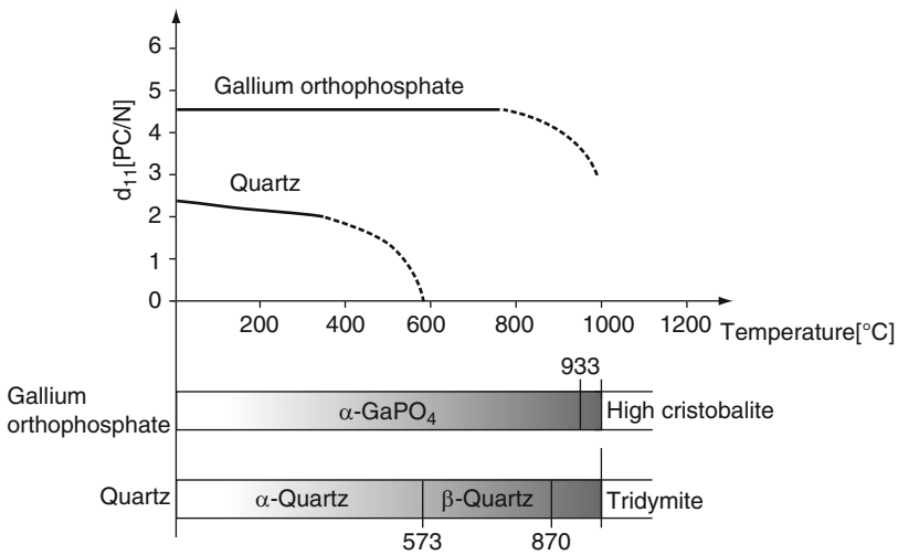
Fig. 3.8 Temperature dependence of the piezoelectric constant d_{11} for quartz and gallium orthophosphate
