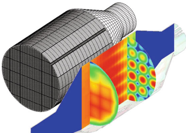
Fig. 9.11 Temperature distribution during the regeneration of a segmented SiC filter
