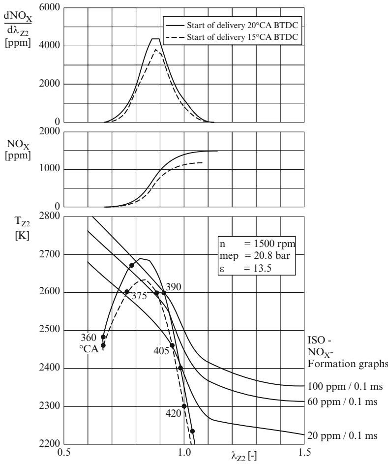
Fig. 7.21 Start of delivery variation, acc. to Hohlbaum (1992)
