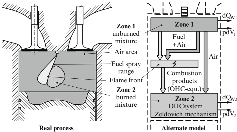
Fig. 7.18 Two-zone model for diesel combustion
