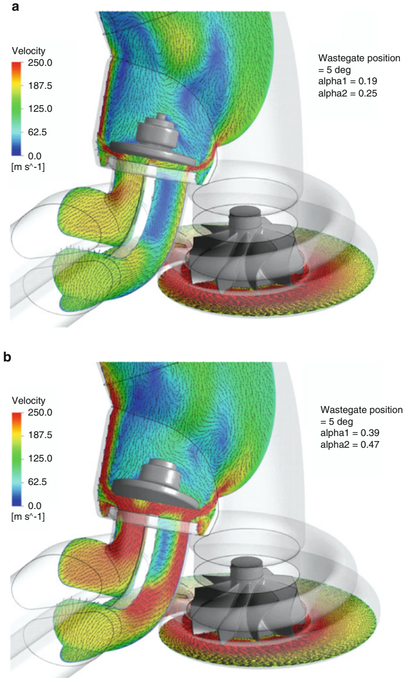
Fig. 15.14 Flow around the wastegate flap of a twin scroll turbine. (a) aperture angle 15°. (b) aperture angle 5°
