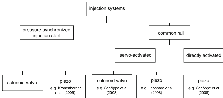
Fig. 4.9 Classification of current injection systems for passenger cars
