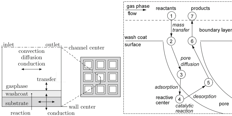
Fig. 9.1 Effects with one single channel of a honeycomb type catalytic converter and schematic of a heterogeneous catalytic reaction ( left figure taken from Wurzenberger and Peters 2003, right figure taken from Hayes and Kolaczowski 1997)
