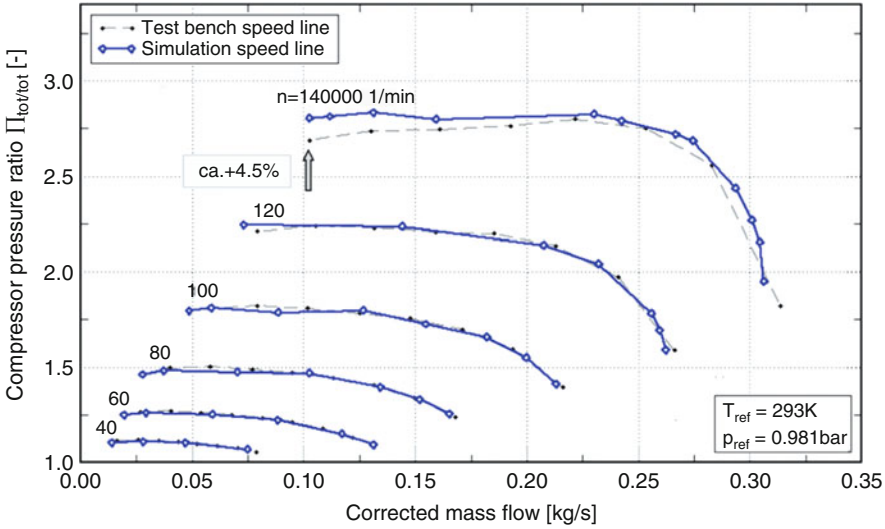
Fig. 15.12 Comparison of calculated and measured compressor map
