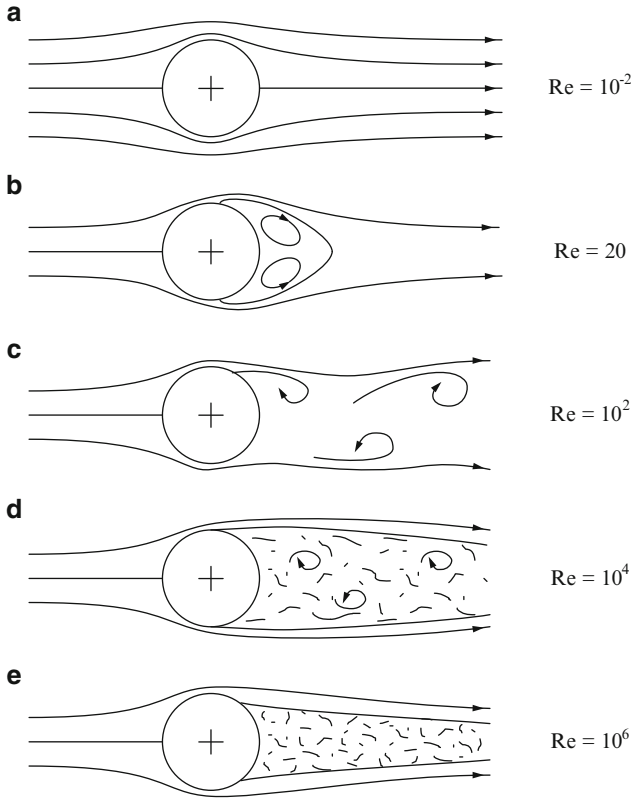
Fig. 12.1 Kármán vortex street (flow over a cylinder) at varying Reynolds' numbers
