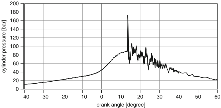
Fig. 4.30 Example of a strongly knocking combustion
