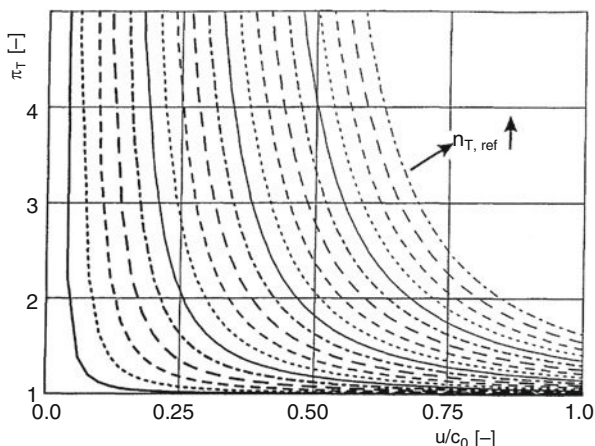
Fig. 8.29 Relation of the referenced turbine speed, blade speed ratio and turbine pressure ratio
