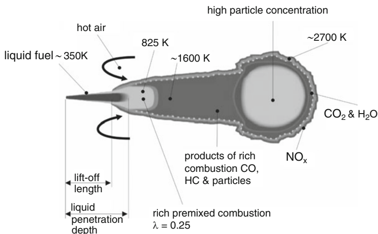
Fig. 4.21 Conceptional model of diesel combustion, acc. to Dec (1997) and Flynn et al. (1999)
