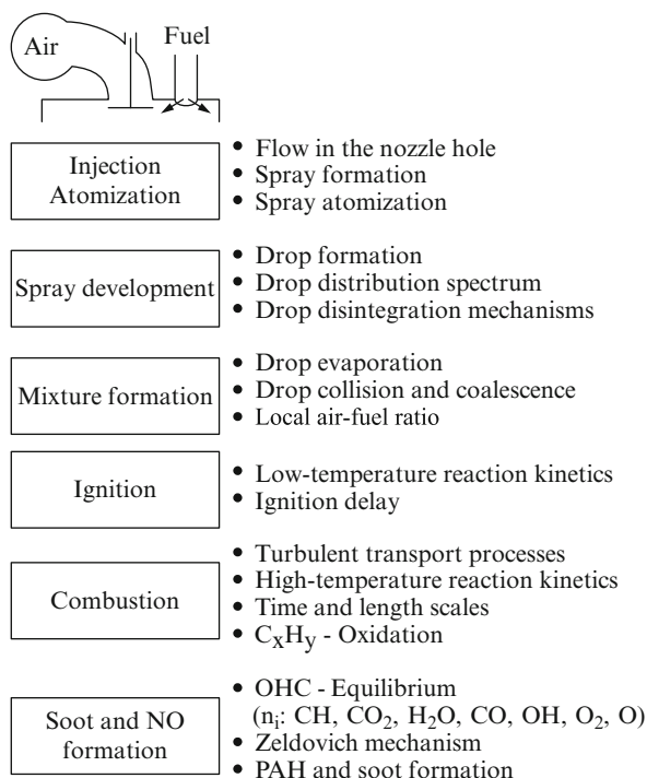
Fig. 4.8 Subprocesses of mixture formation and combustion in diesel engines
