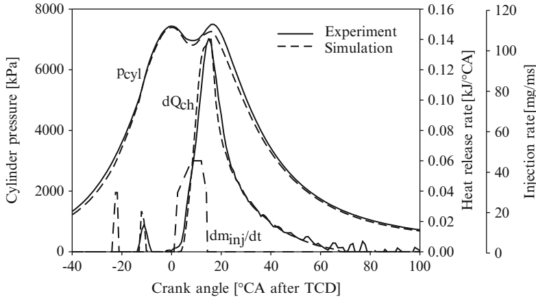
Fig. 11.11 Calculated and measured heat release rate and pressure progressions of a truck diesel engine with pilot injection, Thoma et al. (2002)
