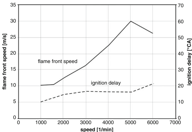
Fig. 4.28 Example measurement of a SI engine with tumble ducts to determine the flame front speed at the spark plug along the full load line
