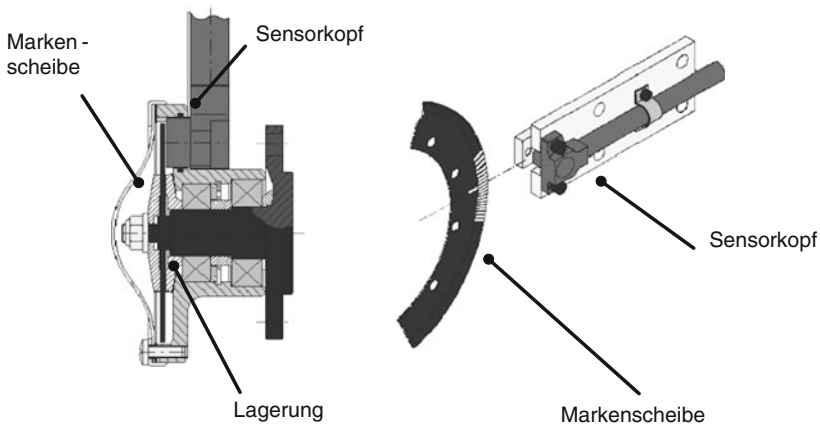
Fig. 3.23 Examples of angle sensor designs (AVL)
