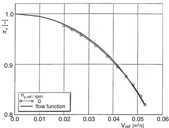
Fig. 8.25 Comparison of the zero speed line and the flow function
