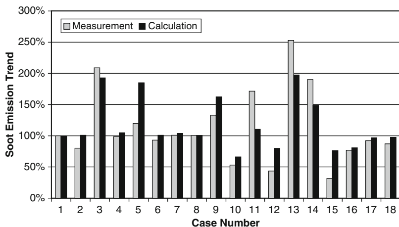
Fig. A.23 Comparison of calculated and measured soot emission trends in a DI diesel engine for combustion system parameter variations (Priesching et al. 2007)
