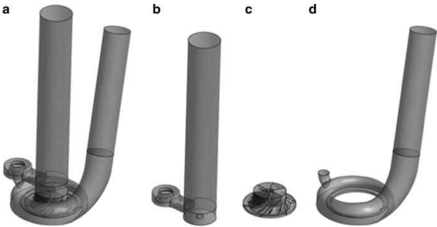
Fig. 15.4 Subdivision of compressor geometry into different subareas. (a) overall model; (b) casing in; (c) impeller; (d) casing out
