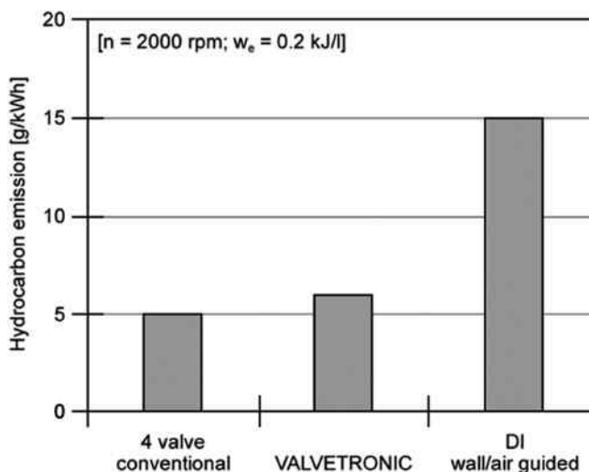
Fig. 4.38 Increasing the HC mass flow at operating point 2,000 rpm, w_e = 0.2 kJ/l in the wall-guided process compared to stoichiometrically operated engines, Göschel (2006)
