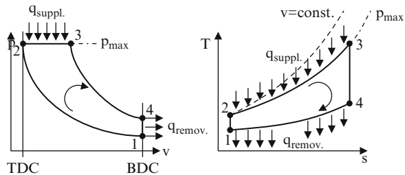
Fig. 2.16 The constant-pressure cycle in the p, v and T, s diagram
