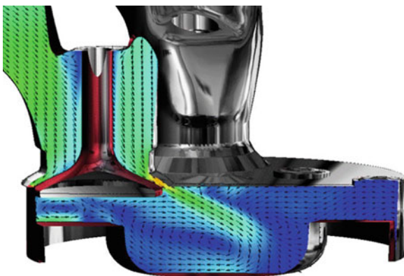
Fig. A.5 Flow velocities and turbulence intensity distribution during the intake stroke of a DI diesel engine
