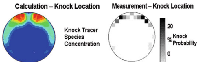
Fig. A.19 Calculated knock onset locations ( left ) vs. experimentally obtained knock probability distribution ( right ) in the cylinder head gasket plane of a 4V SI-engine (Tatschl et al. 2005)
