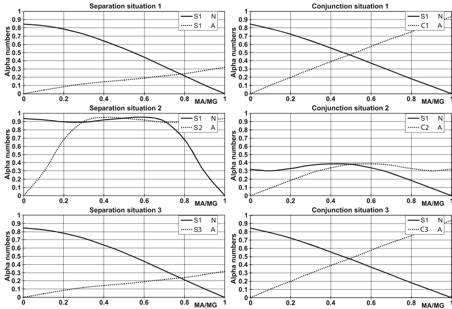
Fig. 7.34 Flow coefficients at a pipe branching
