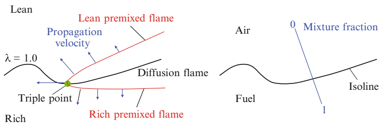
Fig. 14.14 Structure of a triple flame
