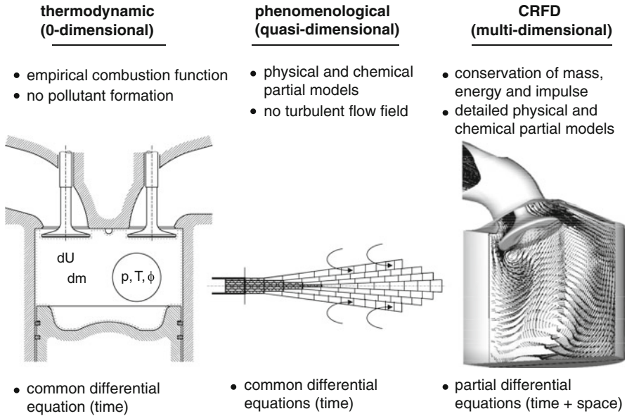
Fig. 11.1 Classification of combustion models
