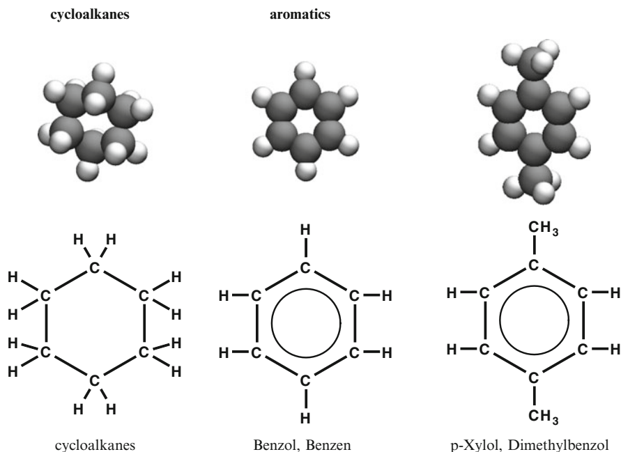
Fig. 4.2 Structural formulae and graphic representation of alicyclic and aromatic hydrocarbons
