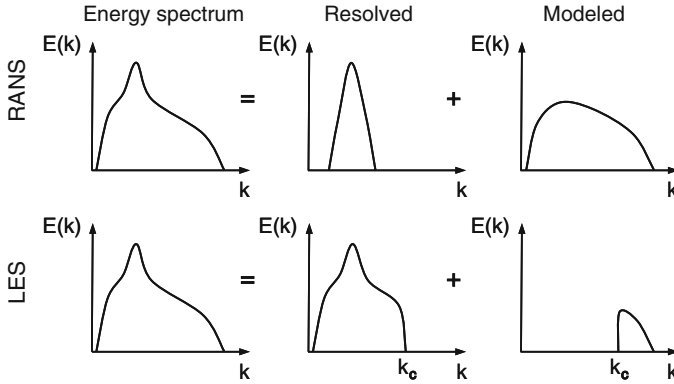
Fig. 12.4 While in Reynolds-averaged turbulence models like the k - \epsilon -model, only a narrow range of the energy spectrum is resolved, LES resolves the entire spectrum until filter width k_c (Angelberger 2007)
