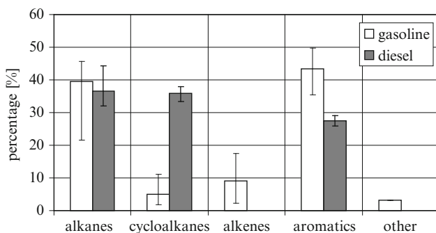
Fig. 4.4 Composition of diesel and gasoline acc. to DGMK (2002, 2003)
