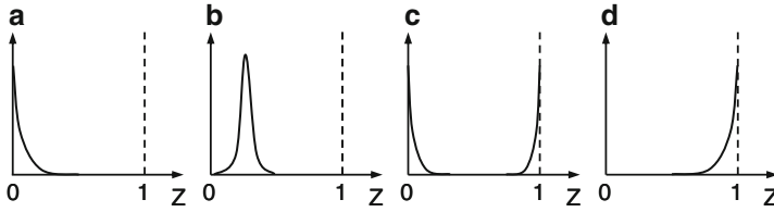
Fig. 12.2 Distribution functions for different mixture conditions: (c) describes a slightly mixed and (b) a heavily mixed state. (a) and (d) are the results of a very small/very large average value
