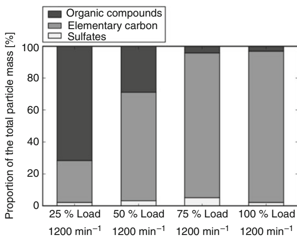
Fig. 6.14 Composition of diesel particles, Kweon et al. (2002)
