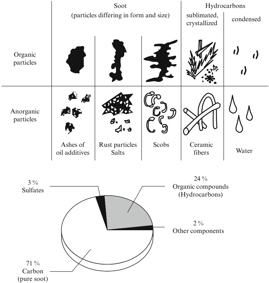
Fig. 6.13 Various components in particle emissions
