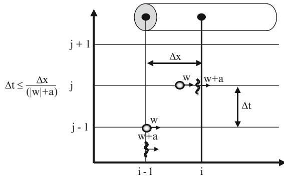
Fig. 7.35 Courant Friedrichs Levy stability criterium
