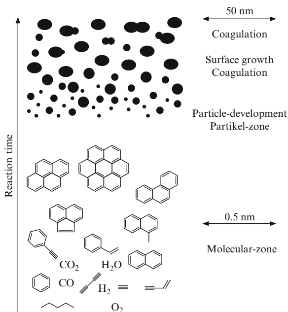
Fig. 6.15 Schematic diagram of soot formation, acc. to Bockhorn (1994)
