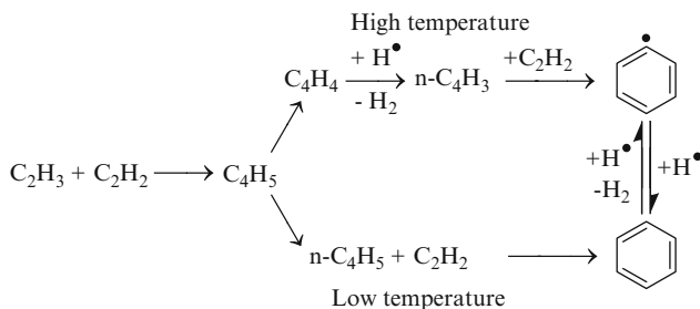
Fig. 6.16 Reaction path in the formation of benzene rings, acc. to Frenklach and Wang (1994)
