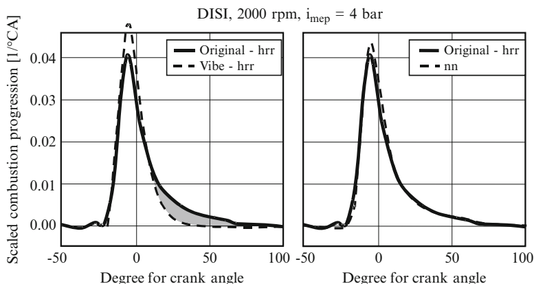
Fig. 7.14 Heat release rate for a DISI engine at n = 2.000 \text{ min}^{-1} and i_{mep} = 4 \text{ bar} . Comparison of the original heat release rate with the Vibe heat release rate ( left ) and with the neural network heat release rate ( right )
