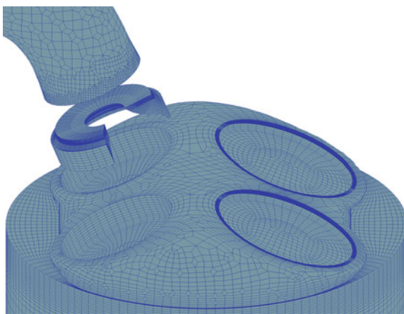
Fig. A.1 Computational mesh of an SI-engine configuration composed of a set of sub-domain meshes for the intake ports, valve seats and combustion chamber
