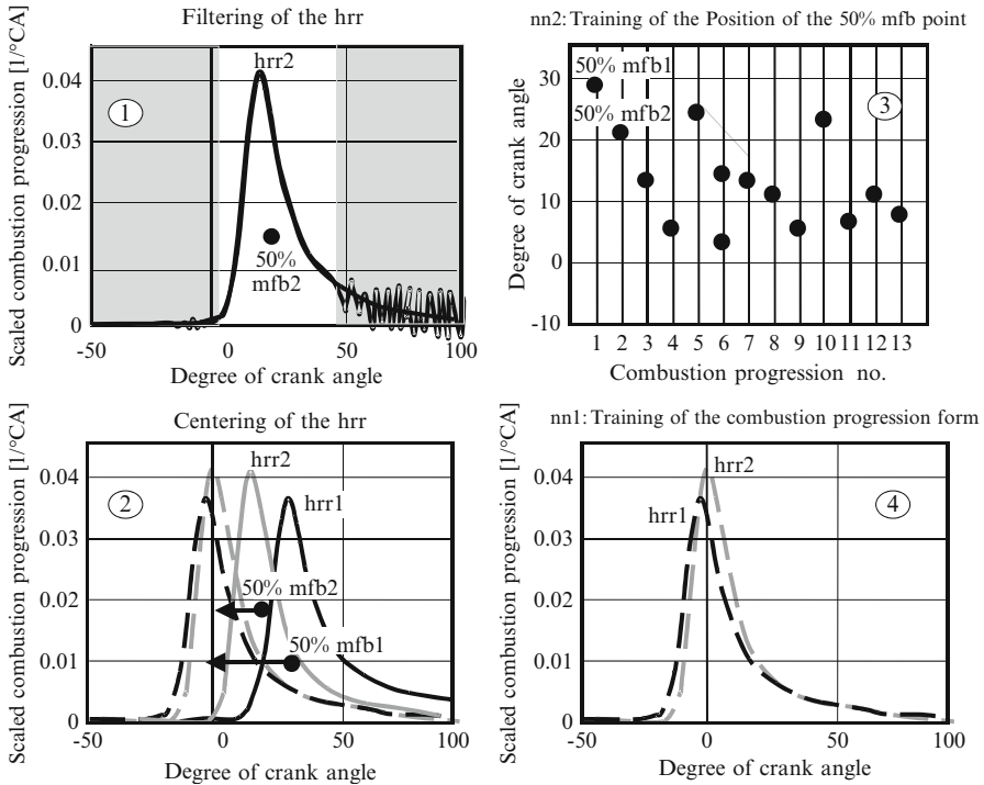
Fig. 7.15 Net training procedure
