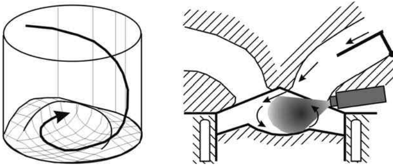
Fig. 4.26 Basic forms of global charge motion: swirl ( left ) as a swirling motion around the vertical axis of the cylinder, here in conjunction with a recessed-head type piston of a wall guided SI/DI process (Holy et al. (1998)). Tumble ( right ) as a swirling motion around the transverse axis of the cylinder, shown here with the help of a tumble valve (Grigo and Wolters 1998)
