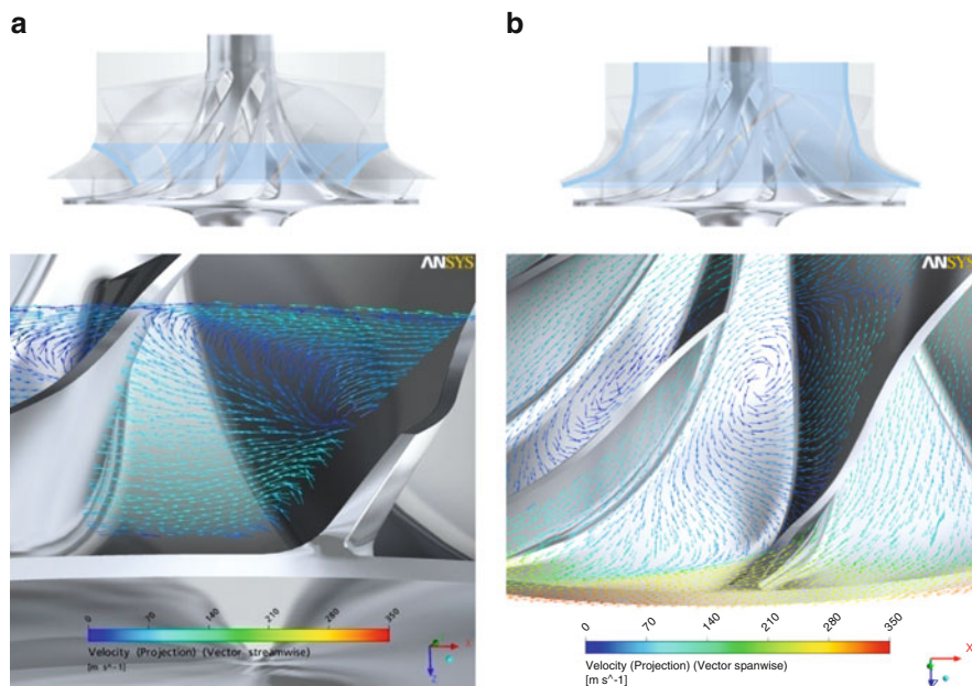
Fig. 15.9 Vector plot on curved surfaces. (a) constant in the span direction; (b) constant in the flow direction
