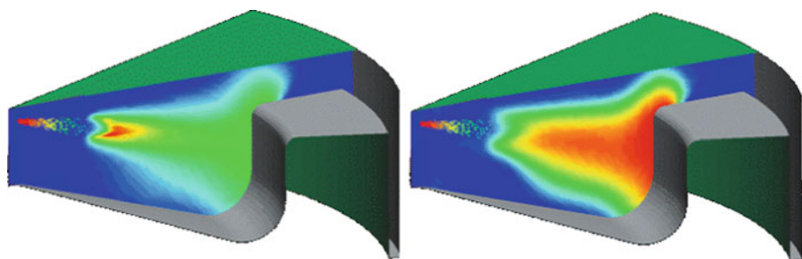
Fig. A.22 Fuel vapor ( left ) and soot concentration ( right ) in a DI diesel engine at 20° crank-angle ATDC
