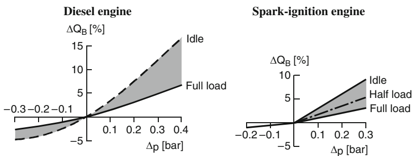
Fig. 3.20 Effect of a zero-point error on the energy balance
