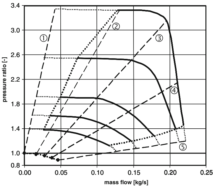
Fig. 8.26 Fan-shaped support lines for compressor extrapolation
