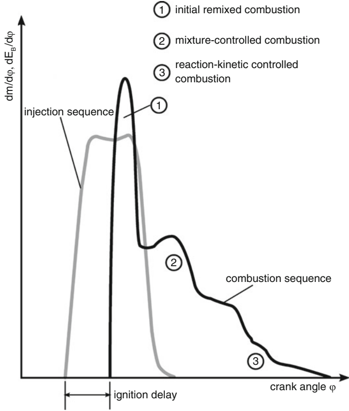
Fig. 4.19 Injection and combustion sequence in a diesel engine
