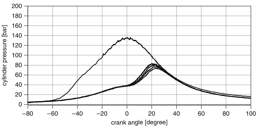
Fig. 4.32 Example of a pressure profile of a fully developed glow ignition without knocking on one cylinder
