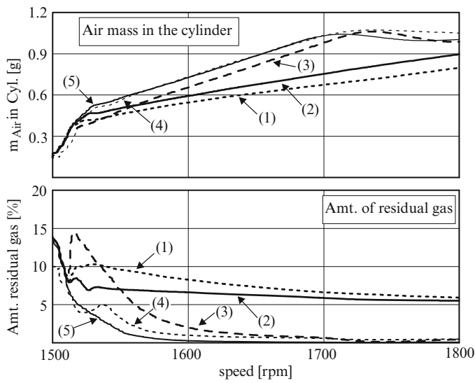
Fig. 10.25 Amounts of fresh and residual gas for different charging concepts
