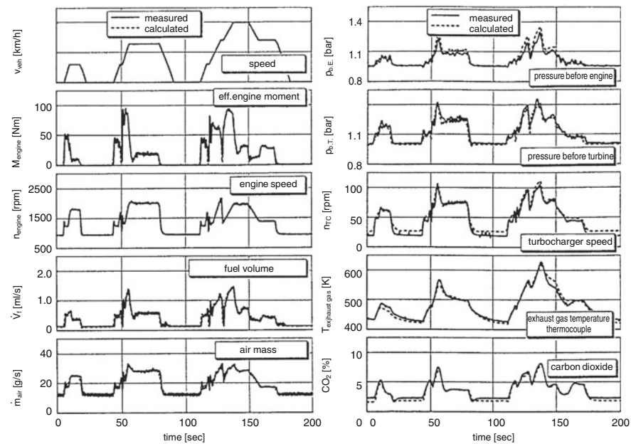
Fig. 10.21 Part of the ECE test cycle
