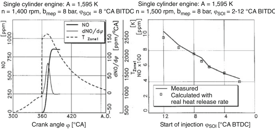
Fig. 7.22 Influence of start of injection on the NO formation rate
