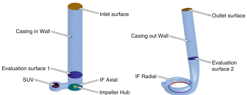
Fig. 15.5 Boundary and edge surfaces of compressor housing
