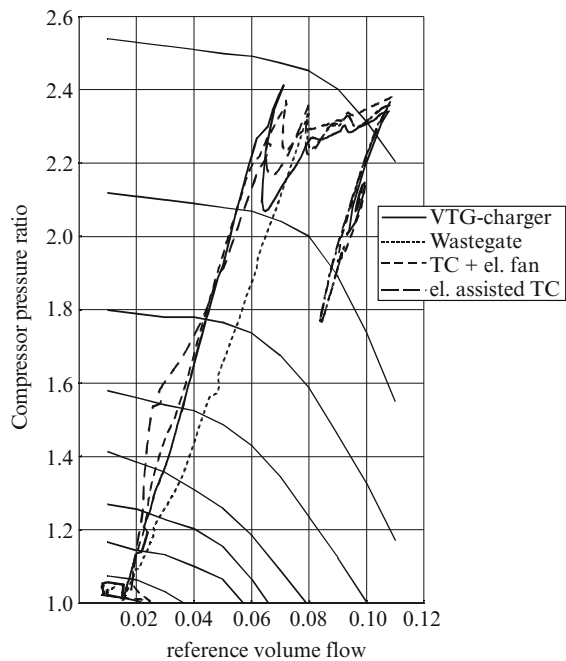
Fig. 10.20 Operating lines in the compressor map
