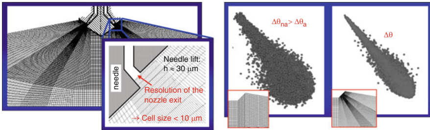
Fig. 13.6 Adaptively refined mesh with nozzle hole resolution for an SI engine with piezo-activated A-nozzle. The spray calculated with it is shown right. An excessively coarse mesh structure creates sprays that are much too bushy (center image)
