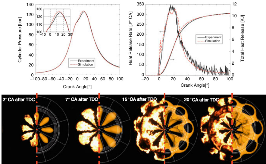
Fig. 14.4 Simulation of the combustion of a commercial vehicle Diesel engine with the pdf time-scale model. (a) Comparison of experimental and calculated pressure paths (b) Comparison of temperature-isosurface (simulation) with film shot from transparent engine (left)
