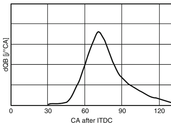
Fig. 4.42 Example of a heat release rate during catalytic converter heating with double injection (EOI2 = ignition angle = 30° after TDC, spray-guided combustion), Preuss (2003)
