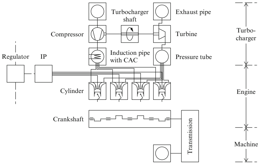
Fig. 7.1 Engine model
