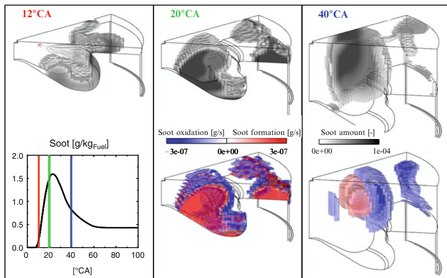
Fig. 14.6 3D simulation of soot distribution in a passenger car Diesel engine with the flamelet concept in different phases of combustion
