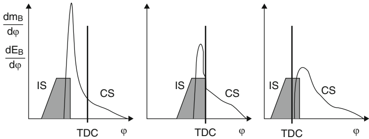
Fig. 4.20 Injection rate (IR) and heat release rate (HRR) with early ( left ) and late ( right ) combustion
