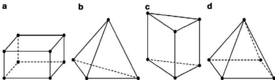
Fig. 15.3 Overview of typical element types for 3D CFD control volumes. (a) hexahedron; (b) tetrahedron; (c) prism; (d) pyramid
