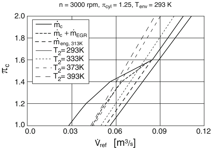
Fig. 10.14 Differences between engine and compressor suction lines under exhaust gas recirculation conditions
