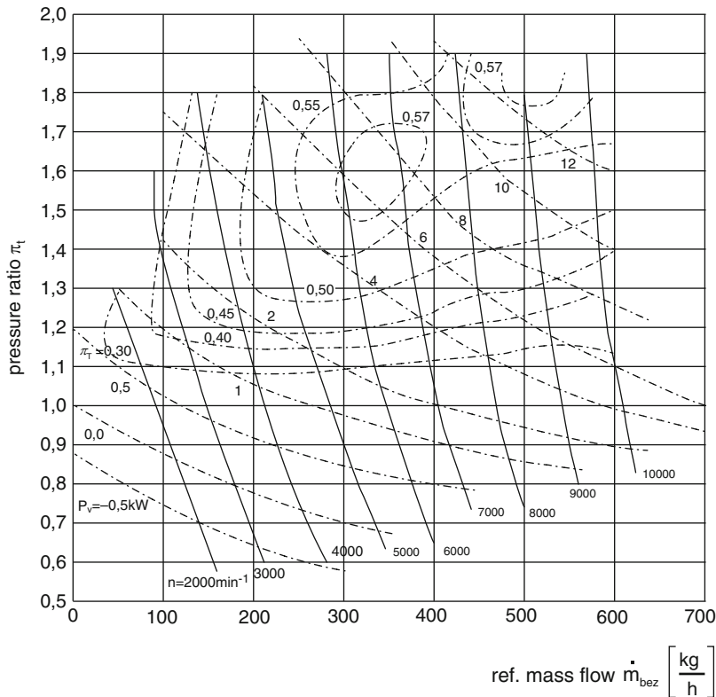
Fig. 8.28 Extrapolation at the positive displacement charger
