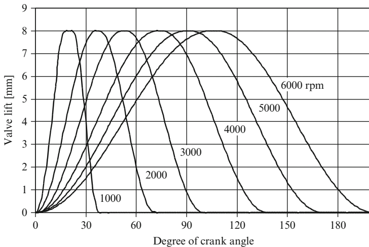
Fig. 7.6 Valve lift curves for an electromechanical valve train
