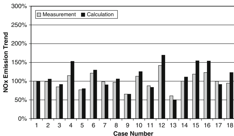
Fig. A.21 Comparison of calculated and measured NO emission trends in a DI diesel engine for combustion system parameter variations (Priesching et al. 2007)
