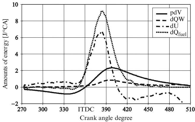
Fig. 3.31 Pressure profile and heat release rate for a SI engine at 1,000 rpm and i_{mep} = 1 bar
