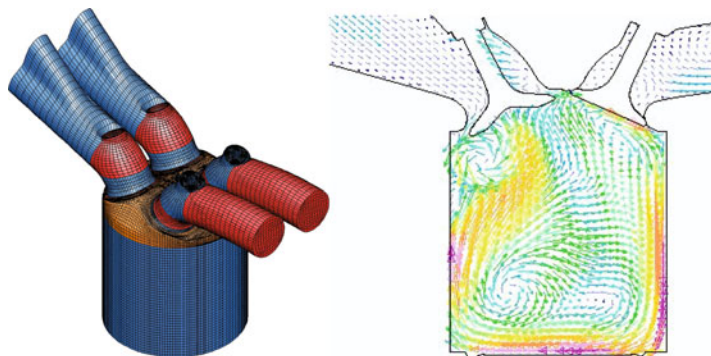
Fig. 12.10 Simulation of the cylinder flow of a SI engine. Basic geometry for the computational mesh ( left ) and the flow image in a section through valves at BDC ( right )
