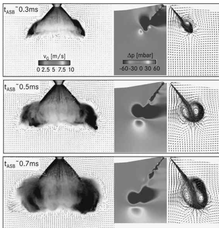
Fig. 13.9 Comparison of parcel image velocimetry (PIV) and simulation (left: static pressure distribution, right: velocity vector field)
