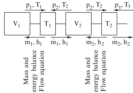
Fig. 7.25 Simple model of the gas path acc. to the filling and emptying method
