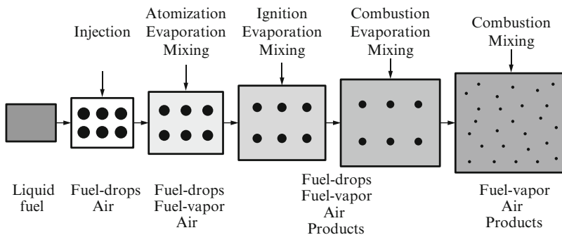
Fig. 11.7 Composition of spray packets
