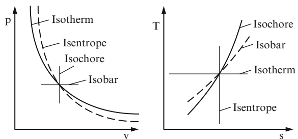
Fig. 2.10 Course of a simple change of state in the p, v - and in the T, s diagram
