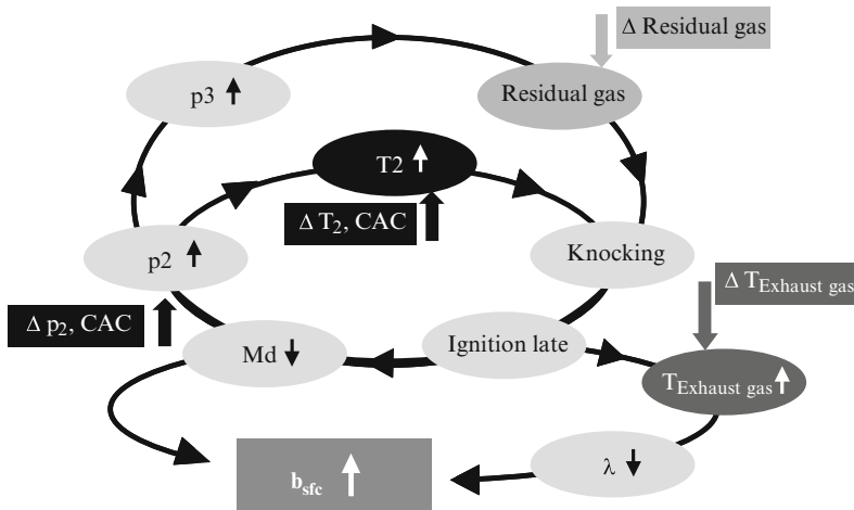
Fig. 8.39 Influence on consumption of a turbocharged SI engine
