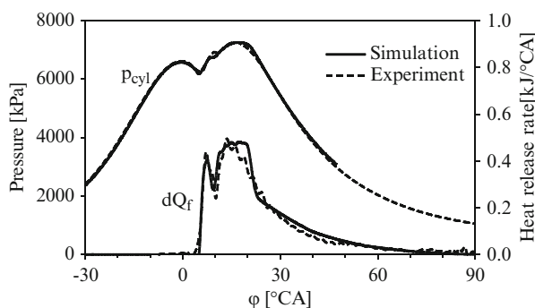
Fig. 11.8 Comparison of measured and calculated pressure progressions and heat release rate for a high speed diesel engine with 3.96 l displacement volume per cylinder at n = 1,500 \text{ rpm} and p_{me} = 9.8 \text{ bar}
