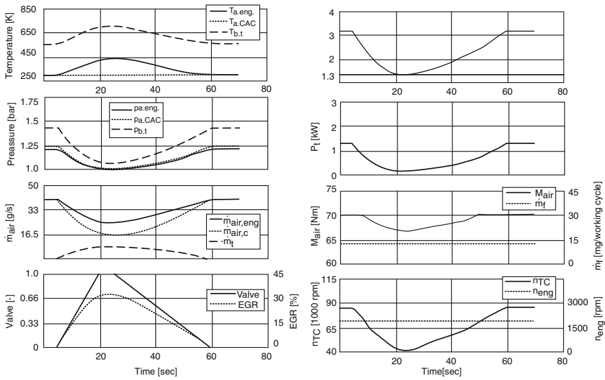
Fig. 10.15 Effect of the lift of the exhaust gas recirculation valve to engine operating conditions
