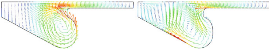
Fig. 12.13 Secondary swirl in the bowl of a diesel engine at 5°C before ignition TDC with BDC-speed at exactly 0 ( left ) and exactly 2.5 ( right )
