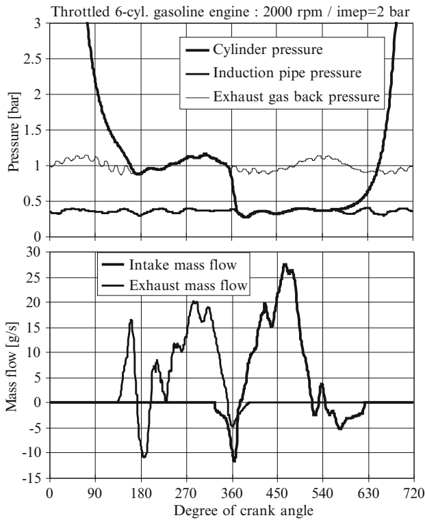
Fig. 10.6 Pressures and mass flows for the operating point i_{mep} = 2 bar
