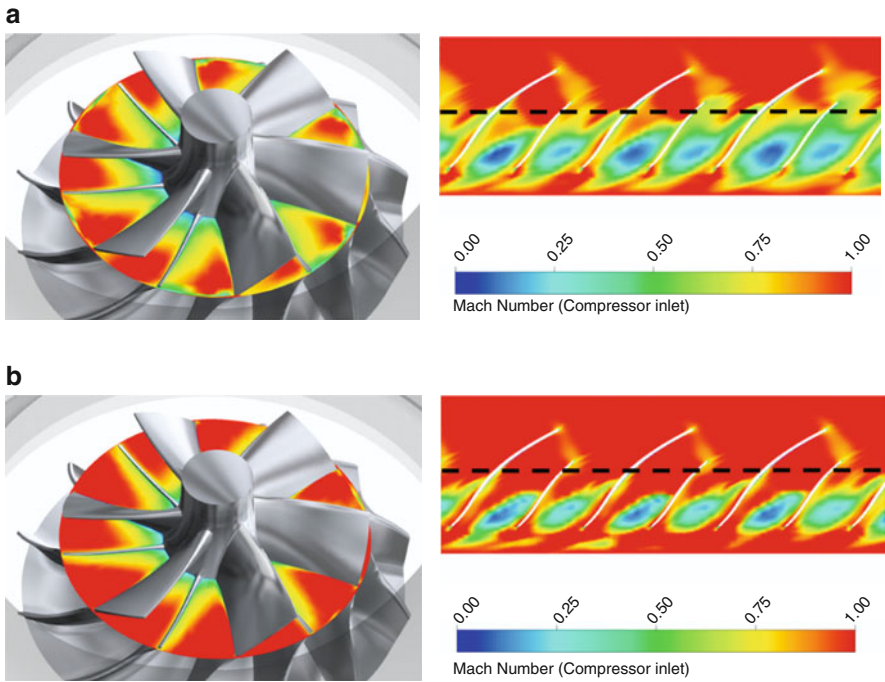
Fig. 15.10 Blade-to-blade views of the Mach number in the impeller of a compressor. (a) Mach number at center of compressor map. (b) Mach number near choke line
