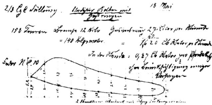
Fig. 3.1 Indicator diagram by August Nikolaus SI from May 18th, 1876
