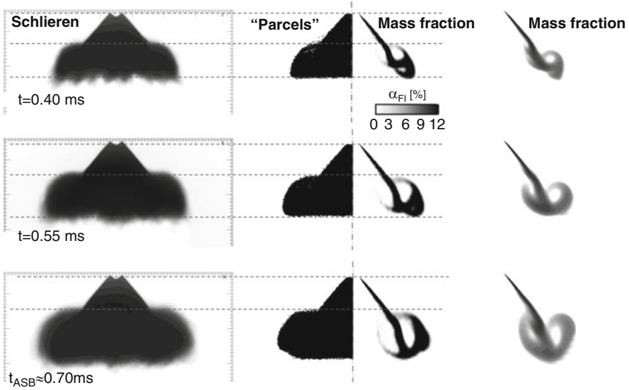
Fig. 13.13 Comparison between diagnostics and simulation for a gasoline direct injection with a outward-opening nozzle. Left: diagnostics; center: simulation in the further developed Lagrangian concept (on the basis of the Fokker–Planck equation) (3D image and 0.5° sector); right: simulation in the 3D Euler model (0.5° sector)
