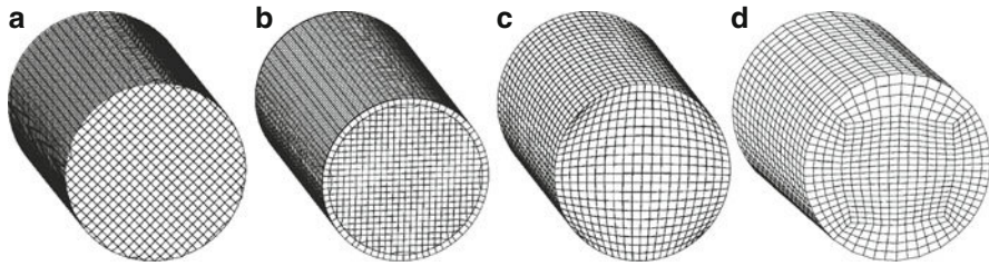
Fig. 12.9 To the far left a truncated Cartesian mesh which has a very poor mesh structure. A Cartesian mesh with a surface layer truncated only on the inside (second to the left) is already clearly better. Second to the right is a representation of a mesh with wall-adapted, hexahedral mesh structure, whereby there are, however, still deformations at the corners of the base meshes. The mesh on the far right displays an optimal, wall-adapted mesh structure
