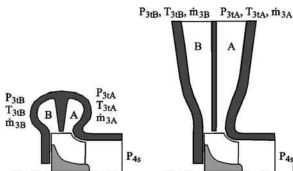
Fig. 8.33 Section through a twin-scroll turbine (Abdel Hamid et al. 2002)
