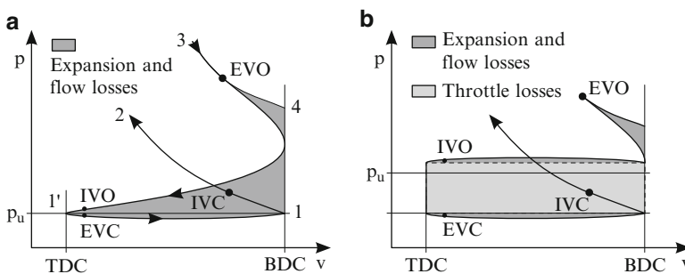
Fig. 2.24 p, v diagram for a four-stroke SI engine under (a) full load and (b) partial load
