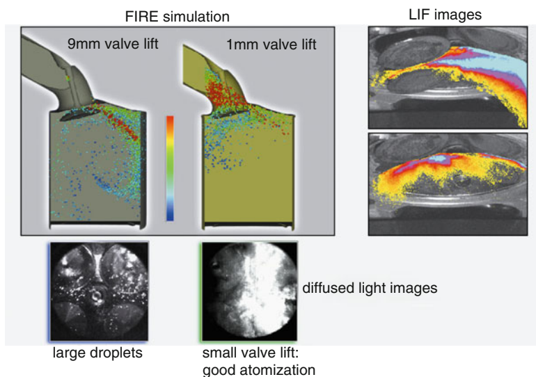
Fig. 4.34 Smaller droplet size and good mixture preparation with manifold injection and reduced intake valve lift, Liebl et al. (2001)
