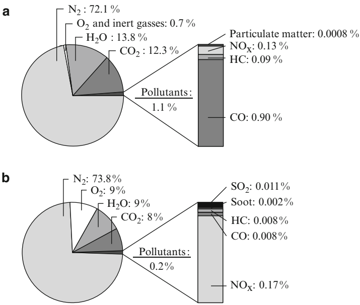
Fig. 6.2 Raw emissions (without catalyst) in percent by volume. (a) SI engine and (b) diesel engine
