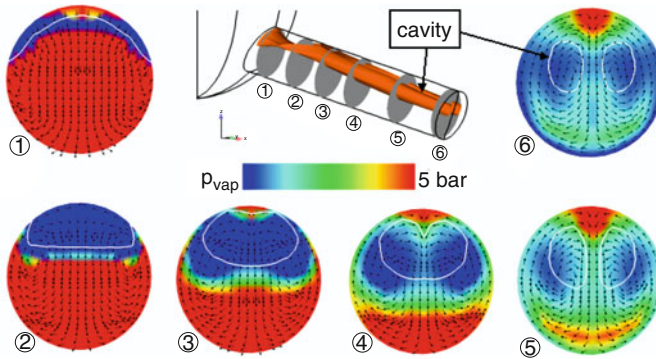
Fig. 12.15 By the strong redirection of the flow at the spray hole entrance, a secondary flow is formed in which cavitation bubbles are transported to the spray hole exit in counter rotating vortices
