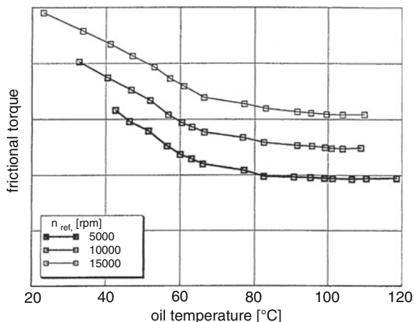
Fig. 8.36 Dependence of the friction torque in a passenger car turbocharger on the oil temperature
