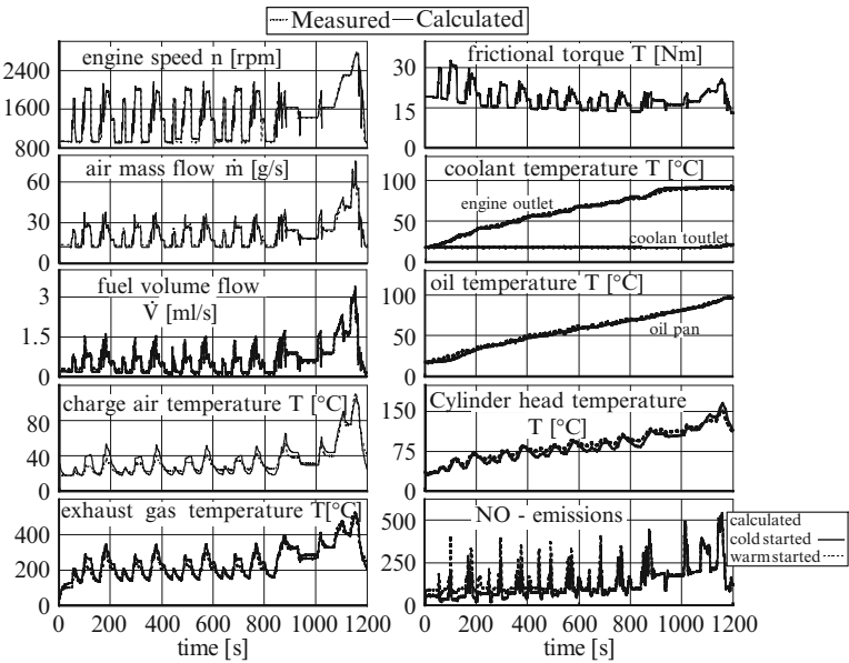
Fig. 10.23 Warming-up in the ECE test cycle
