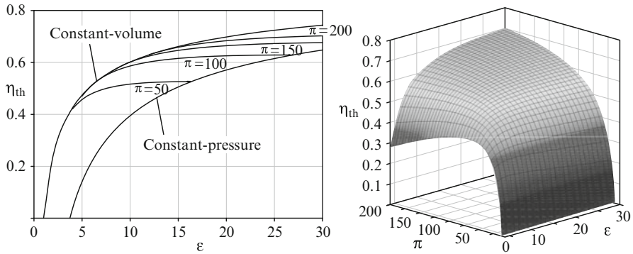
Fig. 2.19 Thermal efficiency of the Seiliger cycle
