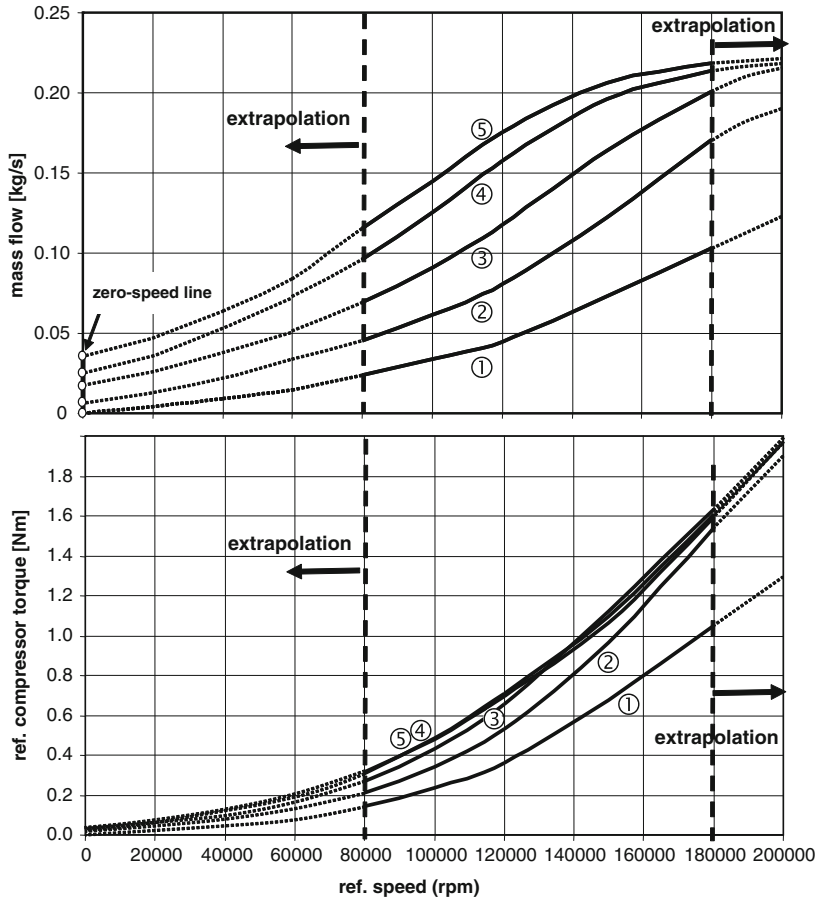
Fig. 8.27 Compressor extrapolation to low and high speeds
