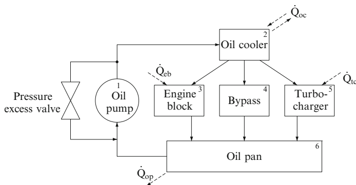
Fig. 10.3 Block diagram of the oil system
