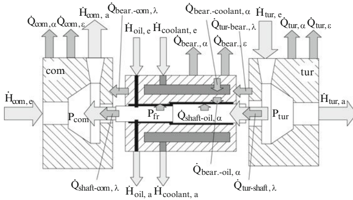
Fig. 8.37 Heat flow model for a water-cooled turbocharger
