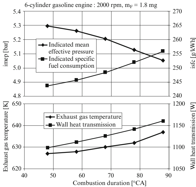
Fig. 10.8 Variation of the combustion duration (SI engine)
