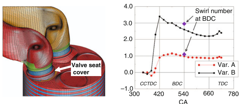
Fig. 12.12 Flow in the intake port of a diesel engine, port geometry ( left ) and time development of the swirl number for two variants ( right )
