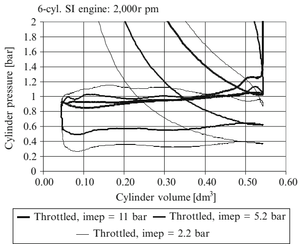
Fig. 10.5 Gas exchange loops under different operating conditions
