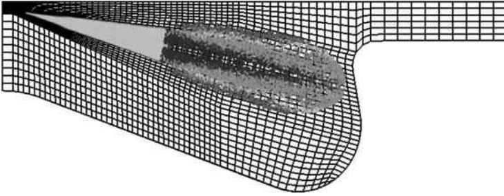
Fig. 13.10 Spray simulation for direct fuel injection in the ICAS embedding method: in the yellow disc 1D calculation, then the standard model
