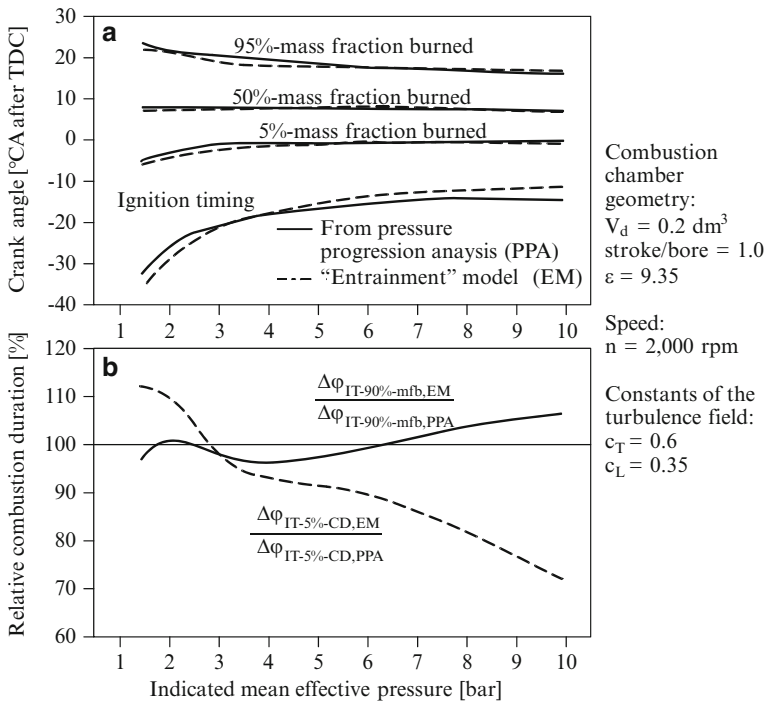
Fig. 11.12 Comparison of the mass conversions determined by the pressure progression analysis and calculated by the entrainment model (from: Scheele 1999)
