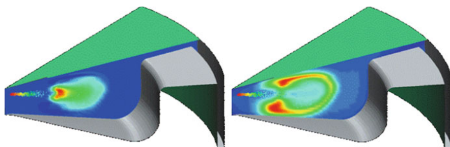
Fig. A.13 Fuel vapor concentration ( left ) and temperature distribution ( right ) in a DI diesel engine at 10° crank-angle ATDC
