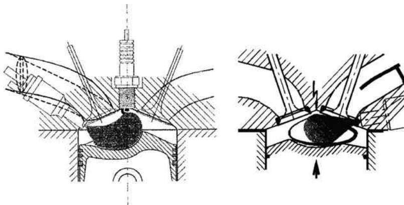
Fig. 4.37 Left: mixture formation in the wall guided process, acc. to Holy et al. (1998). Right: mixture formation in the air guided process with tumble flow, acc. to Grigo and Wolters (1998)
