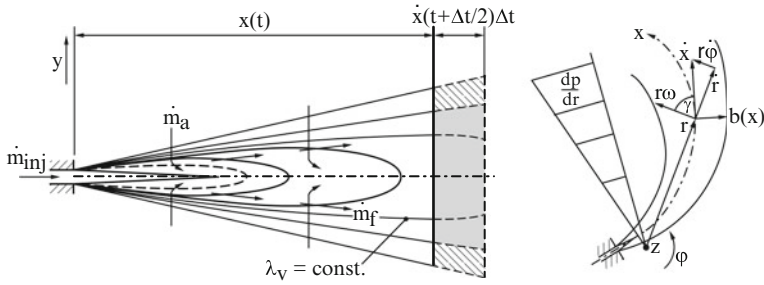
Fig. 11.4 Model of quasi-stationary gas jet in a solid body rotation flow-field
