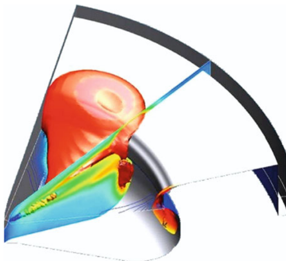
Fig. A.12 Spray droplets, temperature iso-surface and temperature distribution in a cut-plane across the spray axis during DI diesel combustion
