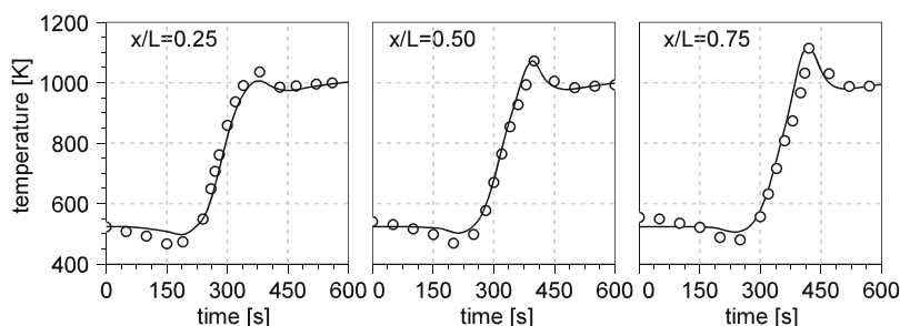
Fig. 9.10 Measured and calculated diesel particulate filter temperatures at three different axial positions along the symmetry line during regeneration
