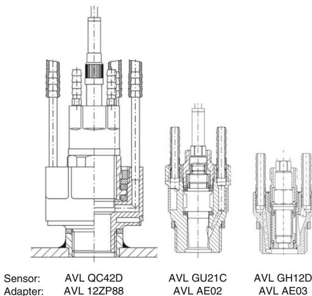
Fig. 3.28 Damping adapters for low-pressure indication with piezoelectric pressure sensors (AVL)
