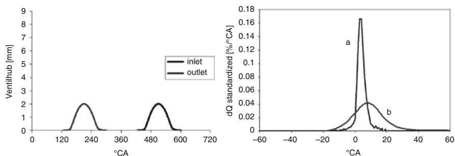
Fig. 4.41 Left: valve lift curves for residual gas storage. Right: heat release rate for HCCI operation (a) and conventional operation (b) at operating point 2,000 rpm, w_i = 0.27 kJ/l (Kaufmann et al. 2004)
