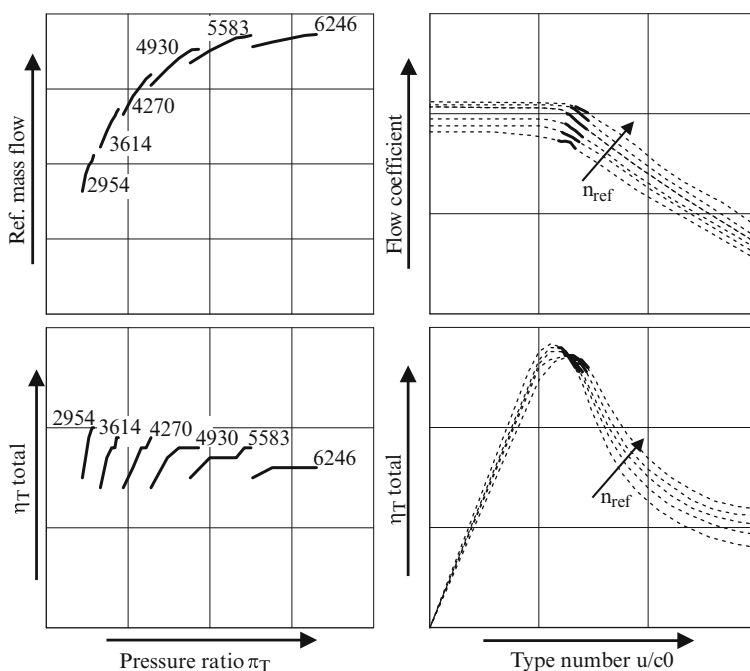
Fig. 8.30 Map for a small radial turbine ( left ), map using the blade speed ratio ( right )
