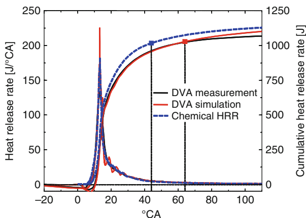
Fig. 14.2 Comparison of two heat release rates from 3D simulation, created by spatial integration and indication evaluation. The heat release rate taken from spatial integration is somewhat earlier
