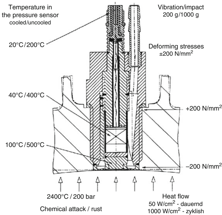
Fig. 3.12 External influences on the pressure sensor
