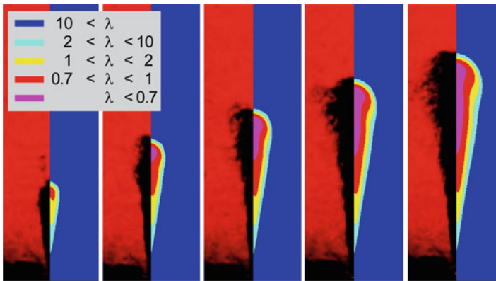
Fig. 13.12 Spray simulation with the ICAS approach (Krüger 2001): in comparison with the schlieren images, the spray form and propagation could be reproduced well
