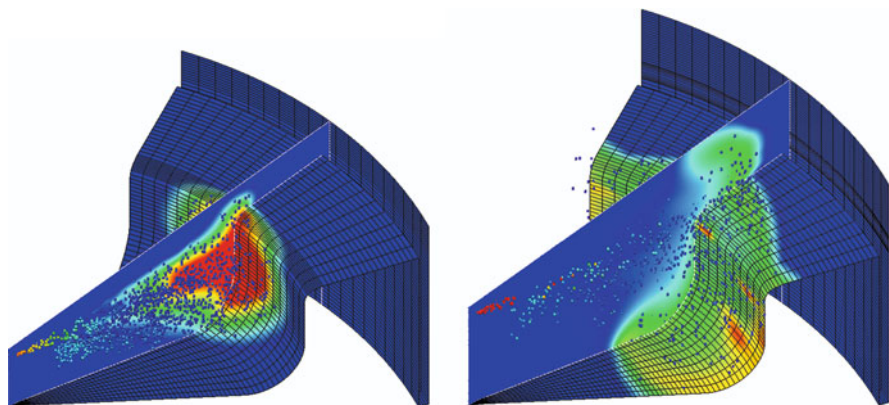
Fig. A.9 Fuel spray propagation and near wall fuel to air equivalence ratio distribution during DI diesel engine cold start at 20° crank-angle ( left ) and 30° crank-angle ( right ) ATDC
