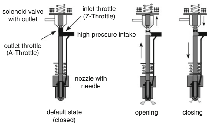
Fig. 4.12 Functionality of a servo-injector
