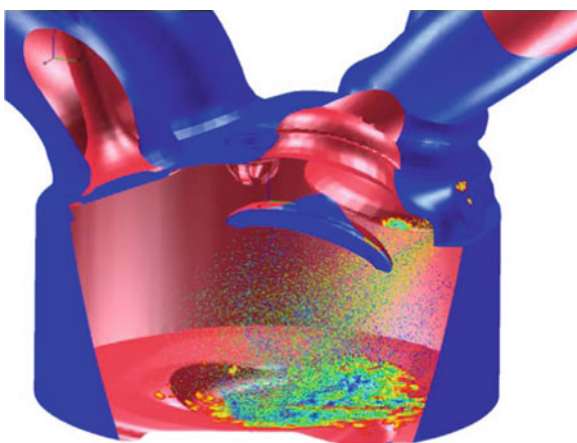
Fig. A.10 Spray droplet distribution and wallfilm formation in a direct injected SI-engine
