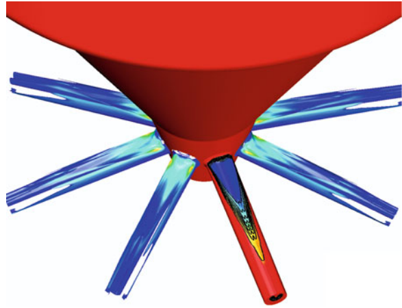
Fig. A.7 Calculated cavitation characteristics in a diesel injector nozzle
