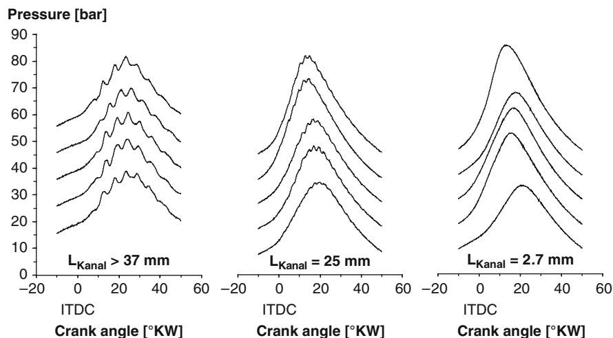
Fig. 3.19 Effect of the length of the indicator channel on the measured pressure profile
