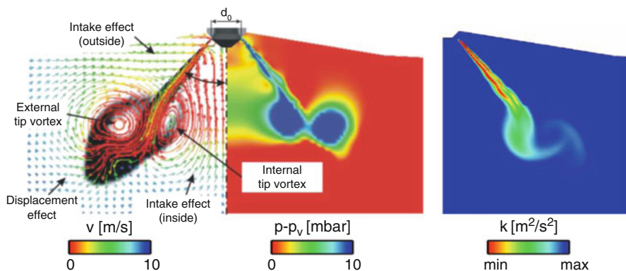
Fig. 13.8 Spray propagation in the case of direct gasoline injection with an outward-opening nozzle at 6 bar combustion chamber pressure. Left: the velocity and pressure field, right: gaseous phase turbulence
