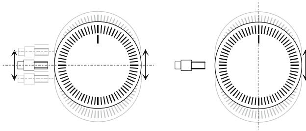
Fig. 3.22 The effect of relative motion between the marked disc and the sensor head
