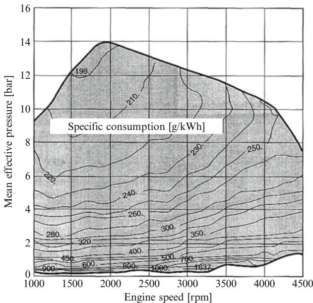
Fig. 2.26 Engine map of a four stroke diesel engine
