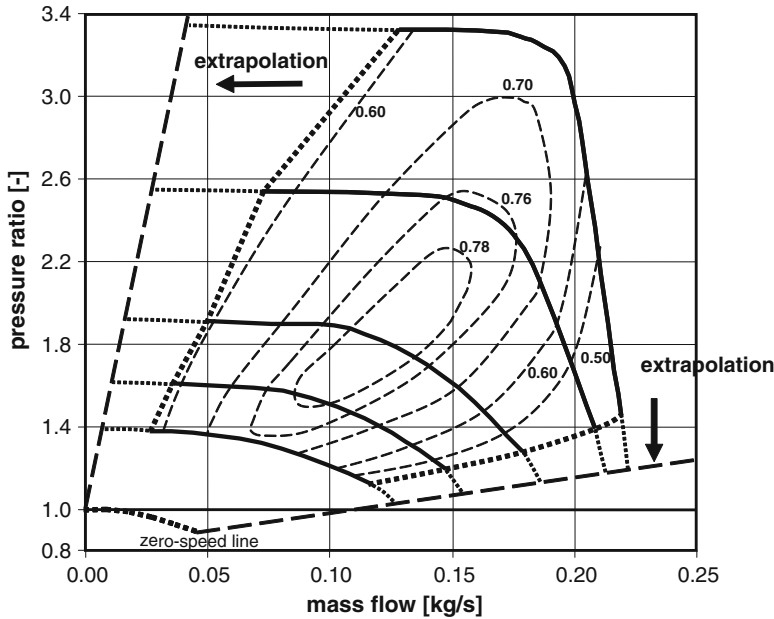
Fig. 8.23 Extrapolation in the pressure ratio/mass flow characteristic map
