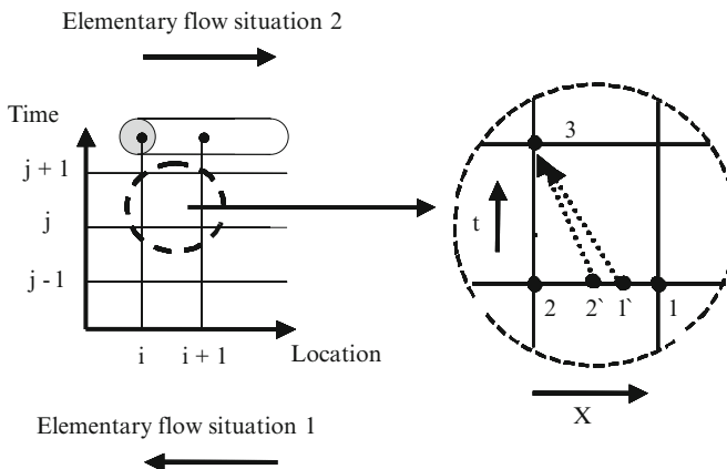
Fig. 7.31 Boundary coupling by of characteristic lines (Miersch 2003)
