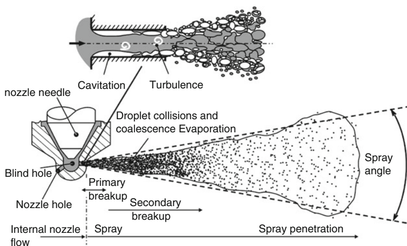
Fig. 4.18 Schematic representation of internal nozzle flow and spray propagation (Baumgarten 2006)
