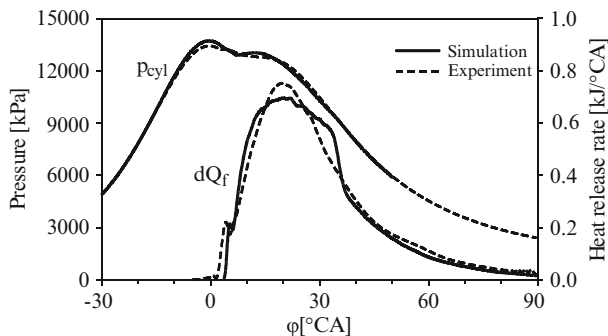
Fig. 11.9 Comparison of measured and calculated pressure progressions and heat release rate for a high speed diesel engine with 3.96 l displacement volume per cylinder at n = 1,500 \text{ min}^{-1} and p_{me} = 22.0 \text{ bar}
