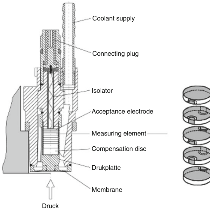
Fig. 3.9 Structure of a piezoelectric pressure sensor built for the longitudinal effect (Fa. AVL)
