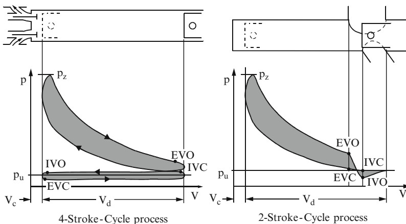
Fig. 2.7 p, V diagram for the four-stroke and two-stroke processes
