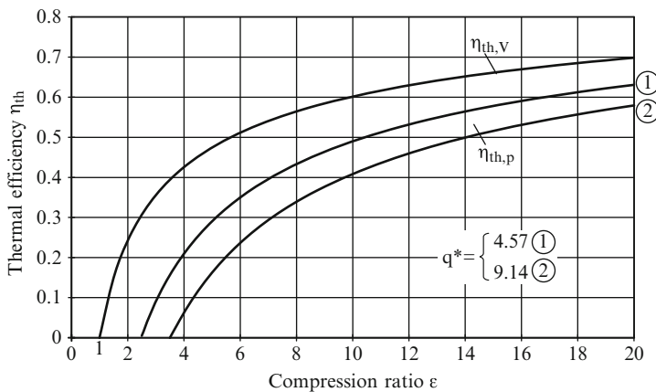
Fig. 2.17 Thermal efficiency of the constant-pressure cycle
