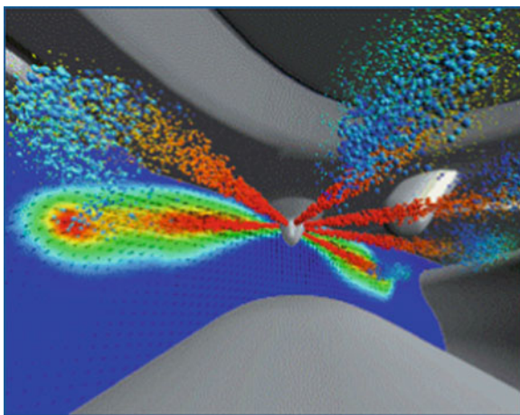
Fig. A.8 Spray droplet distribution and vapor concentration pattern during liquid fuel spray injection in a DI diesel combustion chamber
