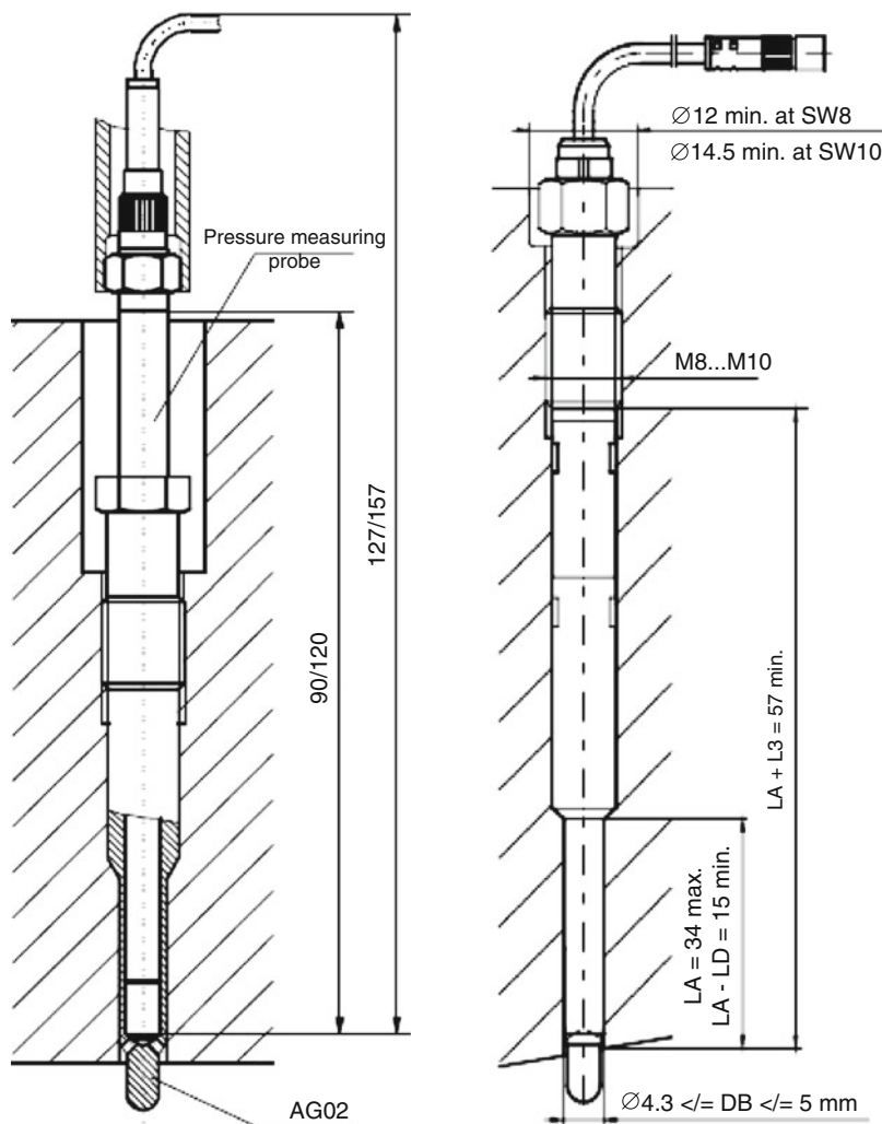
Fig. 3.17 Glow plug adapters with pressure measuring probes and glow plug sensors (AVL)
