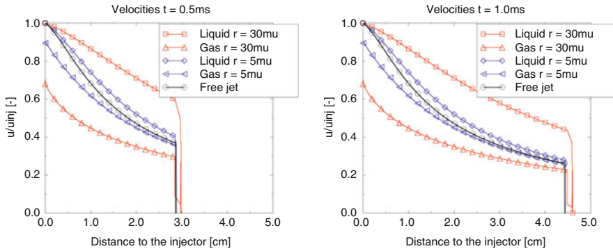
Fig. 13.11 Spray simulation with the ICAS method (Krüger 2001): Propagation behavior of different (non-vaporizing) sprays at various droplet sizes. The spray peak always spreads equally like a stationary free gas jet
