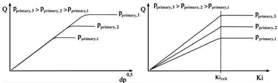
Fig. 7.38 Flow restriction caused by cavitation, plotted over dp^{0.5} (left) and the cavitation index Ki (right)
