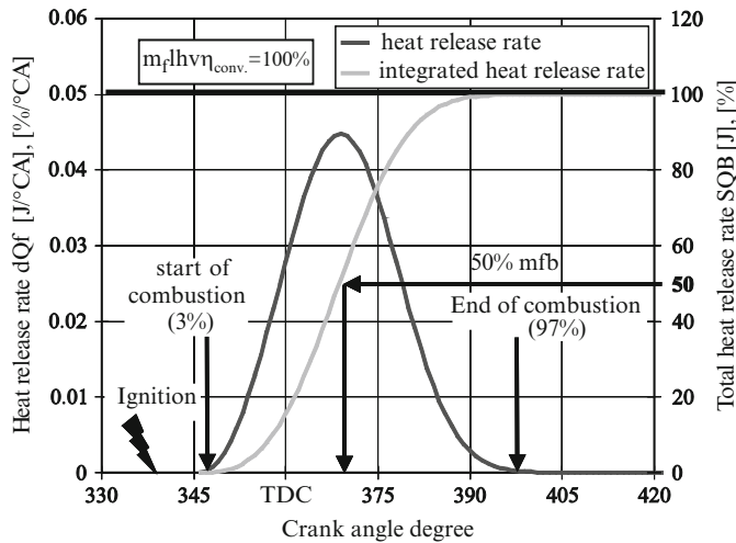
Fig. 3.30 Characteristic values of the combustion profile
