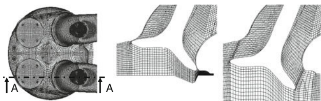
Fig. 12.8 Qualitatively high-grade mesh structure for a 4-valve SI engine for 2 valve lifts
