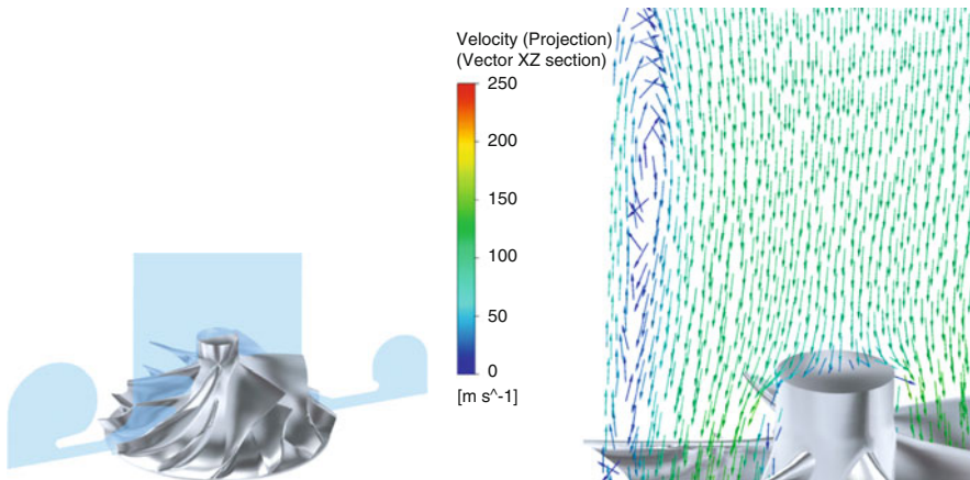
Fig. 15.8 Vector plot at cutting planes
