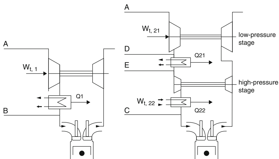
Fig. 8.18 One-stage and two-stage turbocharging
