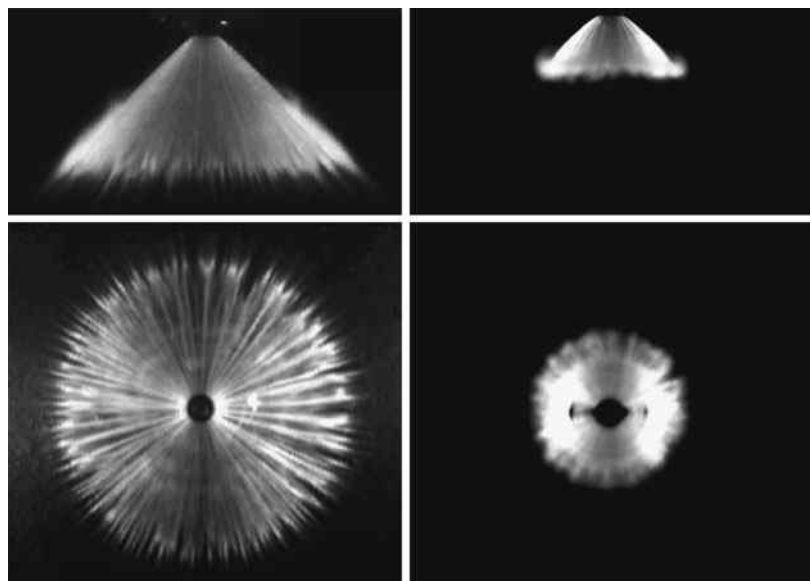
Fig. 4.40 Spray pattern of an outwards-opening piezo-injector under environmental conditions ( left ) and with a late injection time ( right ), Fröhlich et al. (2003)
