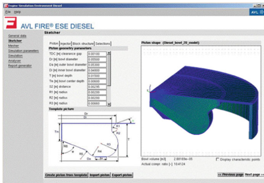
Fig. A.3 AVL FIRE® ESE Diesel – diesel engine meshing/simulation environment
