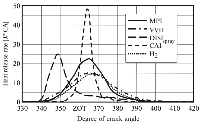
Fig. 3.33 Comparison of the characteristic combustion profiles of various combustion and load control processes
