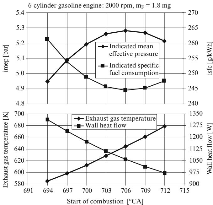
Fig. 10.7 Variation of the start of combustion (SI engine)
