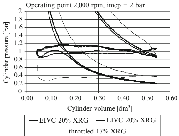
Fig. 10.11 Gas exchange loops for an electromechanical valve train
