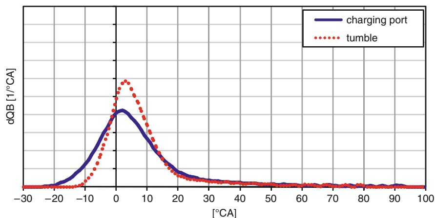
Fig. 4.29 Acceleration of the heat release rate at the homogeneous operating point 2,000/ w_i = 0.27 by increased charge motion in the form of tumble (standardized heat release rates)
