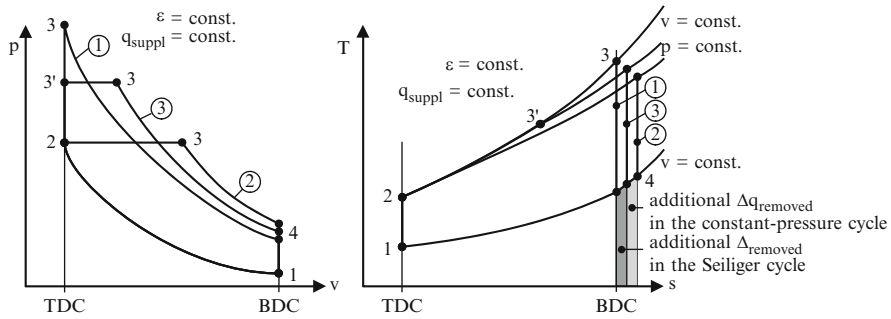
Fig. 2.20 Comparison of the closed cycles, ① = constant-volume, ② = constant pressure, ③ = Seiliger cycle
