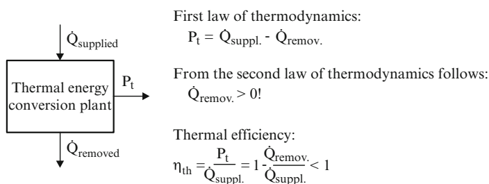
Fig. 2.2 Diagram of thermal energy conversion
