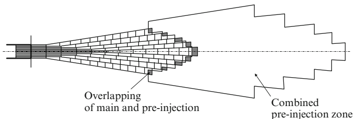
Fig. 11.10 Mixing of the pilot- and main injection pulses, acc. to Thoma et al. (2002)
