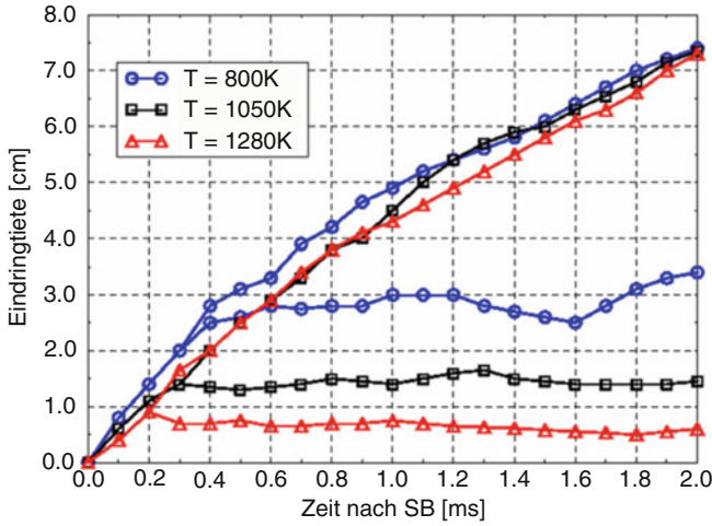
Fig. 13.4 Measurement of the penetration length of a diesel spray in a hot chamber at varying chamber temperatures but equal density (Krüger (2001))
