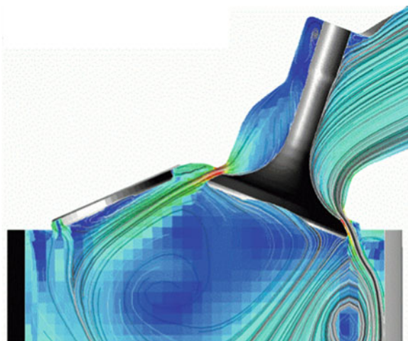
Fig. A.6 Turbulence intensity distribution during SI-engine intake flow adopting the k-\zeta-f turbulence model (Tatschl et al. 2006)
