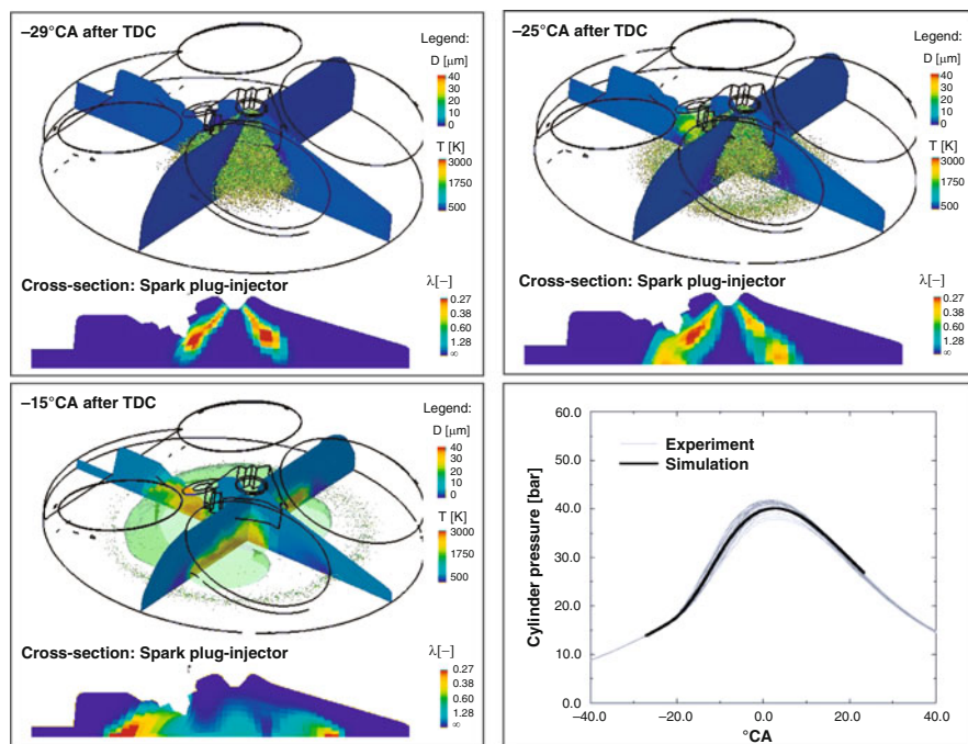
Fig. 14.15 Left top and bottom: simulation of stratified charge combustion in a DE SI engine with a spray-guided combustion process at 2,000 rpm and 2 bar p_{mc} ; right bottom: associated pressure curves, simulation vs. experiment (different cycles)
