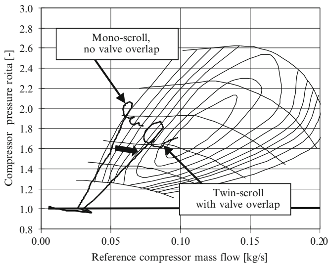
Fig. 10.26 Operating lines for concept 2 and 5 in the compressor map
