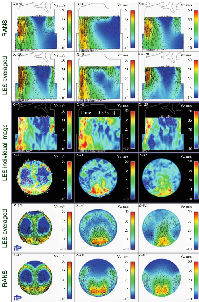
Fig. 12.6 Velocity fields in the valve cross-section and on the level of the cylinder head gasket, simulated for a flow bench test , in which characteristic parameters such as the swirl and tumble numbers of a cylinder head are determined (Angelberger 2007)
