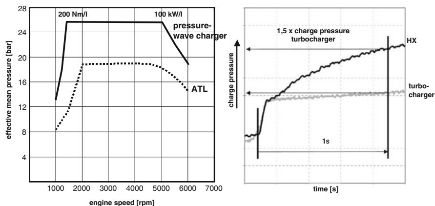
Fig. 8.4 Torque profile and response pressure-wave charger (Flückiger et al. 2006)
