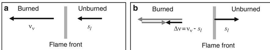
Fig. 14.8 Situation in the reference system (a) of the flame front and (b) of the unburned gases
