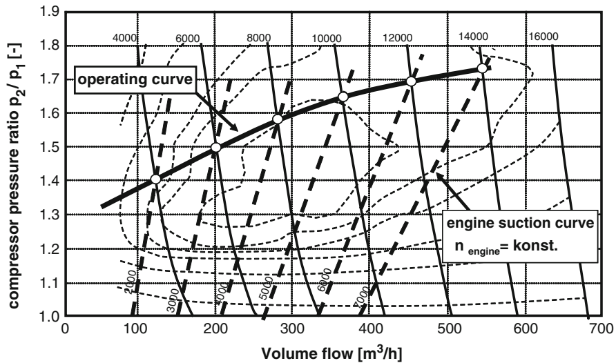
Fig. 8.6 Map and line of operation of a positive displacement charger ---- isentropic efficiency; ——— charger speed [rpm]
