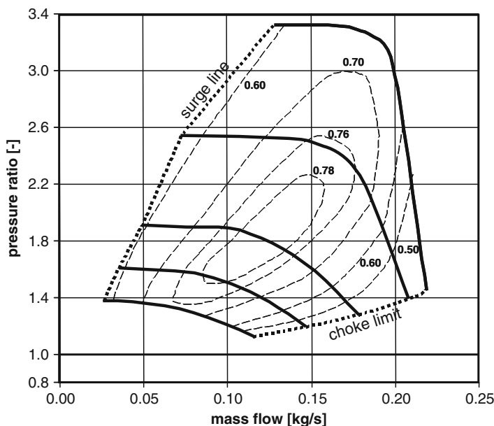
Fig. 8.22 Characteristic map of a turbo compressor
