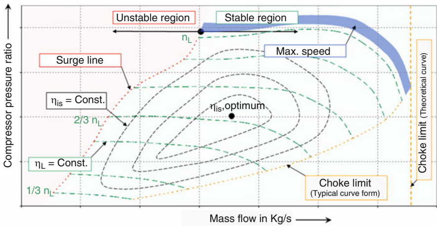
Fig. 15.11 Schematic diagram of a compressor map
