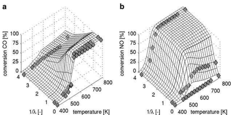
Fig. 9.3 Measured and calculated conversion of CO ( left ) and NO ( right ) in a TWC as function of temperature and gas composition (see Wurzenberger et al. 2006)
