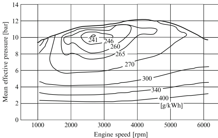
Fig. 2.25 Engine map for a four-stroke SI engine with lines of constant consumption b_e [g/kWh]
