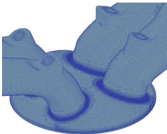
Fig. A.2 Automatically generated computational mesh of an SI-engine intake port/combustion chamber configuration
