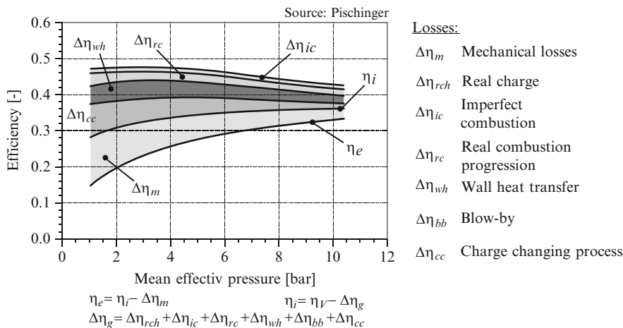
Fig. 2.23 Division of losses in the real internal combustion engine
