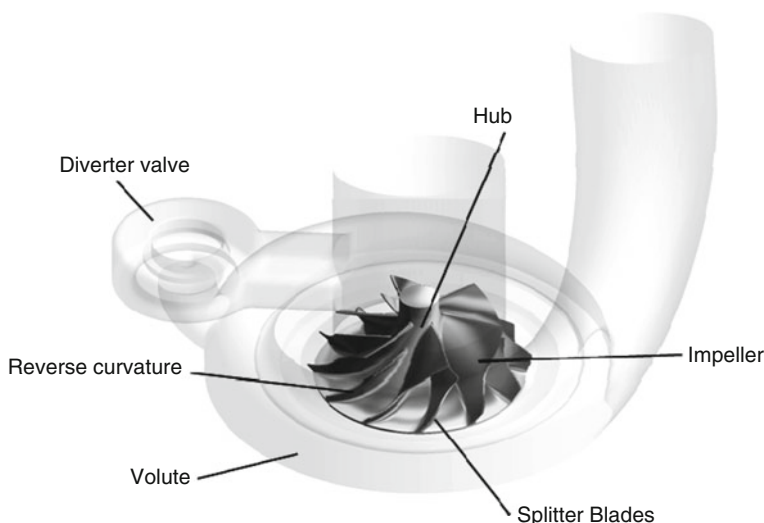
Fig. 15.1 Complex three-dimensional geometry of a compressor
