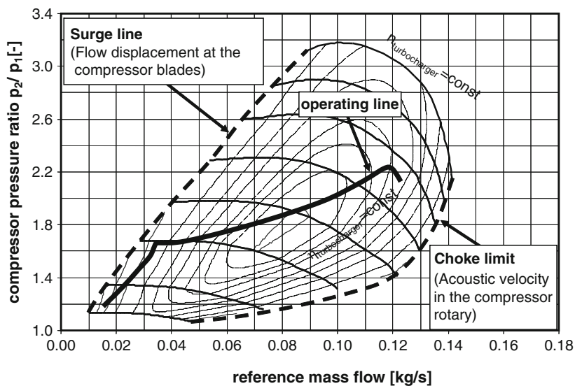
Fig. 8.17 Characteristic map and operating line of a turbo compressor
