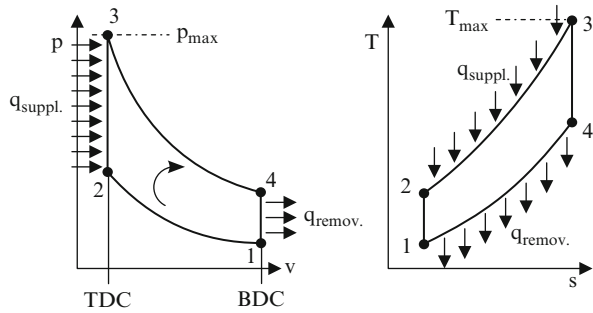
Fig. 2.14 Representation of the constant-volume cycle in the p, v and T, s diagram
