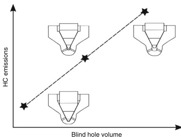
Fig. 6.5 Schematic representation of HC emissions as a function of the blind hole volume
