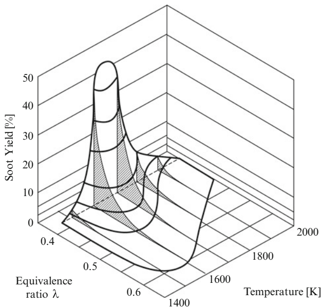
Fig. 6.19 Soot yield as function of equivalence ratio and temperature, Pischinger et al. (1988)
