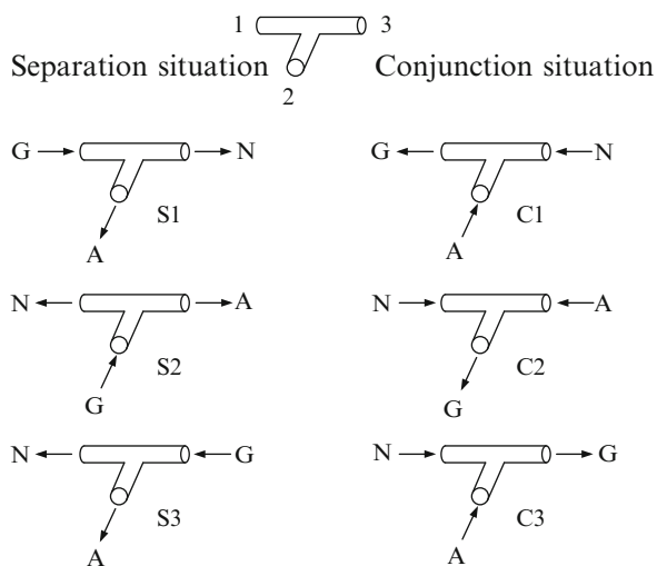
Fig. 7.33 Flow situations at a pipe branching
