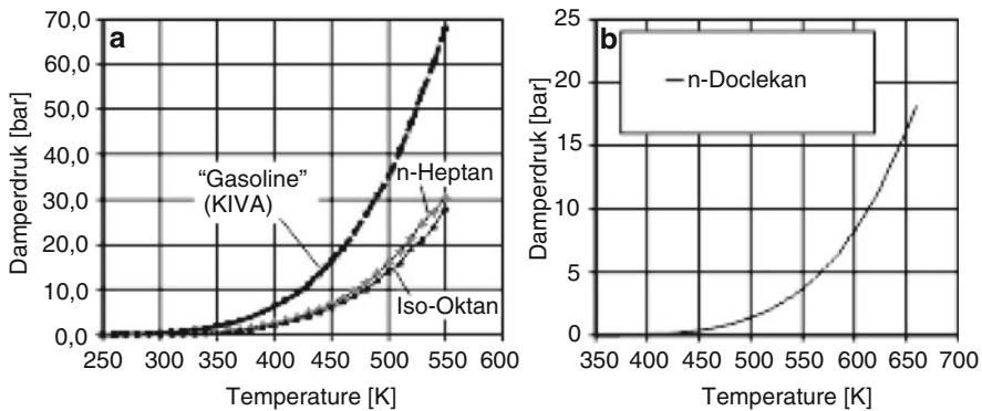
Fig. 13.2 (a) Vapor pressure curve for gasoline-class fuels, (b) Vapor pressure curve of a component typical of diesel
