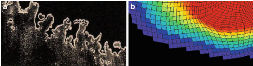
Fig. 14.7 Relation between laminar and turbulent flame fronts. (a) Experimental laminar flame front, position and state of the turbulent flame front are shown (b) The turbulent flame front in the averaged simulation
