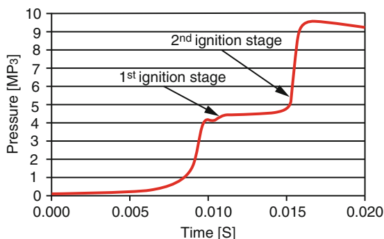
Fig. 5.8 Pressure profile for the ignition of a alkane-air mixture in a fast compression machine
