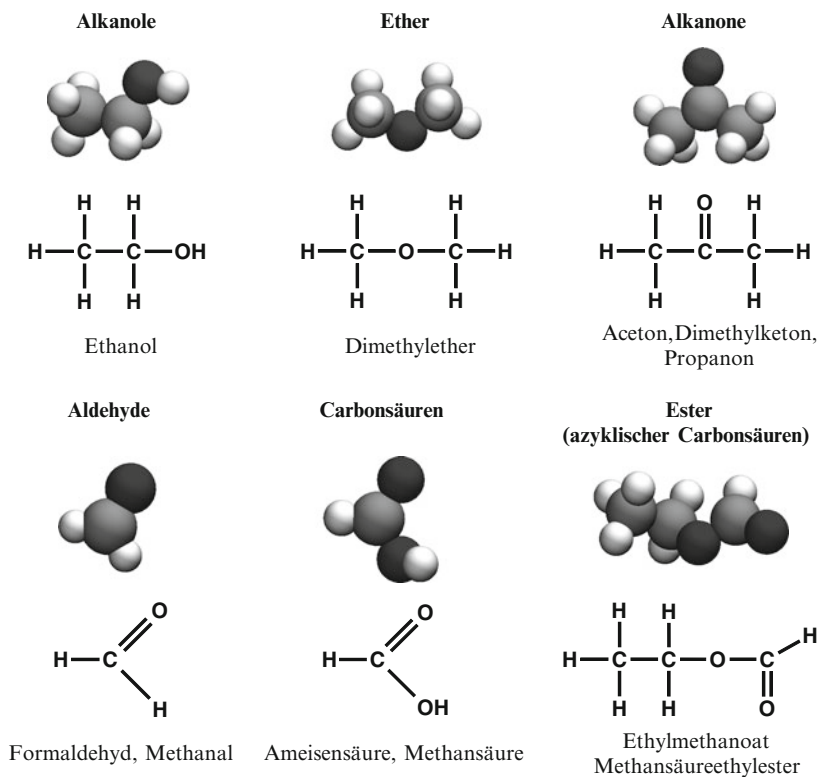
Fig. 4.3 Structural formulae and graphic representation of oxygenic hydrocarbons
