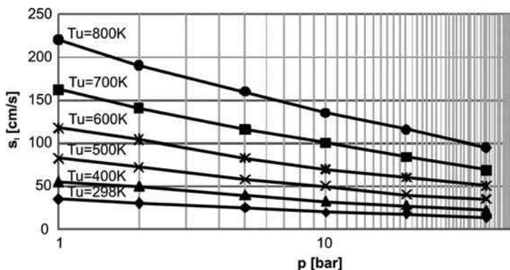
Fig. 4.27 Laminar flame front speed of iso-octane at \lambda = 1 acc. to Pischinger (2001)
