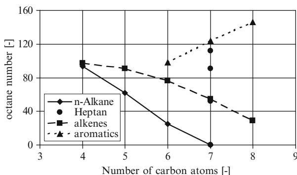
Fig. 4.6 Octane numbers for hydrocarbons of different groups and chain lengths
