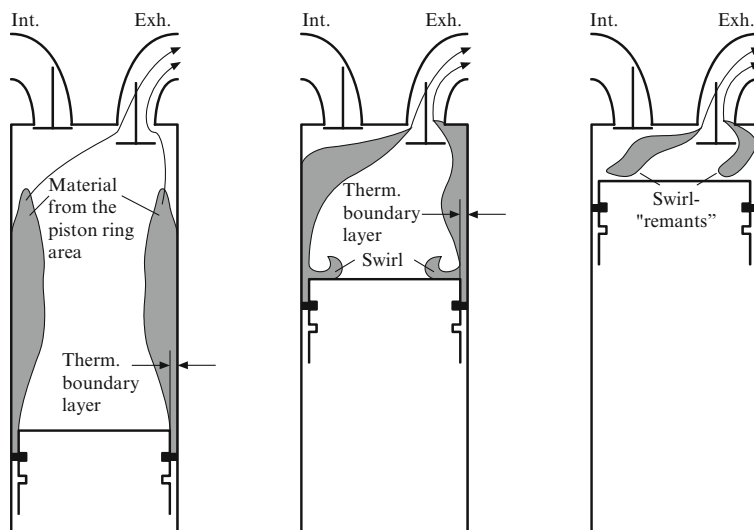
Fig. 6.3 Schematic representation of HC formation
