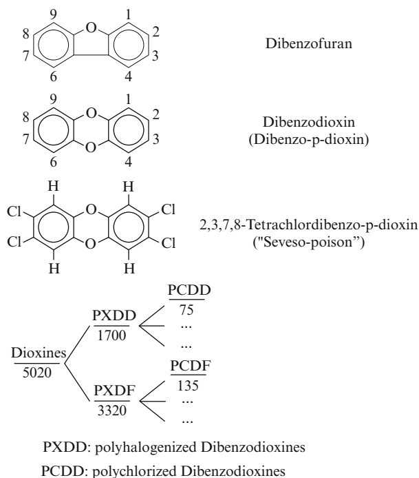
Fig. 6.11 Dioxine structures
