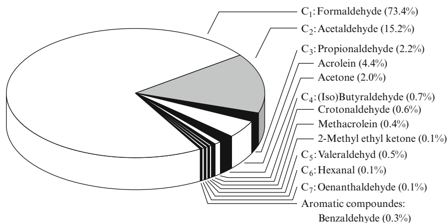
Fig. 6.8 Distribution of carbonyl compounds in the exhaust gas of a truck diesel engine, Lange (1996)
