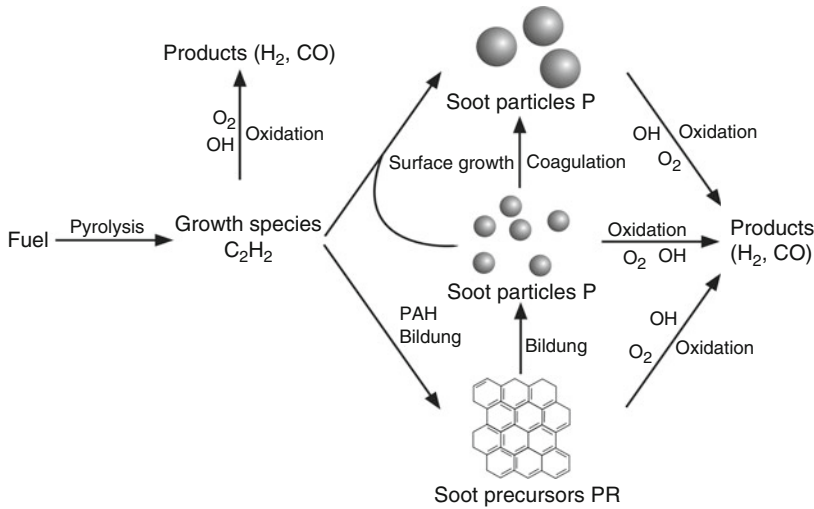
Fig. 6.21 Schematic representation of the phenomenological soot model, acc. to Tao et al. (2005)
