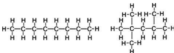
Fig. 5.9 Molecular structure of n-octane ( left ) and isooctane (2,2,4-trimethylpentane, right )
