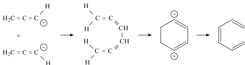
Fig. 6.17 Development of benzene rings, acc. to Warnatz et al. (2001)
