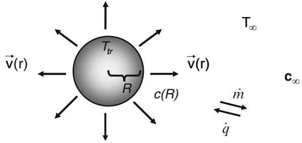
Fig. 13.1 Principle sketch for the representation of vapor and heat fluxes in the droplet environment
