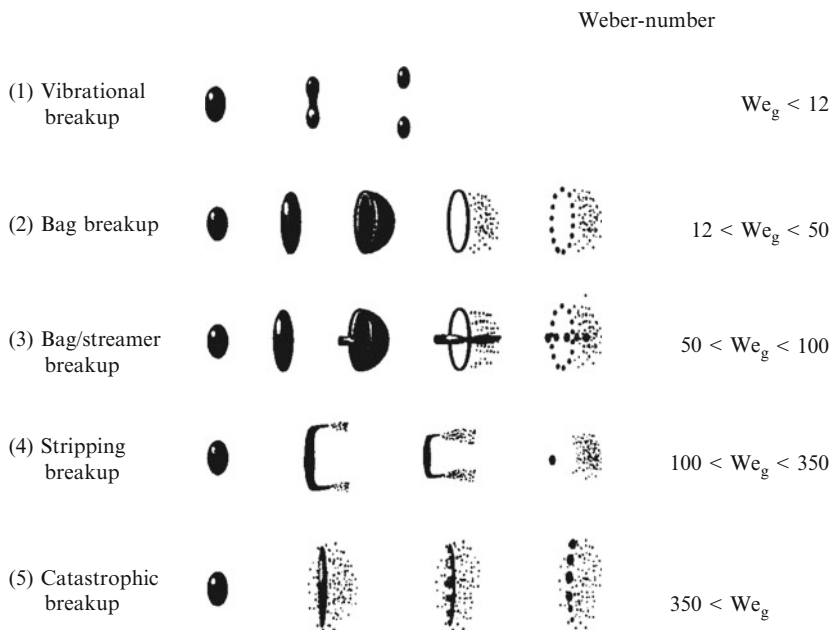
Fig. 13.5 Aerodynamic breakup mechanisms, acc. to Pilch and Erdman (1987)
