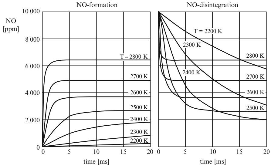
Fig. 6.24 NO-formation and disintegration in a thermal reactor, p = 60 bar; l = 1.0
