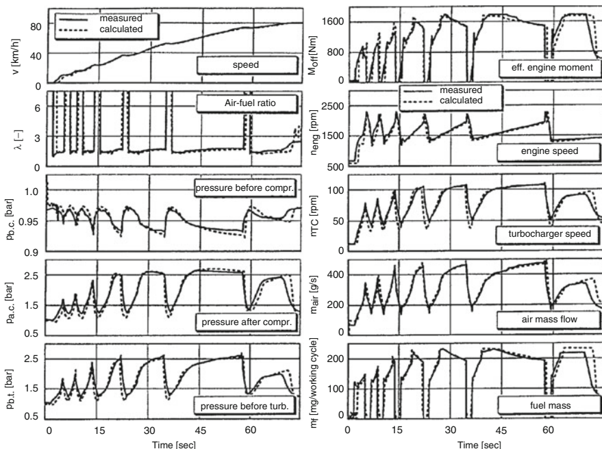
Fig. 10.17 Free acceleration, 40 ton truck
