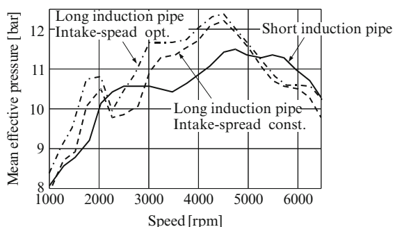
Fig. 10.12 Intake pipe length variation in a SI engine
