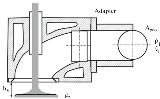
Fig. 7.3 Determining the flow coefficients on the flow bench
