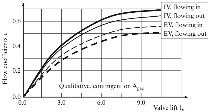
Fig. 7.4 Flow coefficients \mu = f(h_v)
