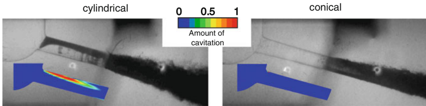
Fig. 12.16 The shape of the nozzle hole has a large effect on the cavitation tendency. The conical nozzle ( right ), almost free of cavitation, leads to a considerably more slender injection jet
