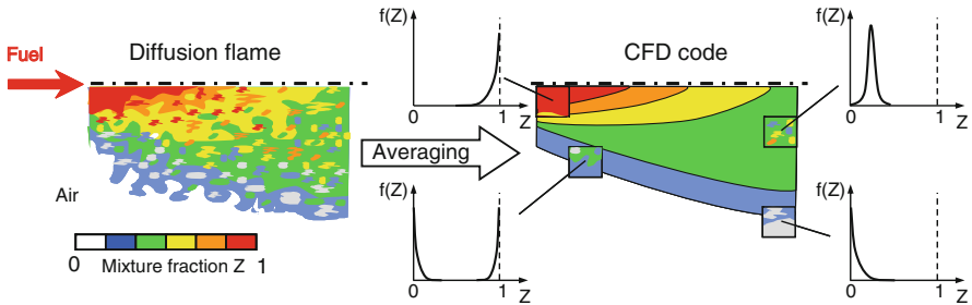
Fig. 12.3 Visual illustration of the effect of ensemble averaging in the case of a turbulent diffusion flame (details of the mixture vanish) and how the statistics of the mixture can be reconstructed by introducing the probability density function
