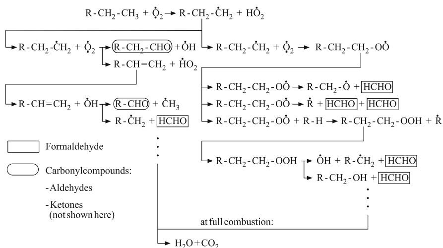
Fig. 6.6 Excerpt from the hydrocarbon oxidation diagram
