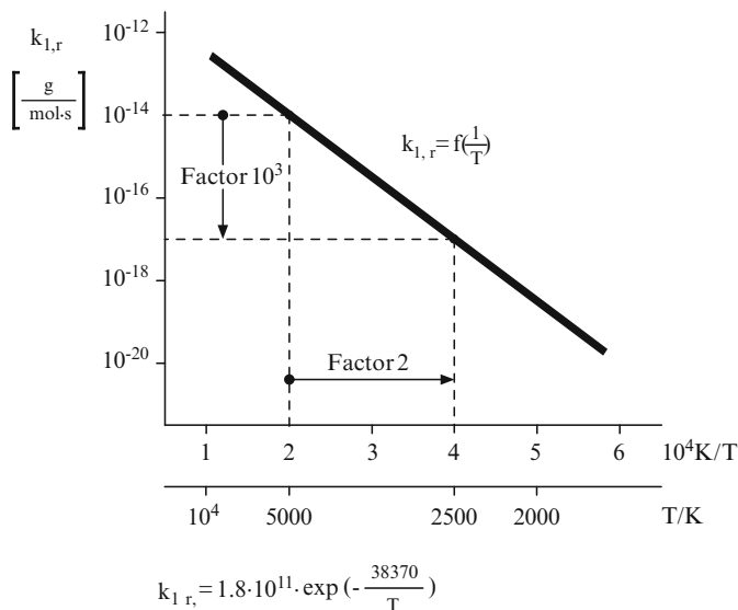
Fig. 6.22 Reaction coefficient of the first Zeldovich reaction
