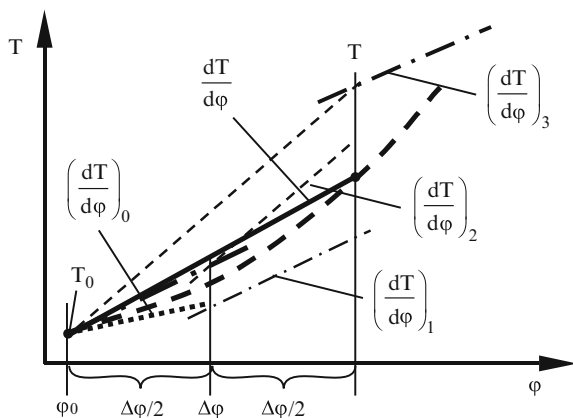
Fig. 7.27 Integration according to the fourth order Runge-Kutta process
