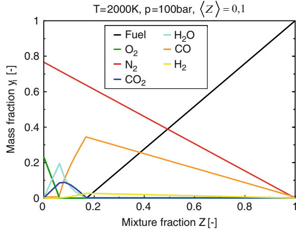
Fig. 14.3 Distributions of the seven species over the fuel mass fraction or the mixture fraction
