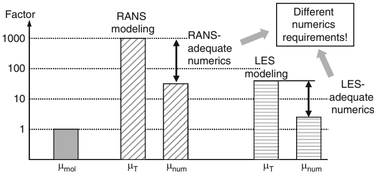
Fig. 12.5 Much higher requirements on the numerics are the result of the much lower turbulent viscosity in LES compared to RANS (see Angelberger 2007)
