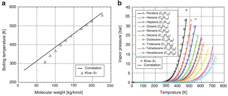
Fig. 13.3 Comparison of model and measurements of boiling temperature (a) and vapor pressure curve (b) for n-alkanes (from Hermann (2008))
