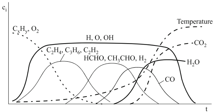
Fig. 5.4 Temporal concentration profile for hydrocarbon combustion
