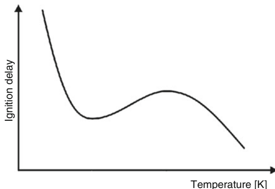
Fig. 5.7 Schematic representation of the negative temperature coefficient (NTC) in the ignition of hydrocarbons
