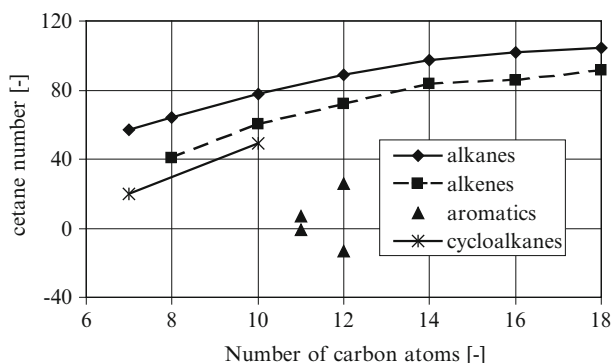
Fig. 4.7 Cetane numbers for hydrocarbons of different groups and chain lengths
