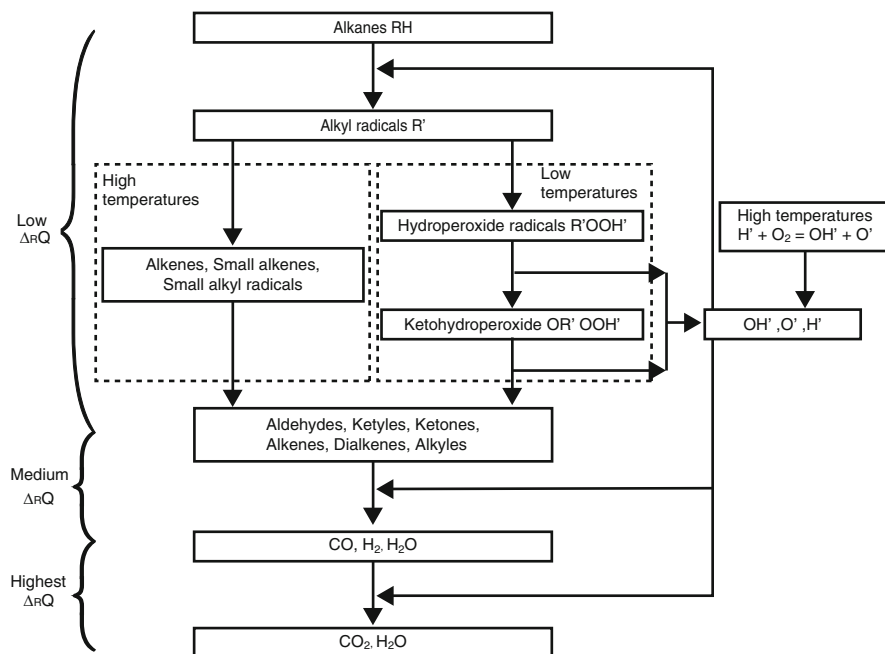
Fig. 5.3 Diagram of the hydrocarbon oxidation process
