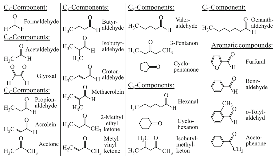
Fig. 6.7 Detectable carbonyl compounds, Lange (1996)
