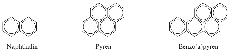
Fig. 6.9 Structure of various aromatic hydrocarbons
