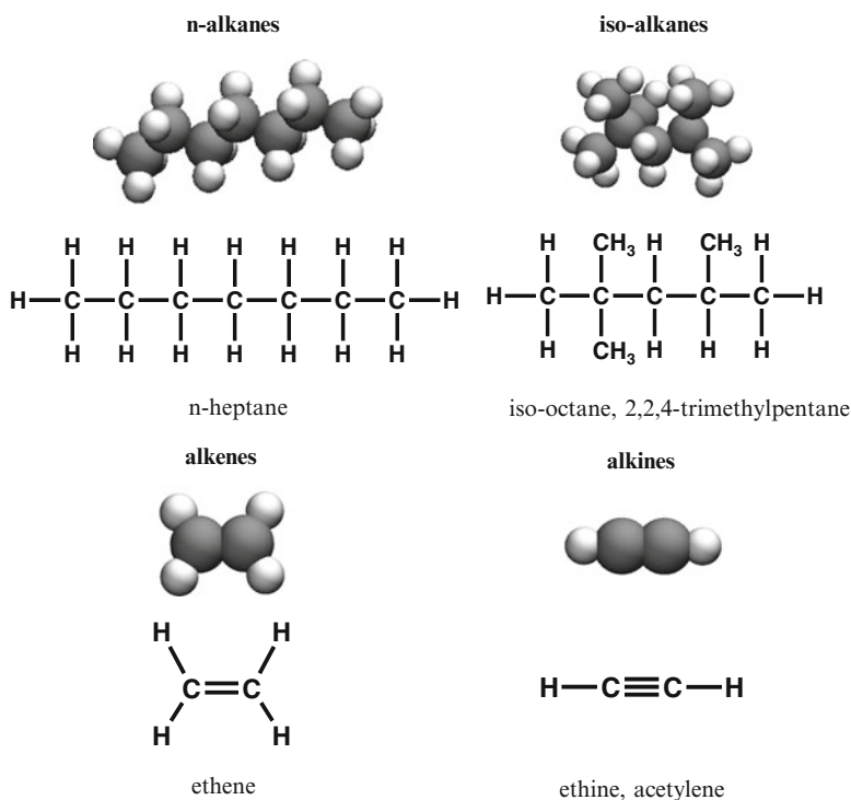
Fig. 4.1 Structural formulae and graphic representation of aliphatic hydrocarbons
