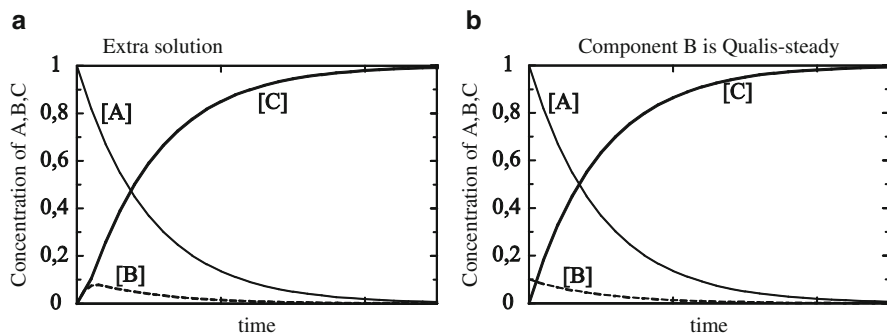
Fig. 5.2 Progression of concentrations of A, B and C under the condition k_{f,1} \ll k_{f,2} in the sequential reaction A \xrightarrow{k_{f,1}} B \xrightarrow{k_{f,2}} C (a) exact solution (b) assuming that B is quasi-steady
