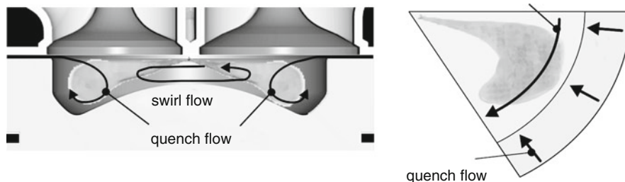
Fig. 4.17 Macroscopic flow structures in the combustion chamber
