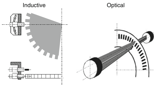
Fig. 3.21 Measuring principles of angle sensors
