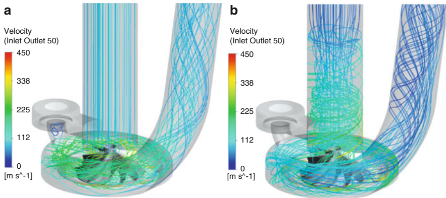
Fig. 15.7 Streamline plot for the visualization of compressor behavior. (a) operating point at center of compressor map; (b) operating point near pump boundary
