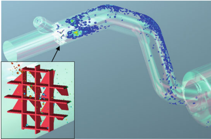
Fig. 9.13 Static mixer downstream of an urea injector and wall film distribution
