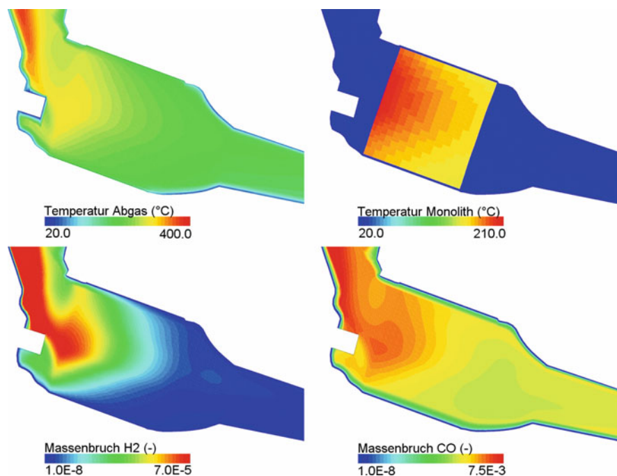
Fig. 9.4 3D CFD simulation of a closed coupled TWC. Spatial distribution of gas and wall temperature ( upper row ) and species mass fractions H 2 and CO ( lower row ); (see Missy et al. 2002)
