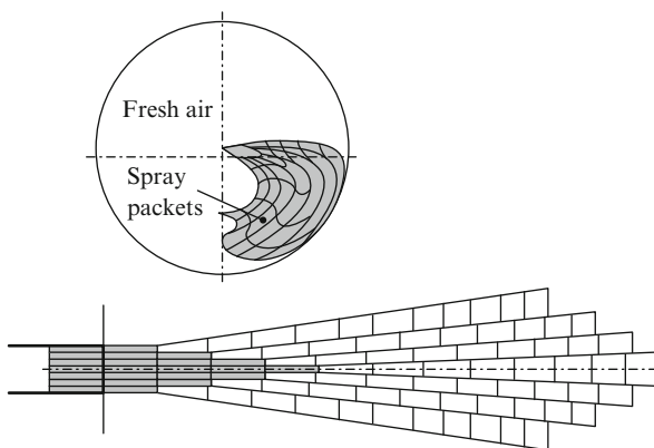
Fig. 11.6 Packet model, see Hiroyasu et al. (1983a, b)
