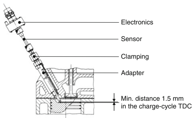
Fig. 3.26 Structure and assembly of a capacitive TDC sensor (AVL)
