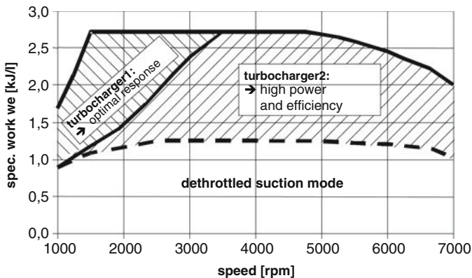
Fig. 8.19 Operating ranges in sequential turbocharging
