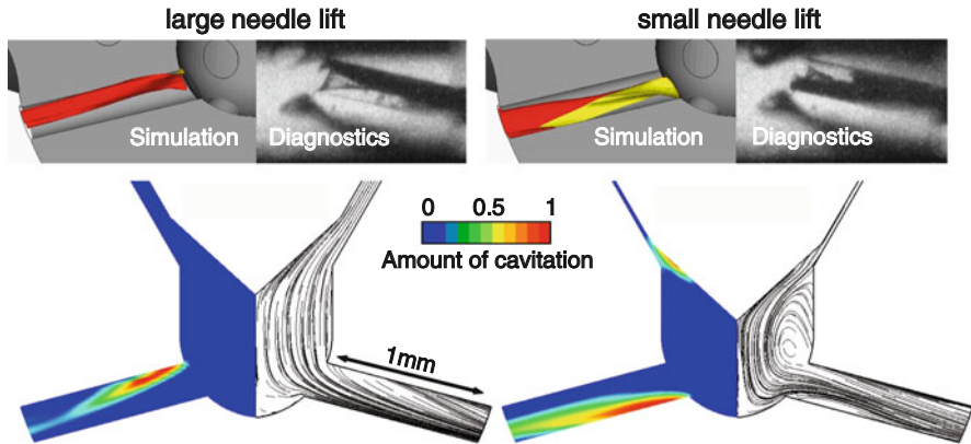
Fig. 12.17 Needle lift affects the in-flow of fuel into the nozzle hole, thus the position of the cavitation tube in the spray hole as well
