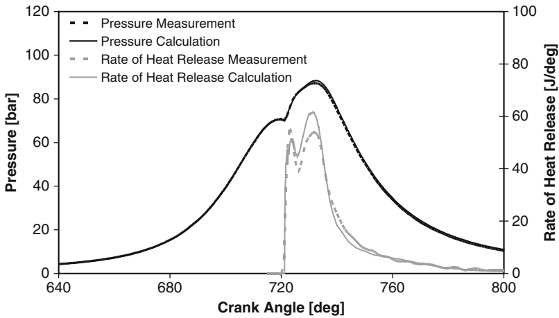
Fig. A.14 Comparison of calculated and measured cylinder pressure evolution and heat release rate for conventional diesel combustion (Tatschl et al. 2007)
