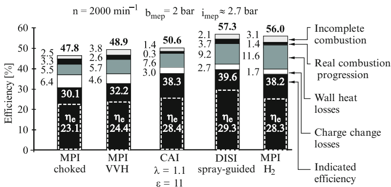
Fig. 3.34 Comparison of loss distribution in various combustion and load control processes
