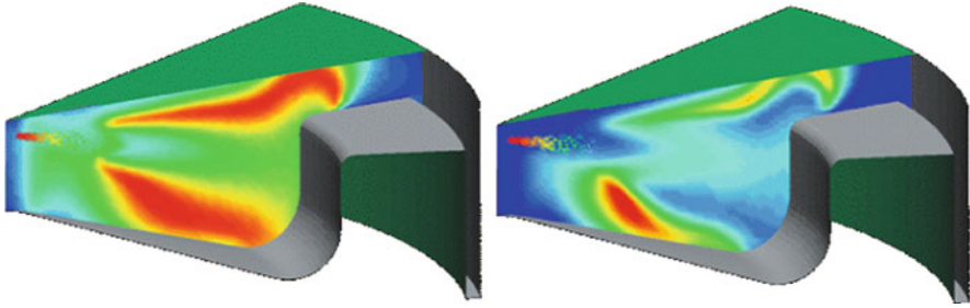
Fig. A.20 Temperature ( left ) and NO concentration ( right ) in a DI diesel engine at 20° crank-angle ATDC
