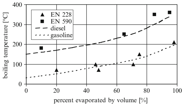
Fig. 4.5 Typical boiling curves for gasoline and diesel
