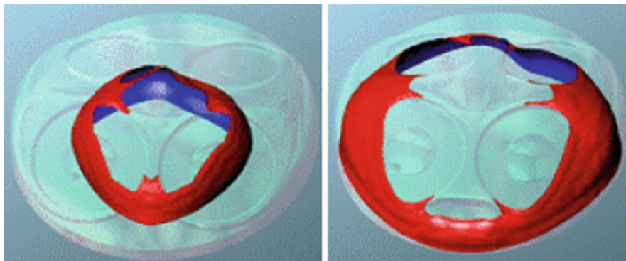
Fig. A.16 Flame front shape and location in a 4V SI-engine at 15° crank-angle ( left ) and 25° crank-angle ( right ) after TDC
