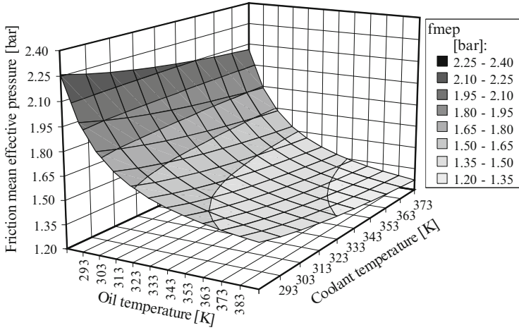
Fig. 10.4 Friction map calculated for a 1.9 l diesel engine at 2,300 rpm, 40 Nm
