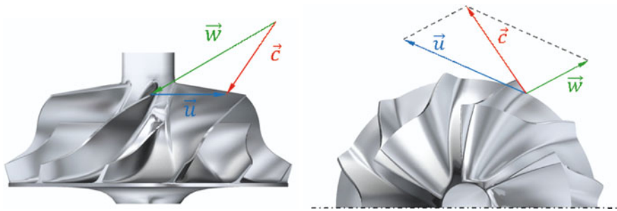
Fig. 15.2 Velocity triangles at the inlet and the outlet of a radial compressor
