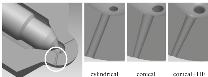
Fig. 4.15 Standard designs of blind hole nozzles
