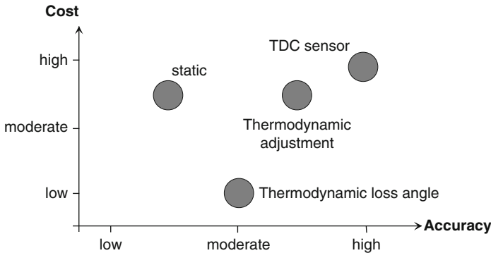
Fig. 3.27 Comparison of cost and accuracy of different TDC determination methods
