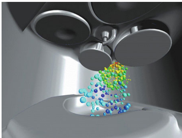
Fig. A.4 Visualization of DI gasoline engine spray simulation results
