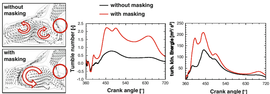
Fig. 12.11 Representation of the flow field during charge changing with and without masking. As a result of the directed tumble motion, a considerably higher level of turbulence results at TDCc (720°) with inlet valve masking TDCc
