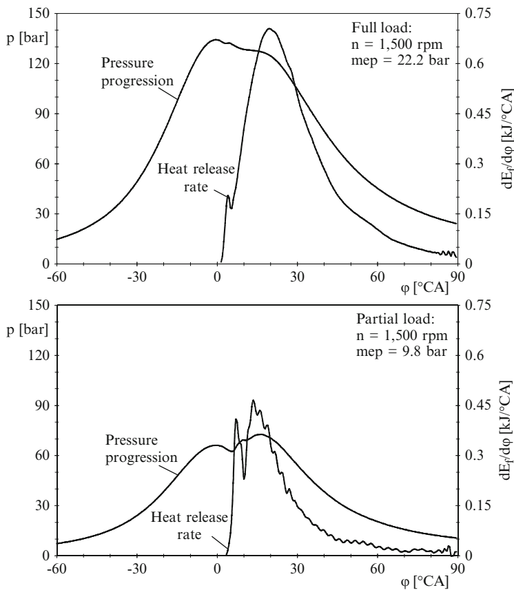
Fig. 4.22 Pressure profile and heat release rate in a high speed diesel engine at full and partial loads
