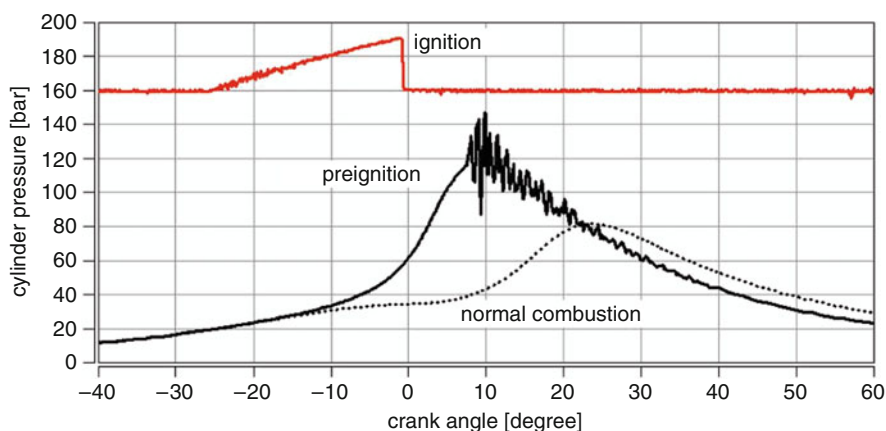
Fig. 4.31 Examples of pressure profiles with preignitions
