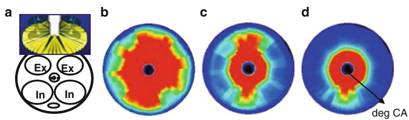
Fig. 3.47 Flame pattern signals in a GDI engine (a): sensor configuration, (b): injection early, sooting combustion of piston wall film, (c): late injection results in diffusion flame near liner, (d): best calibration with residual diffusion flames underneath injector
