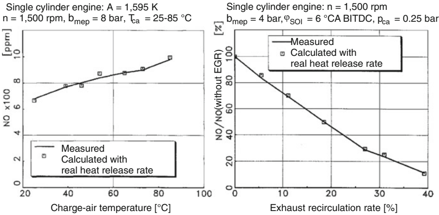
Fig. 7.23 Influence of the charge air temperature ( left ) and the exhaust gas recirculation rate ( right ) on the NO formation rate
