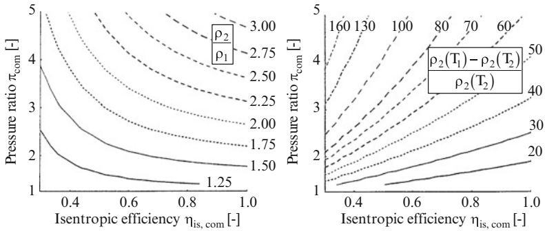
Fig. 8.38 Density ratio due to isentropic compression (left) and percentual density factor due to recooling (right)
