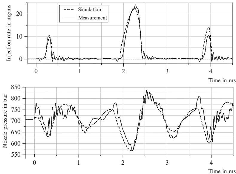
Fig. 7.39 Simulated and measured injection rates and nozzle pressure profiles of a modern piezo-diesel injector
