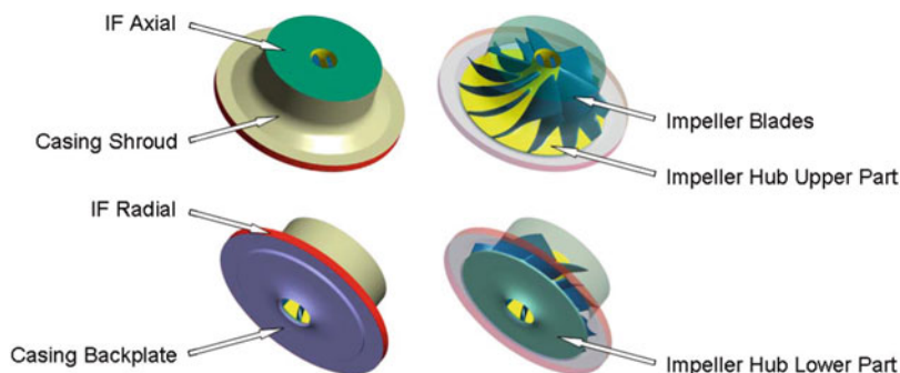
Fig. 15.6 Boundary and edge surfaces in the impeller area
