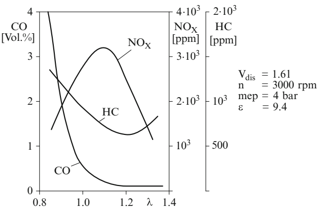
Fig. 6.1 Pollutant formation as a function of the equivalence ratio
