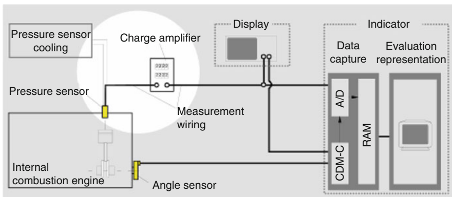
Fig. 3.3 Schematic design of the piezoelectric pressure measurement chain with additional components
