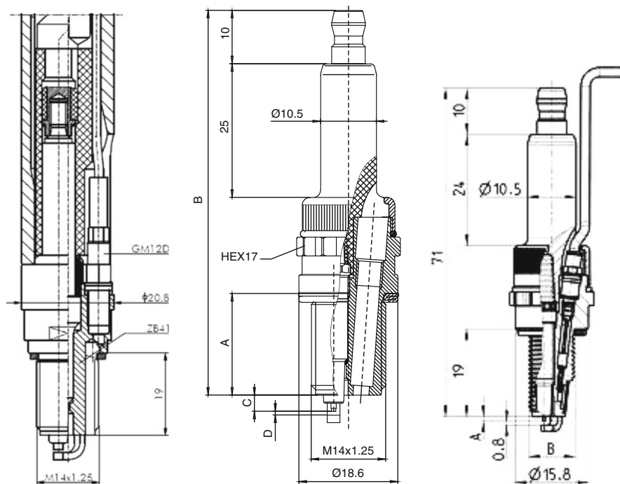
Fig. 3.16 Different measuring spark plug designs (AVL)
