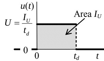
Figure 8-2 Flat impulse
