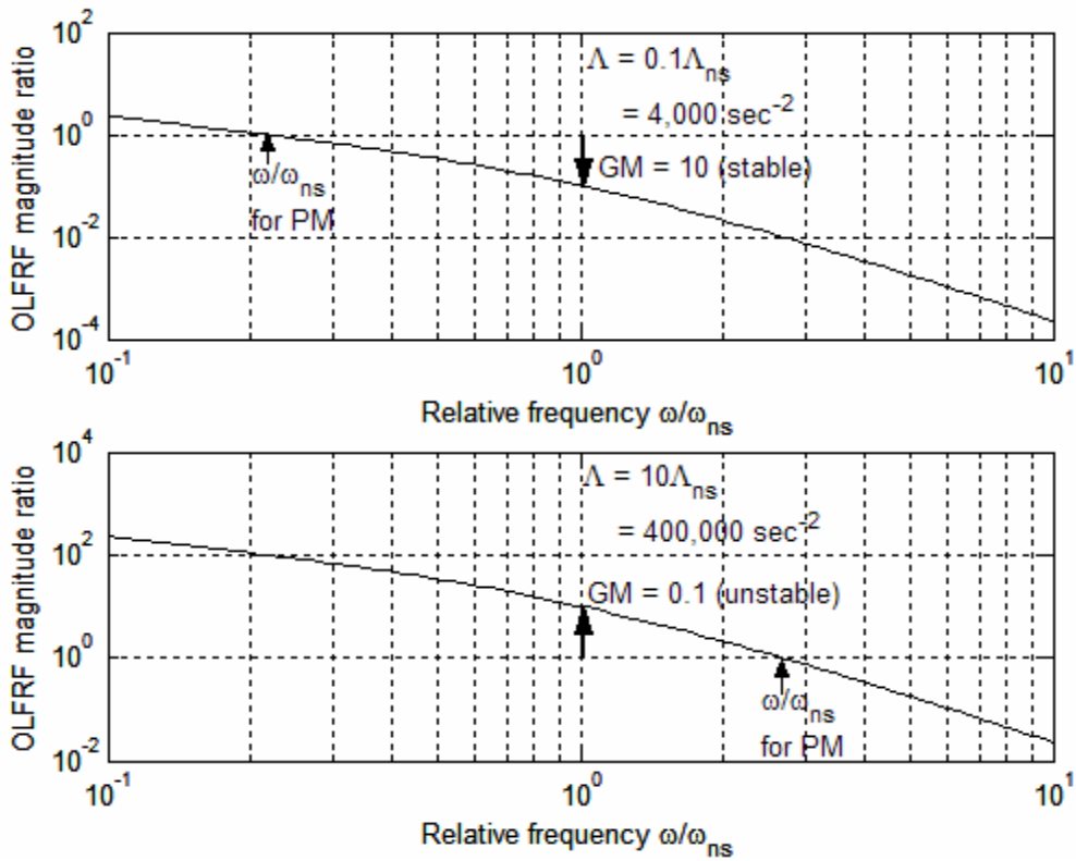
Figure 17-3 Magnitude ratios, Eq. (17-5) for \Lambda = 4,000 and 400,000 \text{ sec}^{-2}
