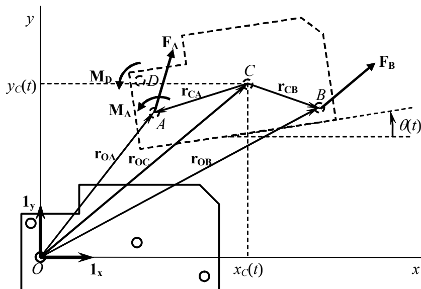
Figure 11-1 Rigid body in general plane motion
