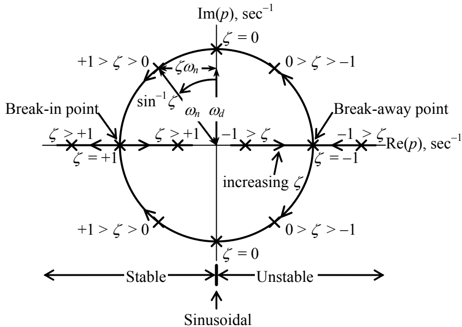
Figure 16-5 Loci of roots of p^2 + 2\zeta\omega_n p + \omega_n^2 = 0 as \zeta varies from less than -1 to greater than +1 , with \omega_n > 0 held constant
