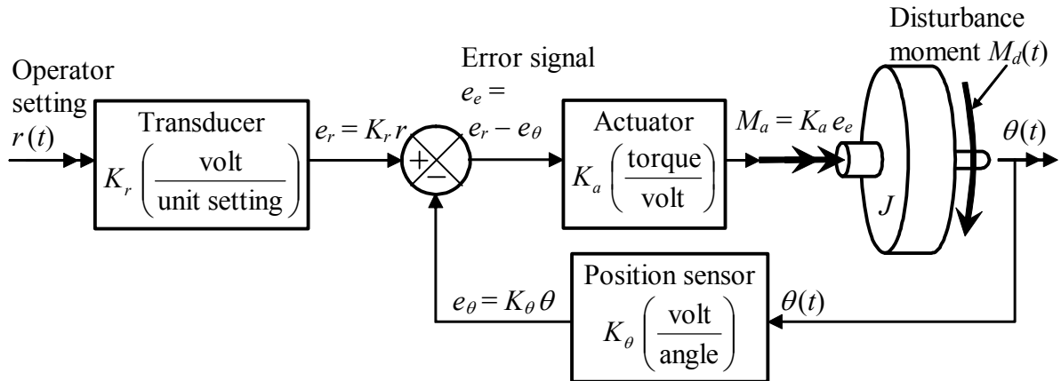
Figure 14-5 Functional diagram of position-feedback control system
