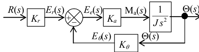
Figure 14-7 Laplace block diagram of SISO position-feedback control system
