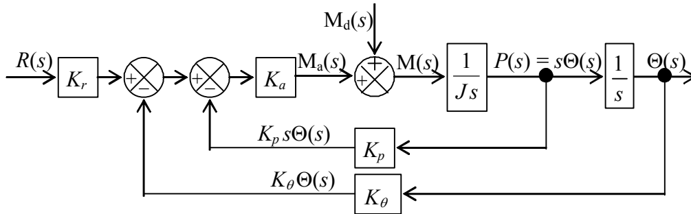
Figure 14-12 Laplace block diagram of rotor-position control system with both position feedback and rate feedback
