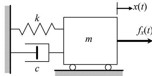
Figure 7-1 Mass-damper-spring system
