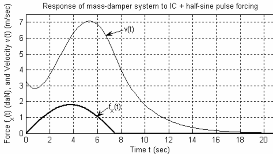
Figure 1-2 Excitation and response of a mass-damper system
