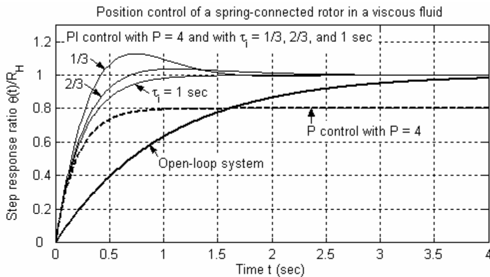
Figure 15-6 Step responses for no control (open-loop), proportional (P) control, and proportional-integral (PI) control
