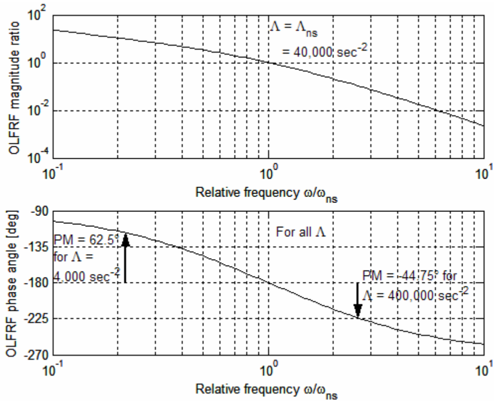
Figure 17-2 Modified Bode diagram, Eq. (17-5), frequency response for \Lambda = \Lambda_{ns} = 40,000 \text{ sec}^{-2} of the open-loop system in Fig. 17-1
