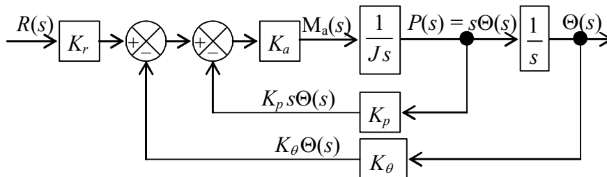
Figure 14-13 Laplace block diagram of SISO rotor-position control system with both position feedback and rate feedback
