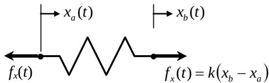
Figure 3-7 Ideal linear spring with stiffness constant k
