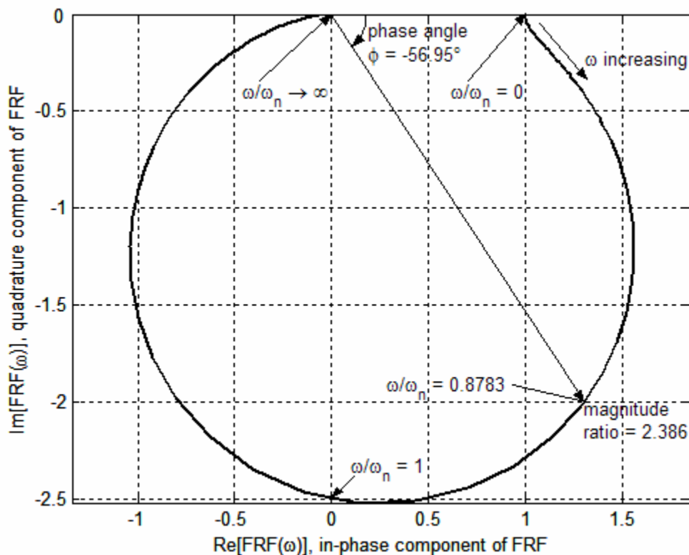
Figure 17-5 Nyquist plot of FRF(\omega) = \omega_n^2/(\omega_n^2 - \omega^2 + j2\zeta\omega_n\omega) for \omega_n = 2\pi rad/sec and \zeta = 0.2
