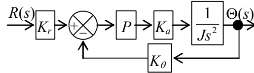
Figure 15-7 Proportional control of rotor position
