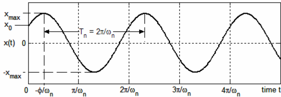
Figure 7-2 IC response of an undamped 2 nd order system
