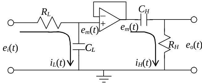
Figure 5-10 RC band-pass filter
