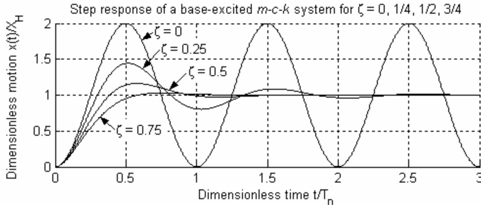
Figure 13-4 (repeated) Base-excitation control of mass position for an m - c - k system
