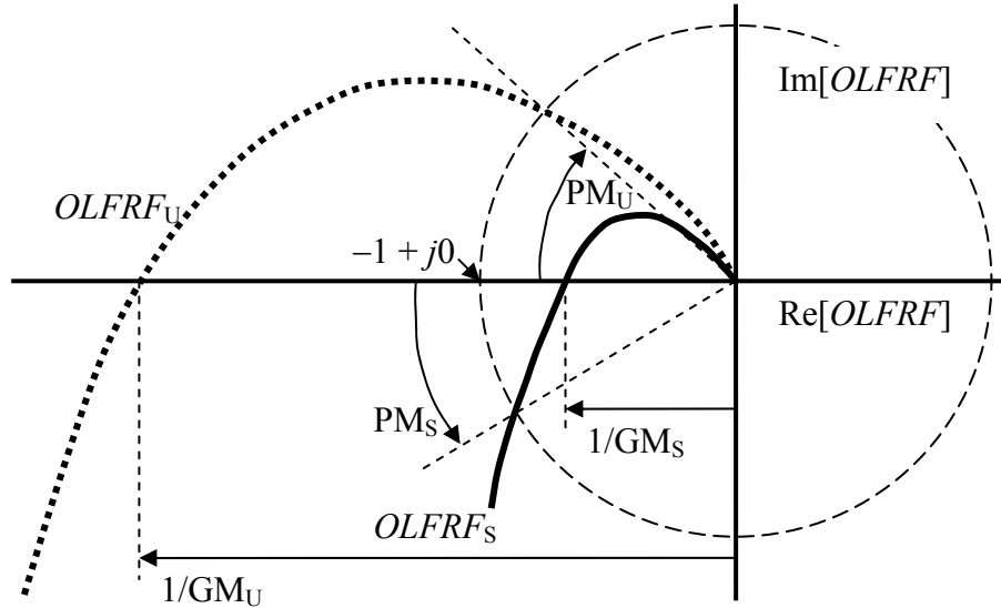
Figure 17-8 Schematic Nyquist plots of open-loop frequency-response functions (OLFRF) for closed-loop-stable and -unstable cases
