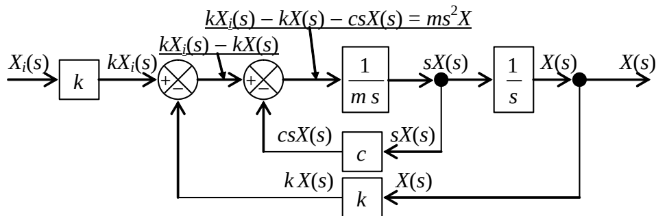
Figure 13-3 Laplace block diagram with feedback branches for a base-excited m - c - k system
