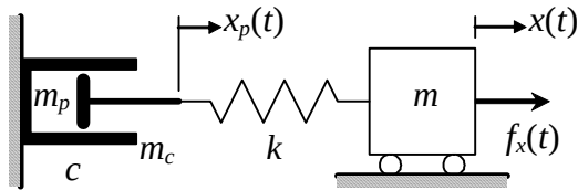
Series mass-dashpot-spring system
