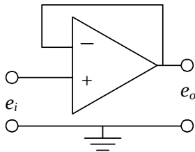
Figure 5-9 Voltage follower
