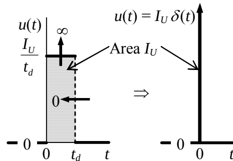
Figure 8-3 Ideal impulse
