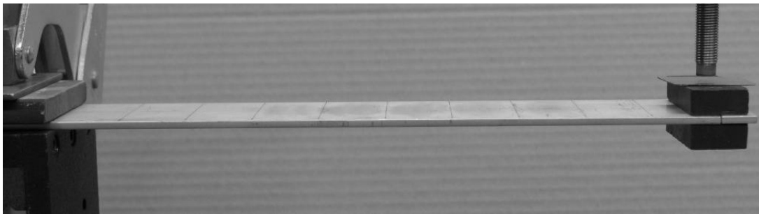
Figure 7-10 Structural system of Fig. 7-6, with the addition at the beam tip of two ceramic magnets and an aluminum spacer. Note the same steel-plate tip-target for the proximity sensor as on Fig. 7-6.
