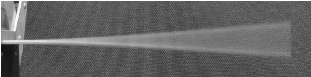
Figure 7-8 Edge-on, \frac{1}{4} -second exposure photo of the beam of Fig. 7-6 vibrating after an initial static deformation and release of the beam tip.
