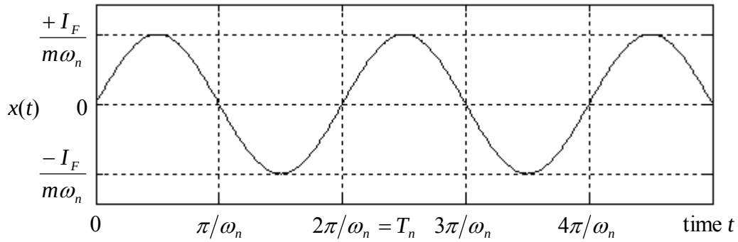
Figure 8-4 Ideal impulse response of a mass-spring system
