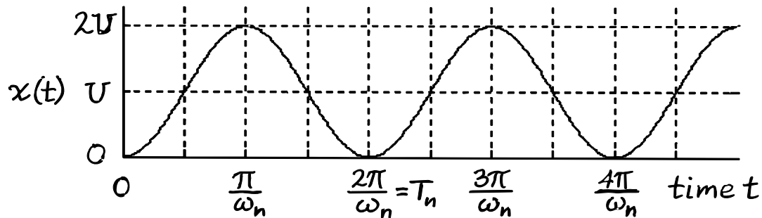
Figure 7-3 Step response of an undamped 2 nd order system
