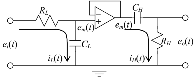
Figure 5-10 RC band-pass filter (repeated)
