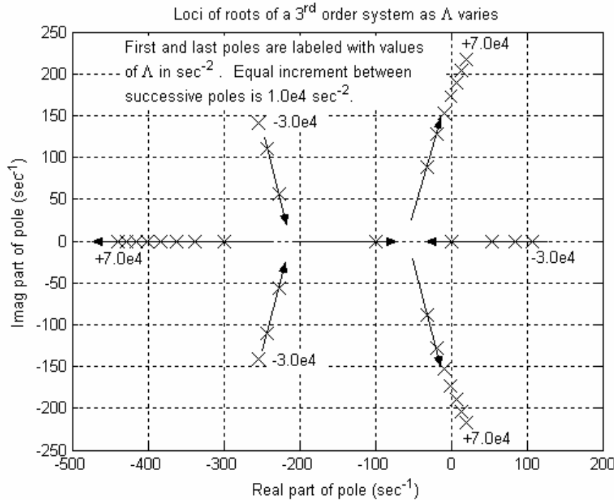
Figure 16-7 First-pass loci of roots of Eq. (16-51a) for varying control parameter \Lambda = K_a K_\theta / J
