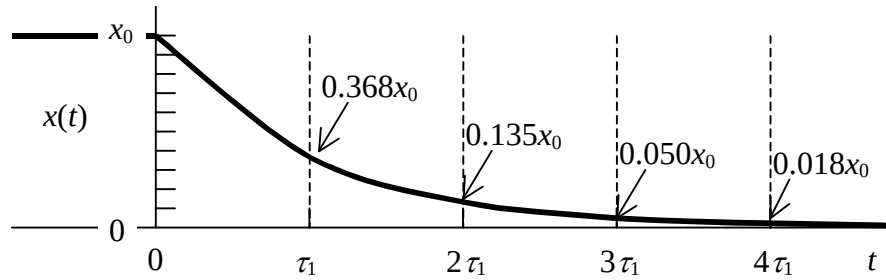
Figure 3-2 1 st order initial-condition response
