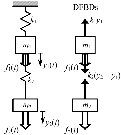
Figure 12-2 Two-mass-two-spring mechanical system
