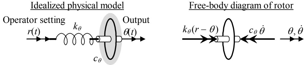
Figure 15-3 Lightweight rotor immersed in a viscous liquid, with connection to the input through a soft torsion spring
