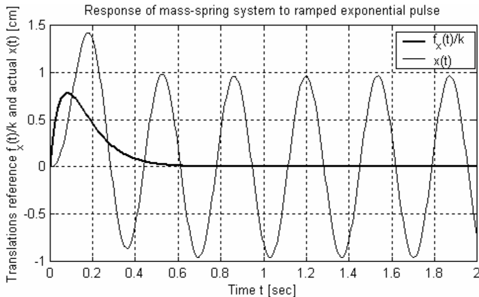
Figure 1-5 Excitation and response of a mass-spring system
