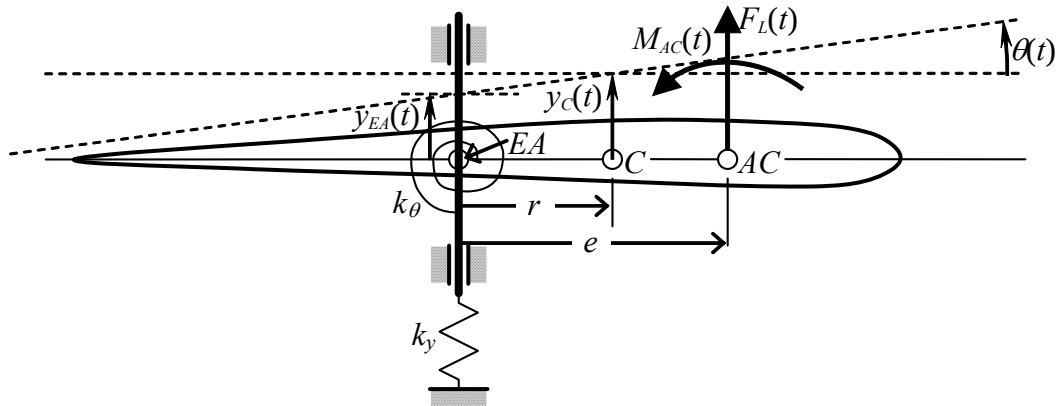
Figure 11-5 Example 11-3: 2-DOF typical section
