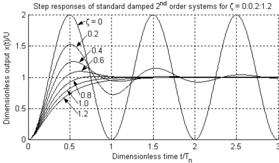
Figure 9-7 Step responses of standard 2 nd order systems as viscous damping varies
