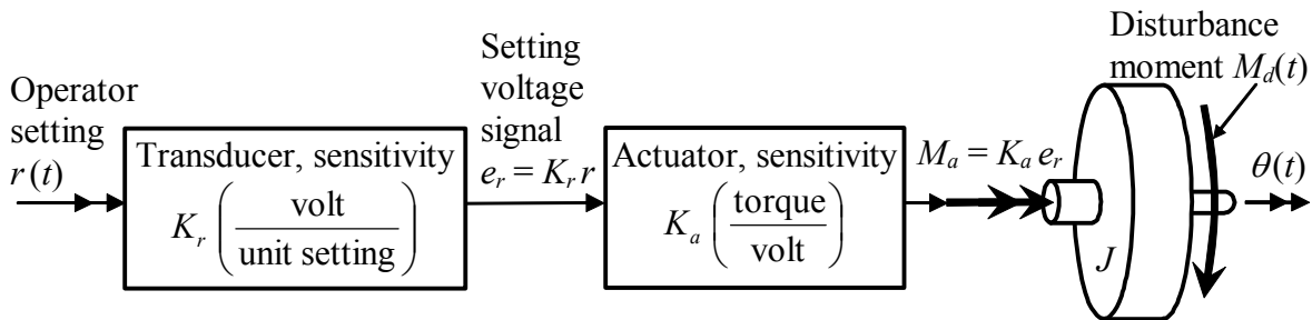
Figure 14-2 Functional diagram of open-loop rotor-position control system
