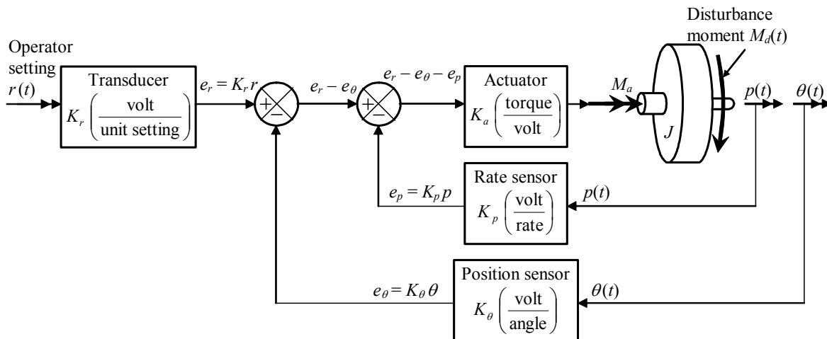
Figure 14-11 Functional diagram of rotor-position control system with both position feedback and rate feedback
