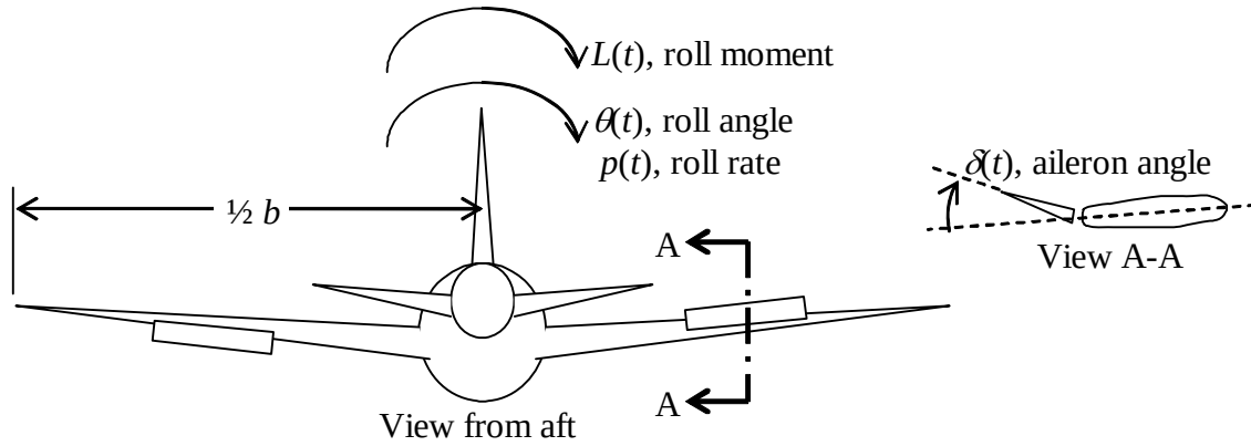
Figure 3-4 Aileron-induced rolling of an airplane
