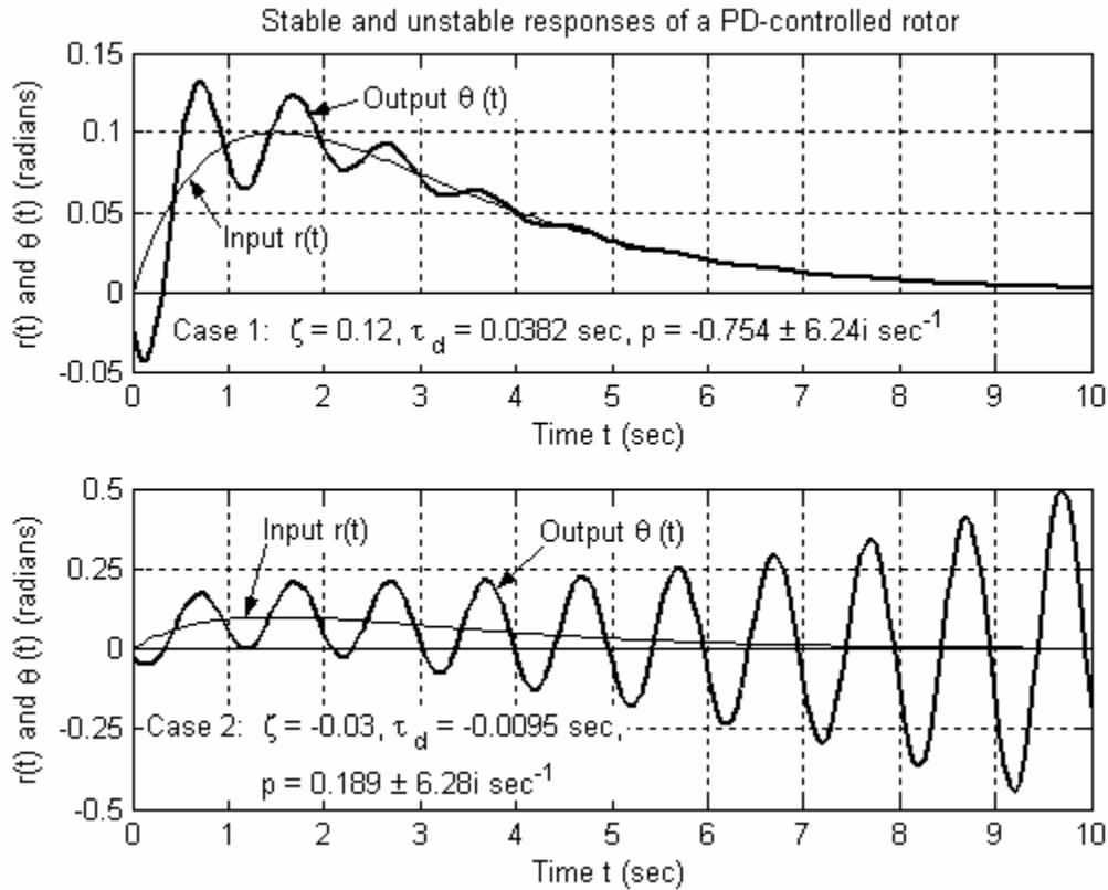
Figure 16-1 Ramped-exponential input operator setting r(t) and output rotor positions \theta(t) for an ideal proportional-derivative (PD) controlled rotor, with two different derivative time constants
