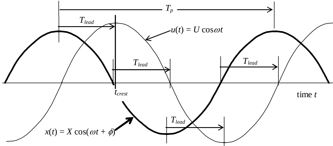
Figure 4-3 Frequency response phase measurement from time-history graphs
