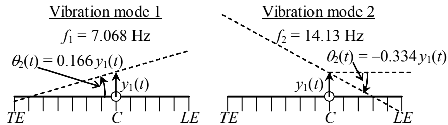
Figure 12-6 Vibration modes of the example typical section
