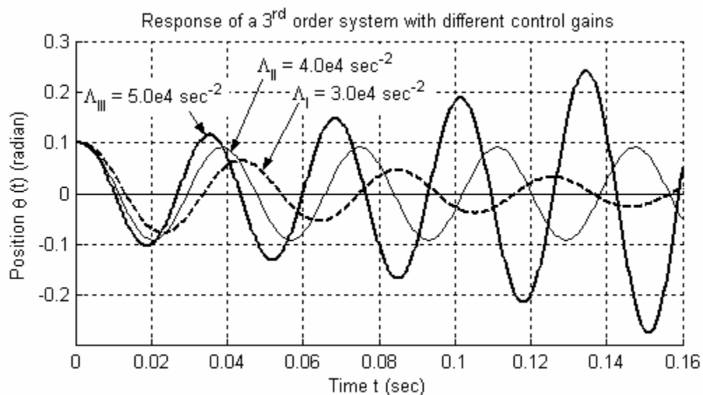
Figure 16-4 Initial-condition response of a rotor output-position-feedback control system with a 1 st order low-pass filter in the feedback branch
