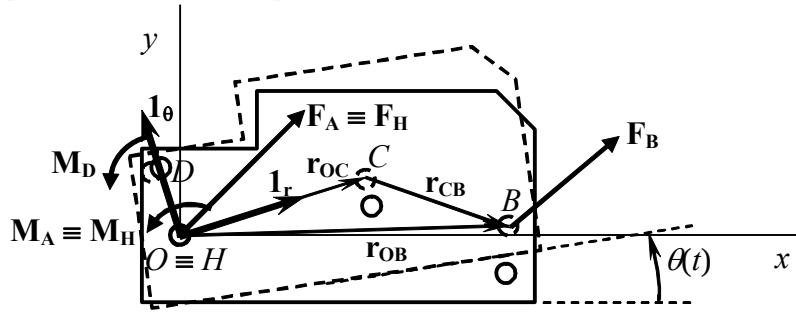
Figure 11-2 Rigid body in pure rotation about point O
