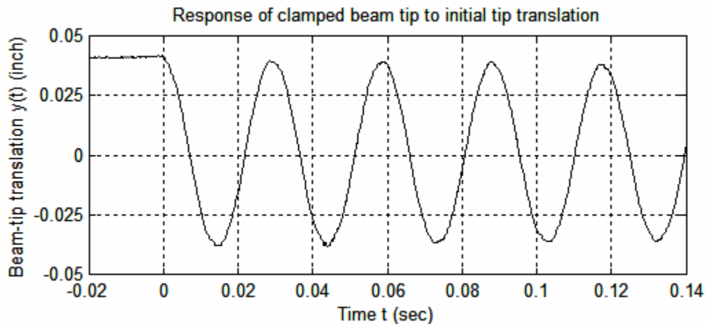
Figure 7-7 Initial-translation dynamic response of the beam in Fig. 7-6, as detected by the proximity sensor.
