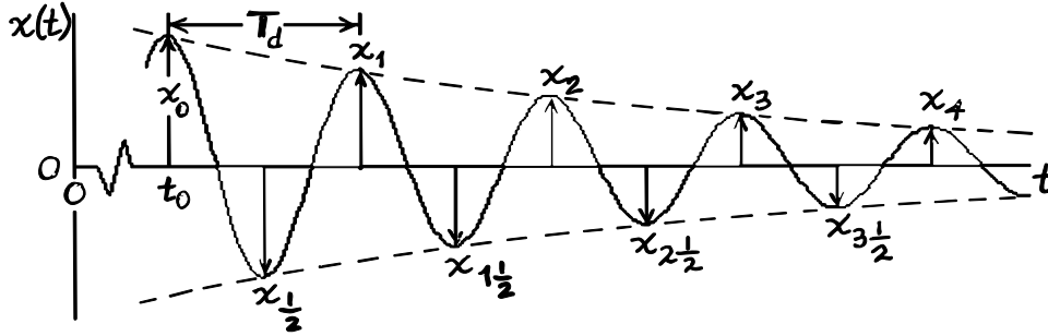
Figure 9-3 Free-vibration response of a damped 2 nd order system
