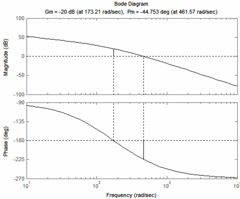
Figure 17-4 MATLAB’s traditional Bode diagram, Eq. (17-5), frequency response for \Lambda = 10\Lambda_{ns} = 400,000 \text{ sec}^{-2} of the open-loop system in Fig. 17-1
