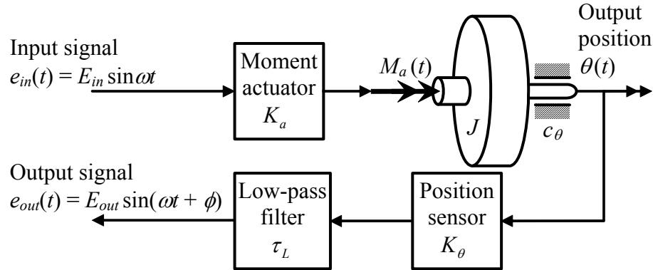
Figure 17-1 Functional diagram of frequency-response testing of the open-loop portion of Figs. 16-2 and 16-3
