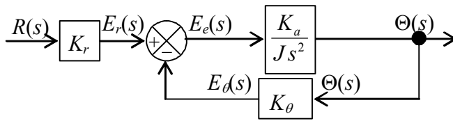
Figure 14-7a (repeated) Laplace block diagram of SISO position-feedback control system
