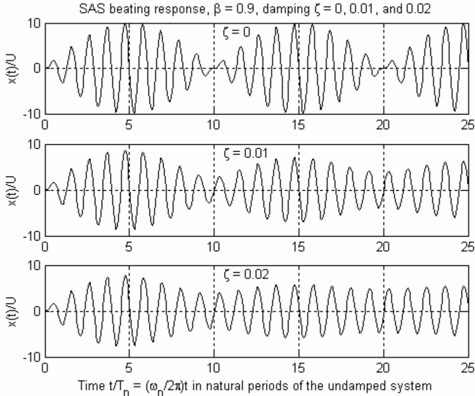
Figure 10-4 Calculations of Eq. (10-43) for a standard 2 nd order system having undamped natural frequency \omega_n , with zero damping (top) and two positive values of viscous damping ratio, \zeta = 0.01 and 0.02 ; response from rest initial conditions to a suddenly applied (at t = 0 ) sinusoidal (SAS) excitation with frequency \omega = 0.9\omega_n .
