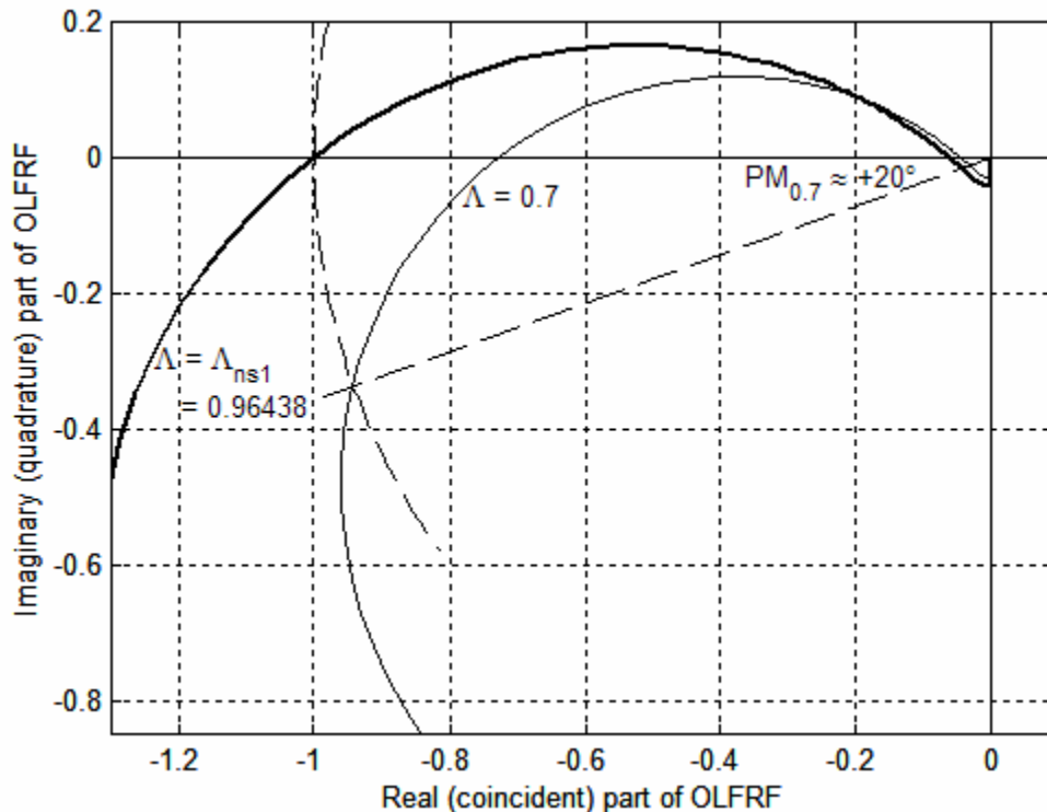
Figure 17-10 Nyquist plots, Eq. (17-20), open-loop frequency-response functions (OLFRF) for \Lambda = 0.7 and \Lambda = \Lambda_{ns1} = 0.96438 in the system of Eq. (17-18)
