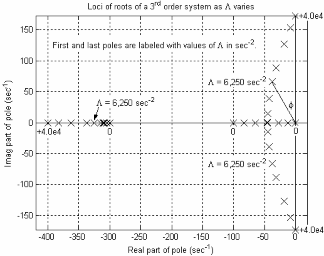
Figure 16-8 Refined loci of roots of Eq. (16-51a) for varying control parameter \Lambda = K_a K_\theta / J
