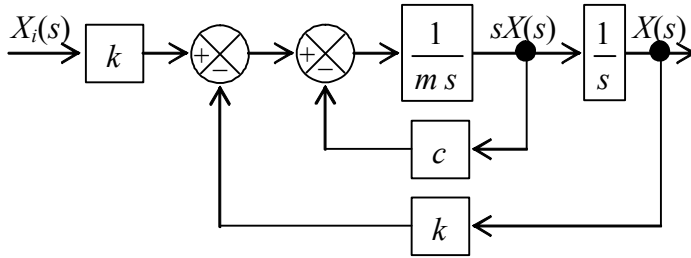
Figure 14-9 Laplace block diagram with feedback branches for a base-excited m - c - k system
