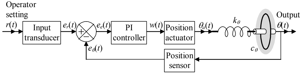
Figure 15-4 Functional diagram of a system for controlling the position of a spring-connected rotor in a viscous liquid, based on proportional-integral control
