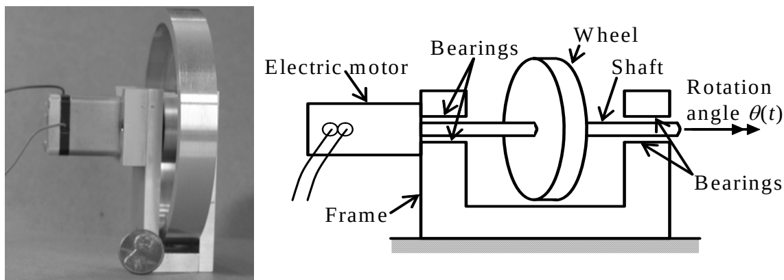
Figure 3-1 Laboratory reaction-wheel assembly: photograph at left, schematic drawing at right
