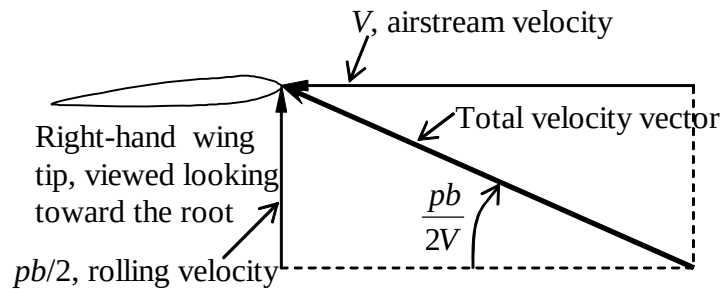
Figure 3-5 Angle of attack induced by rolling velocity
