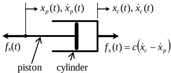
Figure 3-8 Ideal linear, viscous dashpot with damping constant c
