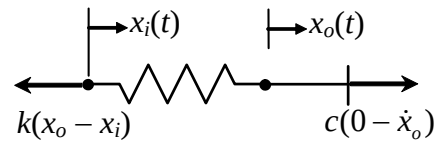
Figure 3-12 Series damper-spring idealized mechanical filters
