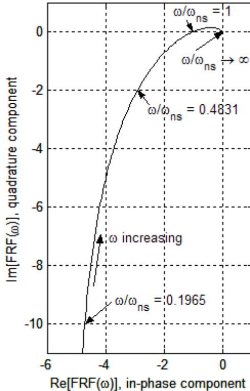
Figure 17-6 Nyquist plot, Eq. (17-5), frequency response for \Lambda = \Lambda_{ns} = 40,000 \text{ sec}^{-2} of the open-loop system in Fig. 17-1, with parameters \omega_b = 300 \text{ sec}^{-1} , c_\theta/J = 100 \text{ sec}^{-1} , and \omega_{ns} = \sqrt{(\omega_b \times c_\theta/J)} = 173.2 \text{ rad/sec}
