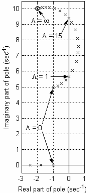
Figure 17-9 Loci of roots of Eq. (17-19)
