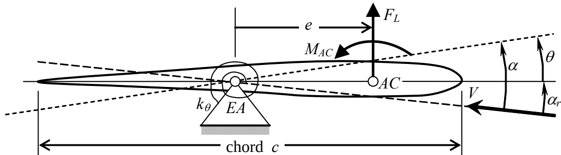
Figure 11-4 Example 11-2: 1-DOF typical section in an airstream
