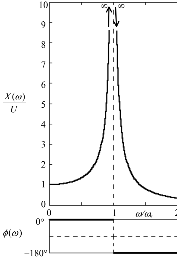
Figure 10-1 Frequency response function of an undamped 2 nd order system
