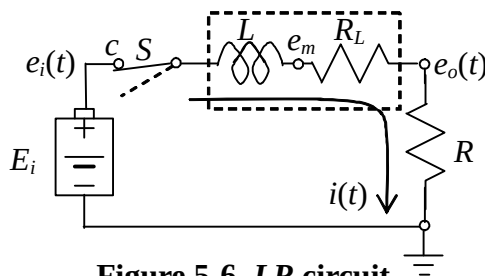
Figure 5-6 LR circuit
