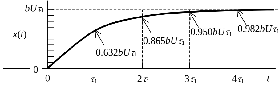
Figure 3-3 1 st order step response
