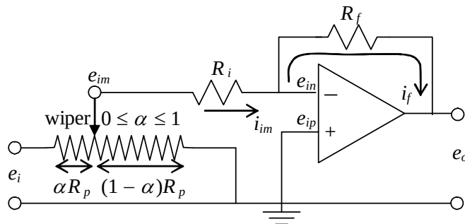
Inverting amplifier with coefficient-setting potentiometer
