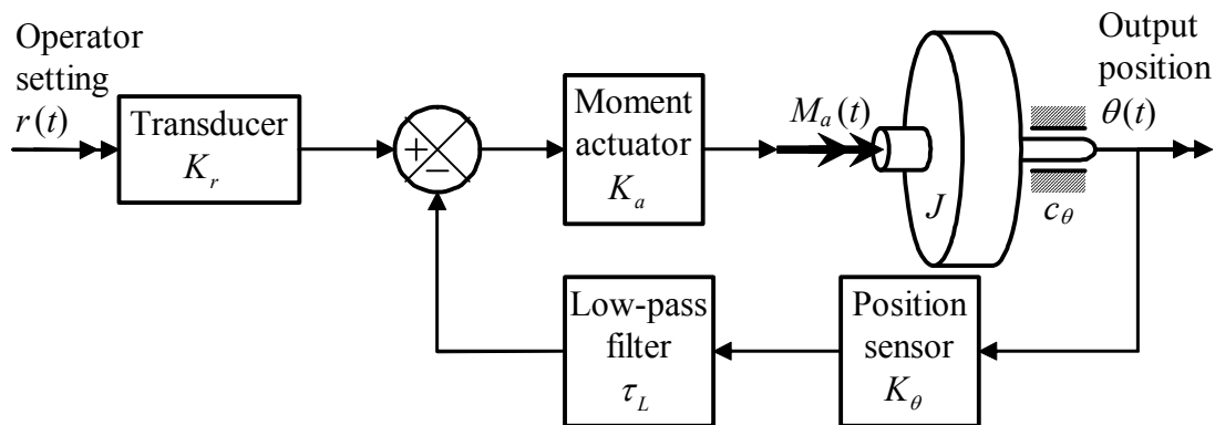
Figure 16-2 Functional diagram of a rotor position-feedback control system with a 1 st order low-pass filter in the feedback branch
