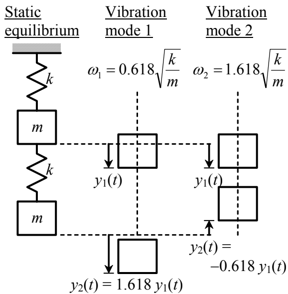
Figure 12-3 Vibration modes of the 2-DOF mass-spring system that has equal masses and equal springs
