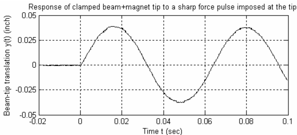
Figure 7-11 Dynamic response to a hammer tap at time t = 0 sec of the beam on Fig. 7-10, as detected by the proximity sensor.
