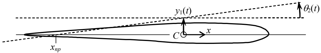
Figure 12-5 Nodal point of the 2-DOF typical section in a mode of vibration
