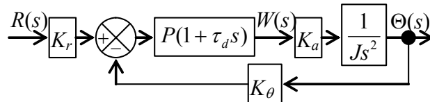
Figure 15-8 Ideal proportional-derivative (PD) control of rotor position
