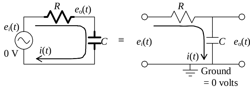
Figure 5-3 RC low-pass filter circuit
