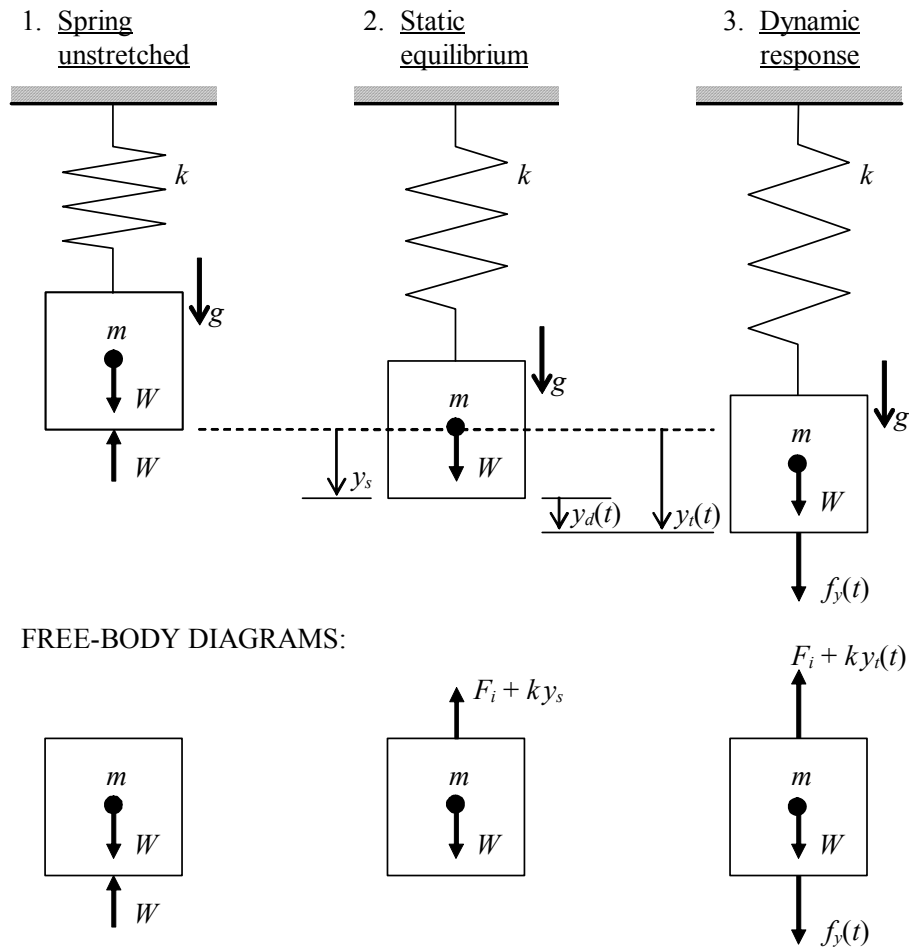
Figure 7-4 Static and dynamic positions of a hanging, spring-supported weight
