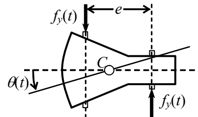
Figure 14-3 Pitch control of a re-entry capsule
