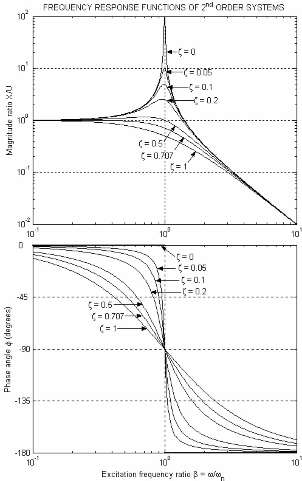
Figure 10-2 Frequency response functions for standard 2 nd order systems with viscous damping ratios \zeta varying from 0 to 1
