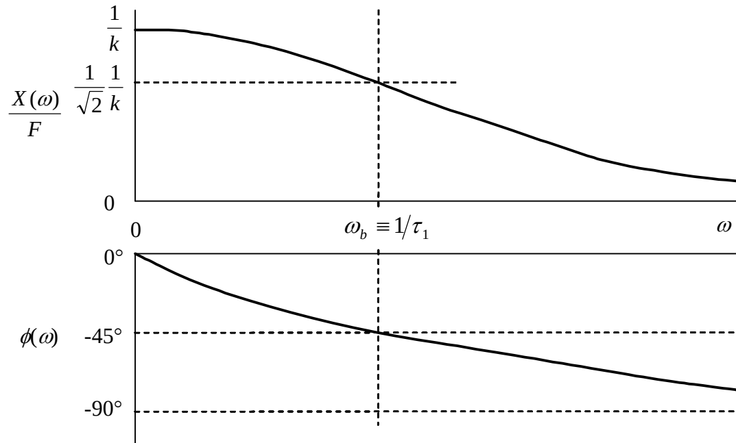
Figure 4-1 Frequency-response function of 1 st order damper-spring system
