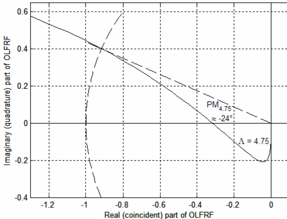
Figure 17-11 Nyquist plot, Eq. (17-20), open-loop frequency-response function (OLFRF) for \Lambda = 4.75 in the system of Eq. (17-18)
