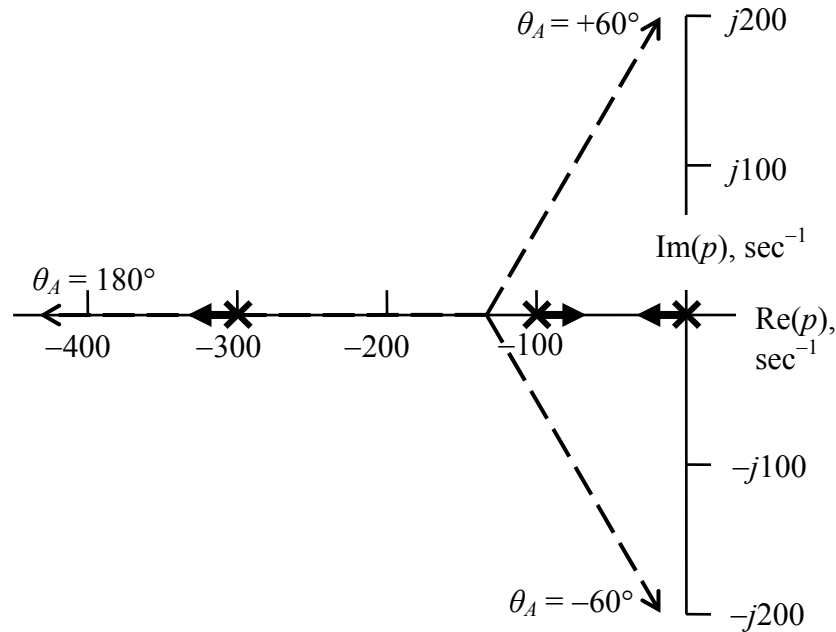
Figure 16-9 Example of information about loci of roots that is provided by the open-loop poles
