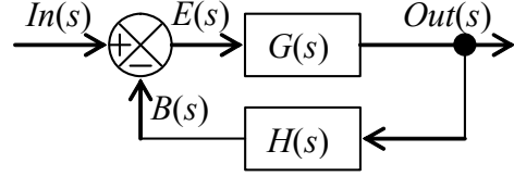
Fig. 14-8 (repeated) Laplace block diagram of general closed loop
