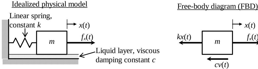
Figure 1-3 2 nd order mass-damper-spring mechanical system
