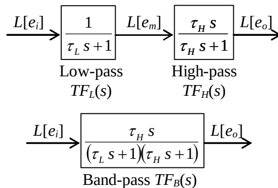
Figure 13-1 Laplace block diagrams of the RC band-pass filter
