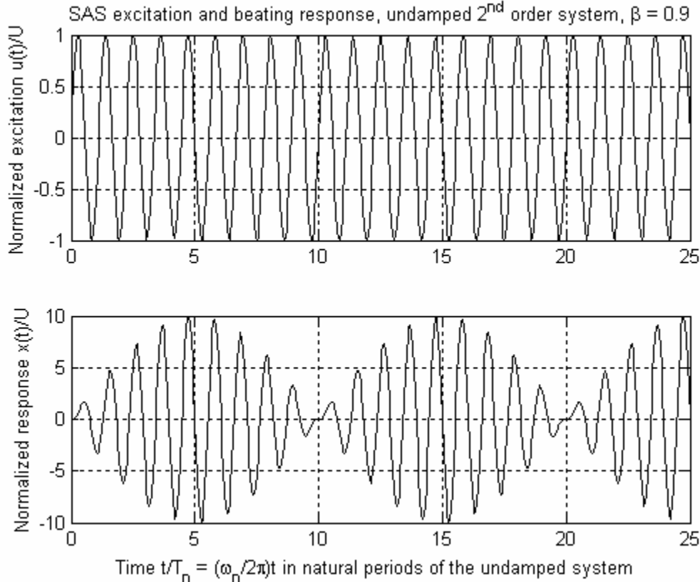
Figure 10-3 Upper graph: suddenly applied (at t = 0 ) sinusoidal (SAS) excitation with frequency \omega = 0.9\omega_n ; lower graph: response from zero initial conditions of a standard undamped 2 nd order system having natural frequency \omega_n .
