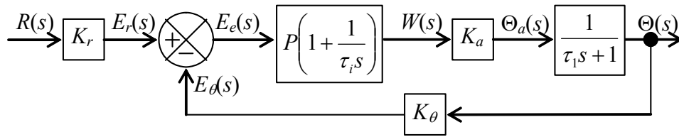
Figure 15-5 Laplace block diagram of a system for controlling the position of a spring-connected rotor in a viscous liquid, based on proportional-integral
