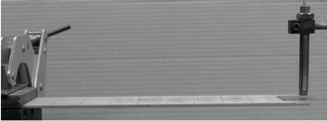
Figure 7-6 Clamped uniform aluminum beam with nominal cross section 2 inch \times 1/8 inch. Test configuration: beam clamped at left between thick steel plates, leaving 10.0 inches of overhang; non-contacting proximity (displacement) sensor over right tip; bonded onto the beam's right tip is a small, thin, steel plate, the "target" in which the proximity sensor induces eddy currents.
