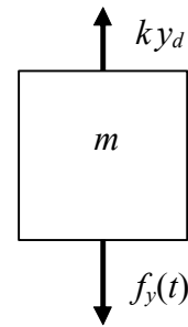
Figure 7-5 Dynamic free-body diagram
