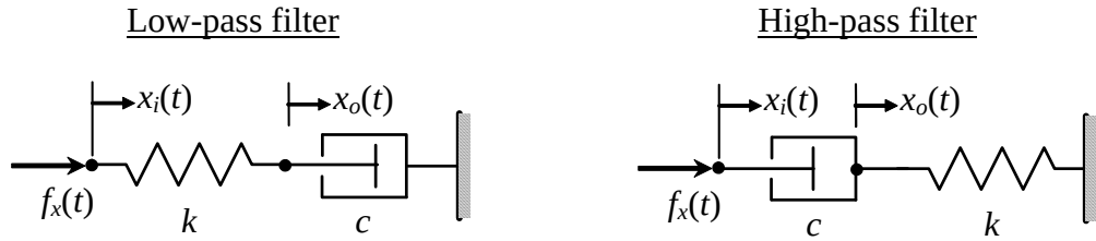
Figure 3-12 Series damper-spring idealized mechanical filters
