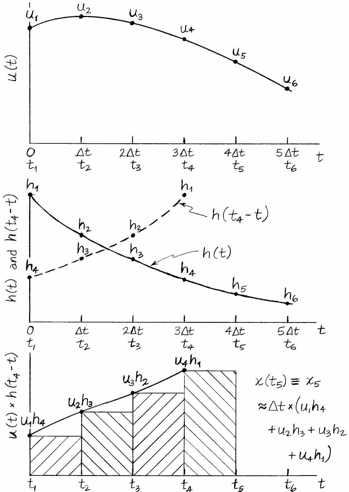
Figure 8-6 Graphical representation of the convolution sum for a conceptual problem with input function u(t) and impulse-response function h(t) , with h(0) \neq 0
