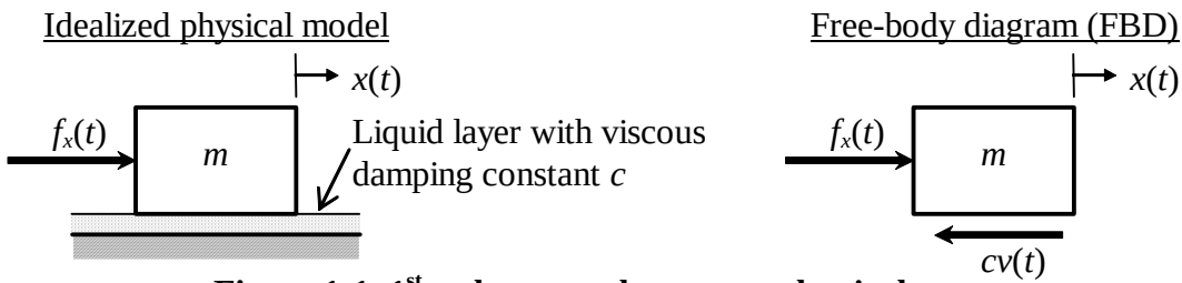
Figure 1-1 1 st order mass-damper mechanical system
