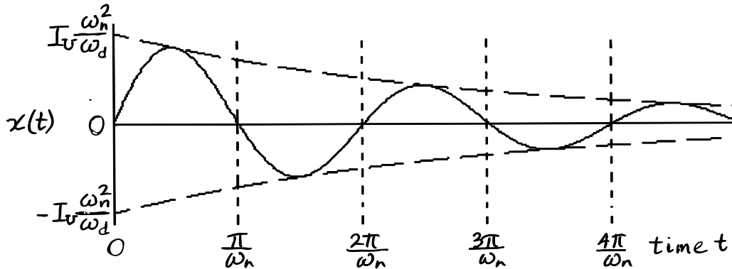
Figure 9-5 Ideal impulse response of a damped 2 nd order system, \zeta = 0.11
