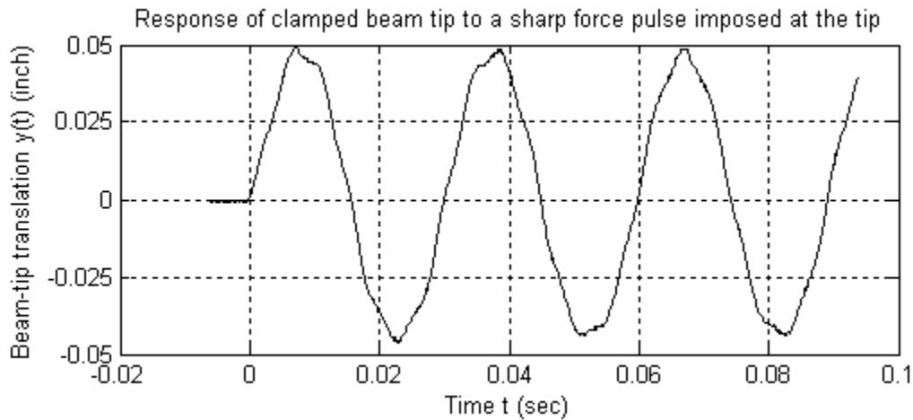
Figure 7-9 Dynamic response to a hammer tap at time t = 0 sec of the beam on Fig. 7-6, as detected by the proximity sensor.
