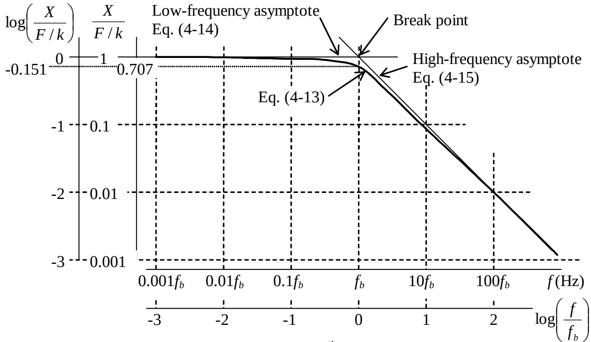
Figure 4-2 Log-log magnitude ratio of 1 st order damper-spring system
