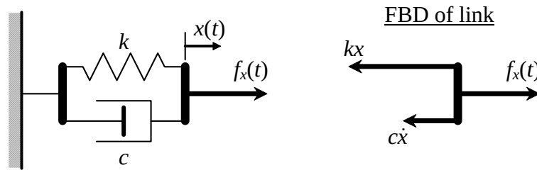
Figure 3-10 Parallel damper-spring system
