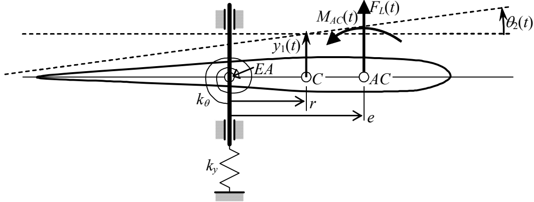
Figure 12-4 2-DOF typical section
