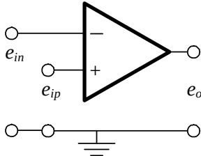
Figure 5-7 Operational amplifier (op-amp)
