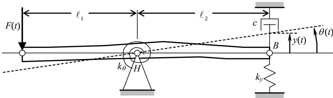
Figure 11-3 Example 11-1: damped, spring-supported, hinged rigid bar
