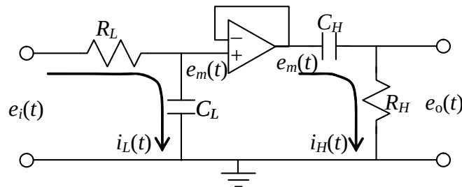
Figure 5-10 (repeated) RC band-pass filter
