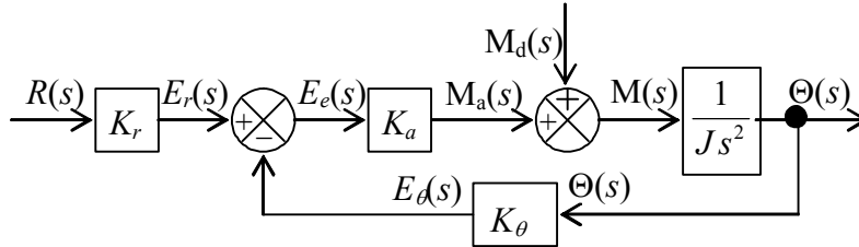
Figure 14-6 Laplace block diagram, including disturbance input, of position-feedback control system
