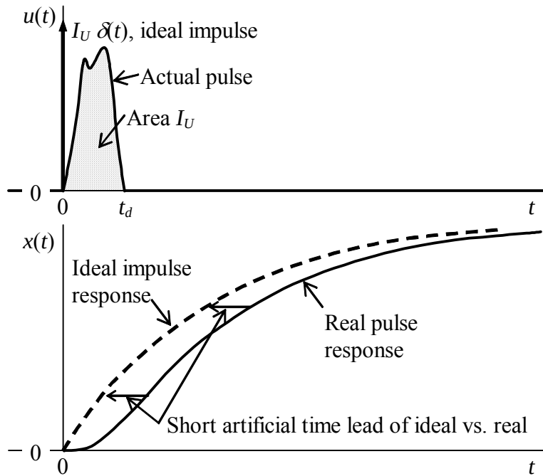
Figure 8-5 Conceptual ideal impulse response and real pulse response for an undamped 2 nd order system
