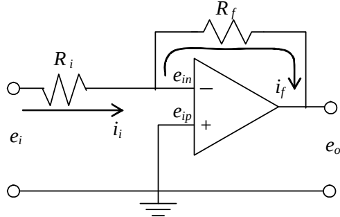
Figure 5-8 Inverting amplifier
