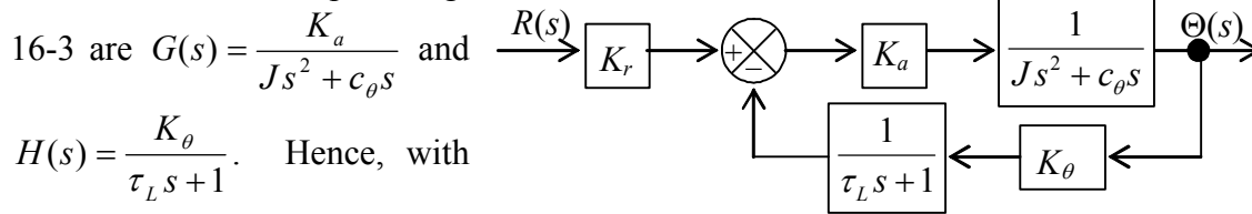
Figure 16-3 Laplace block diagram of position-feedback control system with low-pass filtering
