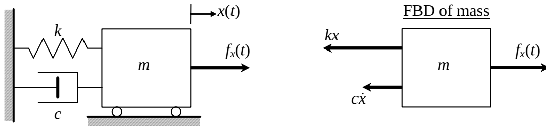
Figure 3-9 Mass-damper-spring system
