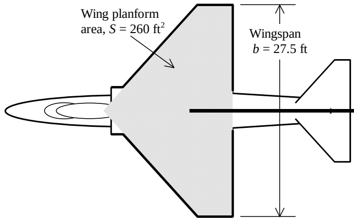
Planform sketch of A4D fighter airplane
