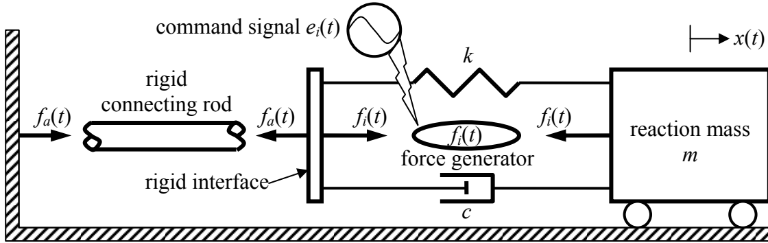
Reaction-Mass Actuator (RMA) in a calibration setup
