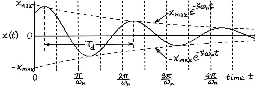
Figure 9-2 IC response of a damped 2 nd order system, \zeta = 0.11
