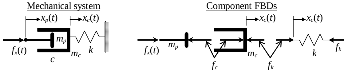
Figure 3-11 Example series mass-dashpot-spring
