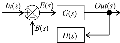
Figure 14-8 Laplace block diagram of general closed loop
