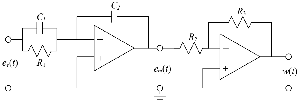
Figure 15-2 Electronic analog PI controller
