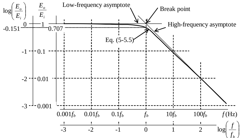
Figure 5-4 Log-log magnitude ratio of 1 st order RC low-pass filter
