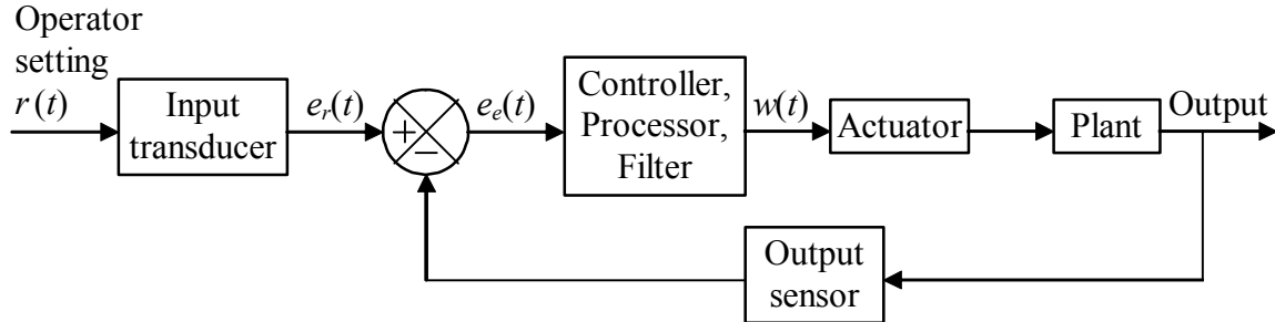
Figure 15-1 Functional block diagram of general control system using input-error operations
