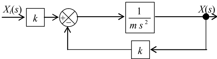
Figure 14-10 Laplace block diagram with feedback branch for a base-excited m - k system
