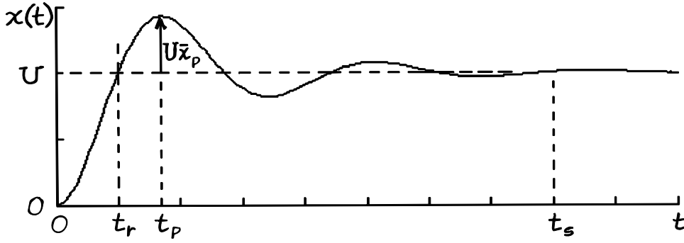
Figure 9-6 Step-response specifications of an underdamped system
