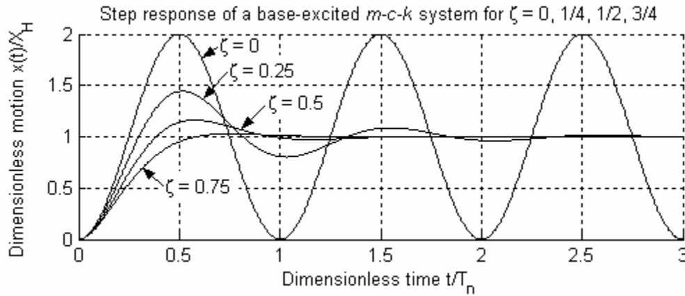
Figure 13-4 Base-excitation control of mass position for an m - c - k system
