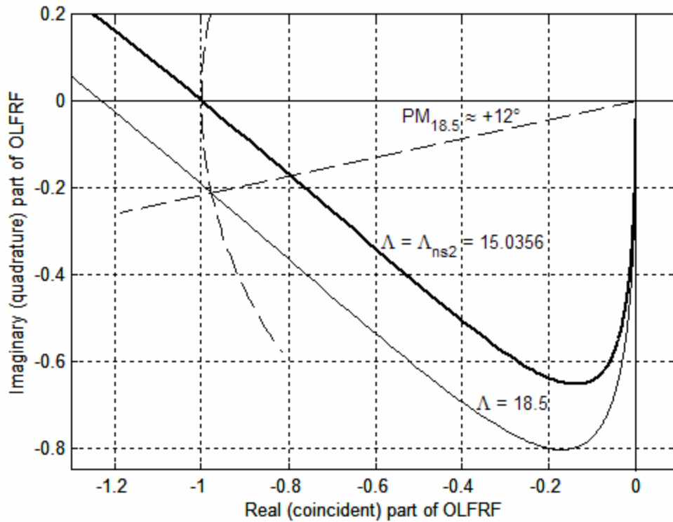
Figure 17-12 Nyquist plots, Eq. (17-20), open-loop frequency-response functions (OLFRF) for \Lambda = \Lambda_{ns2} = 15.0356 and \Lambda = 18.5 in the system of Eq. (17-18)
