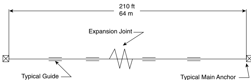
FIGURE 9.2 Expansion joint support calculations example
