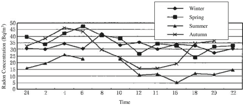
Fig. 29.3 Seasonal and diurnal change of indoor radon concentrations in China (Ren 2001)
