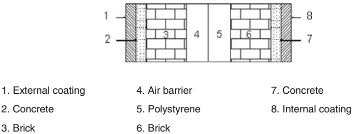
Fig. 27.1 Wall structure
