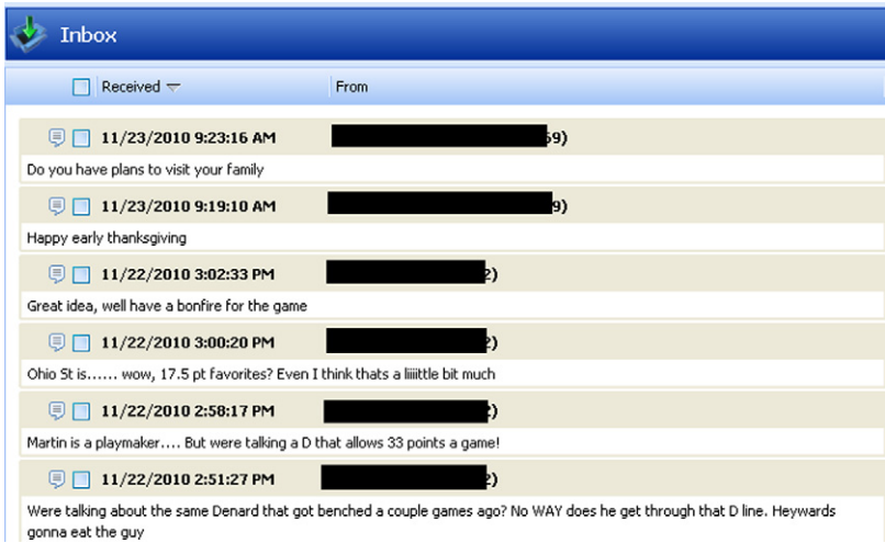
FIGURE 6.27 SMS messages—Inbox.
