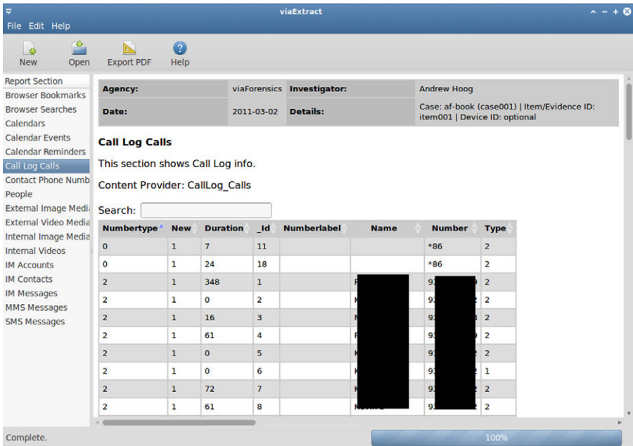
FIGURE 6.63 viaExtract—Call logs.
