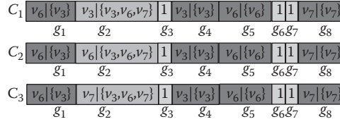
FIGURE 21.18 Illustration of dominatee mutation.
