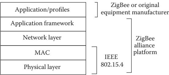
FIGURE 15.3 ZigBee protocol stack.
