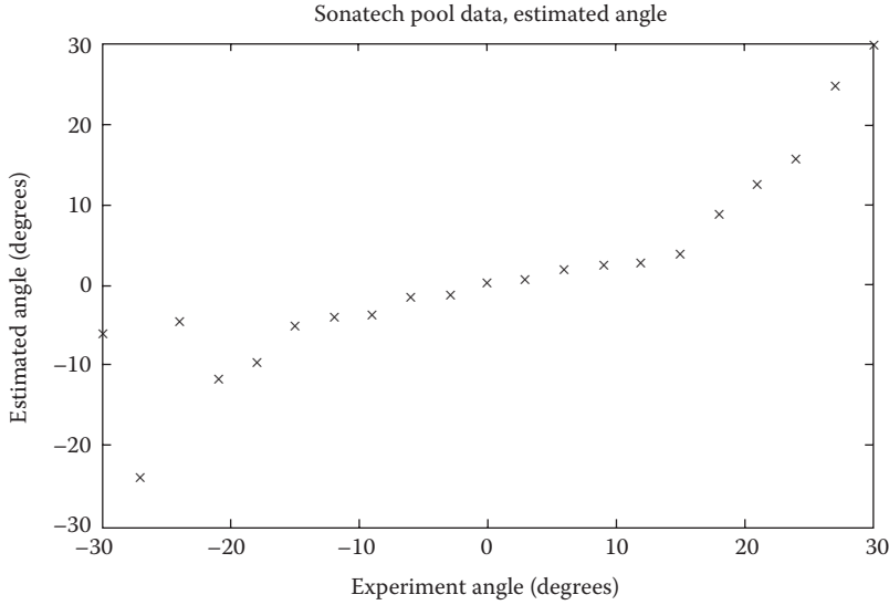
FIGURE 20.8 Estimation of the bearing angles after the nonlinear conversion.
