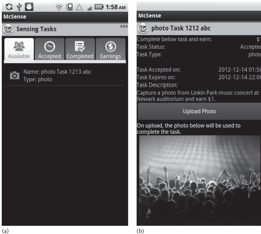
FIGURE 3.2 McSense android application showing tabs (a) and task screen for a photo task (b).
