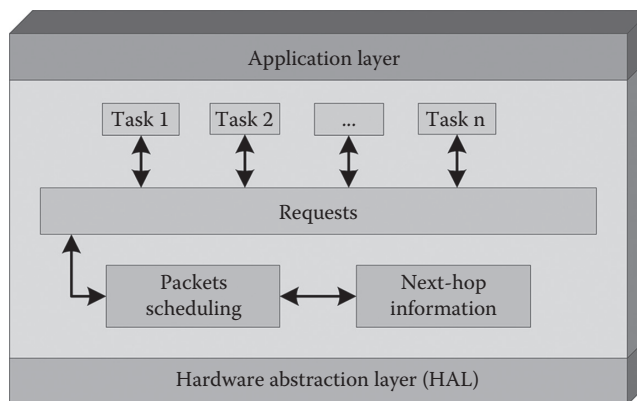
FIGURE 5.9 Multitask architecture.
