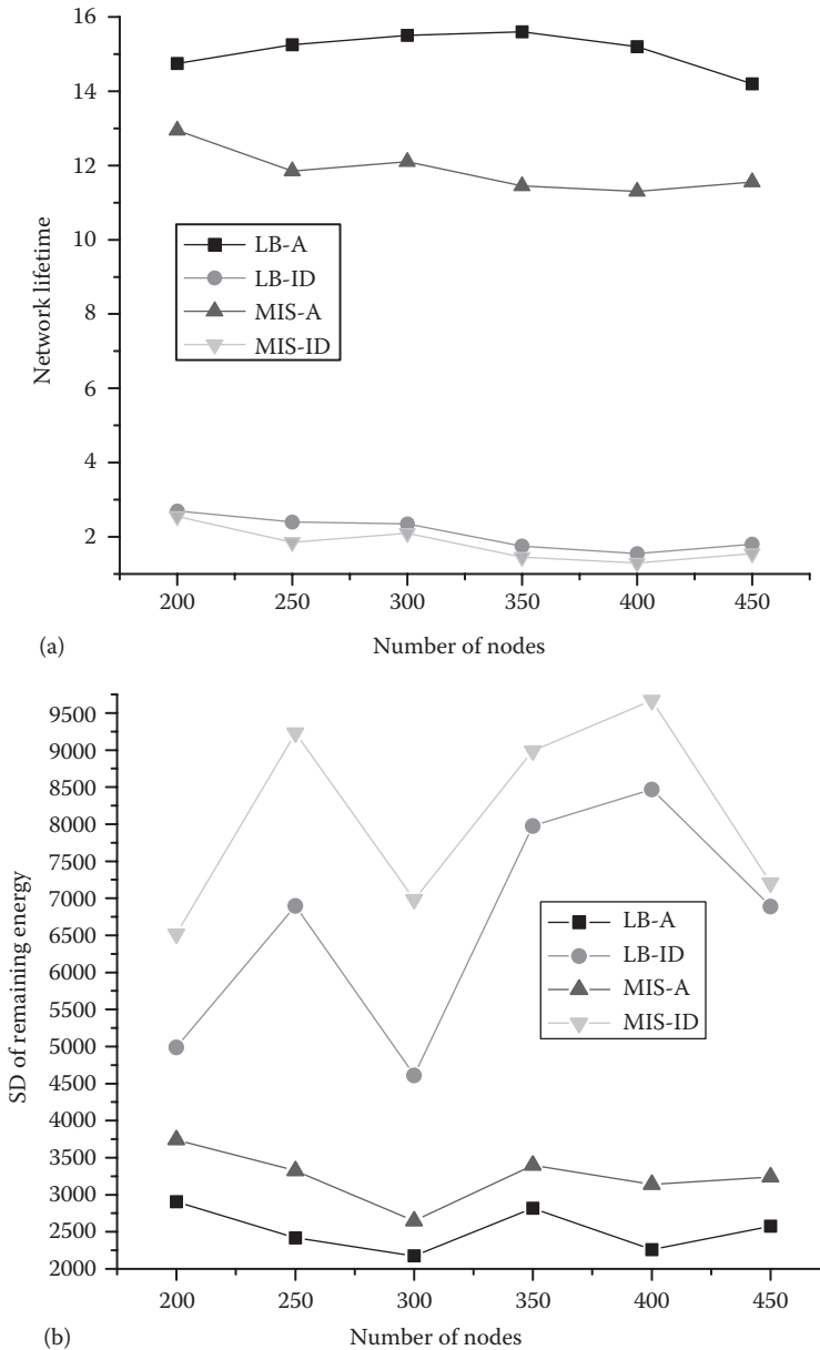
FIGURE 21.9 Simulation results for a square area of 100 m \times 100 m: the node transmission range is 10 m, and the number of nodes changes from 200 to 450—(a) network lifetime and (b) SD of residual energy.
