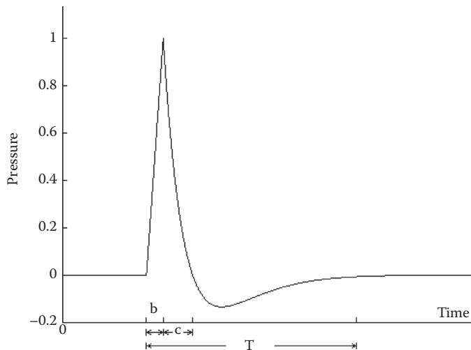
FIGURE 14.3 Theoretical Friedlander wave with finite rise time.
