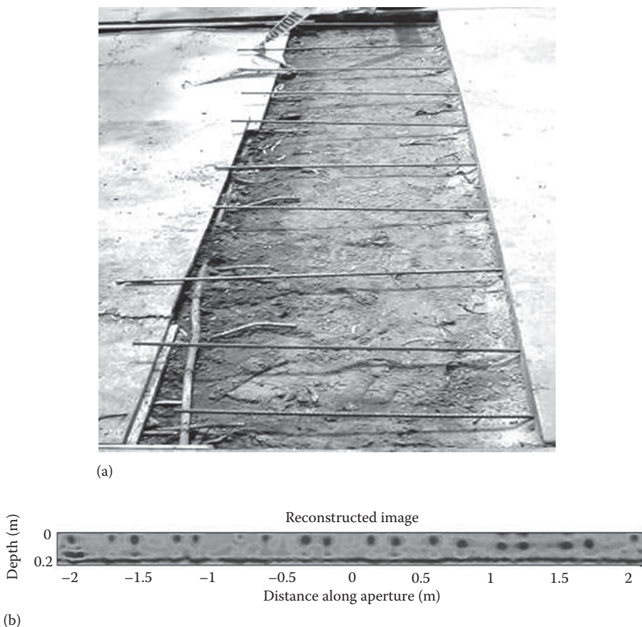
FIGURE 17.3 (a) Subsurface profile of a roadway and (b) image of the subsurface profile.
