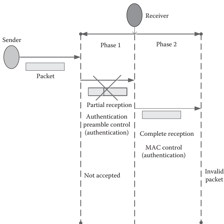
FIGURE 12.7 Invalid packet identified at physical layer.
