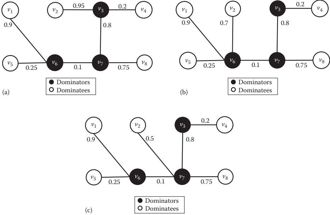
FIGURE 21.11 (a) A imbalanced dominator partition; (b) Another imbalanced dominator partition; (c) A load-balanced dominator partition.
