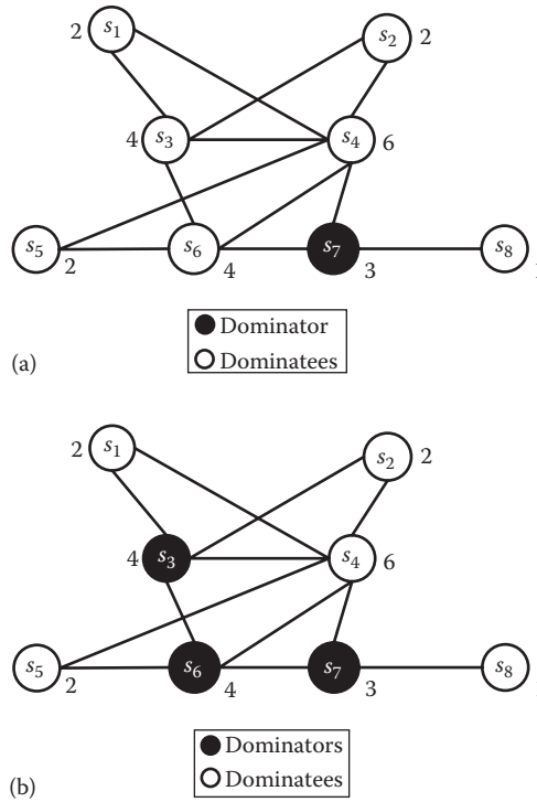
FIGURE 21.3 (a) The first round of running Algorithm LBCDS approximate; (b) The output of running Algorithm LBCDS approximate.
