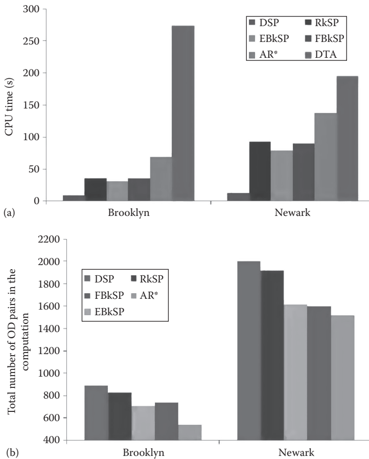
FIGURE 19.10 CPU time for both the networks ( L = 3 , k = 4 , urgency = ACI, period = 450 s, \delta = 0.7 , \beta = 0.05 ): (a) CPU time and (b) the number of OD pairs. (From Pan, J. and Borcea, C., IEEE Trans. Veh. Tech. , 62(8), 3551, 2014.)
