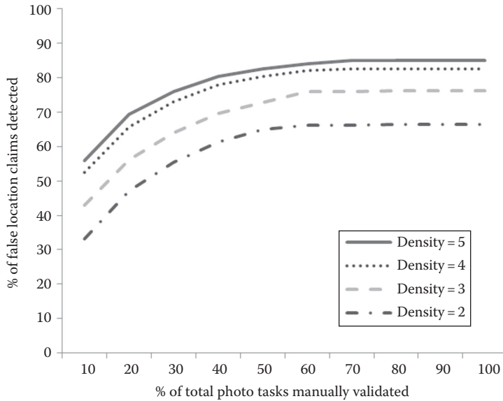
FIGURE 3.6 ILR performance as a function of the percentage of photos manually validated in Phase 1. Each curve represents a different network density represented as average number of neighbors per node.
