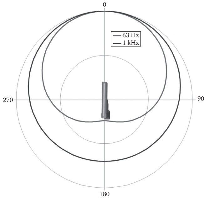
FIGURE 14.5 Simplification of directional attributes of muzzle blast at low and high frequencies.
