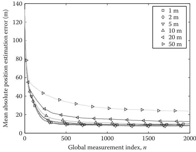
FIGURE 6.6 Comparison of SUKF-based centralized estimation performance for different values of range measurement standard deviation (values shown in the legend).
