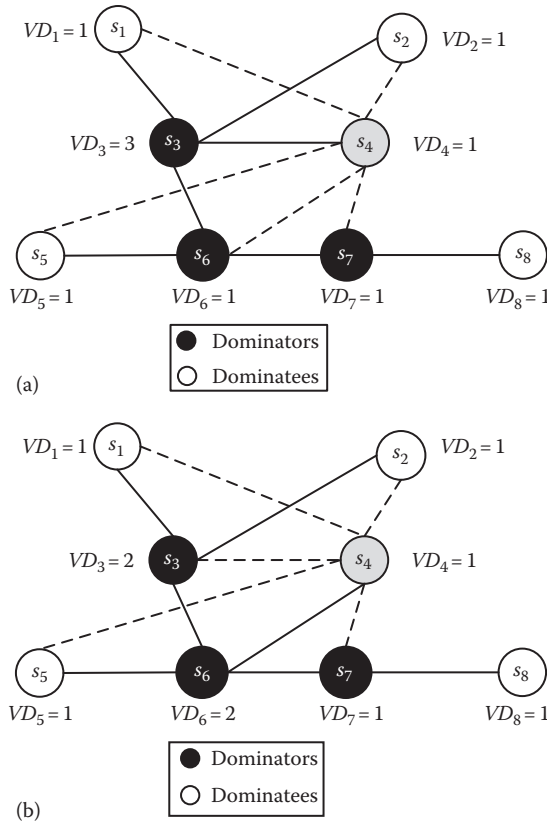
FIGURE 21.4 (a) A imbalanced dominate allocation scheme; (b) A load-balanced dominate allocation scheme.
