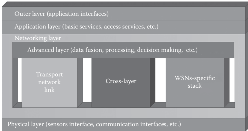
FIGURE 5.1 Hierarchical WSNs.
