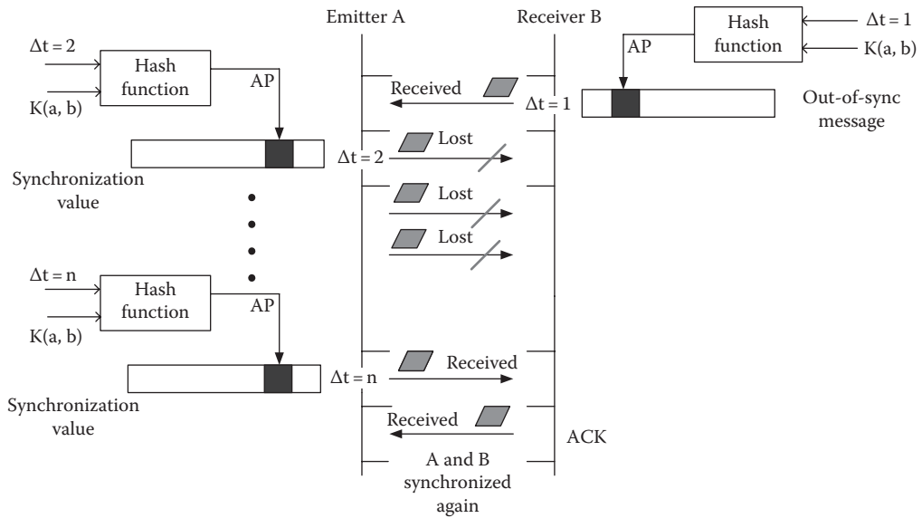
FIGURE 12.16 The emitter “A” receives an out-of-sync packet from the receiver “B.” The same emitter sent the “SYN” value until the ACK reception from “B.”
