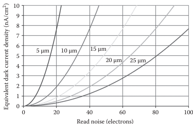
FIGURE 18.19 Dark current density versus read noise for different pixel pitches. (From MacDougall, M. et al., Opt. Eng. , 50(6), 061011, 2011.)
