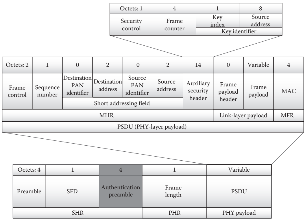
FIGURE 12.2 IEEE 802.15.4e standard packet format adapted to include the AP mechanism at PHY layer.
