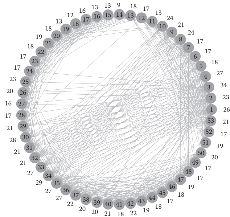
FIGURE 13.2 The WSN topology obtained when the probability of sending a message is larger than or equal to 0.1. The values outside of the circle indicate the degree of each sensor node.
