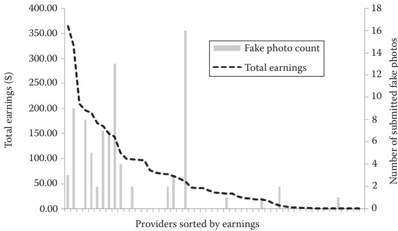
FIGURE 3.7 Correlation of earnings and fake photos.
