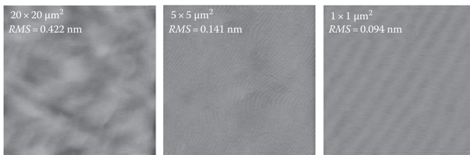
FIGURE 18.14 Microscopic surface morphology using AFM on GaN p-i-n structure grown on GaN/sapphire template. No specific surface defects are observed. (From Sood, A.K. et al., Proc. SPIE , 7780, 77800E, 2010.)
