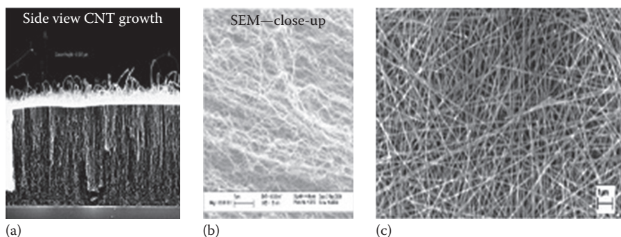
FIGURE 18.28 Growth of MWCNT forest with the ability to separate the CNT from the growth substrate with good length/diameter uniformity and the MWCNT released from the template.
