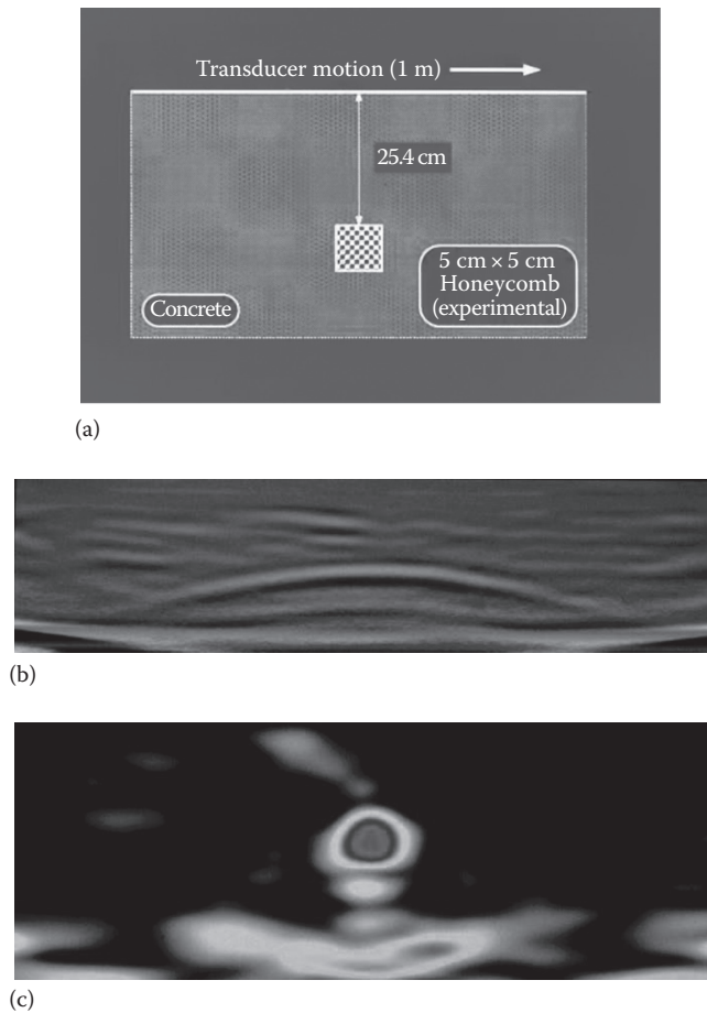
FIGURE 16.9 (a) Arrangement of the test specimen (honeycomb). (b) Signature of the microwave echoes. (c) Reconstructed image (honeycomb).
