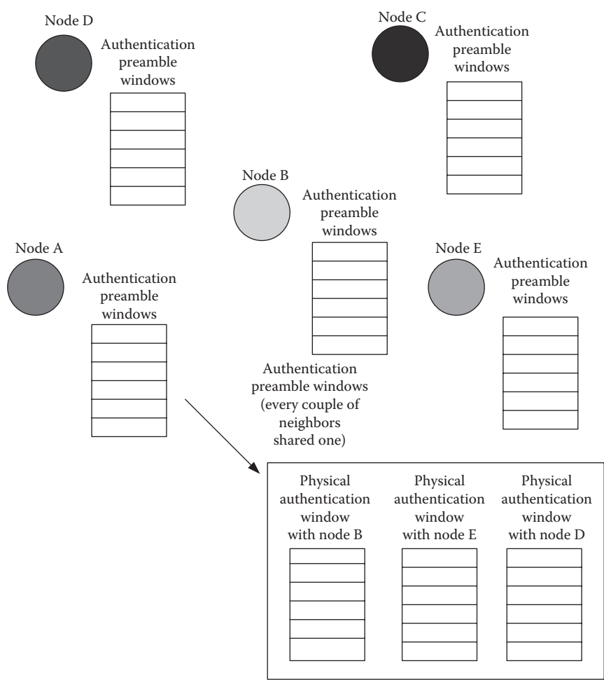
FIGURE 12.3 The initial scenario with all the AP windows.
