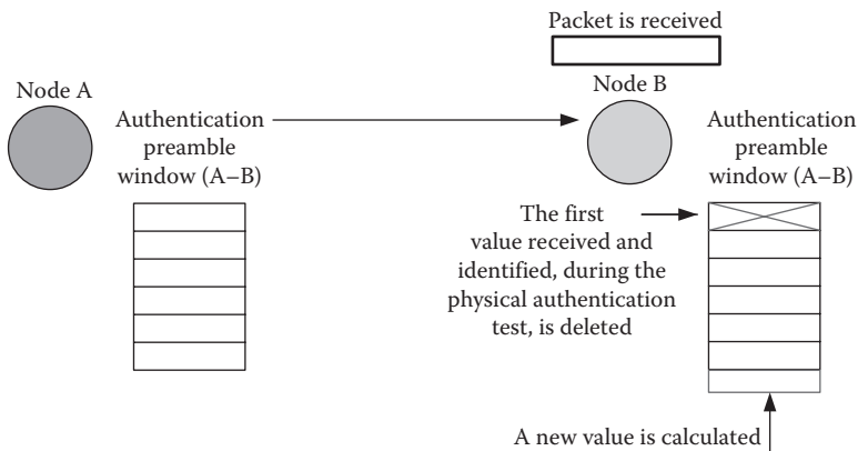
FIGURE 12.6 Updates of the AP window of node “B.”
