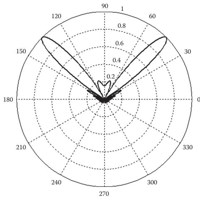
FIGURE 10.3 Directivity pattern of a linear array of 20 pressure microphones with the main lobe steered to 45° ( d = 0.1 m, f = 680 Hz).
