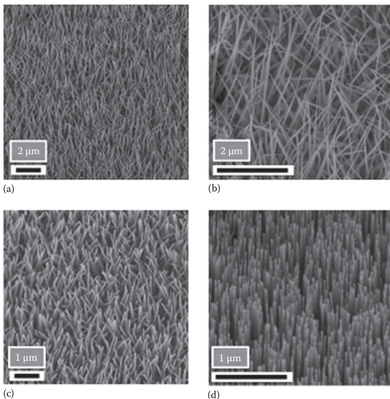
FIGURE 18.2 SEM images of NWs grown on the various substrates taken at room temperature, showing NWs grown on (a) ZnO/sapphire, (b) ZnO/SiO 2 /p-Si, (c) ZnO/p-Si, and (d) ZnO/GaN/sapphire. (From Anwar, M. et al., Proc. SPIE , 8868, 8868B, 2013.)
