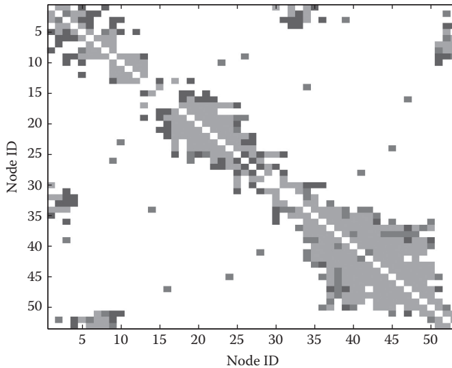
FIGURE 13.5 T-test conducted on the correlation matrix of Topology 2. Dark gray squares show evidence of correlation between nodes. Black squares indicate the existence of a link between nodes. Light gray indicate both evidence of correlation and the existence of a link between nodes.
