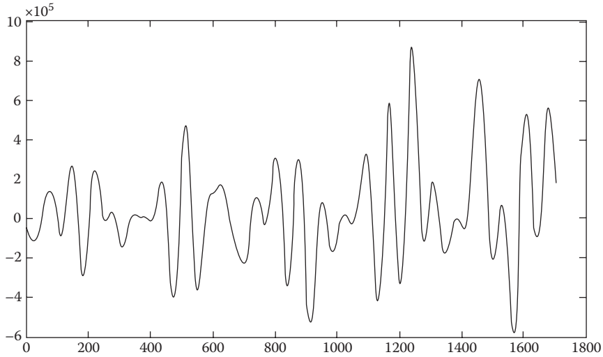
FIGURE 20.5 A received signal after matched filtering.
