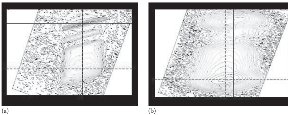
FIGURE 18.13 Reciprocal space mapping of AlGaIn p-n junctions on (a) AlN and (b) sapphire substrates. (From Long, J.P., Opto-Electron. Rev. , 10(4), 251, 2002.)
