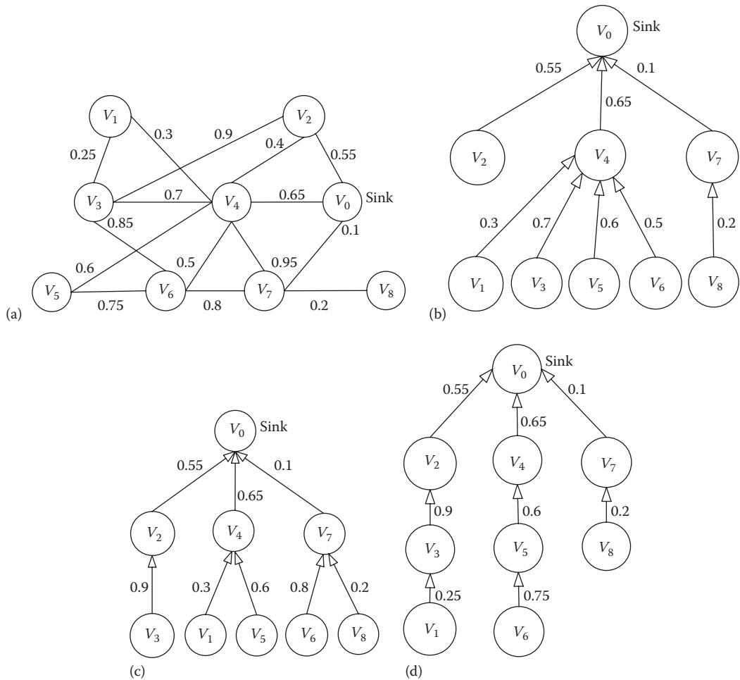
FIGURE 7.1 (a) A probabilistic wireless sensor network (WSN), (b) A imbalanced data aggregation tree (DAT), (c) another imbalanced DAT, (d) A load-balanced DAT (LBDAT).
