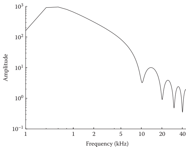
FIGURE 14.4 Frequency spectrum of a theoretical Friedlander wave.
