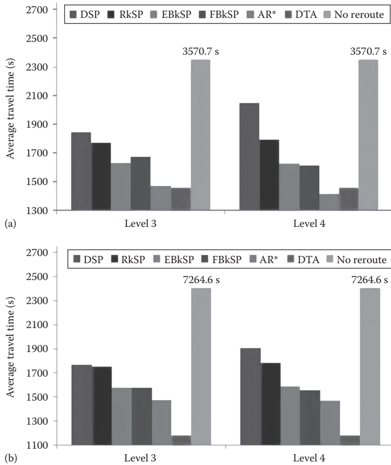
FIGURE 19.8 Average travel time ( L = (3, 4) , k = 4 , urgency = ACL, period = 450 s, \delta = 0.7 , and \beta = 0.05 ): (a) Brooklyn and (b) Newark. (From Pan, J. and Borcea, C., IEEE Trans. Veh. Tech. , 62(8), 3551, 2014.)
