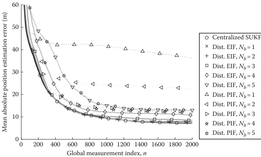
FIGURE 6.7 Comparison of the centralized SUKF and approximate delayed PIF and EIF distributed algorithms.
