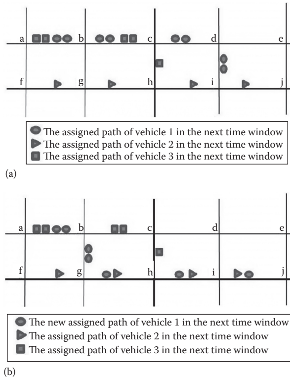
FIGURE 19.5 An FBkSP example. \omega_{fg} = \omega_{gh} = \omega_{hi} = \omega_{ij} = \omega_{ch} = 1 , \omega_{ab} = \omega_{bc} = \omega_{cd} = \omega_{de} = \omega_{af} = \omega_{bg} = \omega_{di} = \omega_{ej} = 2 : (a) the old assignment and (b) the new assignment. (From Pan, J. and Borcea, C., IEEE Trans. Veh. Tech. , 62(8), 3551, 2014.)
