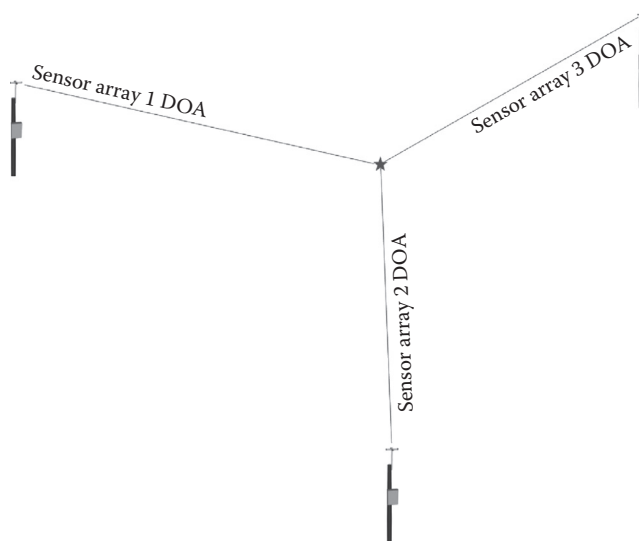
FIGURE 14.9 Triangulation using single transducer at sensor nodes.
