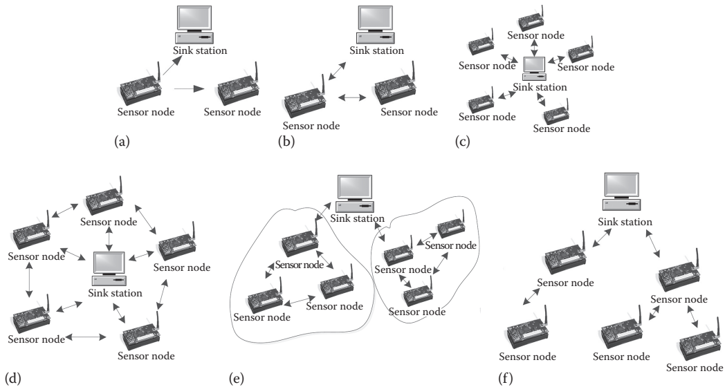
FIGURE 5.2 Topologies of WSNs. (a) One way, (b) bidirectional, (c) star, (d) mesh, (e) cluster, and (f) tree.
