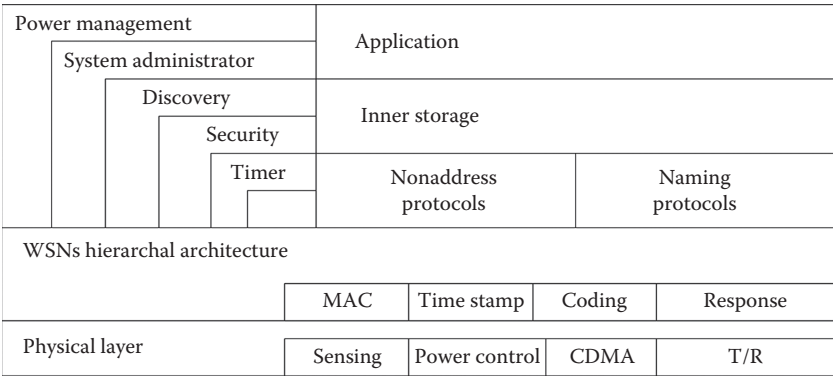
FIGURE 5.6 Narrow-waist architecture.
