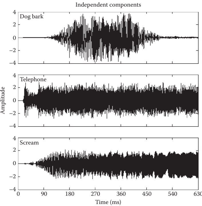
FIGURE 10.9 The three independent components estimated using ICA algorithm.
