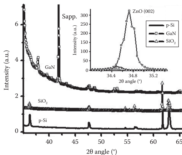
FIGURE 18.3 XRD of ZnO NWs grown using MOCVD on p-Si (solid), GaN/sapphire (square), and SiO 2 (tri-angle). The inset shows the ZnO peak associated with ZnO oriented along (002) and GaN. (From Anwar, M. et al., Proc. SPIE , 8868, 8868B, 2013.)
