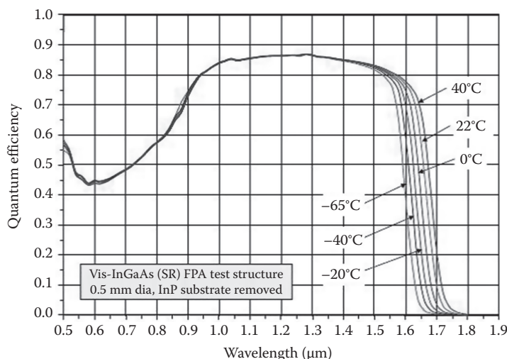
FIGURE 18.23 Spectral QE versus wavelength at different temperatures measured for backside-illuminated InGaAs photodiodes test array demonstrating visible–NIR response with InP substrate removed. (From Yuan, H. et al., Proc. SPIE , 6940, 69403C, 2008.)
