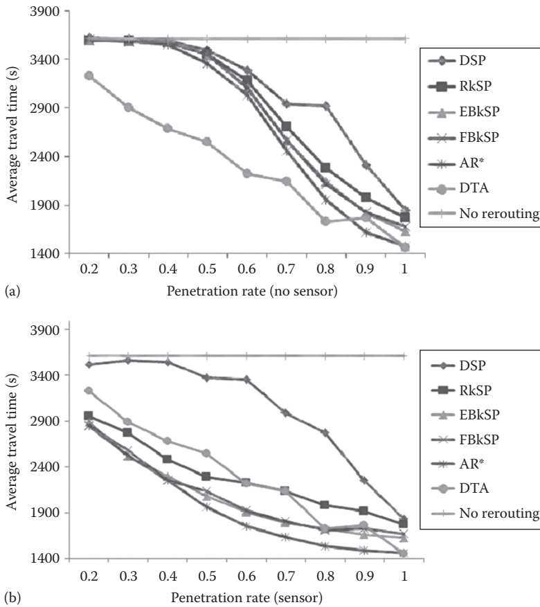
FIGURE 19.13 (a) Average travel time for all penetration rates with no sensor. (b) Average travel time for all penetration rate with sensors. (From Pan, J. and Borcea, C., IEEE Trans. Veh. Tech. , 62(8), 3551, 2014.)
