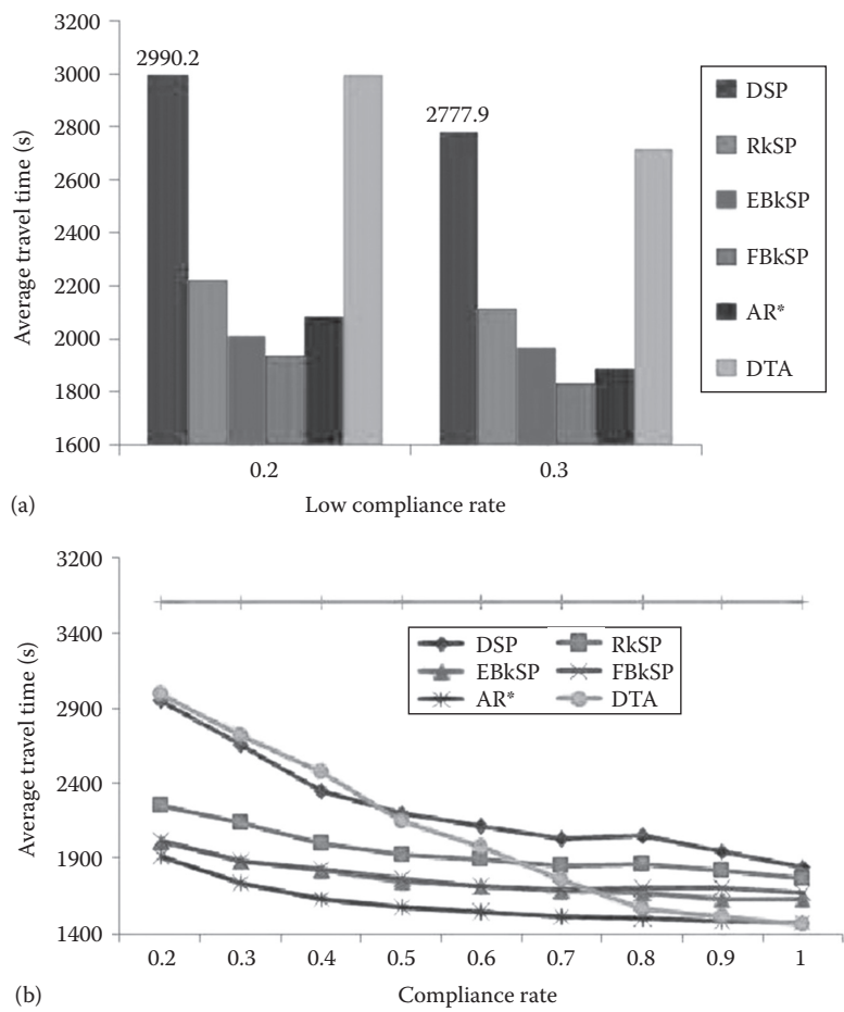
FIGURE 19.12 (a) Average travel time for low compliance rate. (b) Average travel time for all compliance rate. (From Pan, J. and Borcea, C., IEEE Trans. Veh. Tech. , 62(8), 3551, 2014.)
