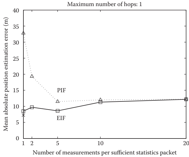
FIGURE 6.8 Comparison of the distributed EIF and PIF algorithms versus SSP block size, for information communication over a single hop.
