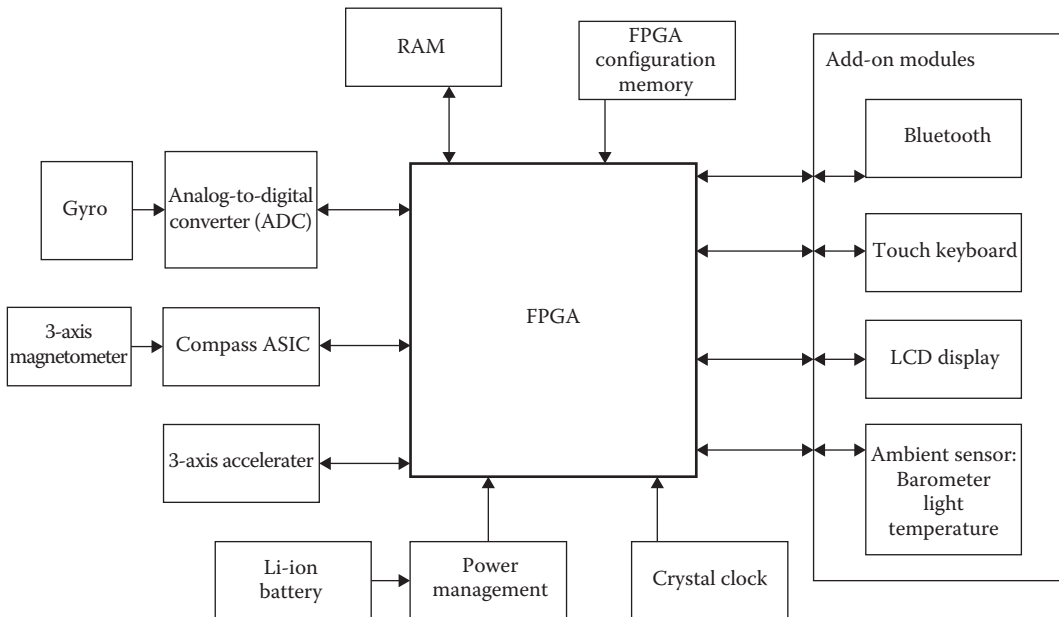
FIGURE 2.8 FPGA-based WSN platform.
