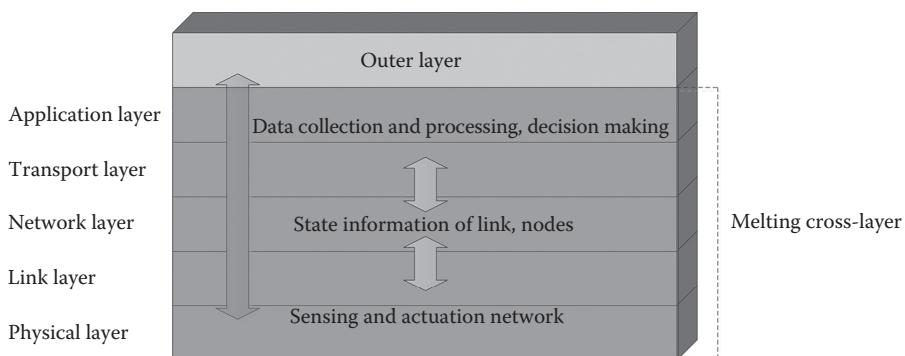
FIGURE 5.3 Cross-layer design.
