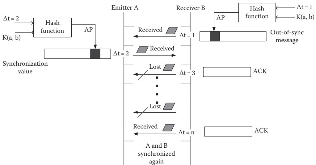
FIGURE 12.17 The receiver “B” receives the “SYN” value from the emitter “A.” The same receiver sent the ACK until the reception of a valid traffic packet from the emitter “A.”
