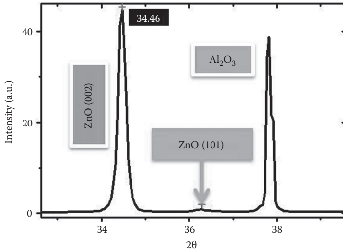
FIGURE 18.4 XRD of ZnO NWs grown using MOCVD on sapphire. (From Anwar, M. et al., Proc. SPIE , 8868, 8868B, 2013.)
