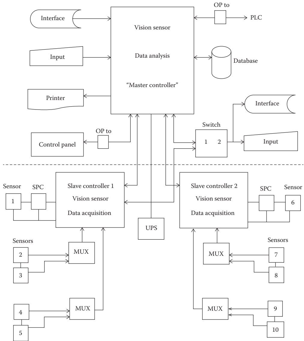
FIGURE 1.8 Sensor hardware architecture and application detail for manufacturing processing.
