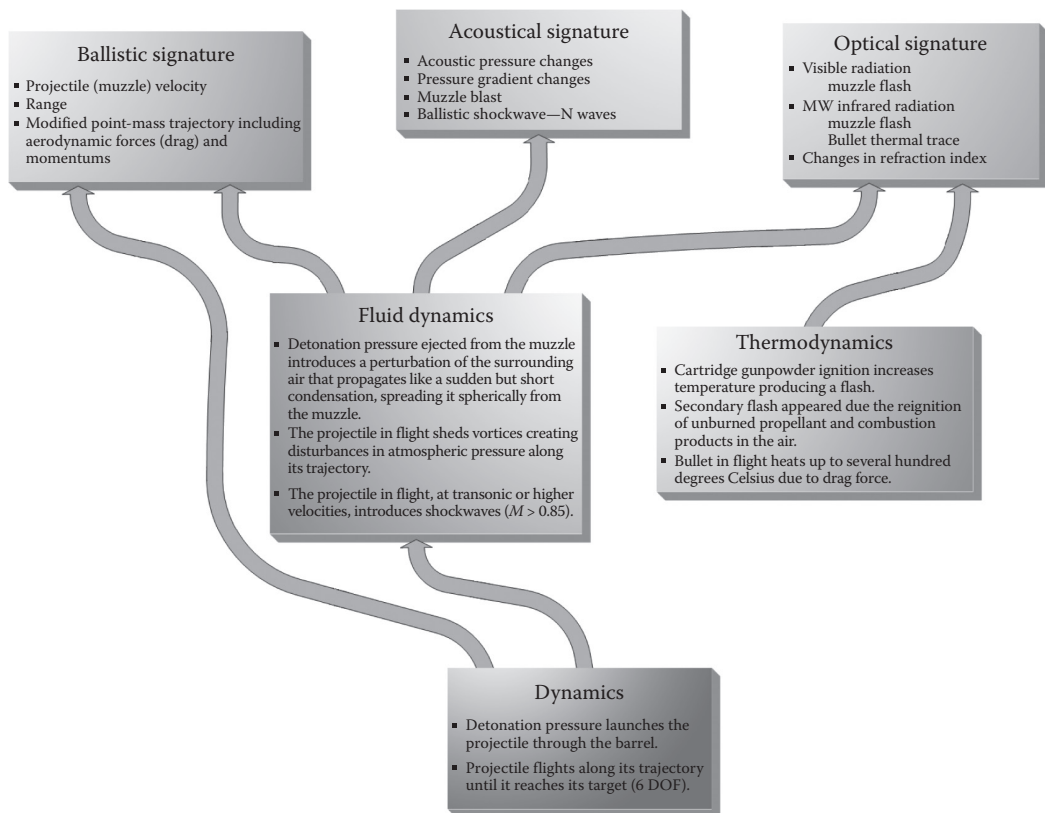
FIGURE 14.2 Roadmap to acoustic signature of a gunshot.
