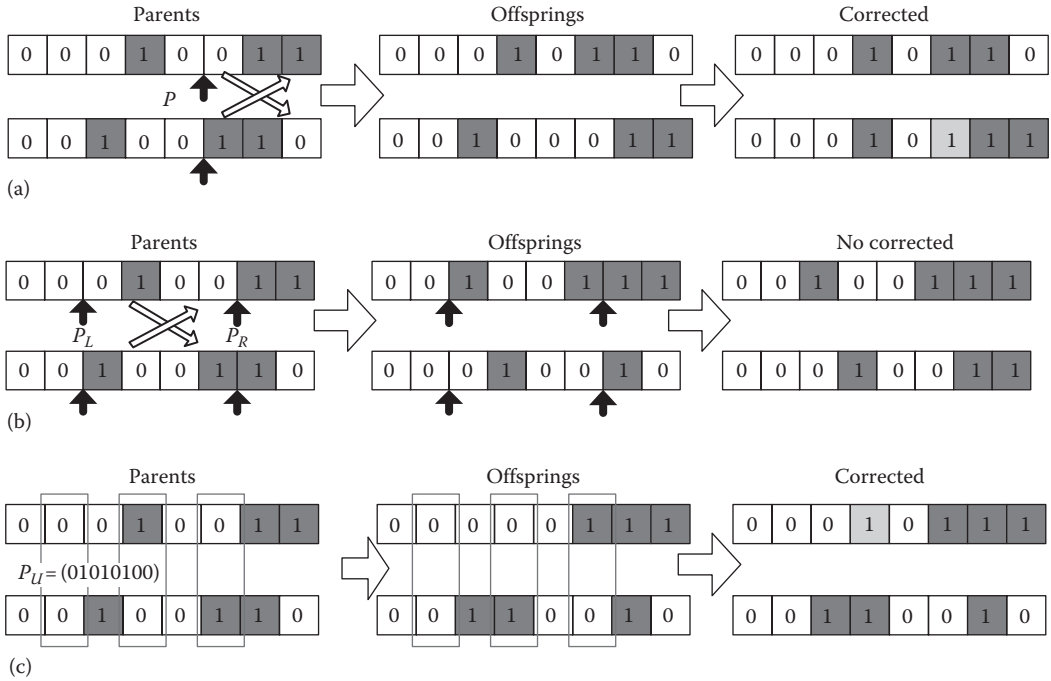
FIGURE 21.17 Illustration of crossover operations: (a) single-point crossover, (b) two-point crossover, and (c) uniform crossover.
