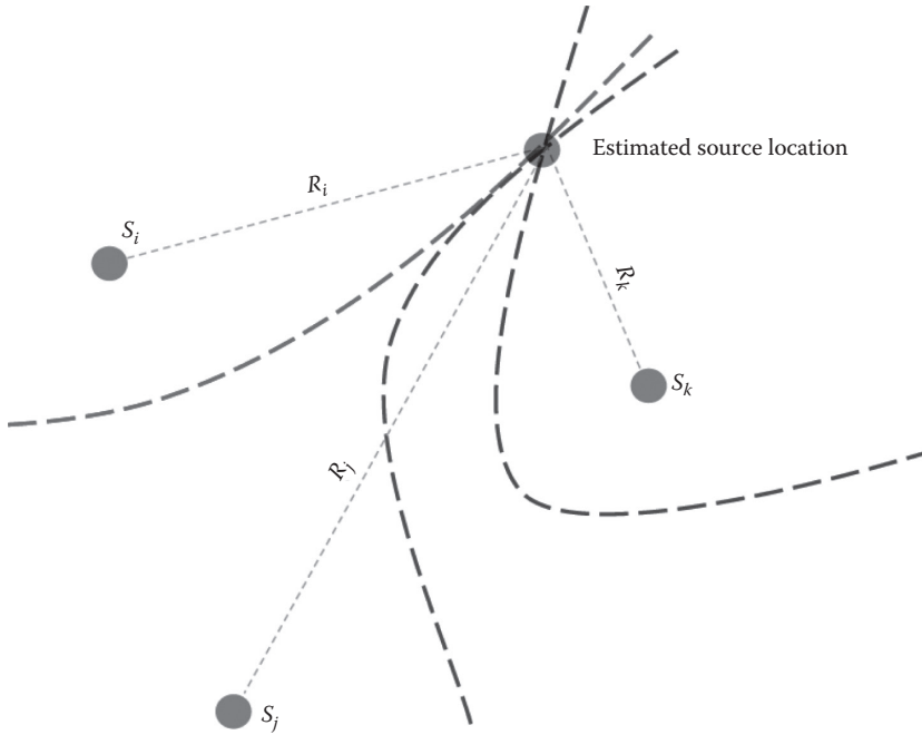
FIGURE 10.7 Explanation of the multilateration algorithm using three pairs of microphones.
