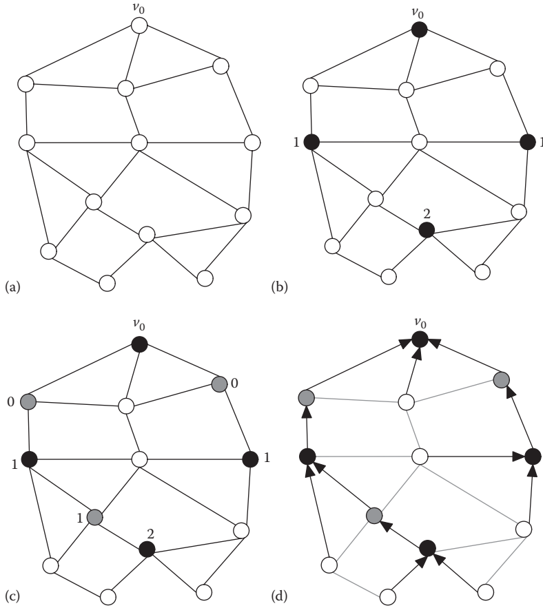
FIGURE 7.2 Illustration of (a) the topology of a WSN, (b) a LBMIS (marked by black nodes), (c) a CMIS (marked by gray nodes), and (d) a LBDAT construction process.
