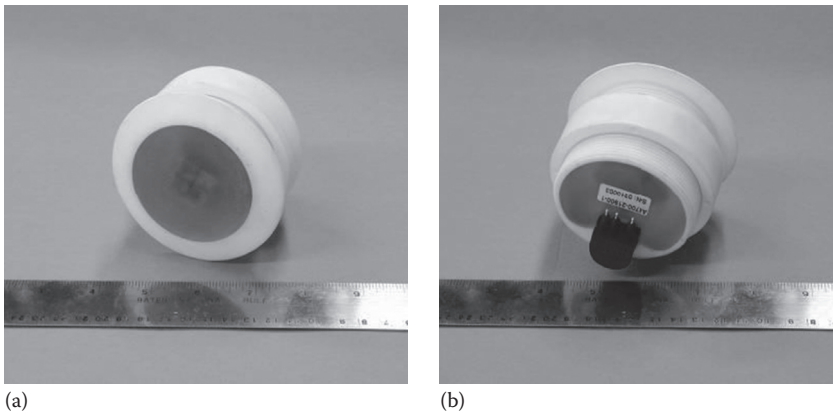
FIGURE 20.2 (a) Front and (b) back view of the single-element receiver.
