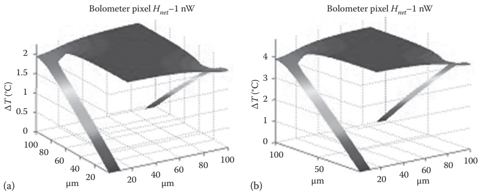
FIGURE 18.26 Temperature map of a bolometer pixel when the net absorbed power H is 1 nW and the CNT thermal resistance is 5 \times 10^8 K/W (left) and 1 \times 10^9 K/W (right). We assumed that the pixel is tightly packed with the CNTs. The temperature gradient of the contact legs connecting the film to the ROIC is clearly shown. (From Sood, A.K. et al., Proc. SPIE , 8353, 83533A, May 2012.)
