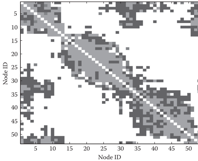
FIGURE 13.4 T-test conducted on the correlation matrix of Topology 1. Dark gray squares show evidence of correlation between nodes. Black squares indicate the existence of a link between nodes. Light gray squares indicate both evidence of correlation and the existence of a link between nodes.
