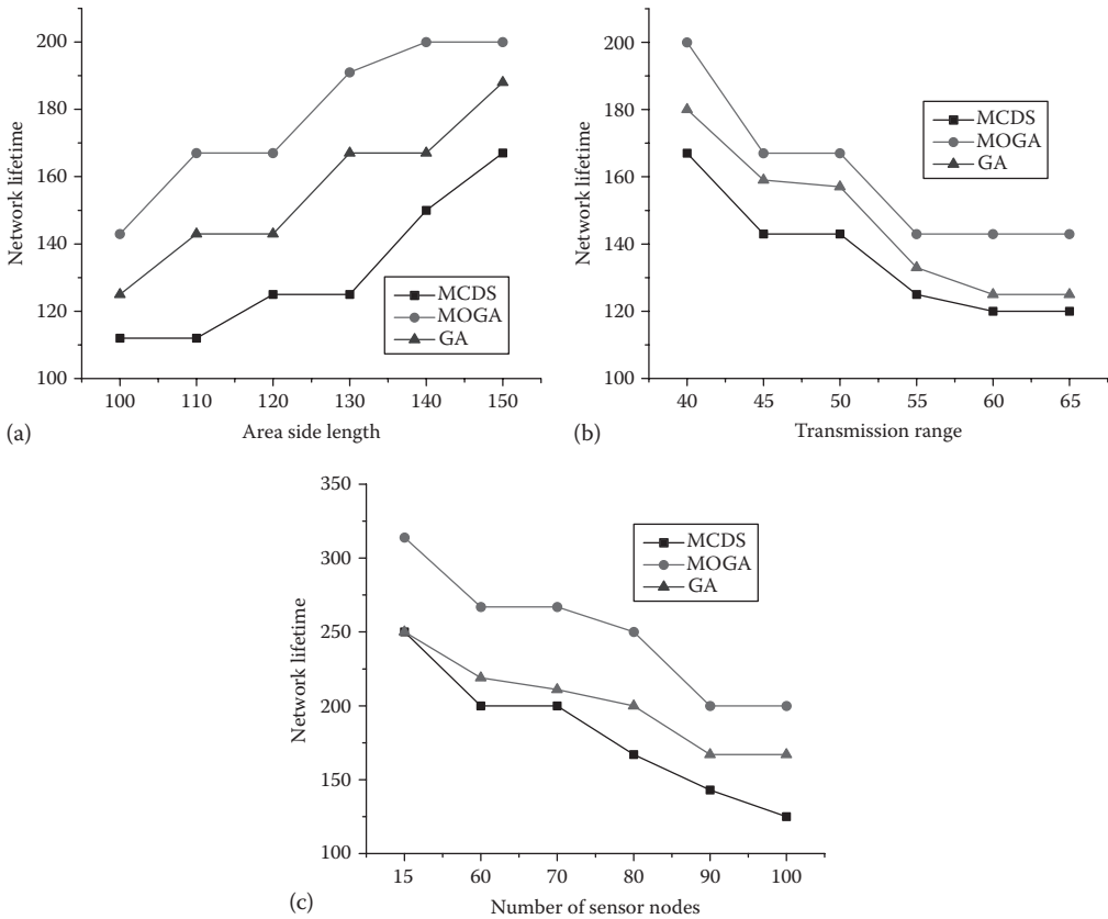
FIGURE 21.19 Network lifetime: (a) the node transmission range is 20 m, the number of nodes is 100, and the side length of the deployed area changes from 100 m \times 150 m; (b) the square area is 300 m \times 300 m, the number of nodes is 100, and the node transmission range changes from 40 to 65 m; and (c) the square area is 300 m \times 300 m, the node transmission range is 50 m, and the number of nodes changes from 50 to 100.
