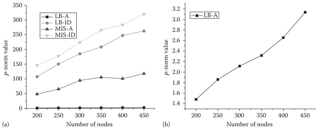
FIGURE 21.8 (a) p -norm values of the four schemes when number of nodes increase; (b) p -norm values of LB-A when number of nodes increase.
