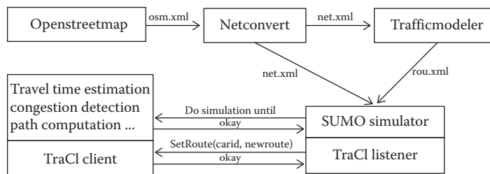
FIGURE 19.6 The simulation process. (From Pan, J. and Borcea, C., IEEE Trans. Veh. Tech. , 62(8), 3551, 2014.)
