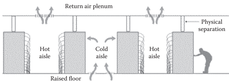
FIGURE 1.3 Hot and cold aisle containment is present in data centers designed to work in tangent with sensor nodes to increase efficiency.
