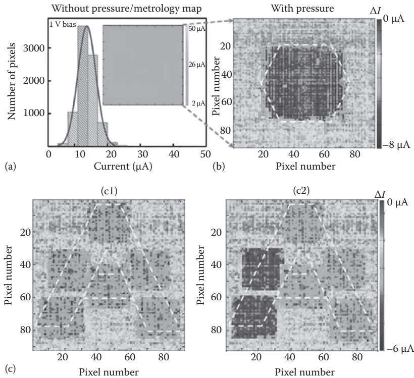
FIGURE 18.9 Tactile imaging and multidimensional sensing by the fully integrated 92 \times 92 SGVPT array. (a) Metrology mapping (inset) and statistical investigation of the fully integrated Strain Gated Vertical Piezo-Electric Transistor (SGVPT) array without applying stress. (b) Current response contour plot illustrating the capability of SGVPT array for imaging the spatial profile of applied stress. The different shades (light to dark) of grayscale represent the current differences for each taxel before and after applying the normal stress. The physical shape of the applied stress is highlighted by the white dashed lines. (c) Multidimensional sensing by an SGVPT array exhibits the potential of realizing applications such as personal signature recognition with maximum security and unique identity. The shape of a “written” letter A is highlighted by the white dashed lines. (From Wu, W. et al., Science , 340(24), 2013.)
