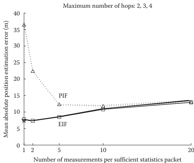
FIGURE 6.9 Comparison of the distributed EIF and PIF algorithms versus SSP block size, for information communication over a maximum of 2, 3, or 4 hops.
