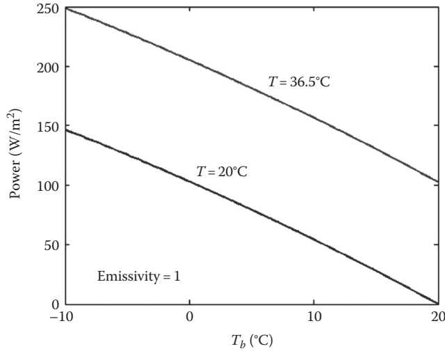
FIGURE 18.24 Net power received by bolometer as a function of bolometer temperature. (From Sood, A.K. et al., Proc. SPIE , 8353, 83533A, May 2012.)
