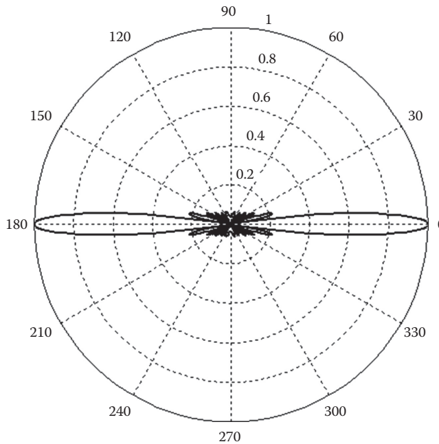
FIGURE 10.1 Directivity pattern of a linear array of 20 pressure microphones ( d = 0.1 m, f = 680 Hz).
