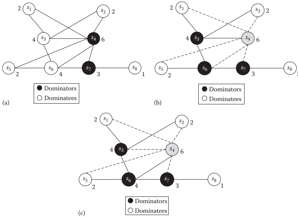
FIGURE 21.1 (a) A regular CDS; (b) a load-balanced CDS with an imbalanced dominate allocation scheme; (c) a load-balanced CDS with a load-balanced dominate allocation scheme.
