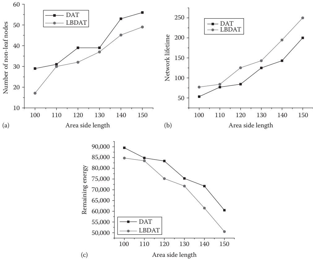
FIGURE 7.3 Simulation results for Scenario 1: (a) number of non-leaf nodes, (b) network lifetime, and (c) remaining energy.
