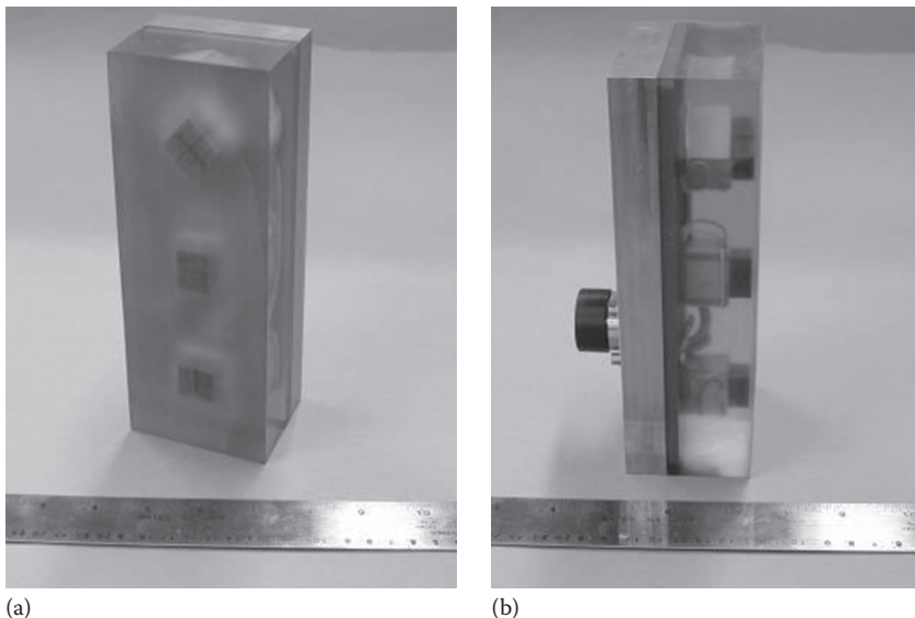
FIGURE 20.1 (a) Front and (b) side view of the laboratory prototype of the three-component transmitter of the base stations.
