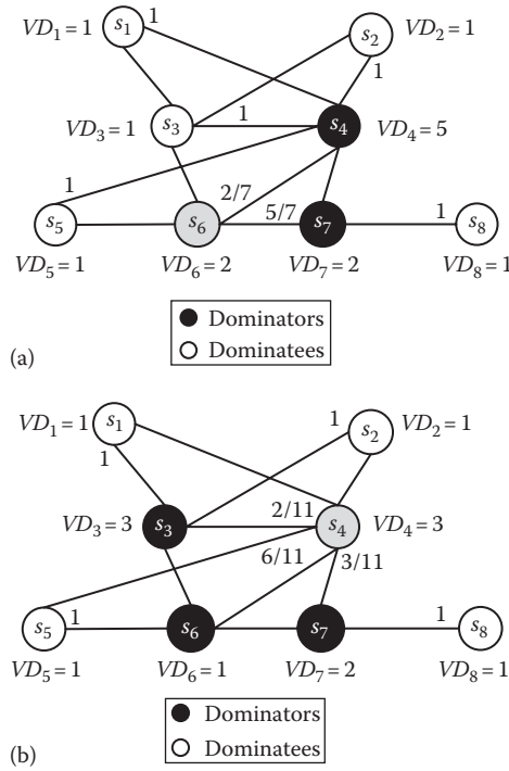
FIGURE 21.6 (a) Calculating EAP with the dominate connecting to two dominators; (b) Calculating EAP with the dominate connecting to three dominators.
