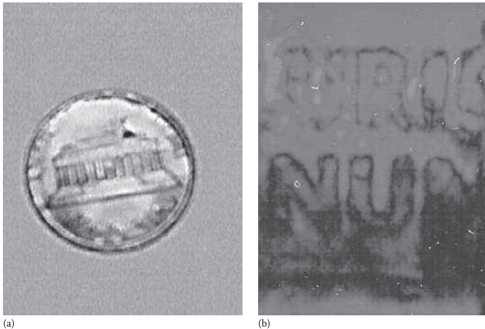
FIGURE 16.4 (a) The penny and (b) STAM image of the penny formed from the waveforms at the opposite side.
