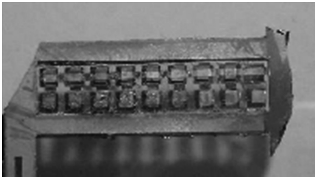
FIGURE 17.1 Micro flexible ultrasound transceiver array prototype.
