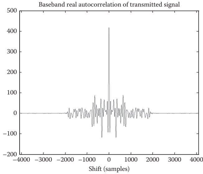
FIGURE 20.4 Autocorrelation function R_0(t) used in the field experiment.
