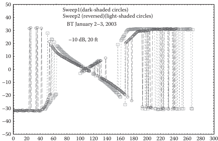
FIGURE 20.3 Bearing angle estimation experiment with the conventional method.
