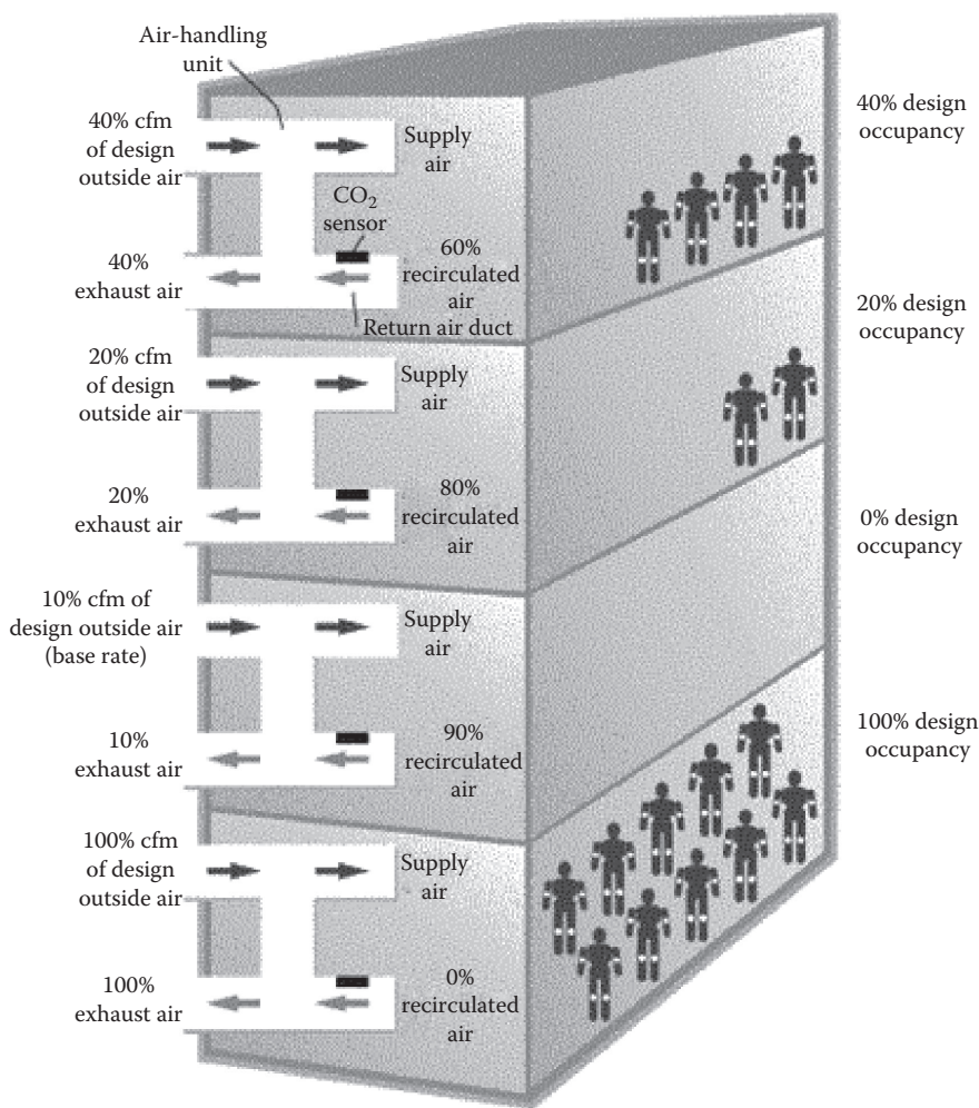
FIGURE 1.2 Buildings have the ability to control the environment in spaces with multiple floors and differing business hours correlated to the amount of employees present.
