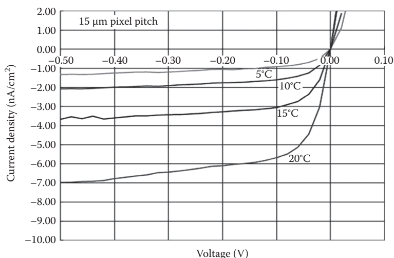
FIGURE 18.20 Dark current density at different temperatures using test structures on the wafer. Test arrays have 225 pixels (15 μm pitch), and the guard ring is not biased. (From Hood, A.D., Proc. SPIE , 8353, 83530A, 2012.)
