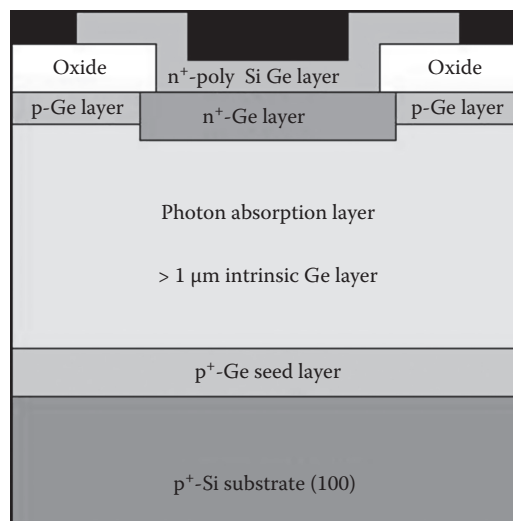
FIGURE 18.16 SiGe/Si-based buried junction approach to be evaluated for reduced surface states and leakage current. (From Sood, A.K. et al., Proc. SPIE , 7780, 77800F, 2010.)
