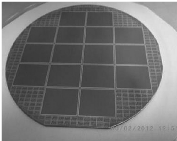
FIGURE 18.22 Experimental 1280 \times 1024/15 \mu\text{m} arrays on 4" wafer surrounded by various test mini-arrays with pitch sizes of 5\text{--}20 \mu\text{m} . (From Yuan, H. et al., Proc. SPIE , 6940, 69403C, 2008.)
