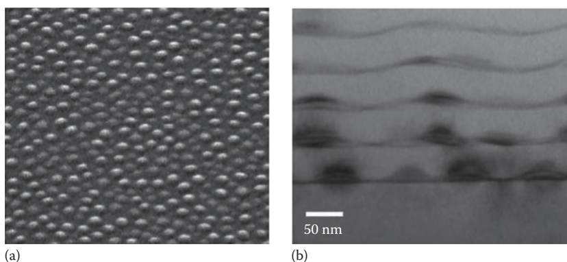
FIGURE 18.18 (a) SEM image (45° tilt) of a Ge quantum dot (QD) layer deposited on Si. The QDs are ~60 nm in diameter with a density of 1020 cm 2 . (b) A cross-sectional TEM image of Ge/Si QDSL grown. Ge QDs appear with dark contrast compared to Si barriers. (From Sood, A.K. et al., Proc. SPIE , 8012, 801240, 2011.)
