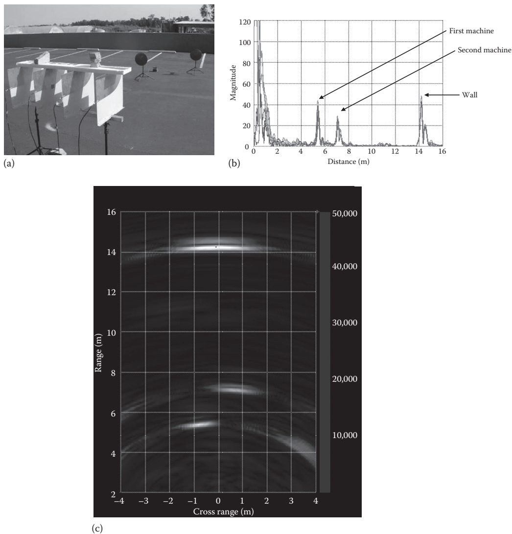
FIGURE 17.4 (a) Experiment setup of the FMCW microwave imaging system. (b) A typical range profile from the experiment. (c) Reconstructed image of the experiment.
