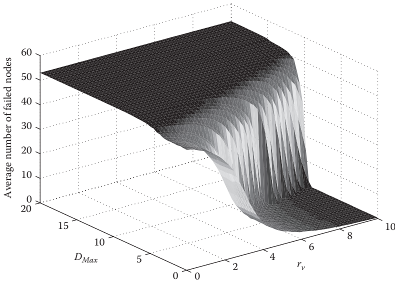
FIGURE 13.8 Average number of failed nodes as a function of the homogeneous robustness vector and maximum distance for Topology 1.
