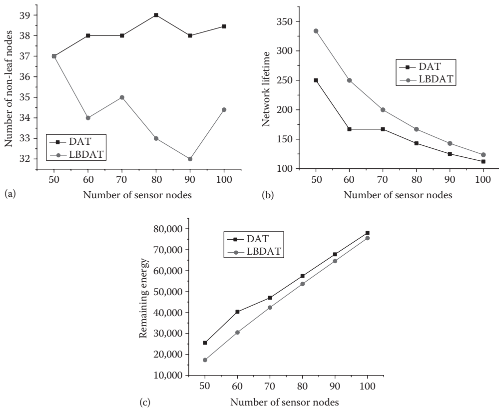
FIGURE 7.5 Simulation results for Scenario 3: (a) number of non-leaf nodes, (b) network lifetime, and (c) remaining energy.
