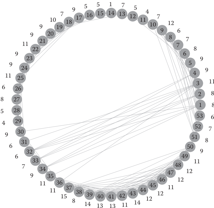
FIGURE 13.3 The WSN topology obtained when the probability of sending a message is larger than or equal to 0.3. The values outside of the circle indicate the degree of each sensor node.
