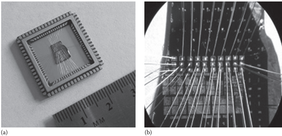
FIGURE 18.7 (a) Mounted solar-blind NW UV 3 \times 9 pixel array detector device and (b) close-up of device, showing wire-bonded pixels. (From Anwar, M. et al., Proc. SPIE , 8868, 8868B, 2013.)
