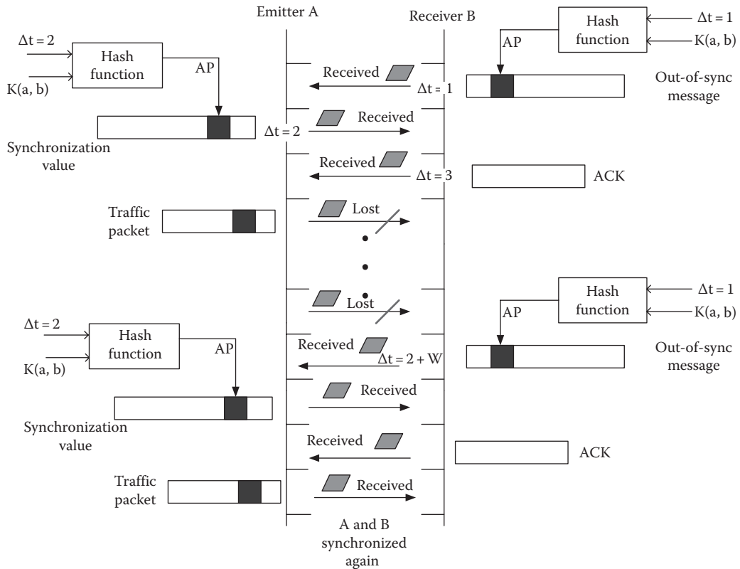
FIGURE 12.18 If “B” is not able to receive a normal traffic packet after W\Delta t , it has to start again the out-of-sync process.
