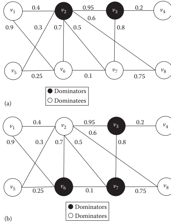
FIGURE 21.2 (a) A regular VB under PNM; (b) a Load-Balanced VB (LBVB) under PNM.
