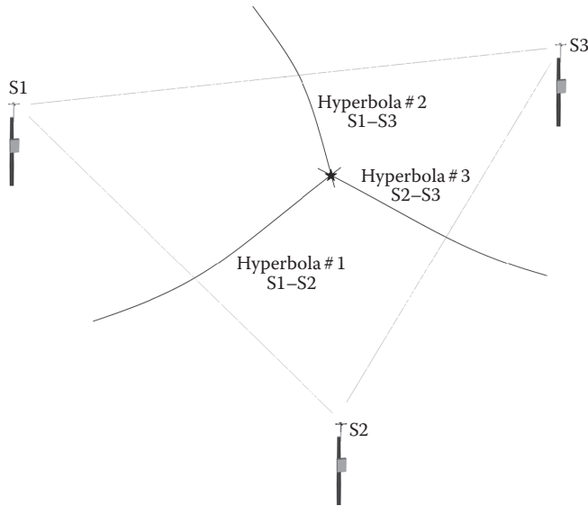
FIGURE 14.10 Triangulation using multiple-transducer arrays at sensor nodes.
