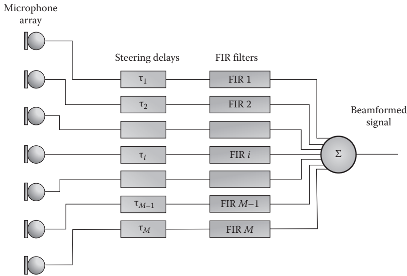
FIGURE 10.5 Schematic diagram of a delay-and-sum beamformer with FIR filters.
