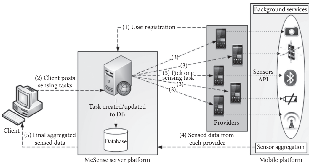
FIGURE 3.1 McSense architecture.
