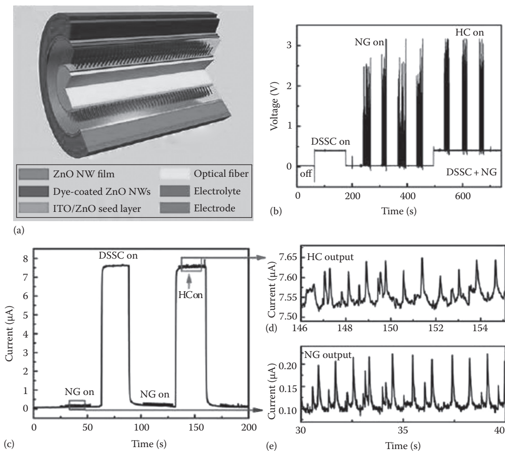
FIGURE 18.8 Design and performance of a 3D optical fiber-based HC consisting of a DSSC and an NG for harvesting solar and mechanical energy. (a) The 3D HC is composed of an optical fiber-based DSSC with capillary tube as counter electrode and an NG on top. (b) Open-circuit voltage (VOC) of the HC when the NG and the DSSC are connected in series, where VOC(HC) = VOC(DSSC) + VOC(NG) . (c) Short-circuit current (ISC) of the HC when the NG and the DSSC are connected in parallel. (d, e) Enlarged view of ISC(HC) and ISC(NG), clearly showing that ISC(NG) is 0.13 \mu A , the ISC(DSSC) is 7.52 \mu A , and the ISC(HC) is about 7.65 \mu A , nearly the sum of the output of the solar cell. (From Wang, Z.L. et al., Mater. Today , 15(12), 532, 2012.)
