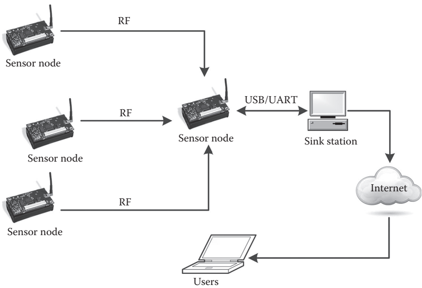
FIGURE 5.5 The architecture of INSIGHT.
