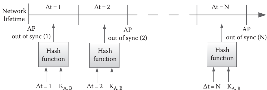
FIGURE 12.10 The AP method used to recover synchronization between couples of devices.
