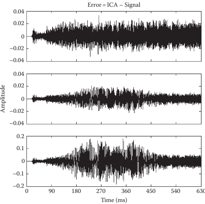
FIGURE 10.10 Independent component estimation error for each signal.
