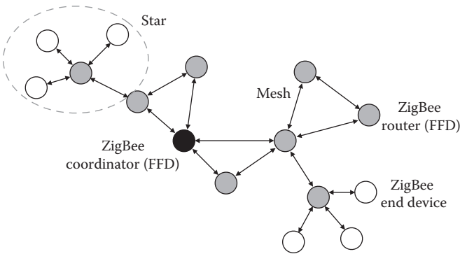
FIGURE 15.4 ZigBee network topologies.
