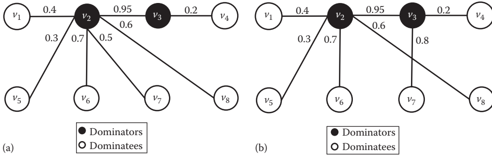
FIGURE 21.14 (a) A imbalanced dominator partition; (b) a load-balanced dominator partition.
