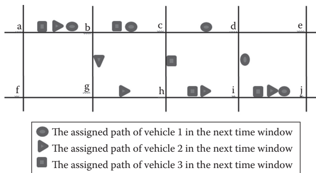
FIGURE 19.3 AR* rerouting example. All road segments have the same weight and \beta = 0.5 . (From Pan, J. and Borcea, C., IEEE Trans. Veh. Tech. , 62(8), 3551, 2014.)
