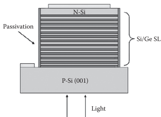
FIGURE 18.17 Schematic of detector array structure consisting of an SiGe/Si SLS grown on (001) silicon. (From Sood, A.K. et al., Proc. SPIE , 8012, 801240, 2011.)
