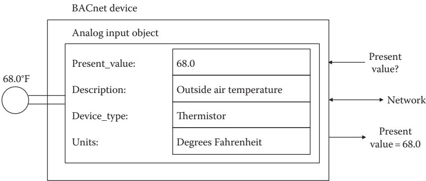
FIGURE 15.2 BACnet analog input object.
