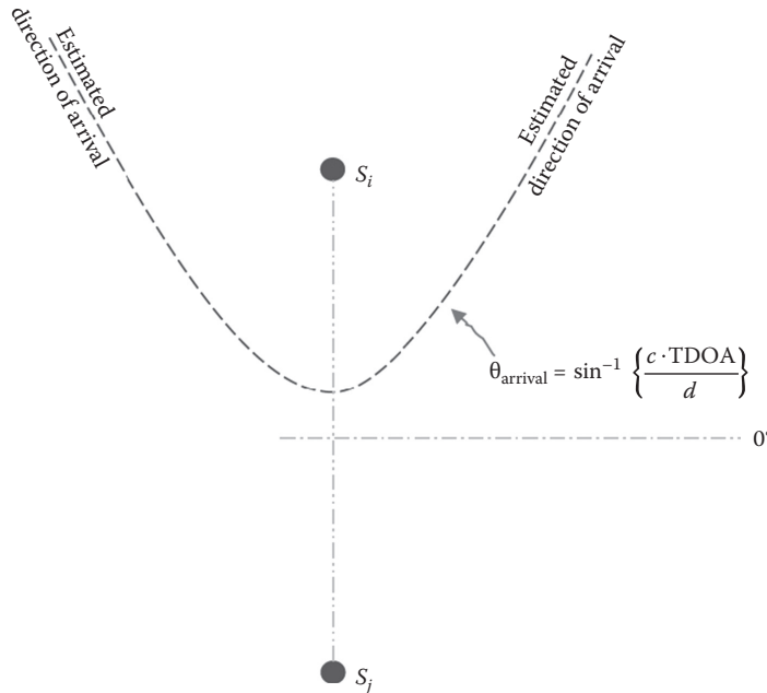
FIGURE 10.6 When estimating the DOA with a single pair of sensors, the analysis leads to a hyperbola pointing out to the source location.
