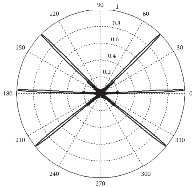
FIGURE 10.2 Directivity pattern of a linear array of 20 pressure microphones showing spatial aliasing or grating lobes ( d = 0.1 m, f = 5160 Hz).
