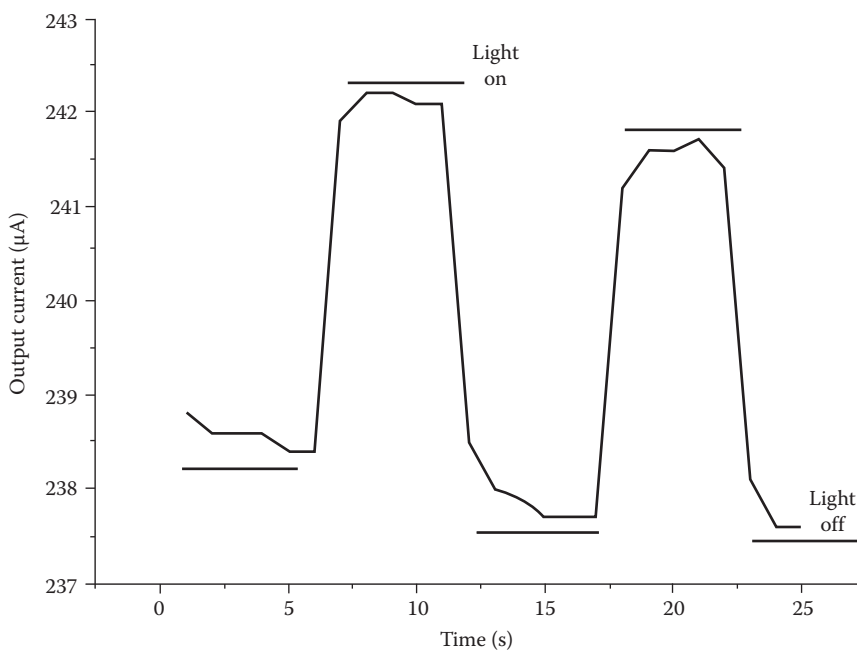
FIGURE 18.6 Switching photoresponse characteristics of ZnO NW device when UV LED source at ~370 nm turned on and off over approximately 10 s intervals. (From Anwar, M. et al., Proc. SPIE , 8868, 8868B, 2013.)
