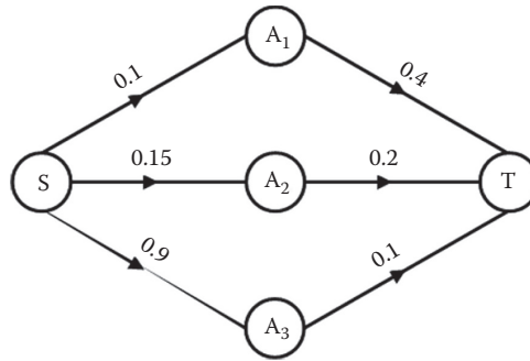
FIGURE 4.4 An example for NC-based opportunistic routing.
