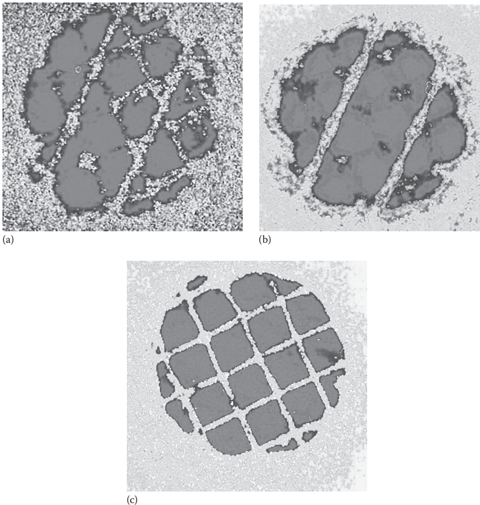
FIGURE 16.3 (a) The conventional SLAM image of two subsurface layers. (b) STAM image of the first layer. (c) Image of the second layer.
