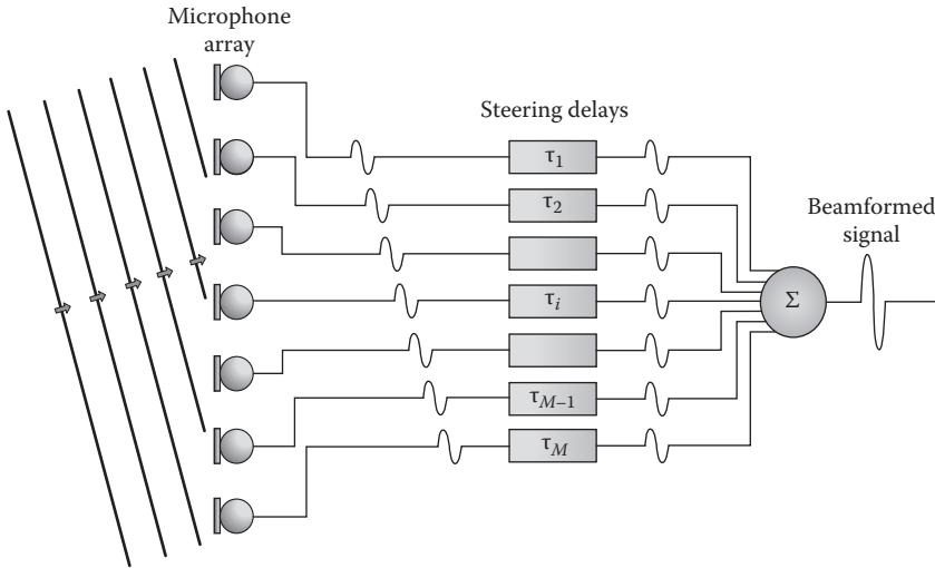
FIGURE 10.4 Schematic diagram of a delay-and-sum beamformer.
