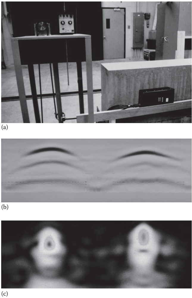
FIGURE 16.7 (a) Laboratory setup of the experiments. (b) Signature of the microwave echoes. (c) Reconstructed cross-sectional image of embedded rebars.
