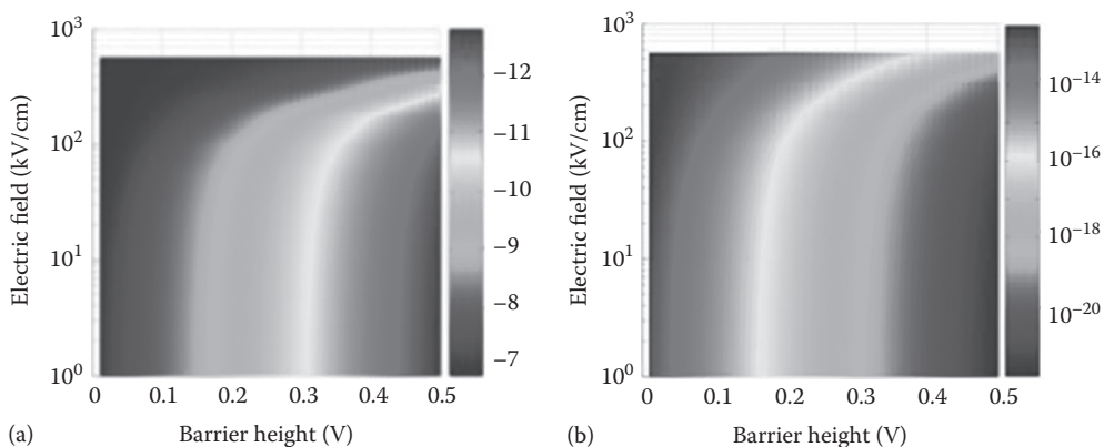
FIGURE 18.27 (a) Contour plot of TCR versus electric field and barrier height between CNTs of the film and (b) bolometer current also as a function of electric field and barrier height. The scales are the bars on the right of each contour plot in units of %TCR and amperes, respectively.
