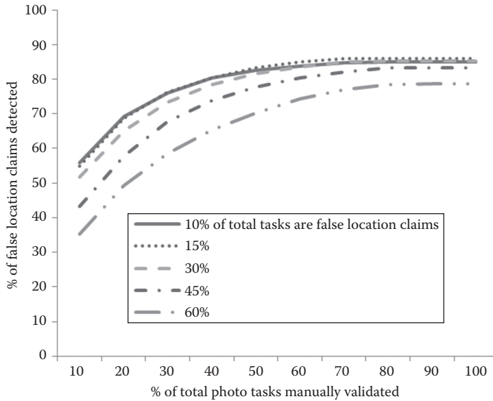
FIGURE 3.5 ILR performance as a function of the percentage of photos manually validated in Phase 1. Each curve represents a different percentage of photos with fake locations.
