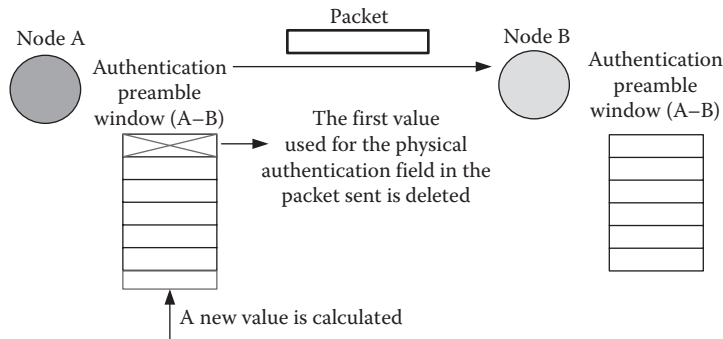
FIGURE 12.5 Updates of the AP window of node “A.”
