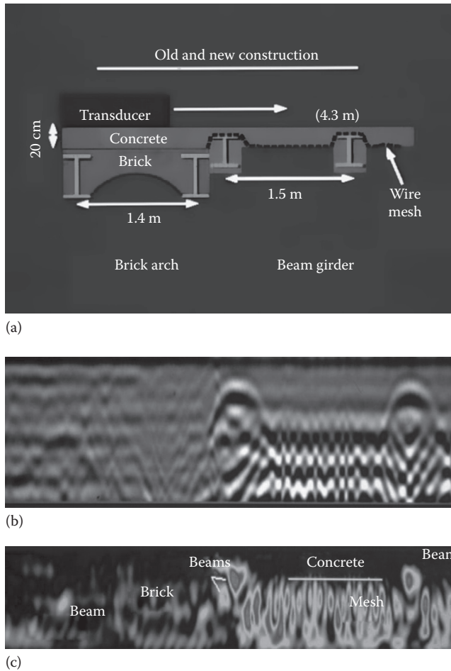
FIGURE 16.10 (a) Building structure of the test area. (b) Signature of the microwave echoes. (c) Reconstructed image of the subsurface profiles.
