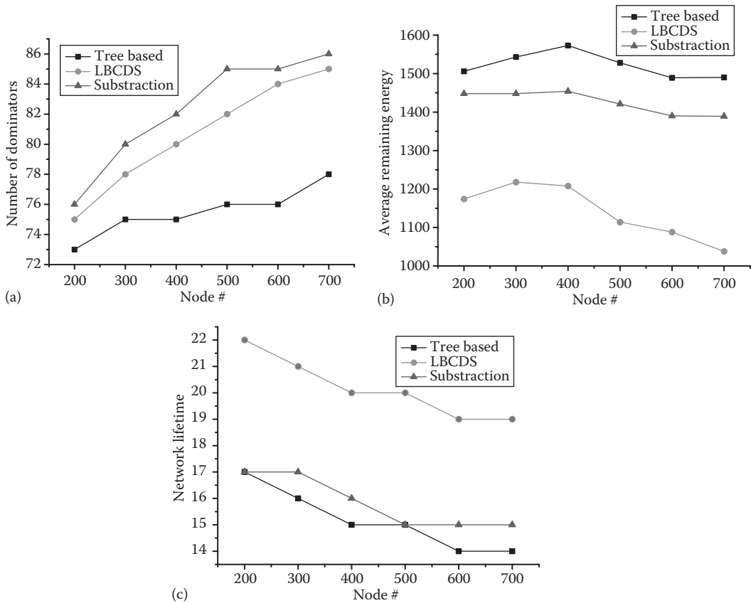
FIGURE 21.10 Simulation results for a square area of 100 m \times 100 m: the node transmission range is 10 m, and the number of nodes changes from 200 to 700—(a) the number of dominators, (b) average residual energy of dominators, and (c) network lifetime.
