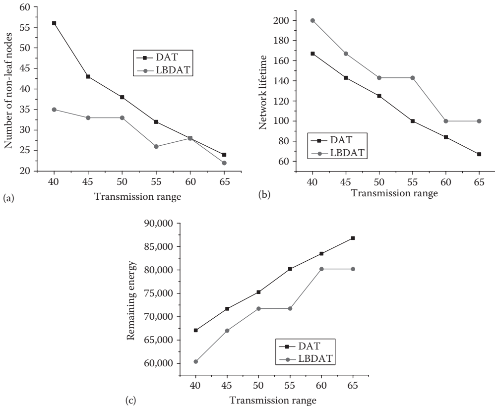
FIGURE 7.4 Simulation results for Scenario 2: (a) number of non-leaf nodes, (b) network lifetime, and (c) remaining energy.
