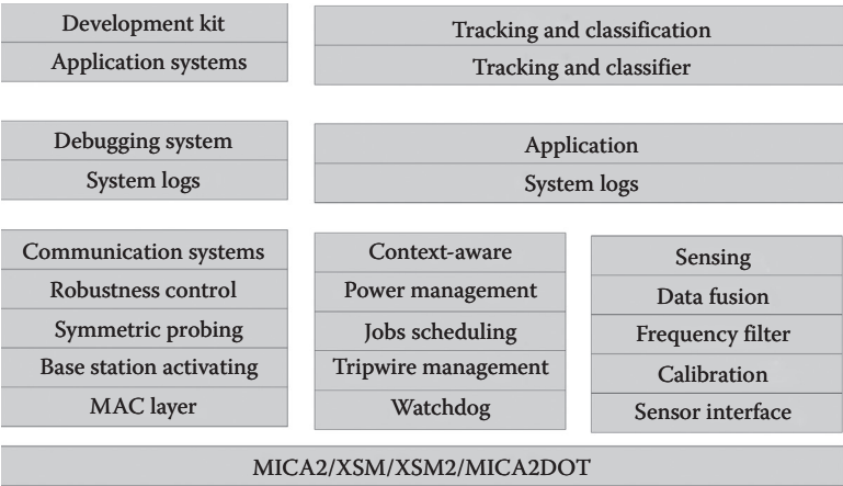
FIGURE 5.4 Hierarchy of VigilNet.
