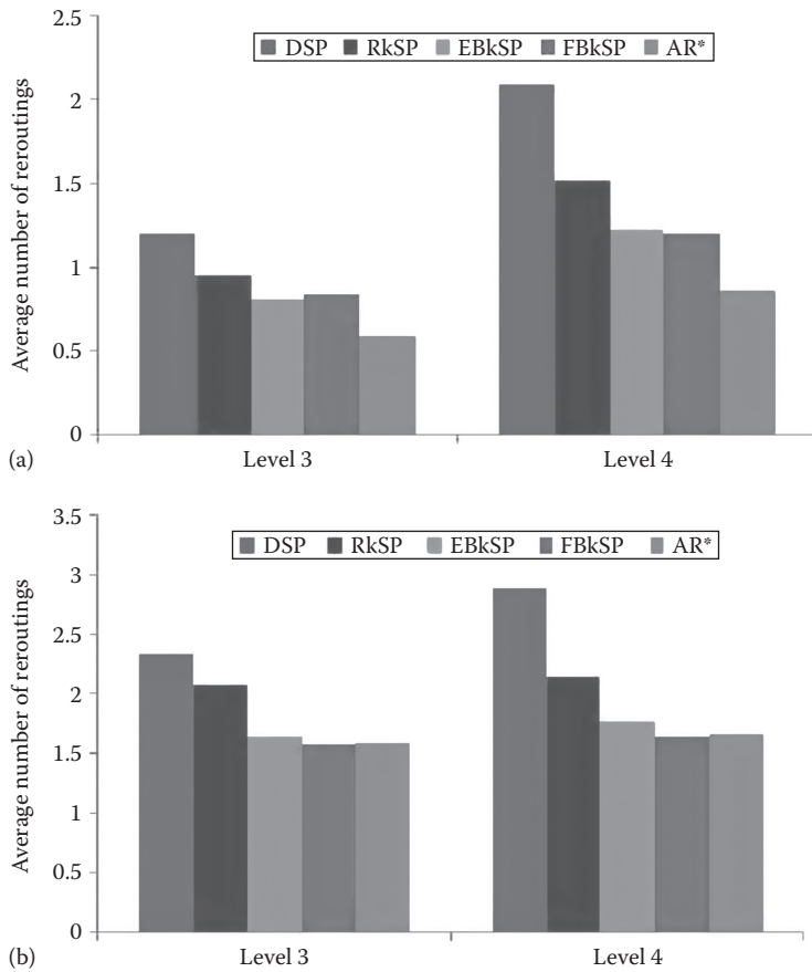
FIGURE 19.9 Average number of reroutings ( L = (3, 4) , k = 4 , urgency = ACI, period = 450 s, \delta = 0.7 , and \beta = 0.05 ): (a) Brooklyn and (b) Newark. (From Pan, J. and Borcea, C., IEEE Trans. Veh. Tech. , 62(8), 3551, 2014.)
