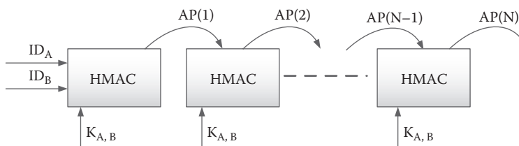
FIGURE 12.1 The AP method used during normal operation.
