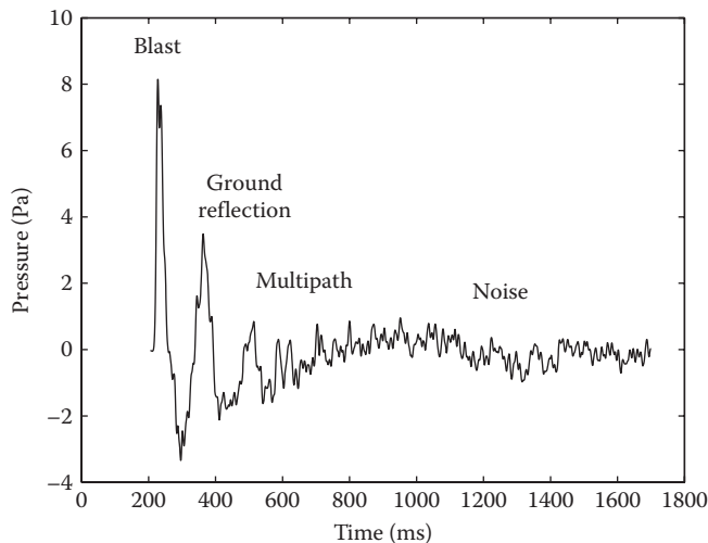
FIGURE 14.7 Muzzle blast wave in the presence of multipath and background noise.
