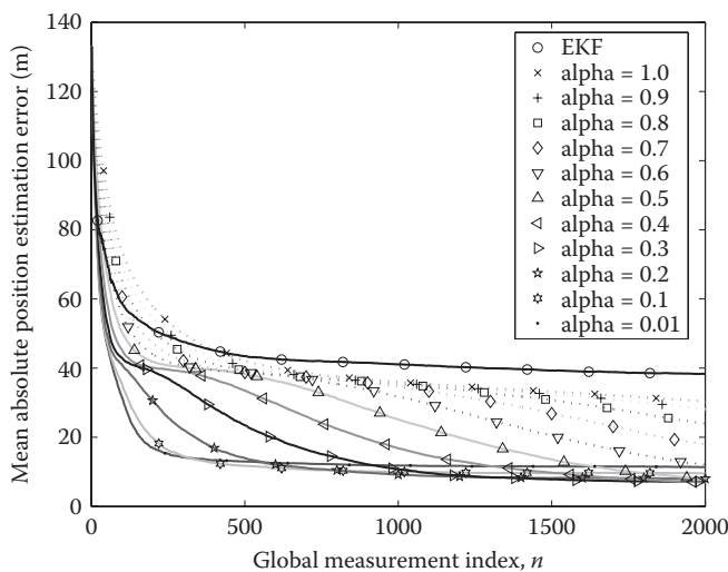
FIGURE 6.5 Comparison of the EKF- and SUKF-based node localization algorithms, for centralized estimation in which all measurements were available without delays ( \alpha is the SUKF scaling parameter).
