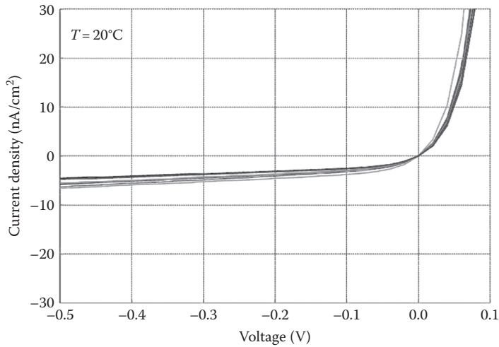
FIGURE 18.21 Experimental results for InGaAs test array demonstrating dark current density for eight separate 300 \times 10, 15 \mu\text{m} pitch pixel test arrays measured across a wafer. The average dark current density for the test arrays at 100 mV reverse bias is 2.95 \text{ nA/cm}^2 at 20^\circ\text{C} . (From Hood, A.D., Proc. SPIE , 8353, 83530A, 2012.)
