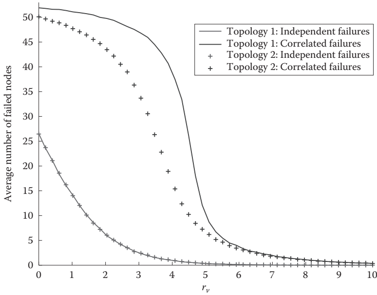
FIGURE 13.6 Average number of failed nodes as a function of the homogeneous robustness vector for Topologies 1 and 2.
