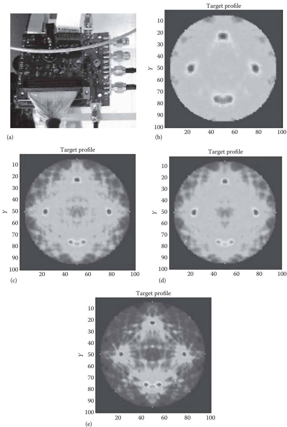
FIGURE 17.2 (a) Data-acquisition hardware of the ultrasound imaging device. (b–e) Reconstructed images of five point targets corresponding to various FMCW bandwidth.
