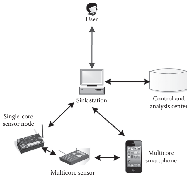
FIGURE 5.10 Multicore architecture.
