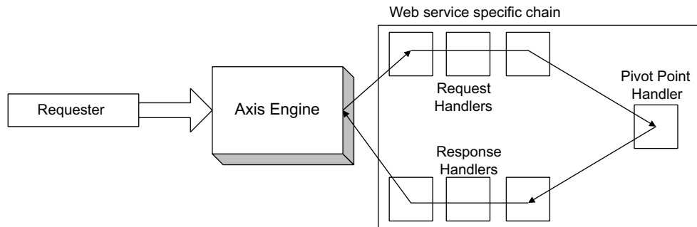
Figure 18.2 Axis allows the developer to define a series of handlers to partition the work performed on a web service request or response.
