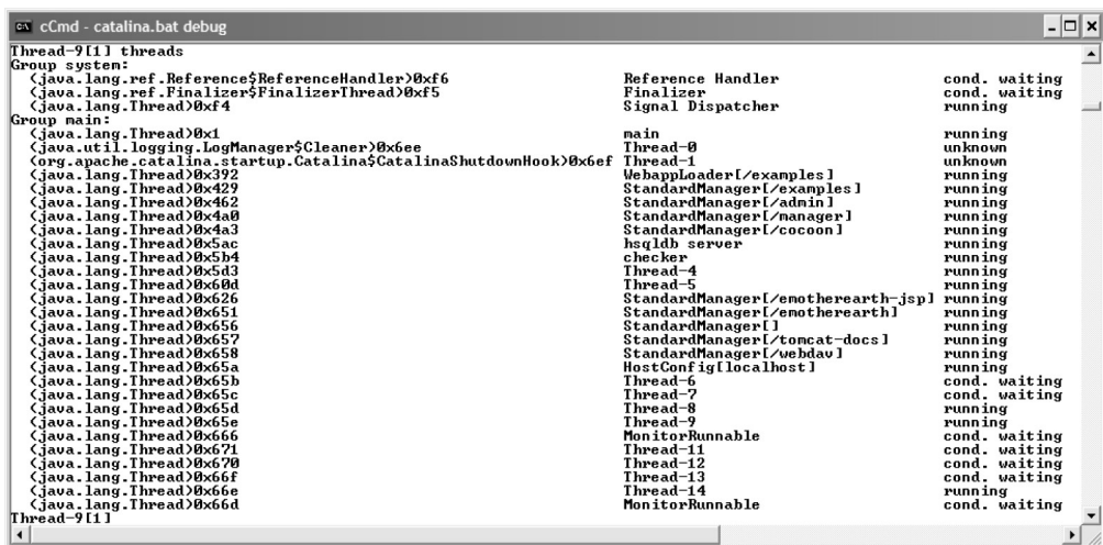
Figure 16.3 The threads command shows all currently running threads in the servlet engine.
