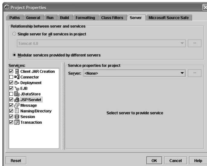
Figure 16.16 JBuilder's Project Properties dialog box lets you assign the application server and its characteristics on a project-by-project basis.
