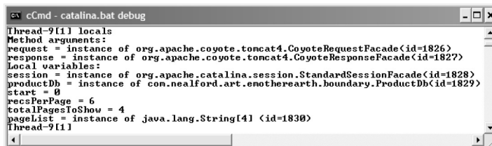
Figure 16.6 The locals command prints a list of all the local variables in scope for the current thread context.
