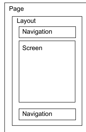
Figure 1.7 The Page assembler encapsulates the other assemblers to construct a complete page. The Layout assembler handles the general layout of the page, which consists of one or more Navigation assemblers and a Screen assembler.
