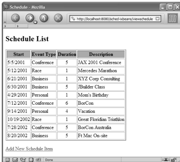
Figure 8.5 The InternetBeans Express schedule application's View page is the combination of DataExpress, InternetBeans Express components, and an HTML template.
