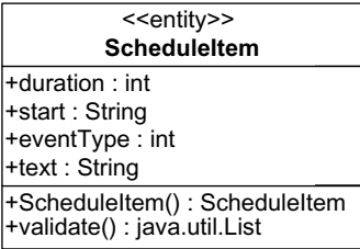
Figure 12.3 The ScheduleItem class represents an entity in the schedule application and should appear in diagrams with the entity stereotype.
