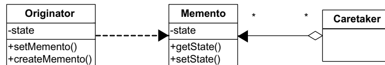
Figure 13.7 The participant classes in the Memento design pattern revolve around their relationship to the Memento class.
