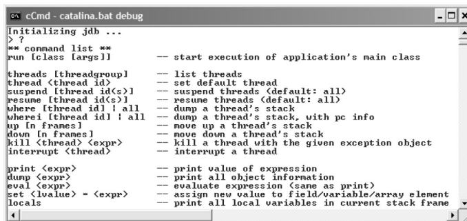
Figure 16.2 The help command (a question mark) lists all the commands available for the debugger.
