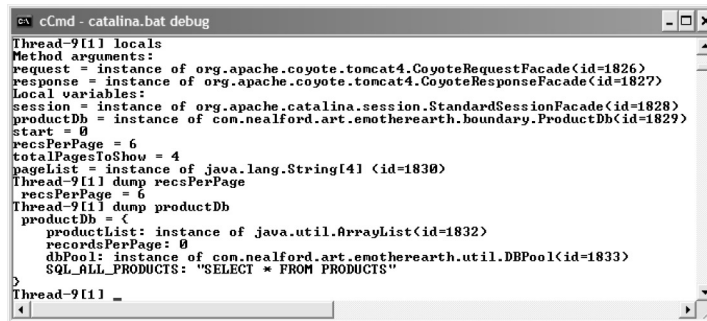
Figure 16.7 The dump command allows you to investigate the contents of object references. In this case, it shows all the fields of the ProductDb class, including the values of the primitives and strings.
