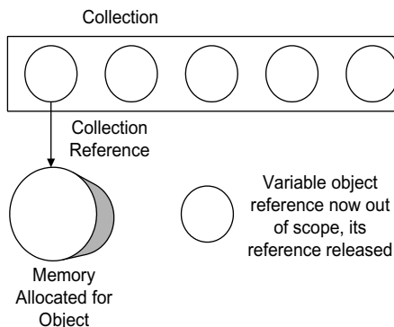
Figure 14.8 Variable object reference has been reclaimed, but the garbage collection cannot clean up the memory because the collection still holds a reference.
