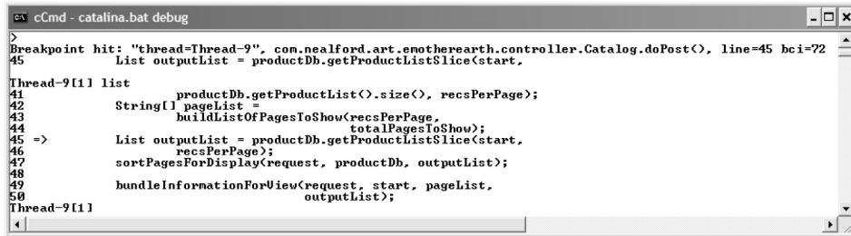
Figure 16.5 The breakpoint halts the application and the list command shows the current execution context.
