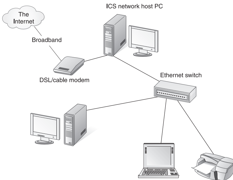
Figure 5-1 Home networking via Internet Connection Sharing (ICS)
