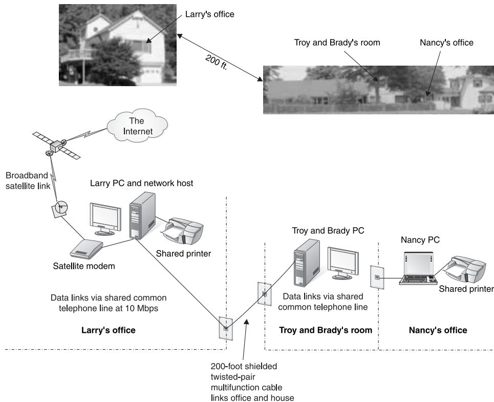
Figure 1-1 A Windows-based home network that uses phoneline connectivity
