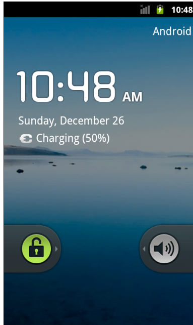
Figure 78. Android keyguard
